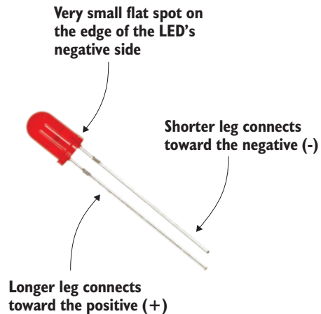
Figure 6.12 LEDs have two legs (wires) coming out of them. The longer leg is called the anode and connects to the positive side of the circuit. The shorter one is called the cathode and connects to the negative side of a circuit.
