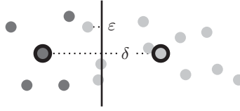
Figure 13.2 If we reassign the leftmost light point – which is at a distance of \varepsilon from the bisecting hyperplane – to the dark cluster, then this decreases the objective function by 2\varepsilon\delta , where \delta is the distance between the two centers.
