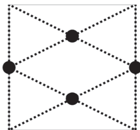
Figure 20.2 Gadget for a variable in the NP -hardness reduction. Figure from Vavasis (2009).
