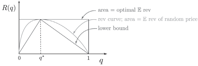
Figure 27.1 Geometric proof of Proposition 27.3.
