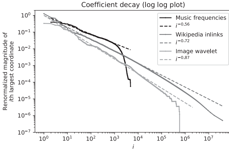
Figure 7.1 Coefficient decay in three example signals of different domains. In each example, the i th largest coordinate has magnitude decaying as i^{-\alpha} for some \alpha \in (0.5, 1) . The audio data contain the frequencies in a 1/10 second clip of a popular music video; the image data are the Haar wavelet representation of one frame of this video; the graph data are the number of inlinks per page on English Wikipedia.
