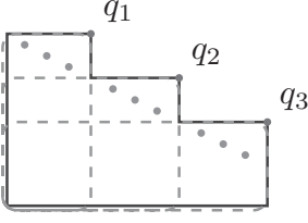
Figure 3.2 A “harder” point set for the computation of the maxima set in two dimensions.
