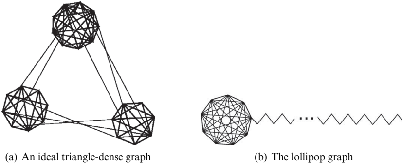
Figure 28.4 Two examples of \delta -triangle-dense graphs with \delta close to 1.
