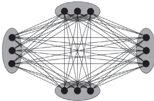
Figure 28.2 The Moon–Moser graph with n = 12 vertices.
