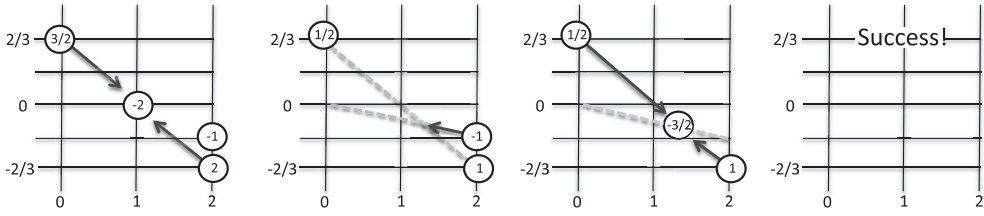
Figure 23.1 Depiction of a successful sequence of “moves” in the game corresponding to the inequality \left(\sum_j x_j^2 y_j^{-2/3}\right)^2 \left(\sum_j x_j^2 y_j^{-1/3}\right)^{-1} \left(\sum_j x_j\right)^{-2} \left(\sum_j y_j^{2/3}\right)^{3/2} \geq 1 , showing that the inequality is true. The first diagram illustrates the initial configuration of positive and negative weights, together with the “Hölder-type move” that takes one unit of weight from each of the points at (0, 2/3) and (2, -2/3) and moves it to the point (1, 0) , canceling out the weight of -2 that was initially at (1, 0) . The second diagram illustrates the resulting configuration, together with the “ \ell_p monotonicity move” that moves the -1 weight at location (2, -1/3) toward the origin by a factor of 2/3 while scaling it by a factor of 3/2 , resulting in a point at (4/3, -2/9) with weight -3/2 , which is now collinear with the remaining two points. The third diagram illustrates the final “Hölder-type move” that moves the two points with positive weight to their weighted average, zeroing out all weights.
