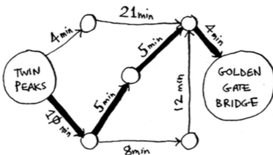
WEIGHTED GRAPH (USE DIJKSTRA'S ALGORITHM)
