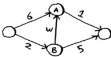
WEIGHTED GRAPH
