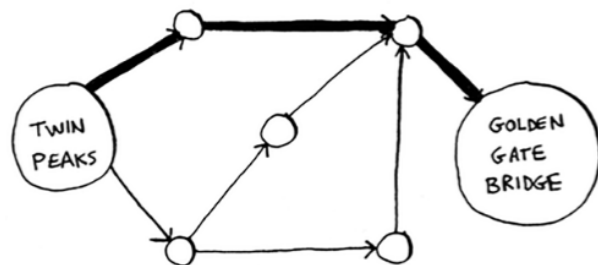
UNWEIGHTED GRAPH (USE BFS)
