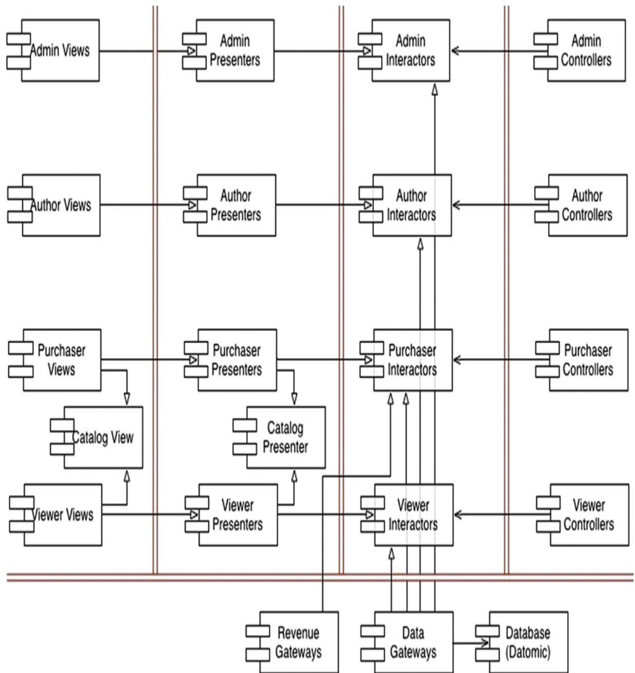
Figure 33.2 A preliminary component architecture
