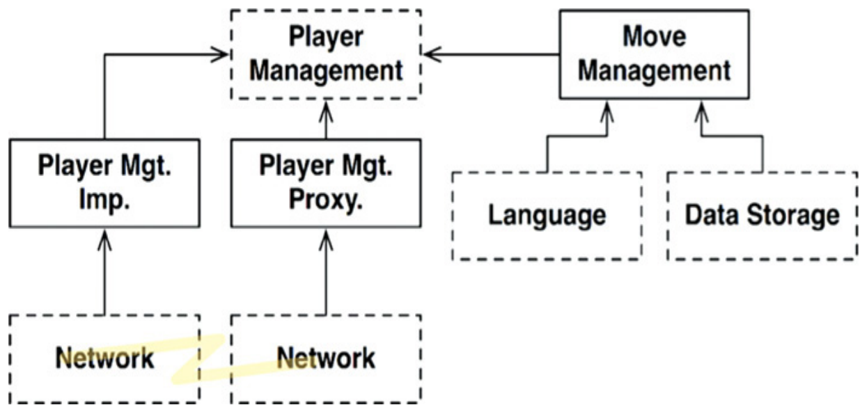
Figure 25.7 Adding a micro-service API
