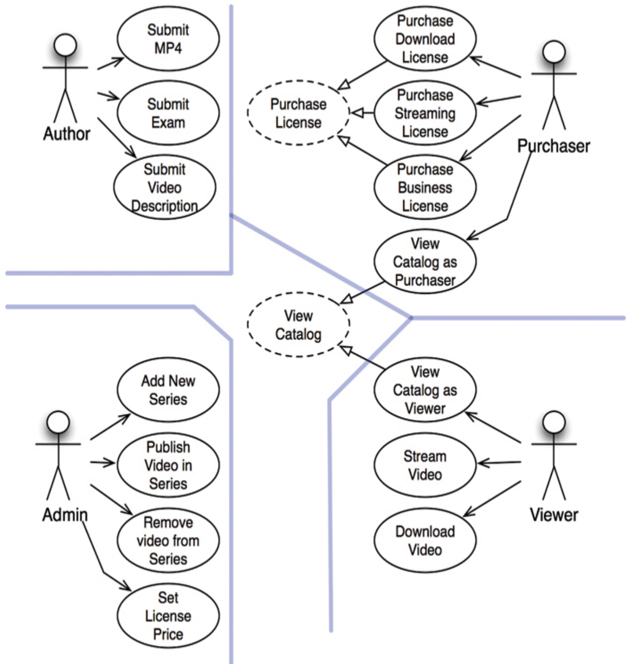
Figure 33.1 A typical use-case analysis
