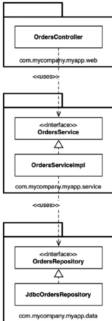
Figure 34.1 Package by layer
