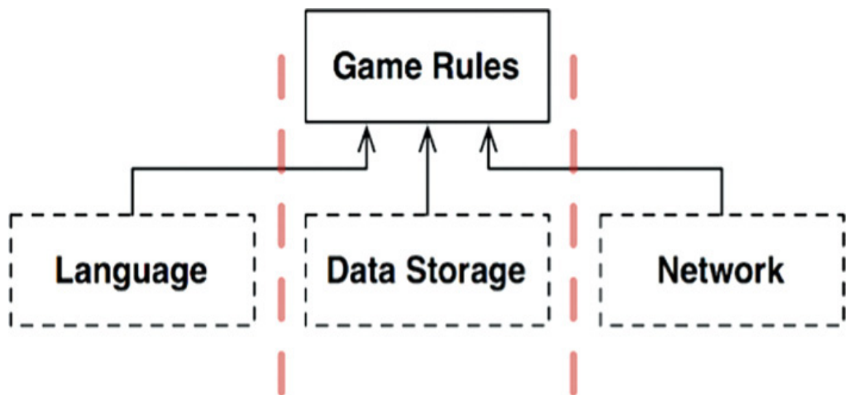
Figure 25.5 Adding a network component
