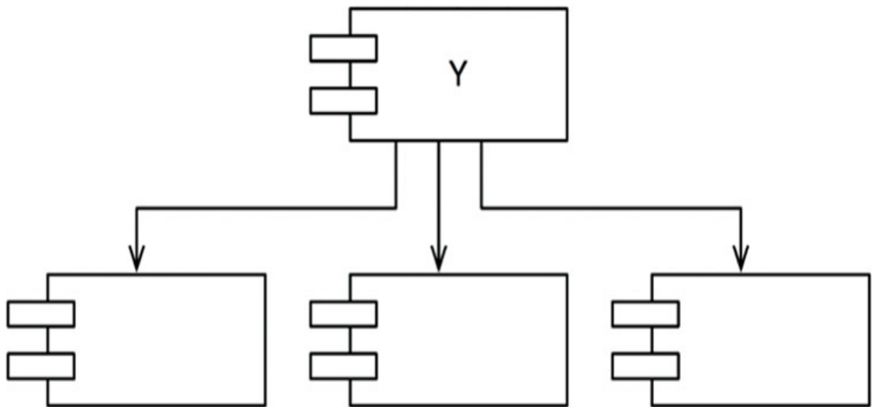
Figure 14.6 y : a very unstable component
