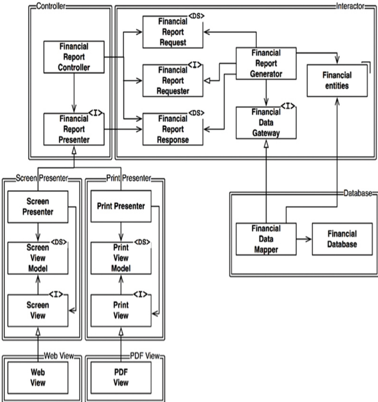
Figure 8.2 Partitioning the processes into classes and separating the classes into components
