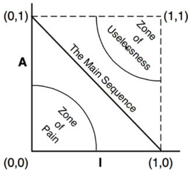
Figure 14.13 Zones of exclusion
