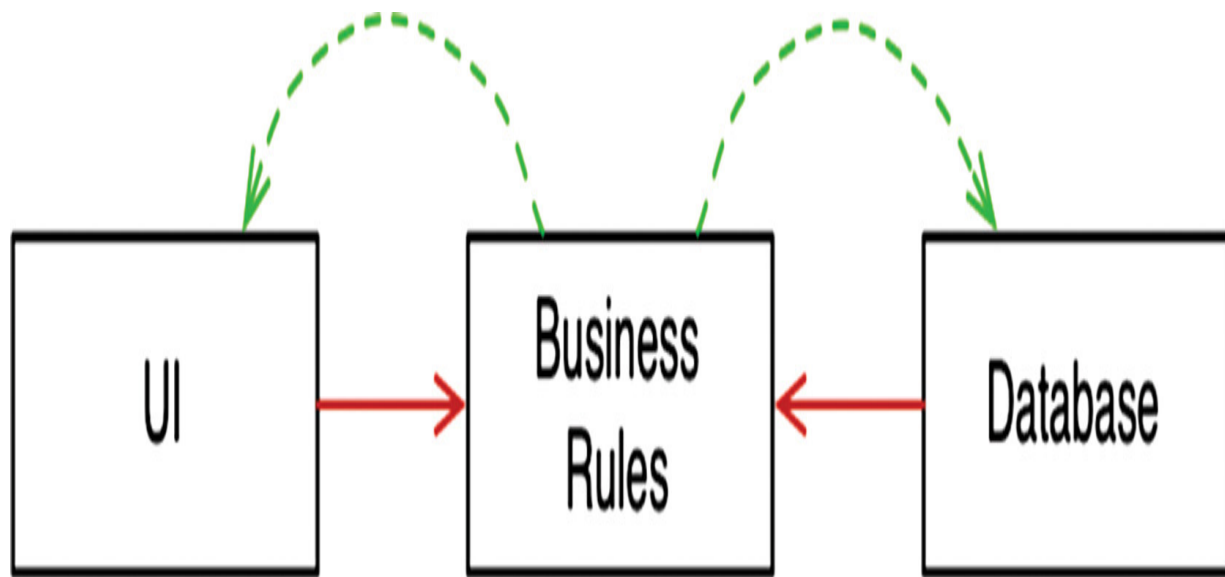
Figure 5.3 The database and the user interface depend on the business rules
