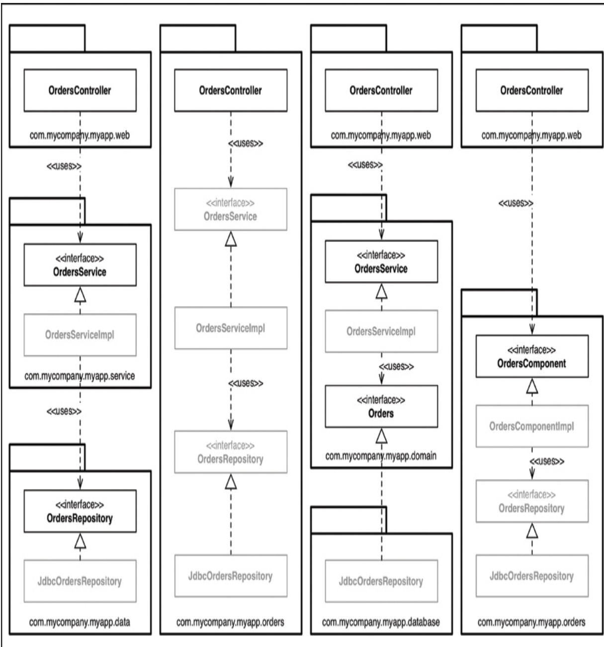
Figure 34.8 Grayed-out types are where the access modifier can be made more restrictive
