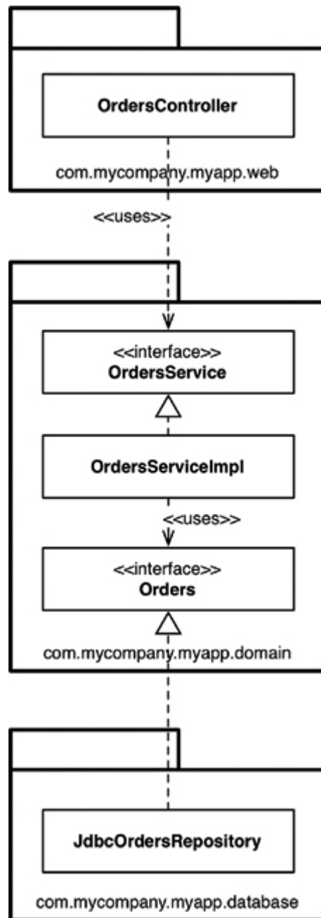
Figure 34.4 View orders use case
