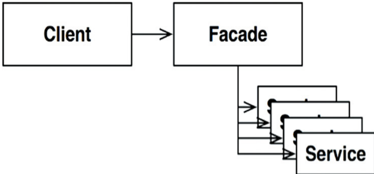
Figure 24.2 The Facade pattern
