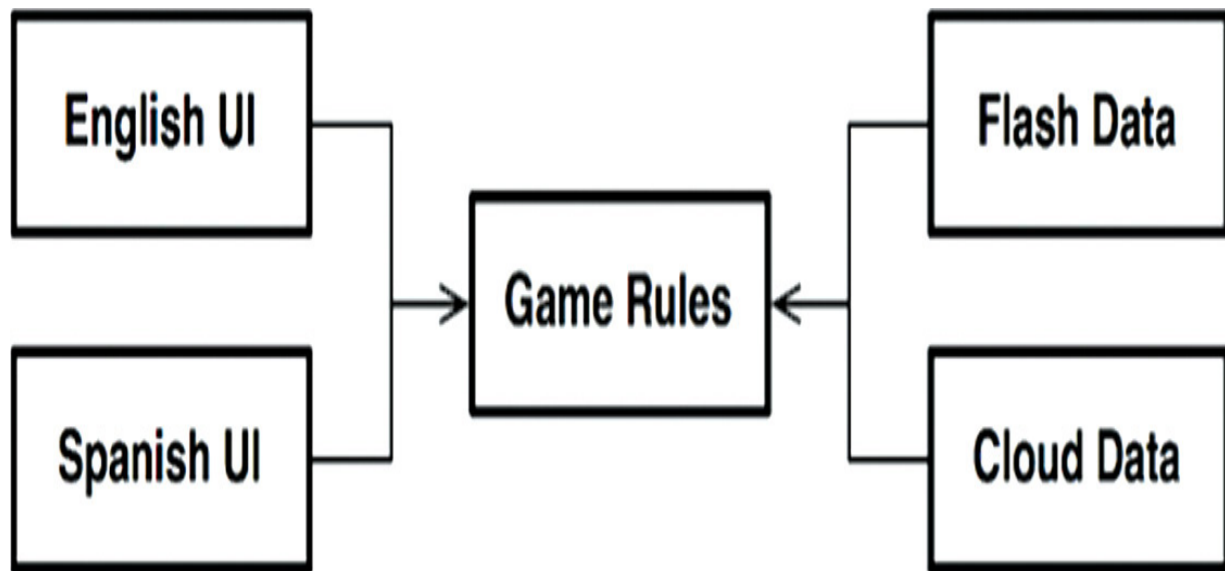
Figure 25.2 Following the Dependency Rule
