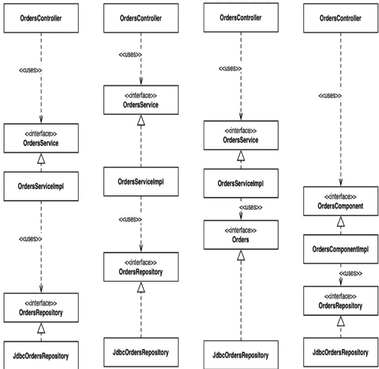
Figure 34.7 All four architectural approaches are the same
