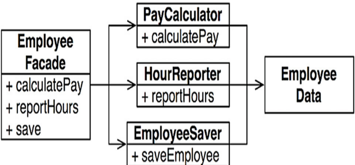
Figure 7.4 The Facade pattern
