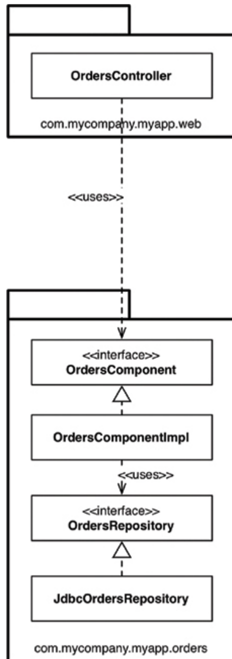
Figure 34.6 View orders use case
