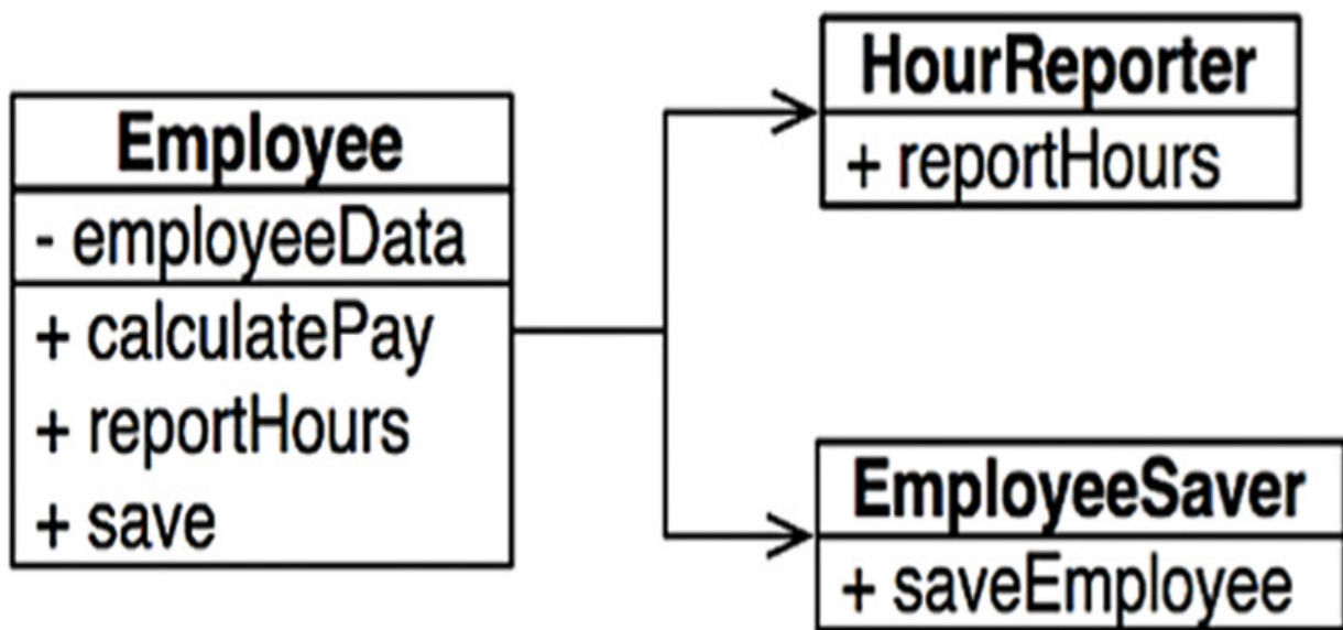
Figure 7.5 The most important method is kept in the original Employee class and used as a Facade for the lesser functions
