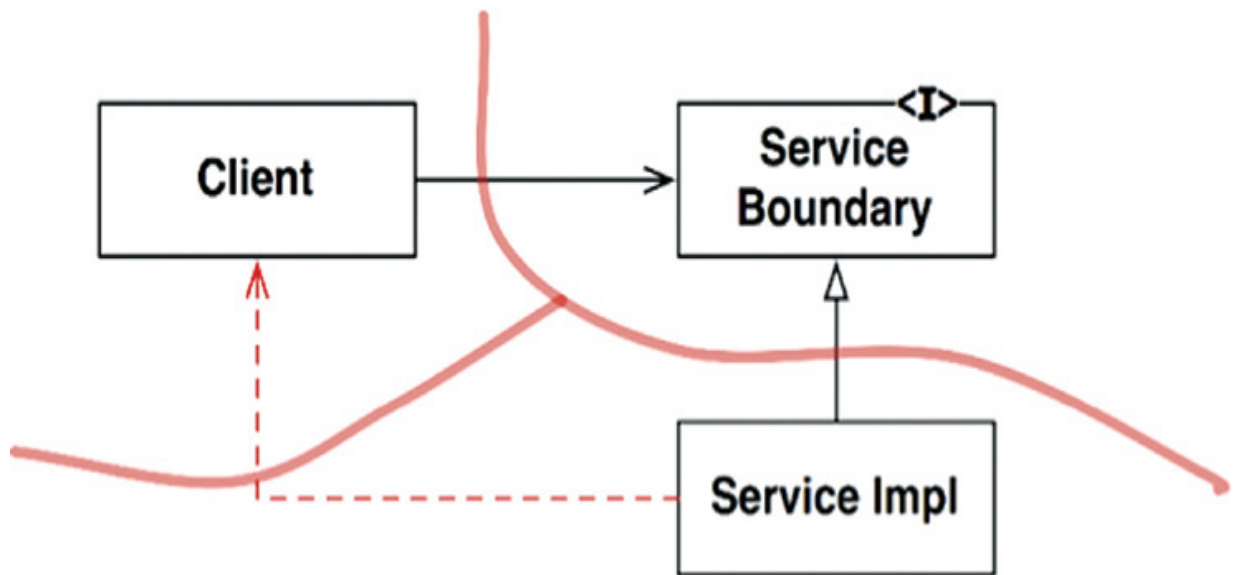
Figure 24.1 The Strategy pattern
