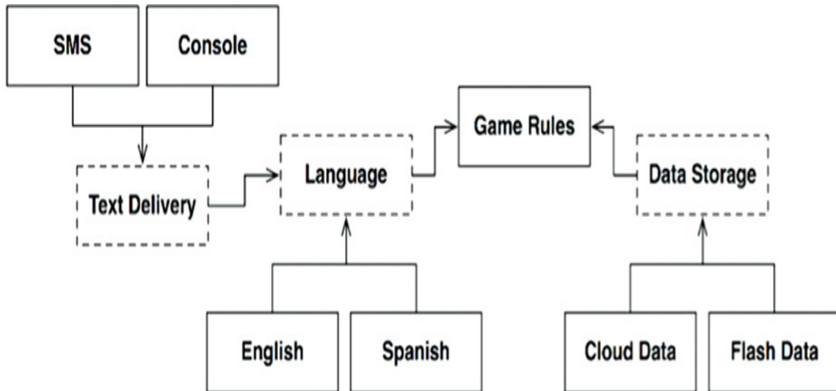
Figure 25.3 The revised diagram
