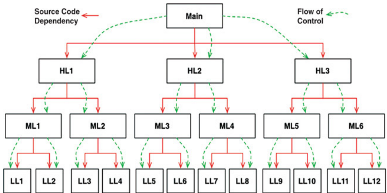
Figure 5.1 Source code dependencies versus flow of control
