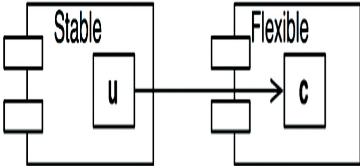
Figure 14.10 U within Stable uses C within Flexible
