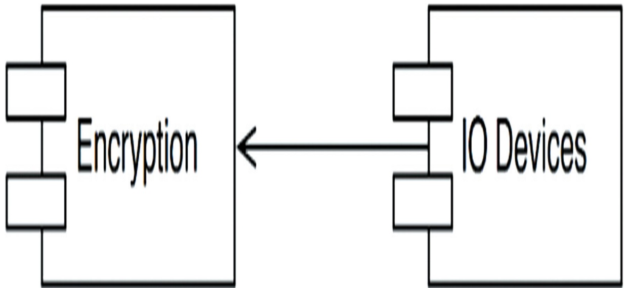
Figure 19.3 Lower-level components should plug in to higher-level components
