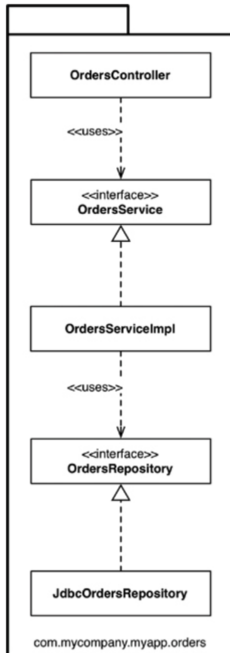
Figure 34.2 Package by feature
