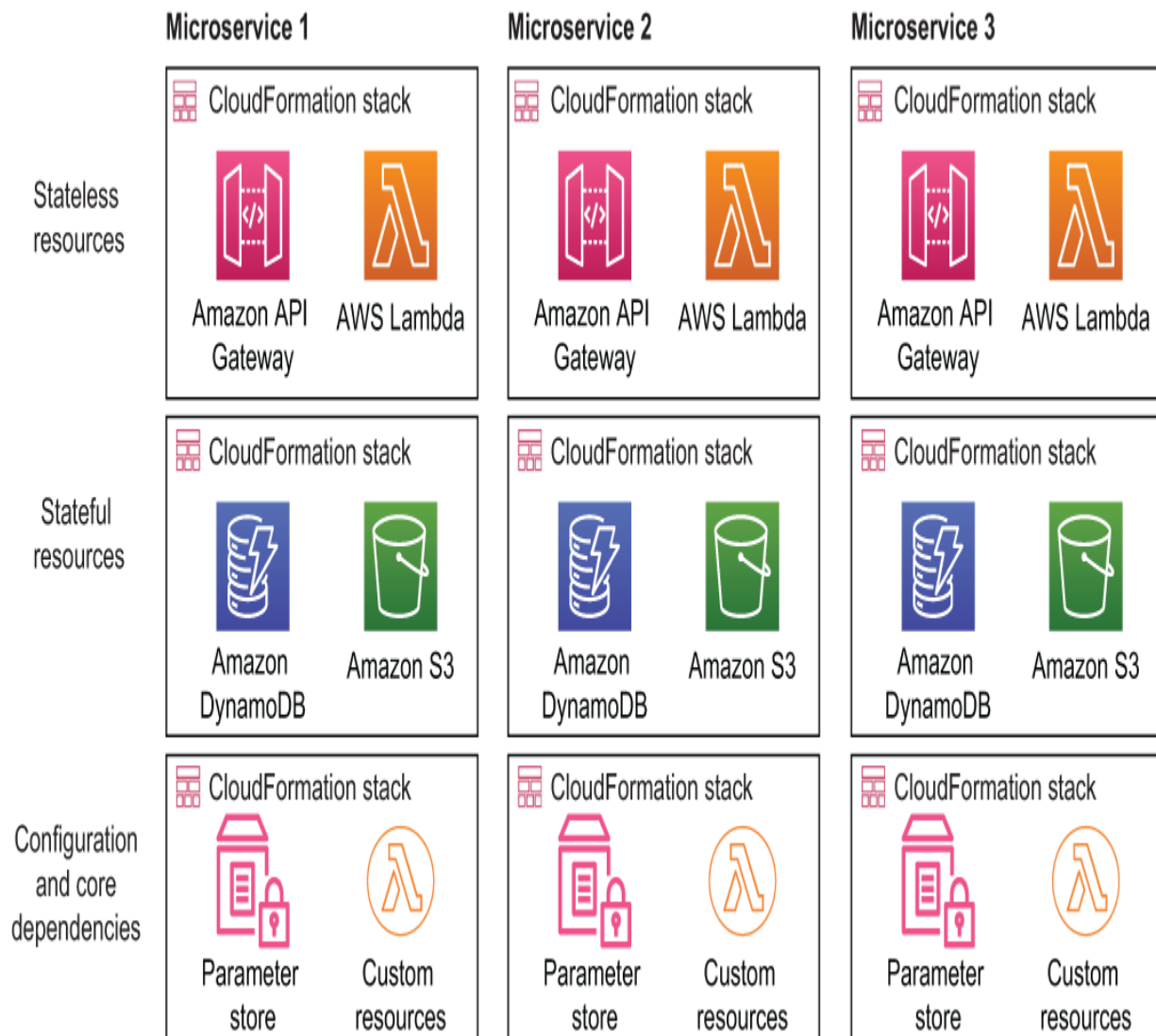
Figure 5.4 Each microservice is in its own CloudFormation stack, which makes it easy to deploy.
