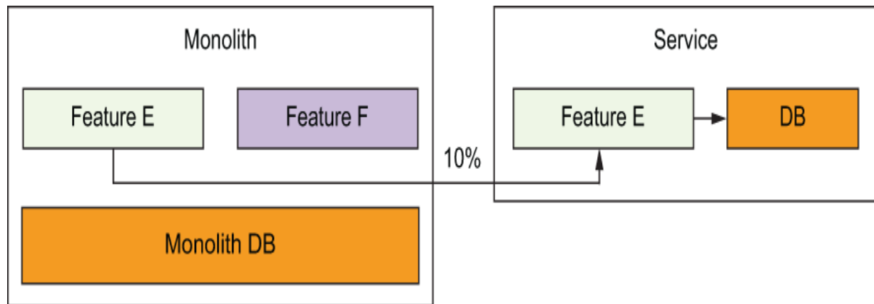
Figure 4.8 Even without ALBs, you can still proxy requests by modifying the monolith.
