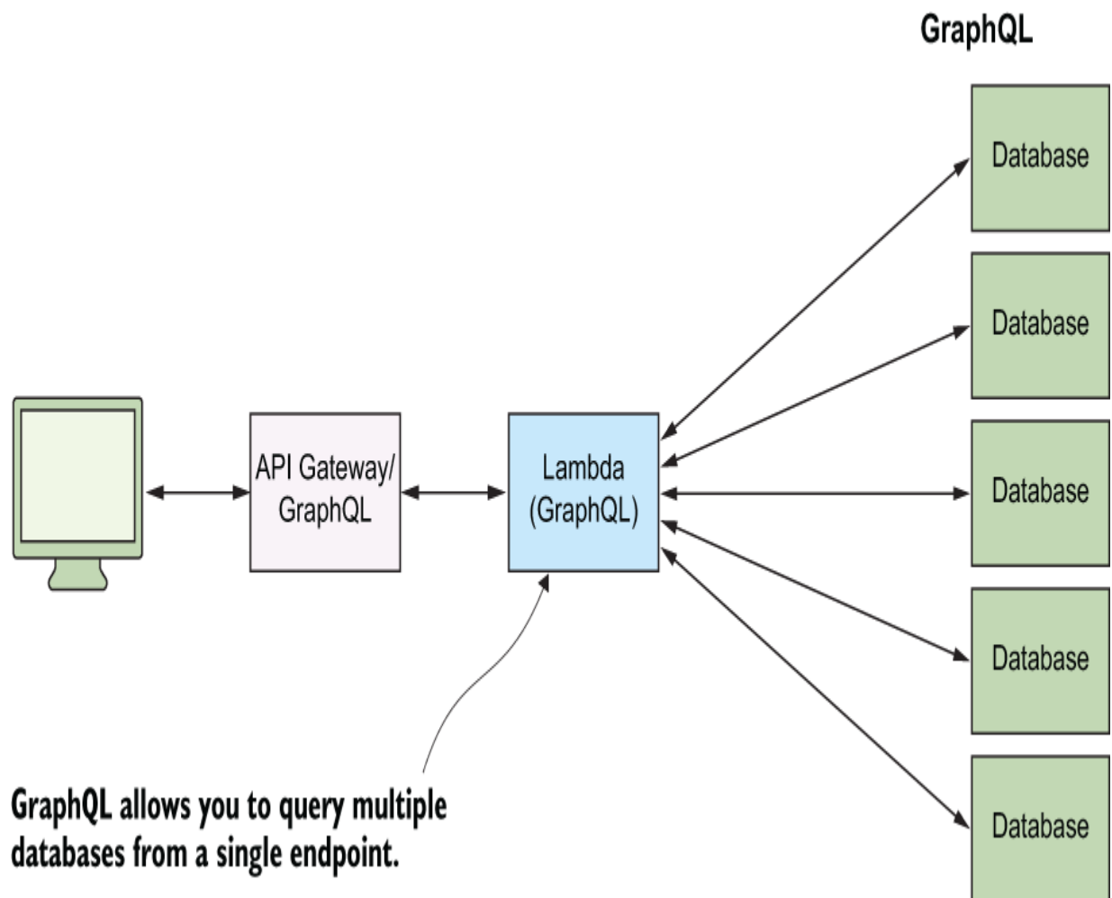
Figure 5.6 A GraphQL library running in a Lambda function can query multiple databases and, using schema stitching, produce a result relevant for each individual client.
