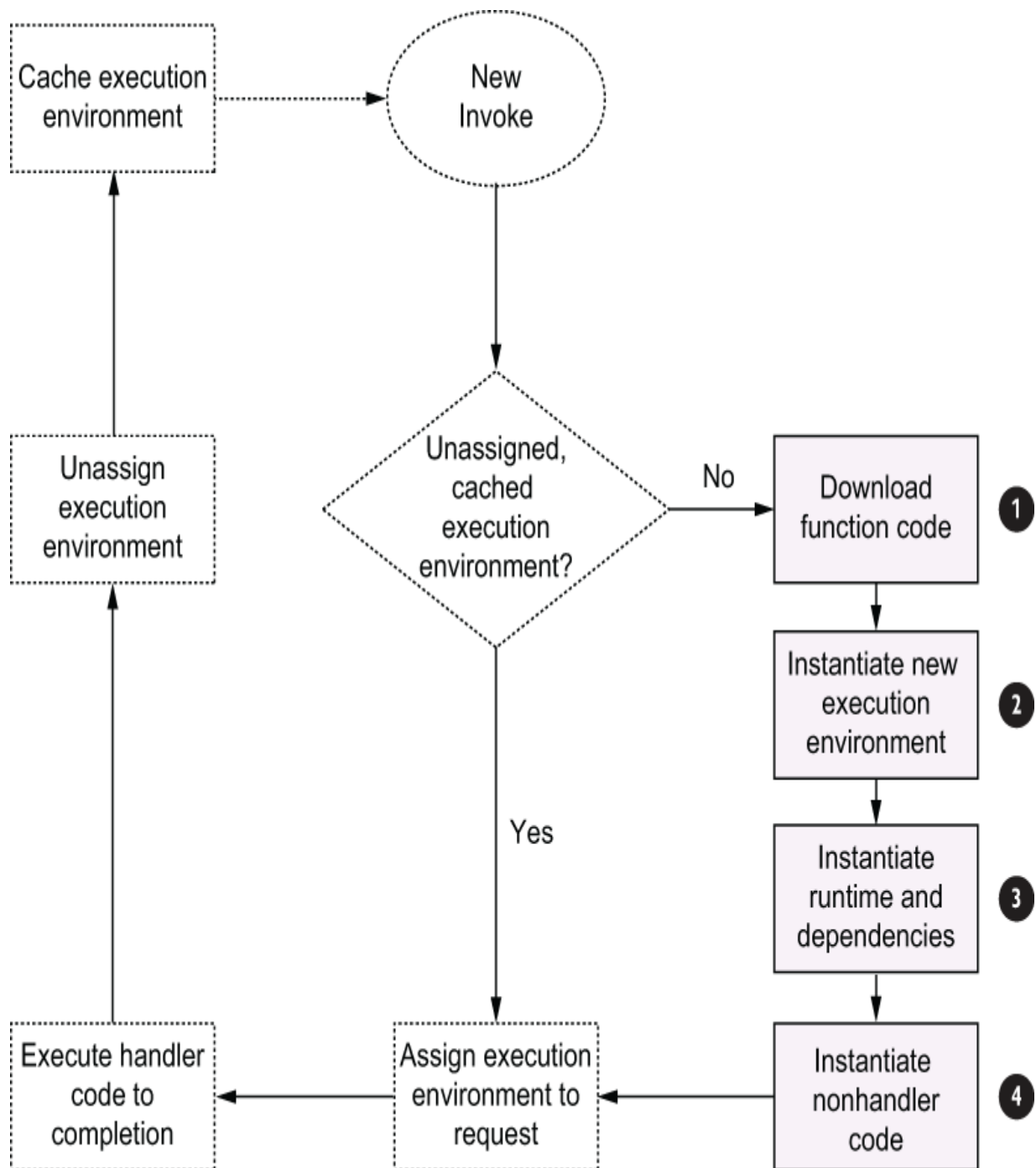
Figure 10.9 Lambda execution request lifecycle
