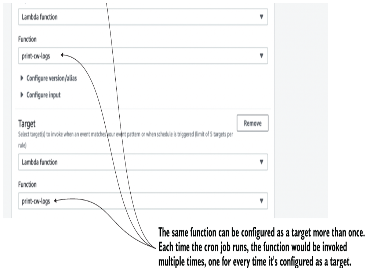
Figure 7.3 You can add the same Lambda function as a target for an EventBridge rule multiple times.
