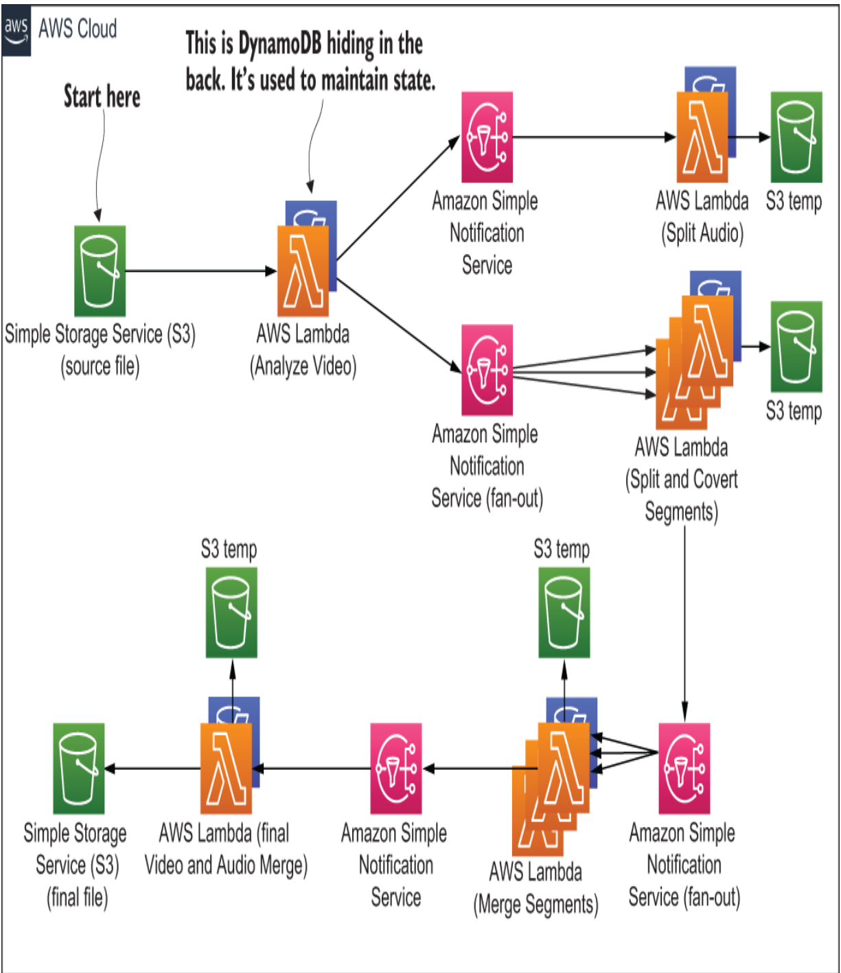
Figure 8.6 The SNS and S3 architecture for the serverless transcoder
