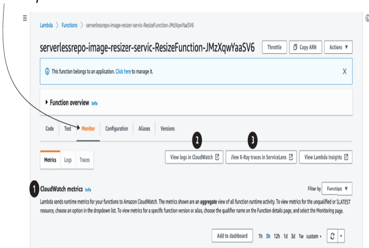
Figure 10.7 Monitoring tab for AWS Lambda functions showing three tools for monitoring
