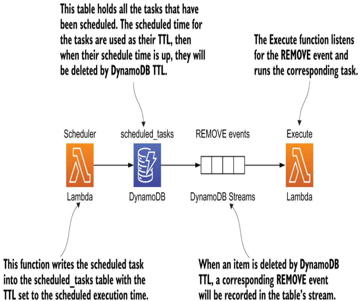
Figure 7.7 High-level architecture using DynamoDB TTL to run ad hoc scheduled tasks.
