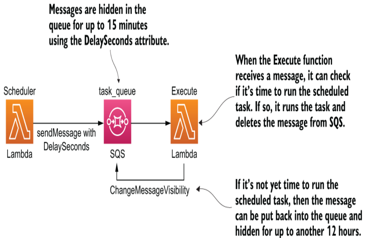
Figure 7.17 High-level architecture of using SQS to schedule ad hoc tasks
