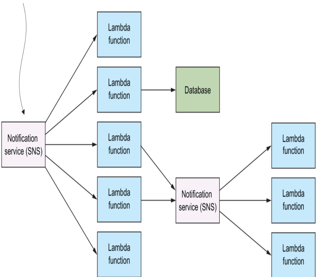
Figure 3.9 The fan-out pattern is useful because many AWS services (such as S3) can't invoke more than one Lambda function at a time when an event takes place.
