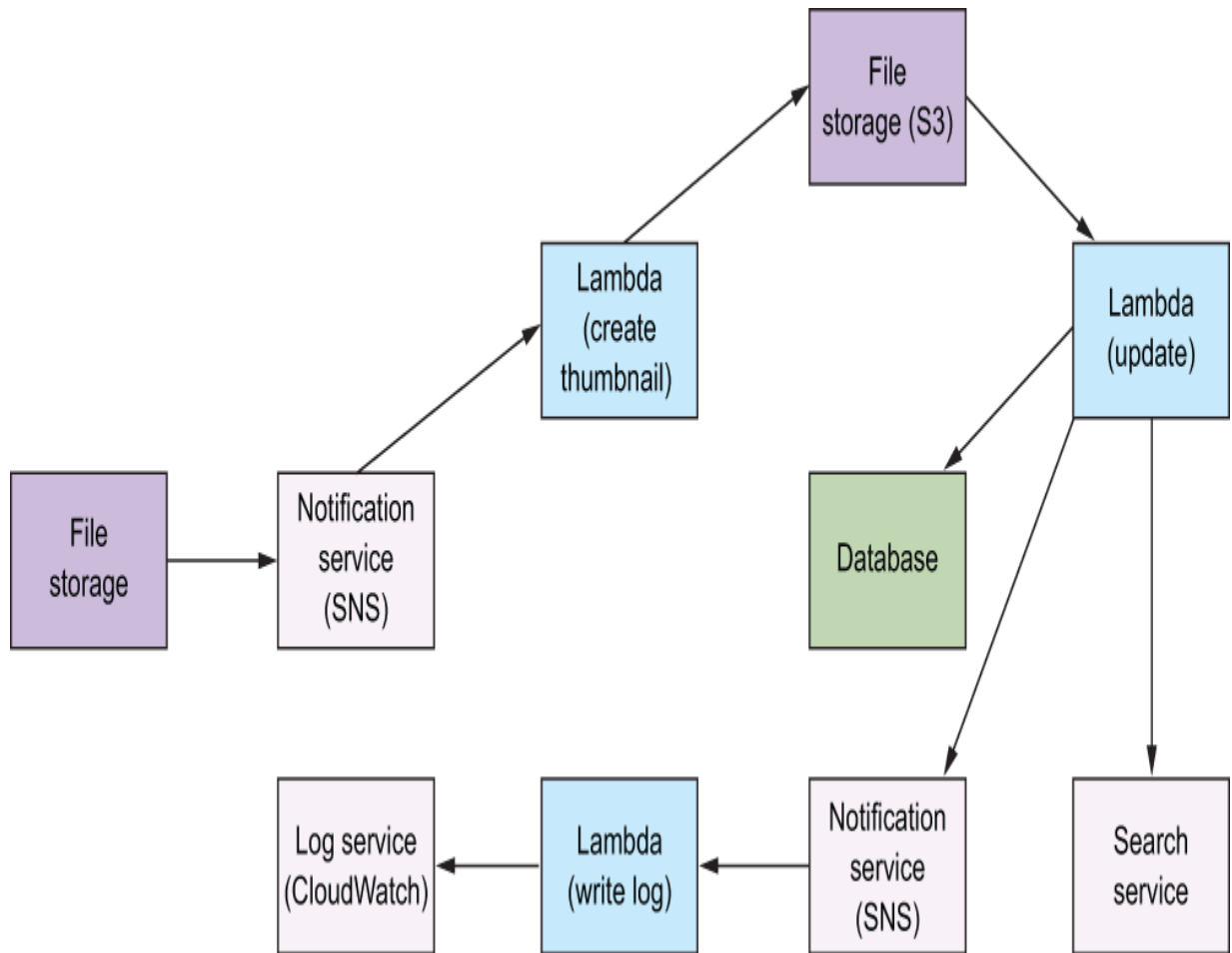
Figure 3.10 The compute-as-glue architecture uses Lambda functions to connect different services and APIs to achieve a task. In this pipeline, a simple image transformation results in a new file, an update to a database, an update to a search service, and a new entry to a log service.
