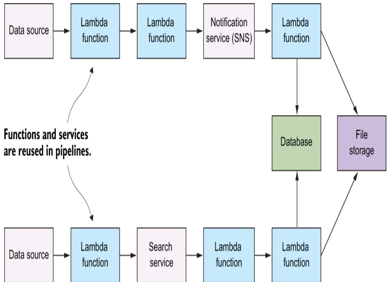
Figure 3.11 The pipes and filters pattern encourages the construction of pipelines to pass and transform data from its origin (pump) to its destination (sink).
