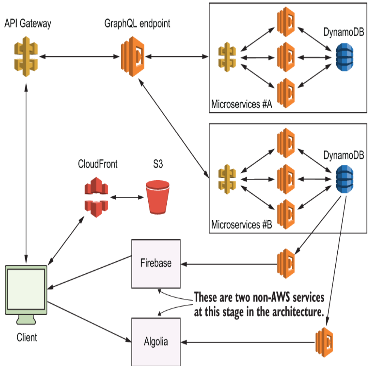
Figure 5.10 A high-level overview of the A Cloud Guru architecture as it was going through a transition
