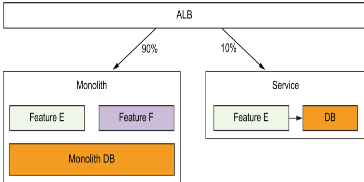
Figure 4.7 You can use the Application Load Balancer (ALB) to distribute traffic between the monolith and the new microservices. This allows you to minimize impact of unforeseen problems to a subset of users.
