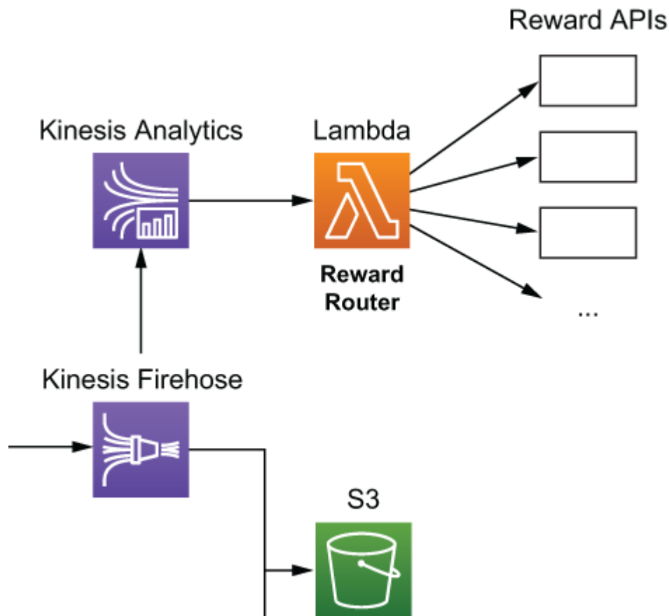
Figure 6.4 The Yle team uses Kinesis Data Analytics and Lambda to reward different personalization models in real time.
