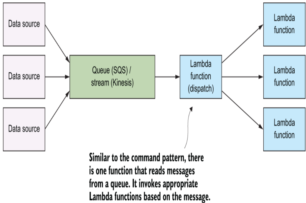
Figure 3.6 The messaging pattern and its many variations are popular in distributed environments.
