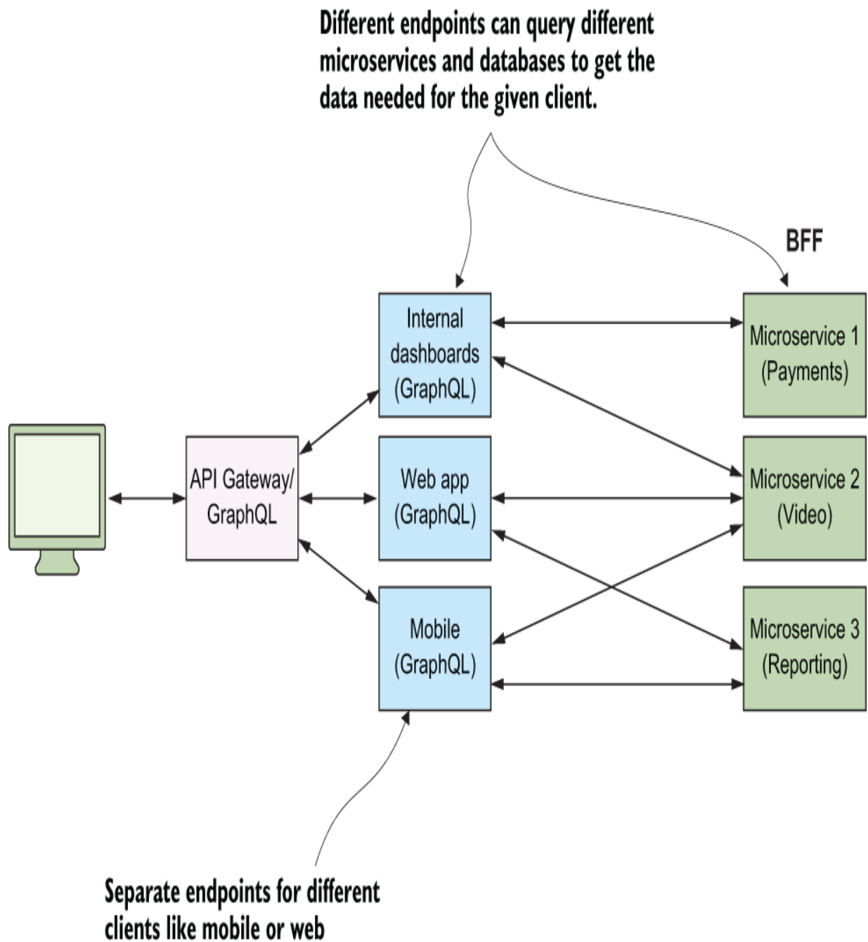
Figure 5.7 An example of the BFF pattern that can be applied to microservices and multiple clients
