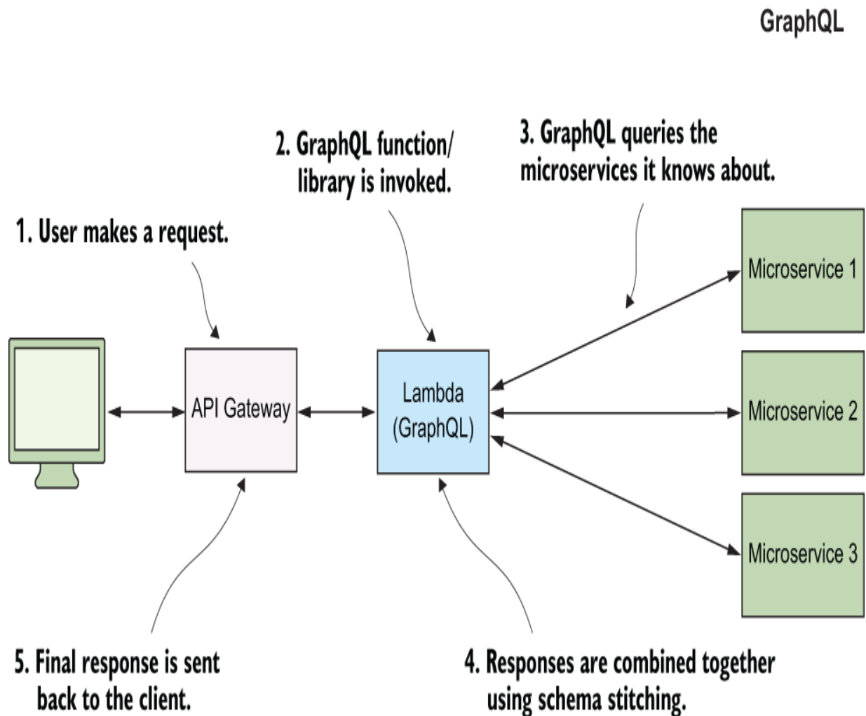
Figure 5.8 The GraphQL endpoint serves as the central point for clients that need data.
