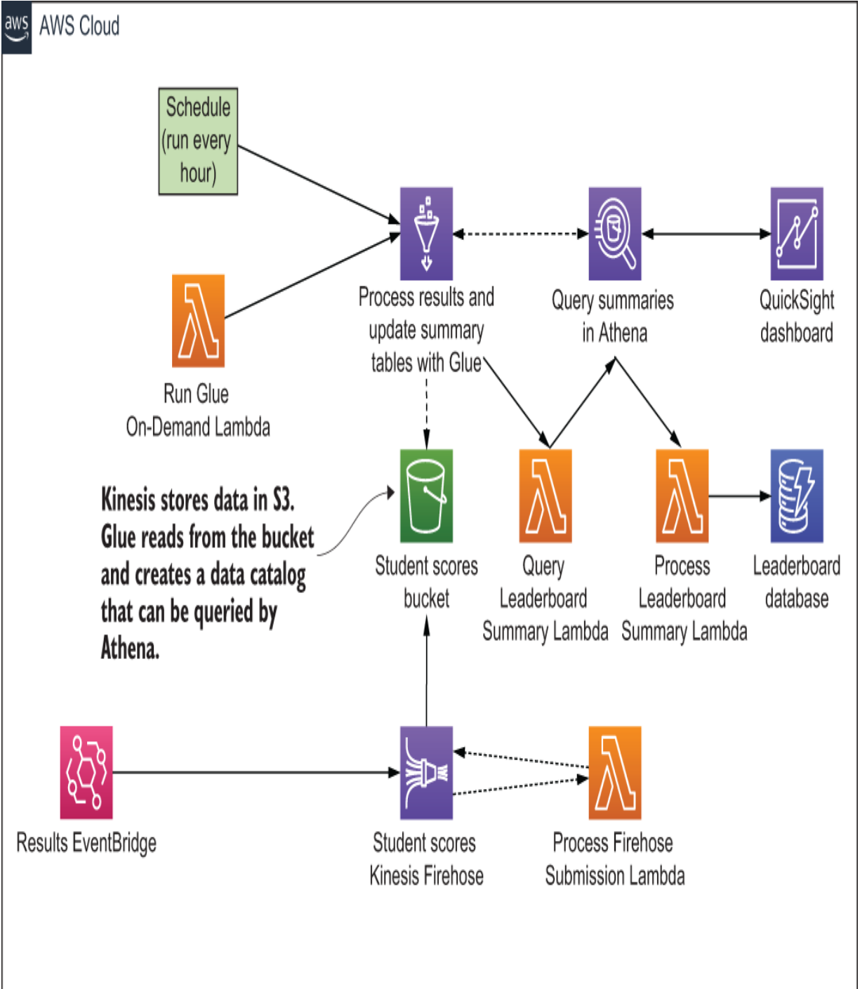
Figure 9.4 The Analytics Service architecture includes Glue, Athena, DynamoDB, Kinesis Firehose, QuickSight, and Lambda.
