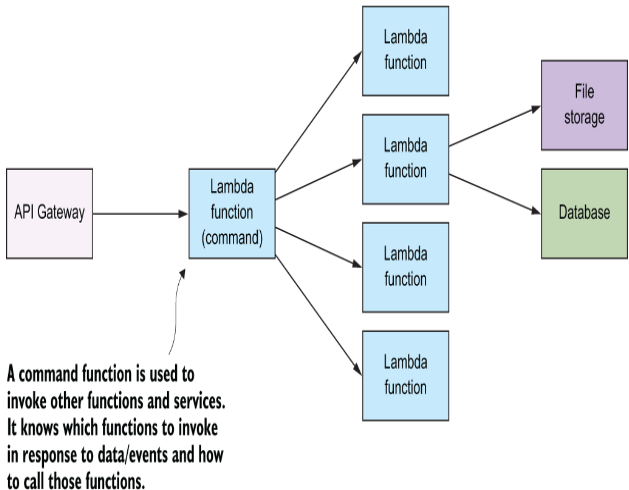
Figure 3.5 The command pattern invokes and controls functions and services from a single function.
