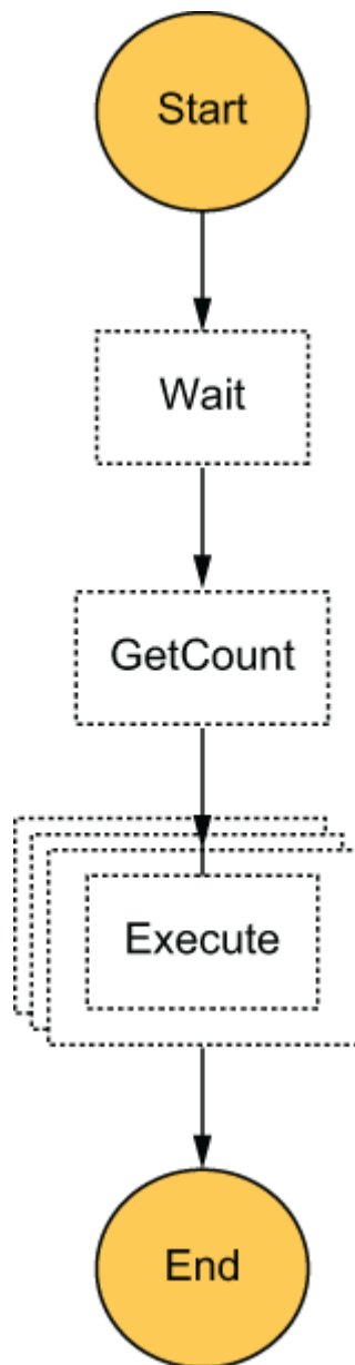
Figure 7.16 An alternative design for the state machine that can run tasks in batches in parallel
