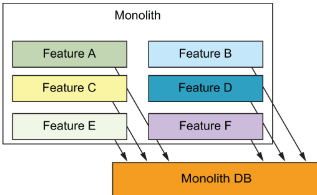
Figure 4.3 A monolithic system where everything has direct access to a shared database
