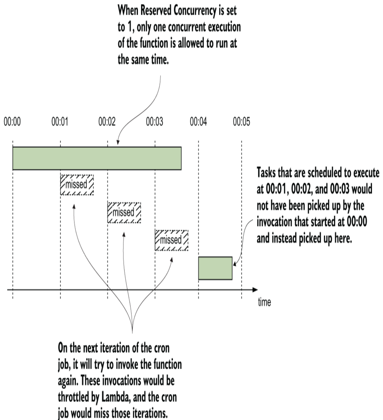
Figure 7.5 If we limit Reserve Concurrency to 1, then there will be only one concurrent execution of the Lambda function running at any moment. This means some cron job cycles will be skipped.
