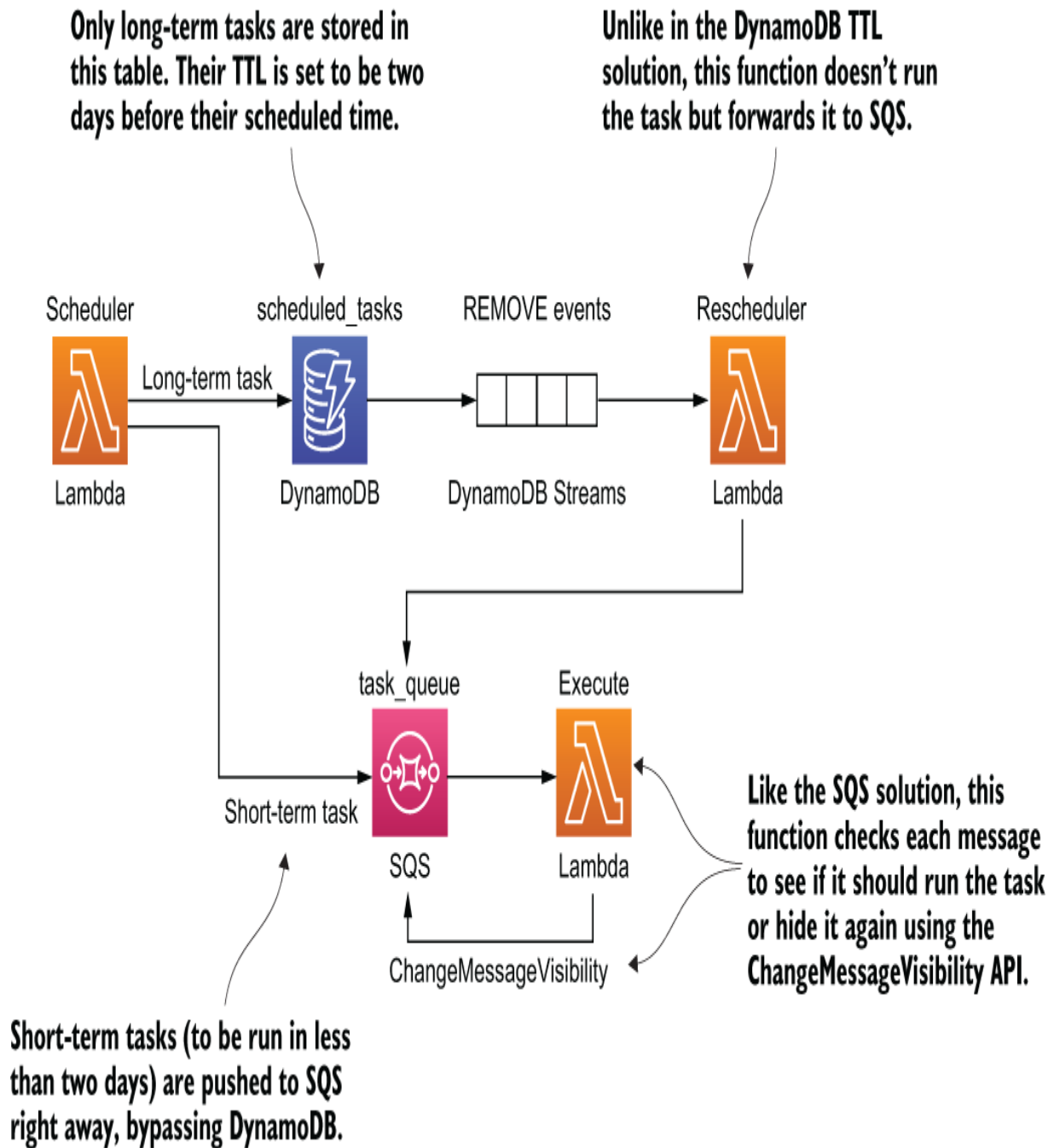
Figure 7.18 High-level architecture of combining DynamoDB TTL with SQS
