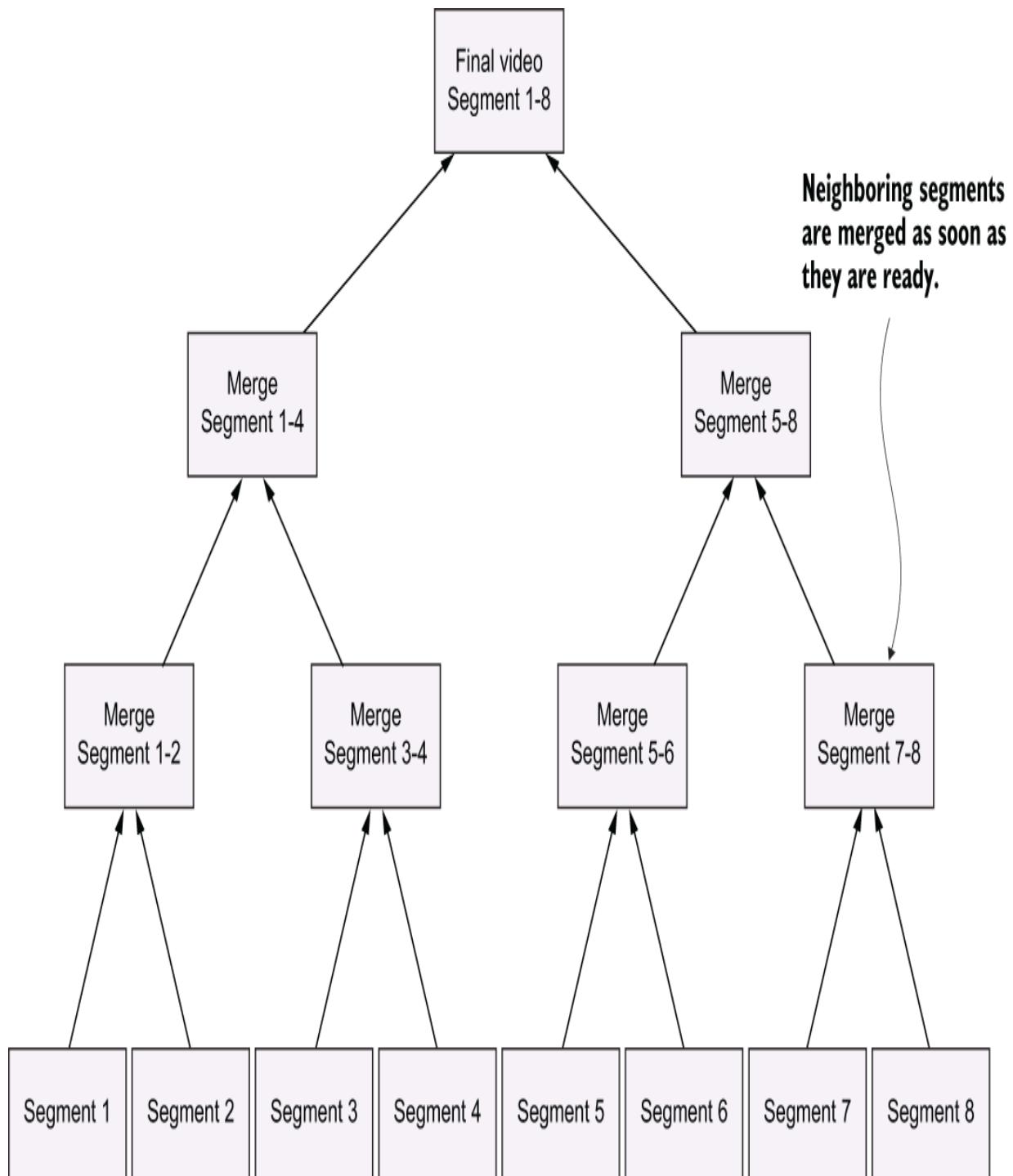
Figure 8.3 Segments are merged together into a new video. The beauty of our engine is that neighboring segments can be merged as
