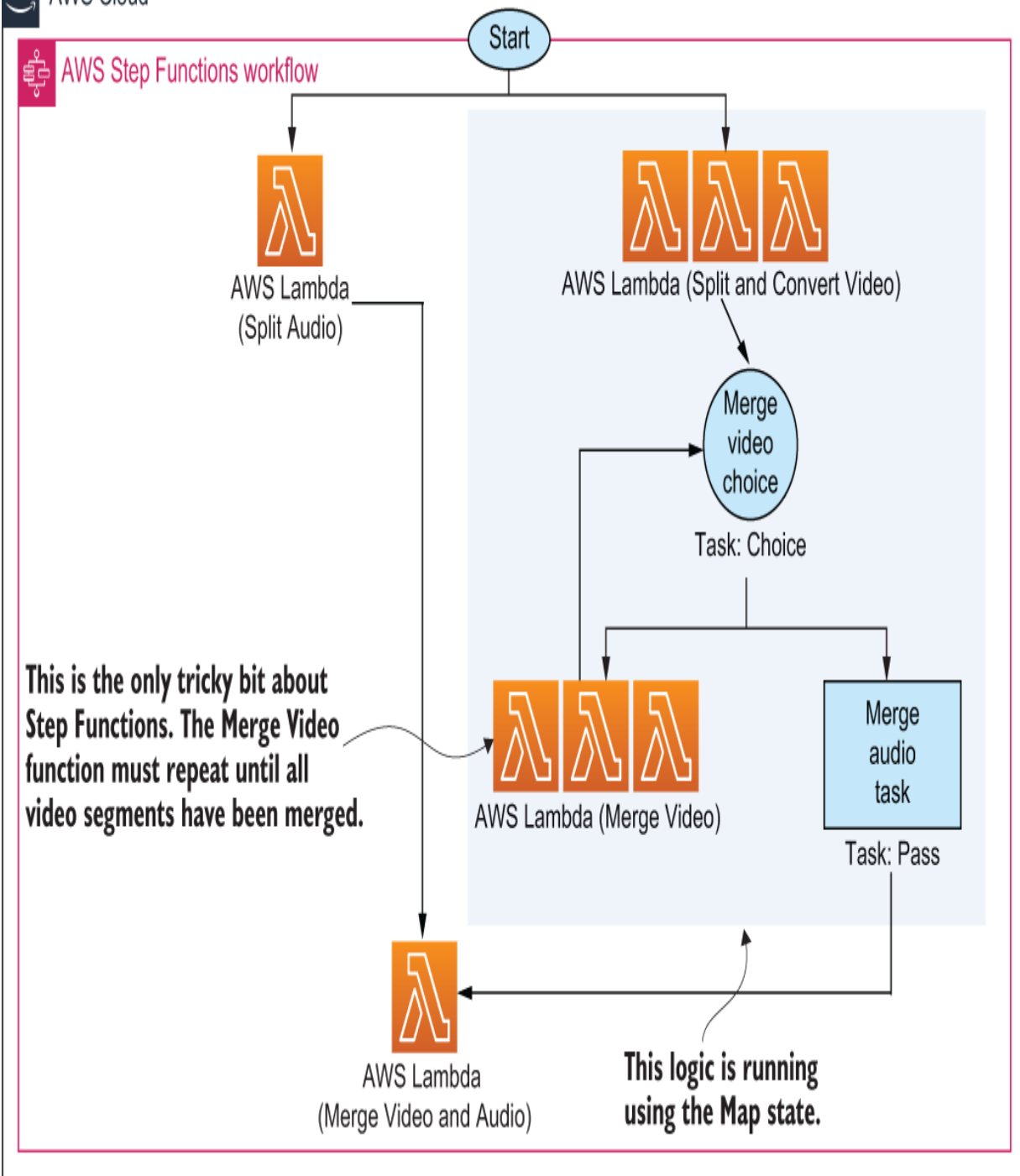
Figure 8.5 The Step Functions execution workflow does all the work in our transcoder. The video is split, converted, and merged again us-
