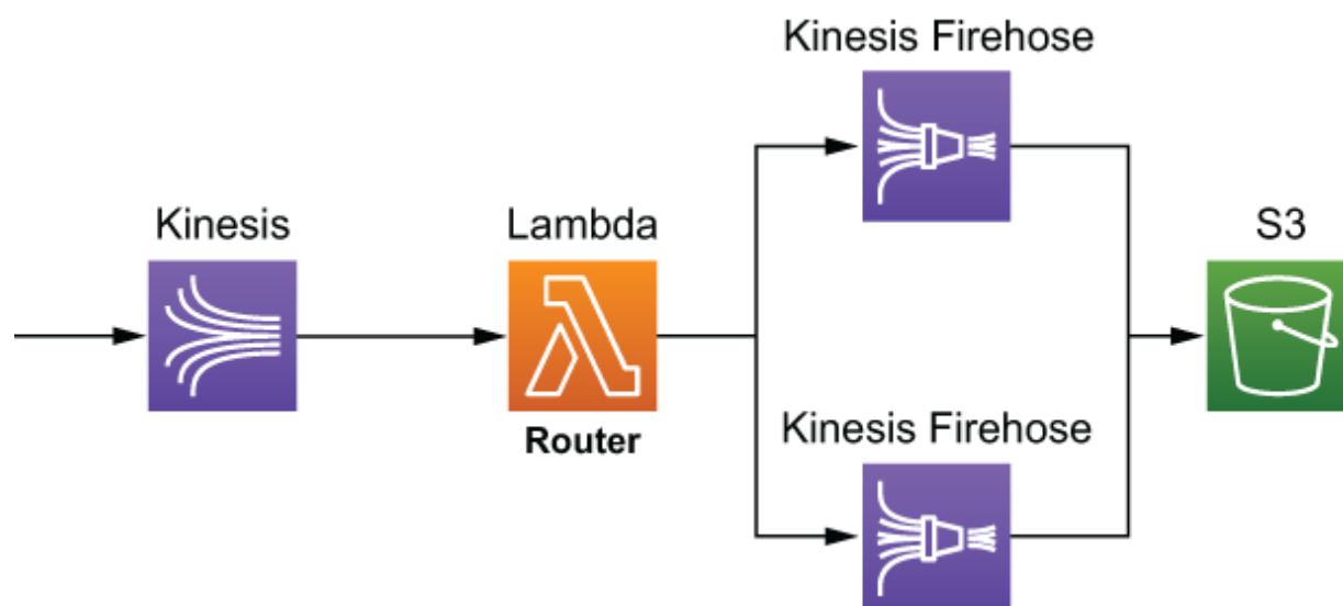
Figure 6.3 The Router function routes incoming events to a number of Kinesis Firehose streams, one for each type of event. The streams then batch, transform, and convert the data into Apache Parquet format and write it to S3.
