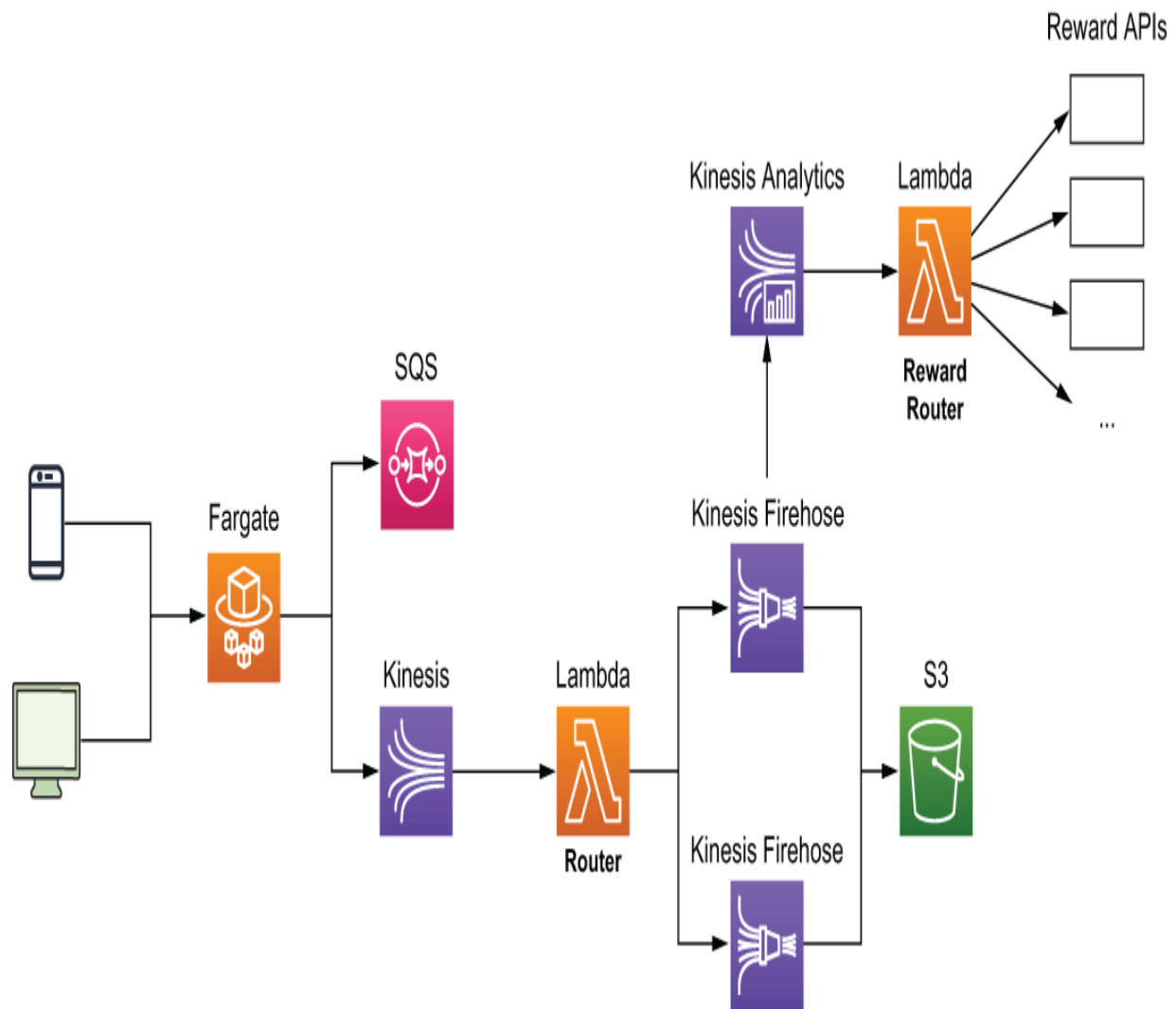
Figure 6.5 Yle's data pipeline architecture. They use Fargate to run the ingestion API because of cost and performance considerations and then process the ingested events in real time using Kinesis Data Streams, Kinesis Firehose, and Lambda. The data is transformed, compressed, and converted to Apache Parquet format and stored in S3 as the data lake. At the same time, they also use Kinesis Data Analytics to perform real-time aggregations and use Lambda to reward the relevant personalization ML models.
