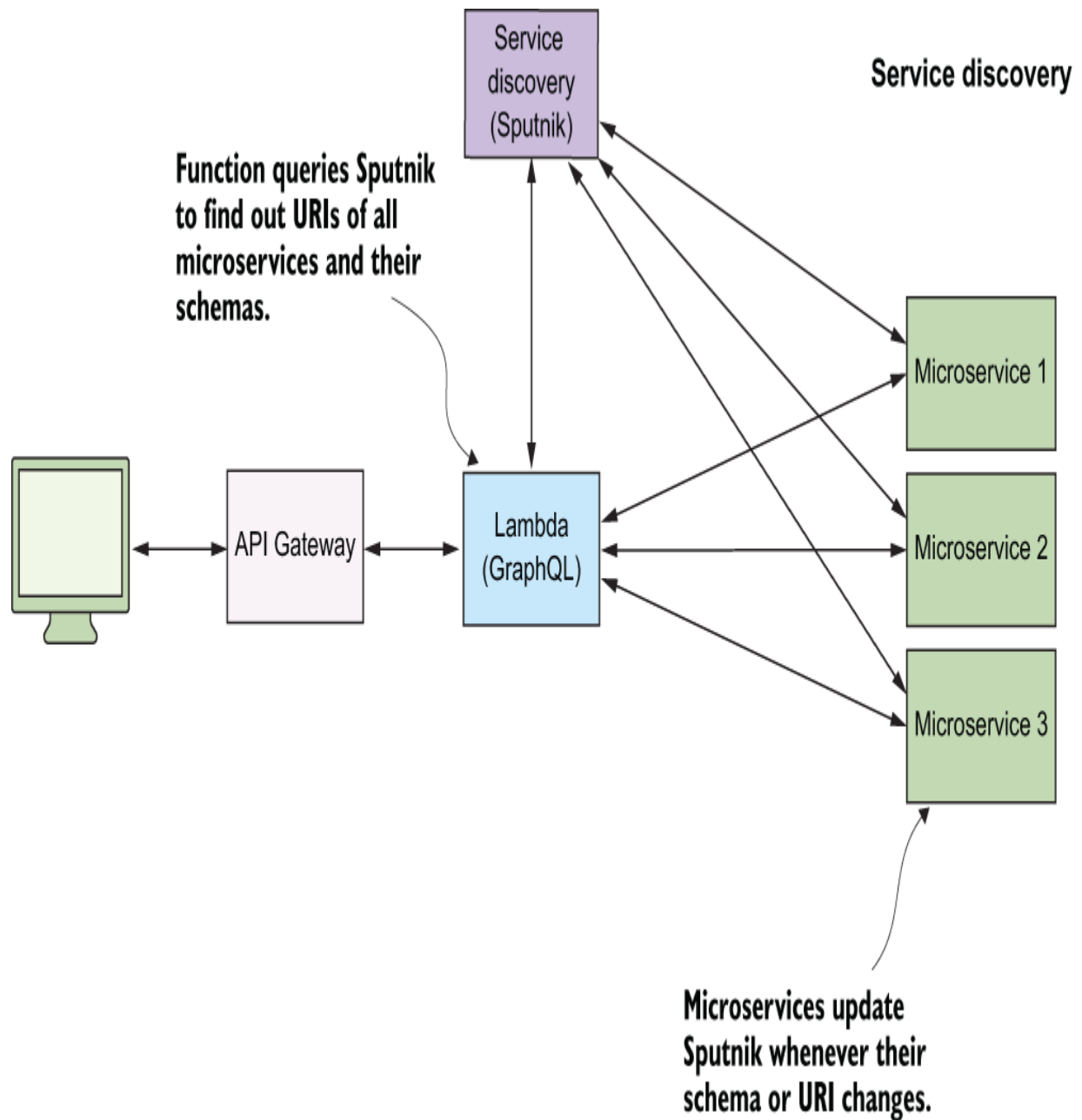
Figure 5.9 The service discovery (Sputnik) mechanism for A Cloud Guru. There's an AWS service called Cloud Map that you may want to check out if you are looking for something similar.
