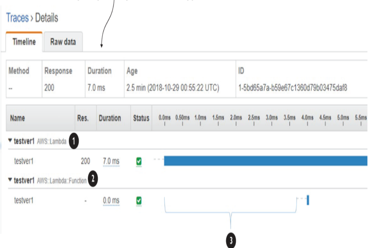
Figure 10.8 X-Ray trace for a sample application
