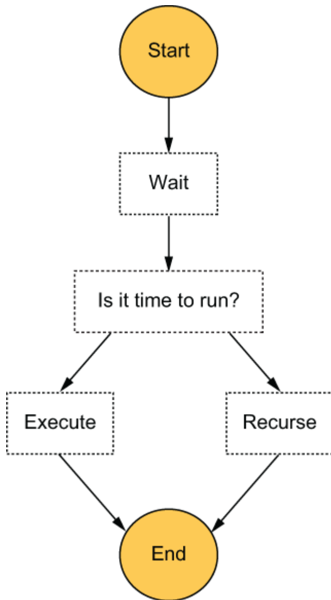
Figure 7.14 A revised state machine design that can support scheduled tasks that are more than one year away
