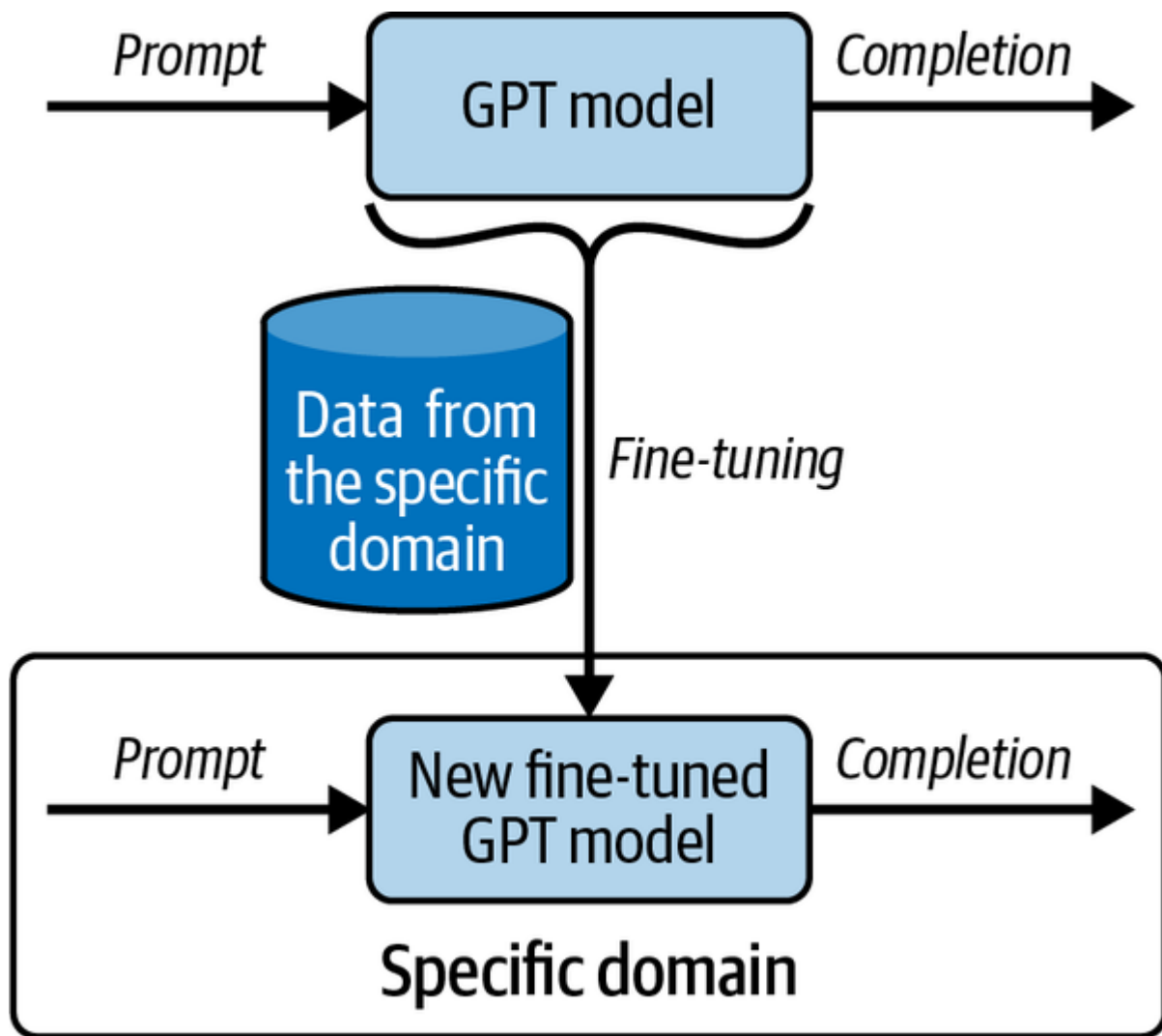
Figure 4-3. The fine-tuning process
