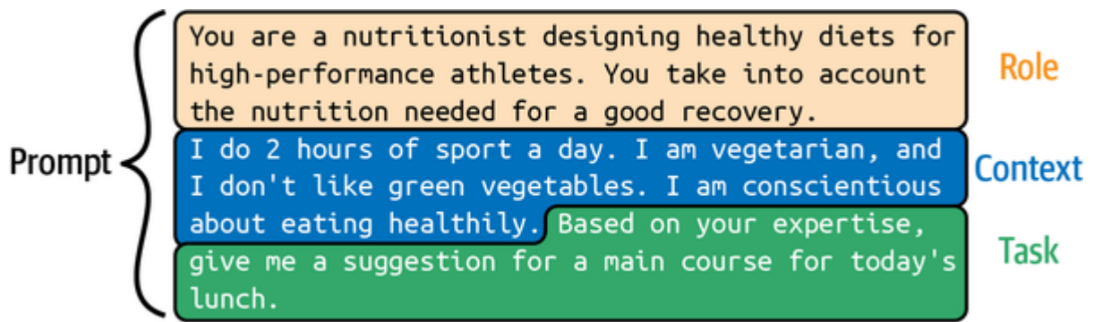
Figure 4-1. An effective prompt
