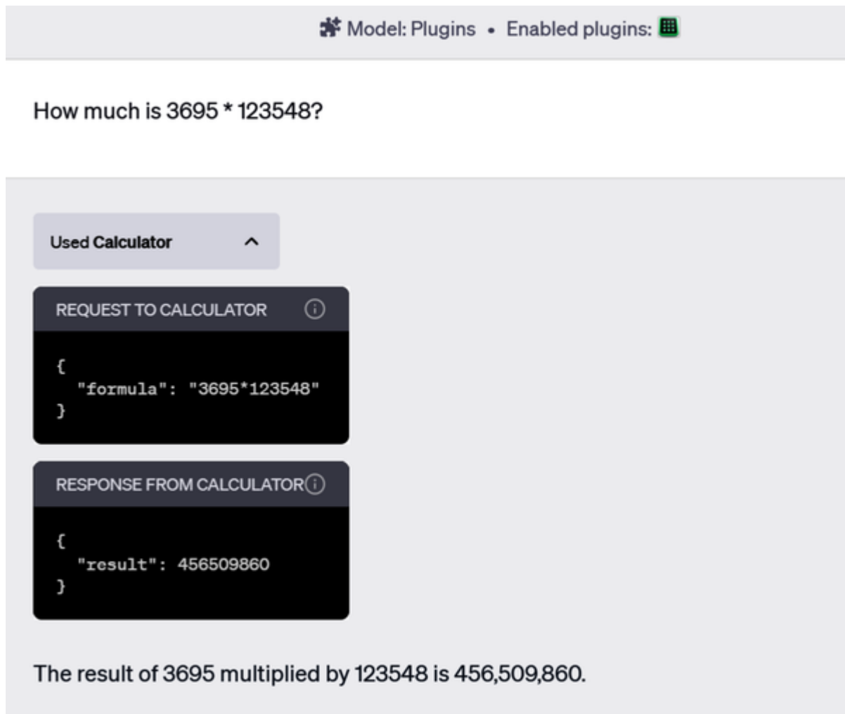
Figure 5-6. GPT-4's use of the Calculator plug-in
