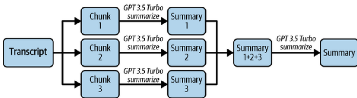
Figure 3-4. Steps to override the maximum token limit
