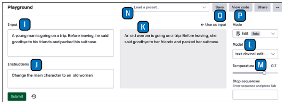
Figure 2-4. The OpenAI Playground interface in Edit mode
