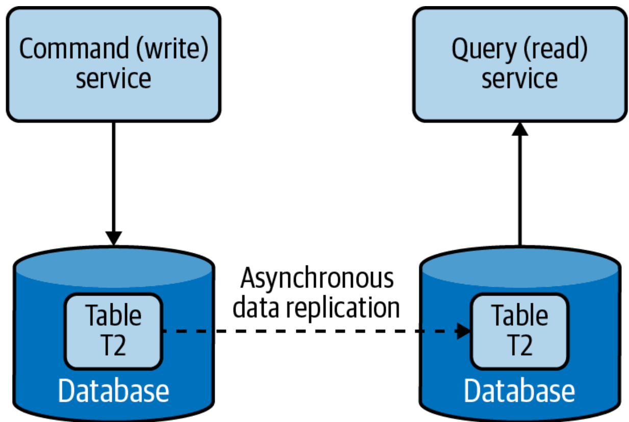
Figure 4-16. Separating command and query operations
