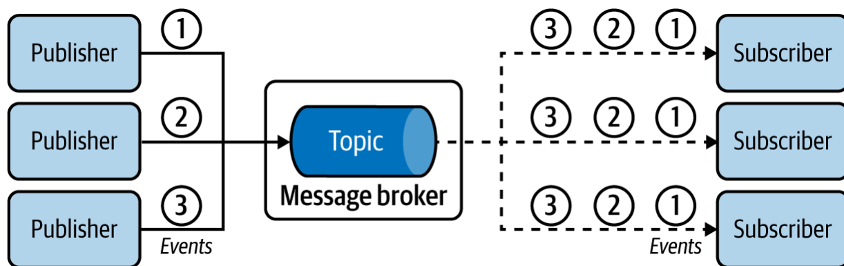
Figure 5-3. Event delivery from publishers to multiple subscribers
