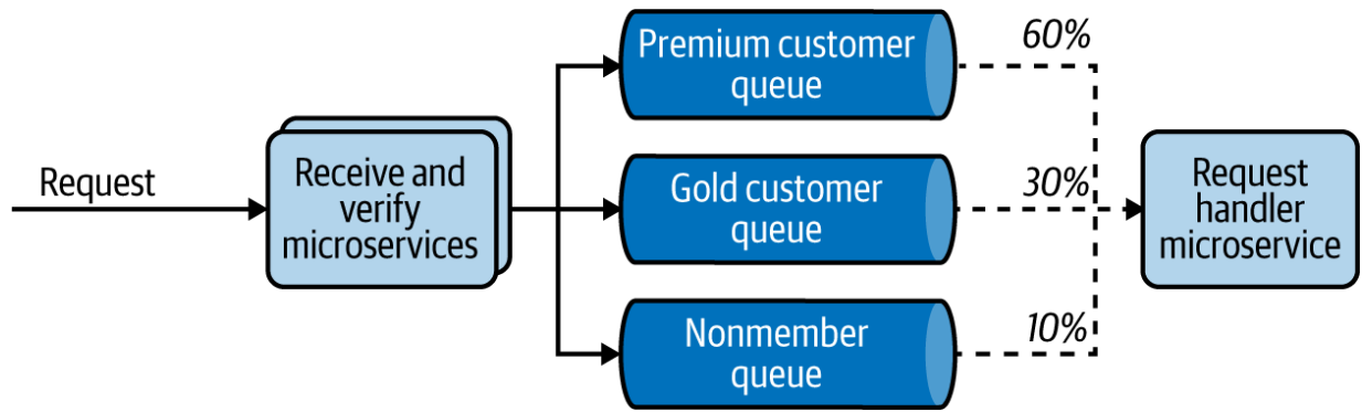
Figure 5-13. Priority-based customer-request handling
