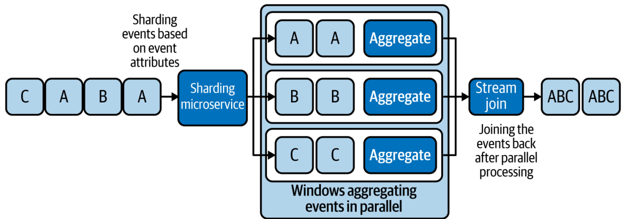
Figure 6-4. Sharding events based on event attributes, processing them in parallel, and joining the results
