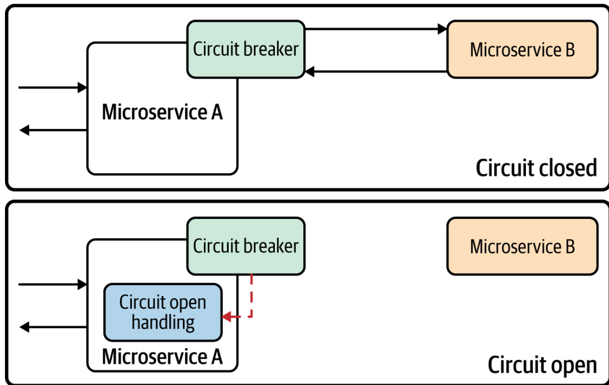
Figure 3-12. Circuit breaker
