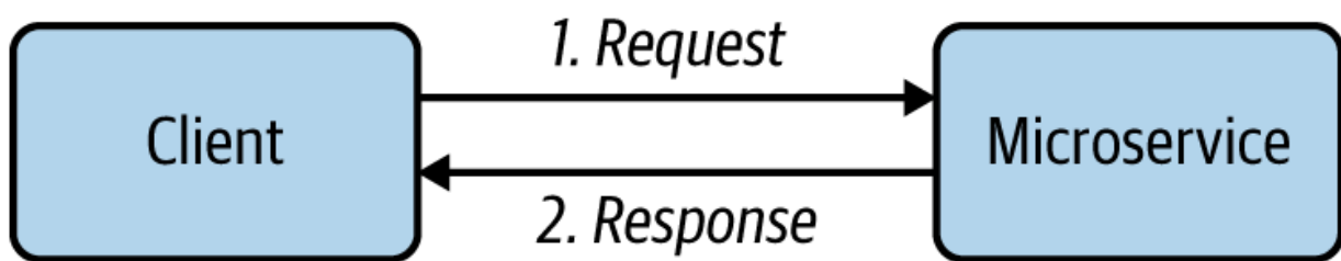
Figure 2-1. Request-Response pattern
