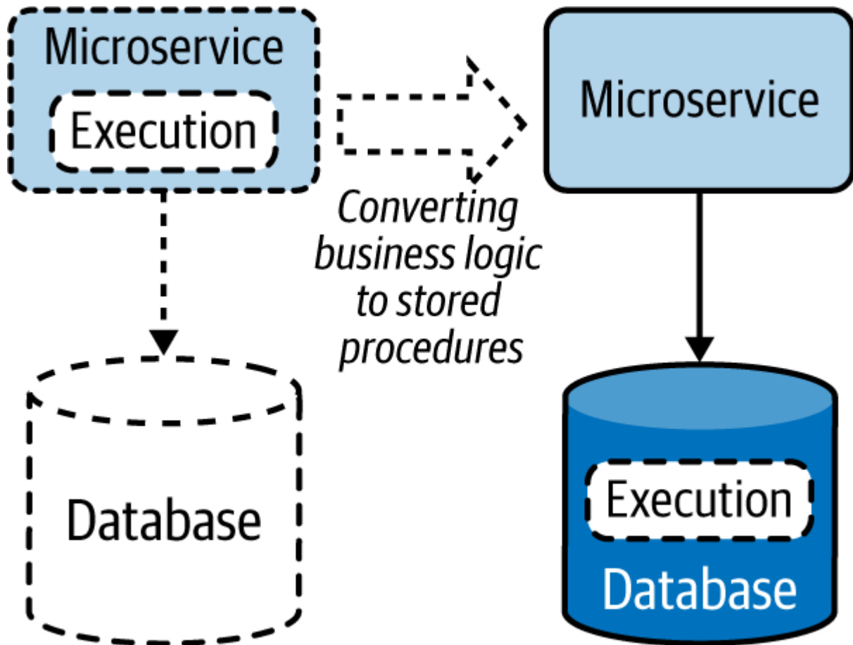
Figure 4-19. Moving execution to data stores as stored procedures
