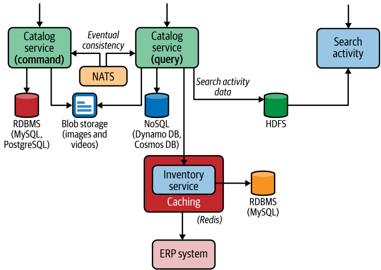
Figure 8-4. Decentralized data management with private databases, CQRS, caching, and heterogeneous databases
