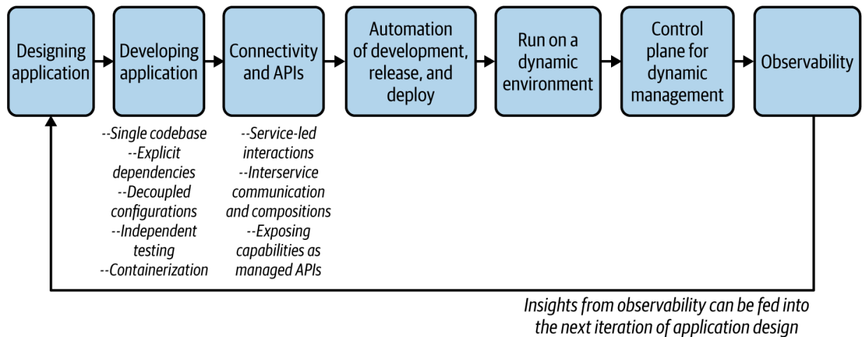
Figure 1-6. Methodology for building cloud native applications
