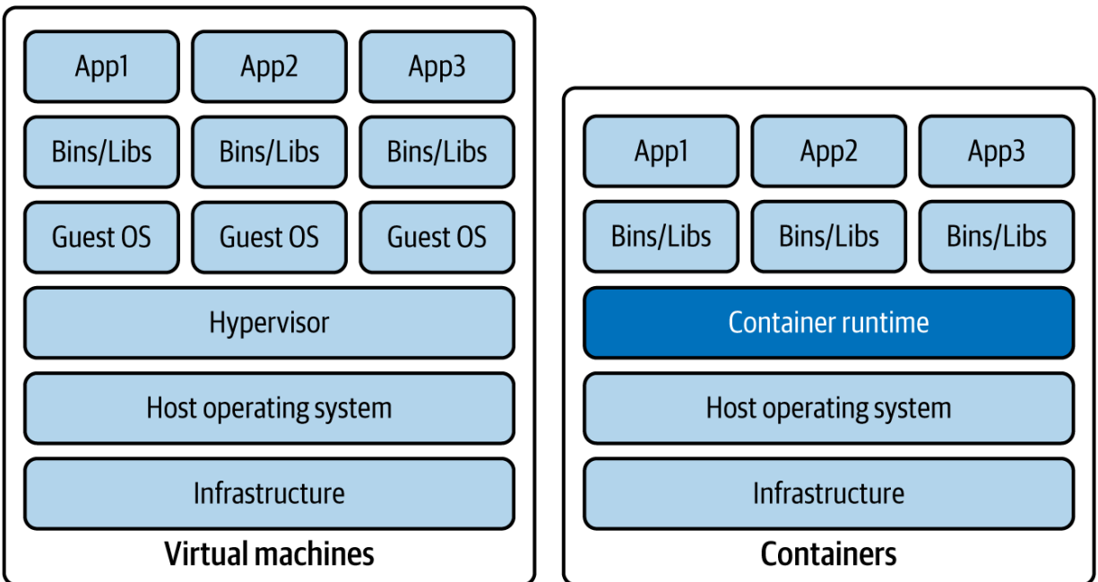
Figure 1-3. Comparing application execution on virtual machines versus containers
