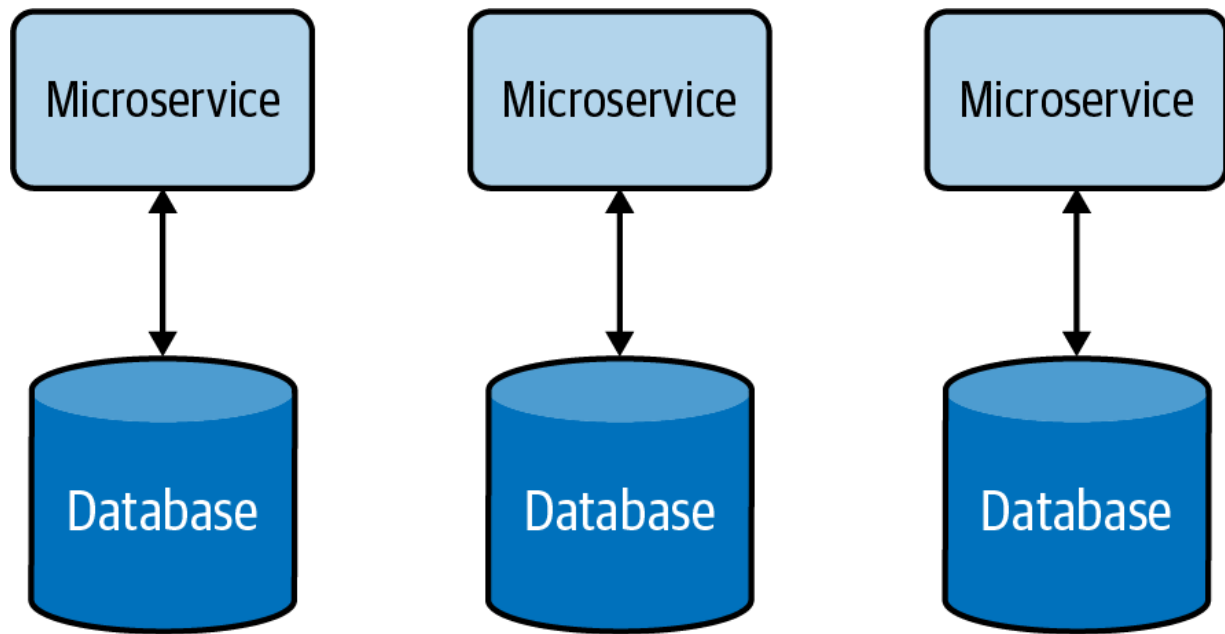
Figure 4-4. Decentralized data management
