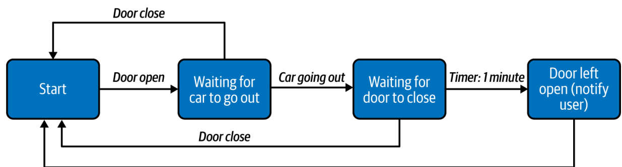
Figure 6-9. Detecting the garage door left open for more than 1 minute after the car leaves the garage
