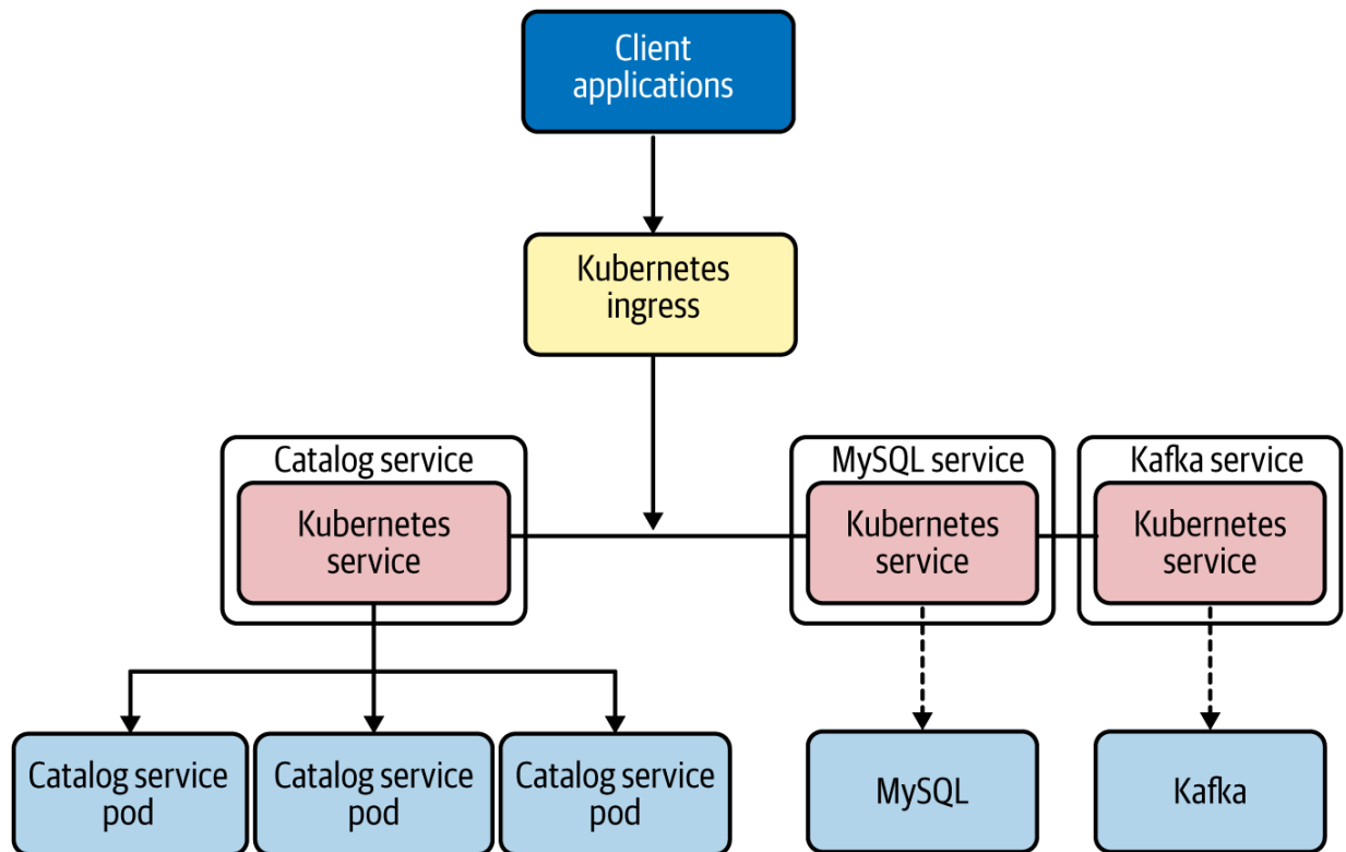
Figure 3-4. Kubernetes groups a set of pods, or any external system, to a single abstraction known as a service
