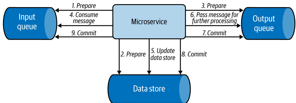
Figure 4-24. Simple message processing use case applying an XA transaction
