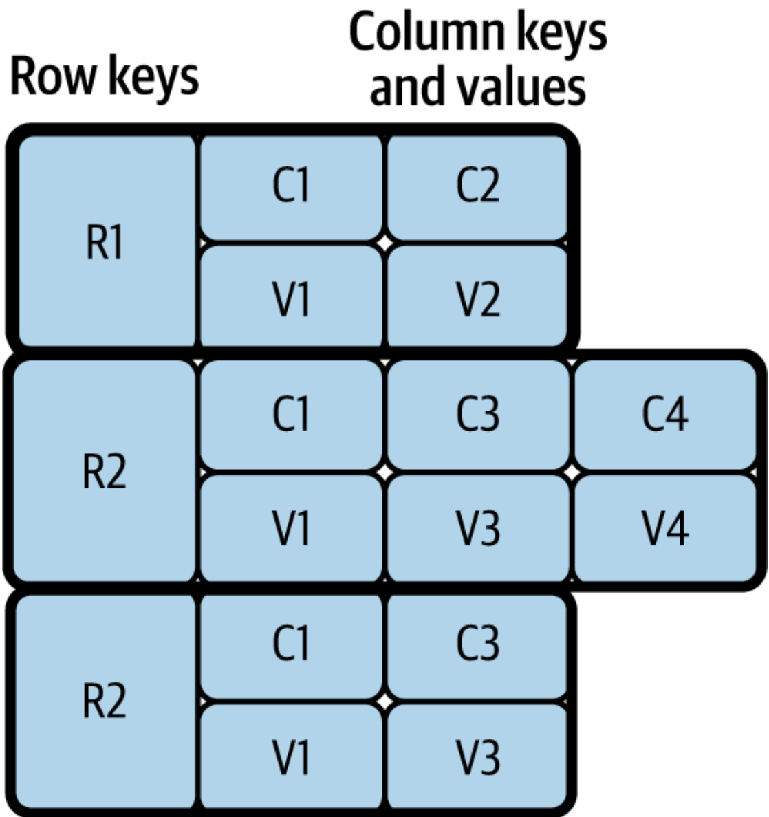
Figure 4-2. Column store
