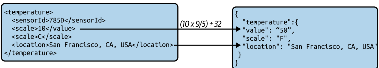
Figure 6-1. XML-to-JSON transformation
