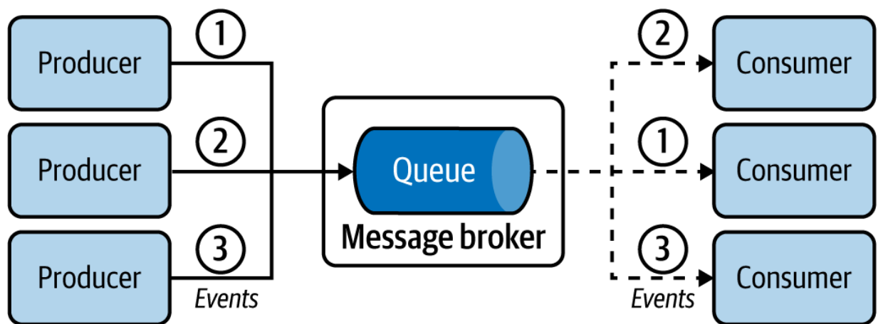
Figure 5-1. Event delivery from producers to consumers
