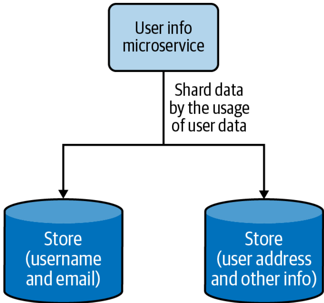
Figure 4-14. Vertical data sharding based on frequency of data access
