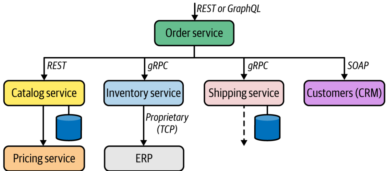
Figure 3-23. Service Orchestration in a real-world service composition use case
