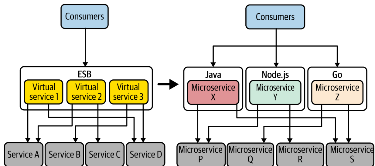
Figure 3-17. Interservice communication: from ESB (left) to microservices (right)
