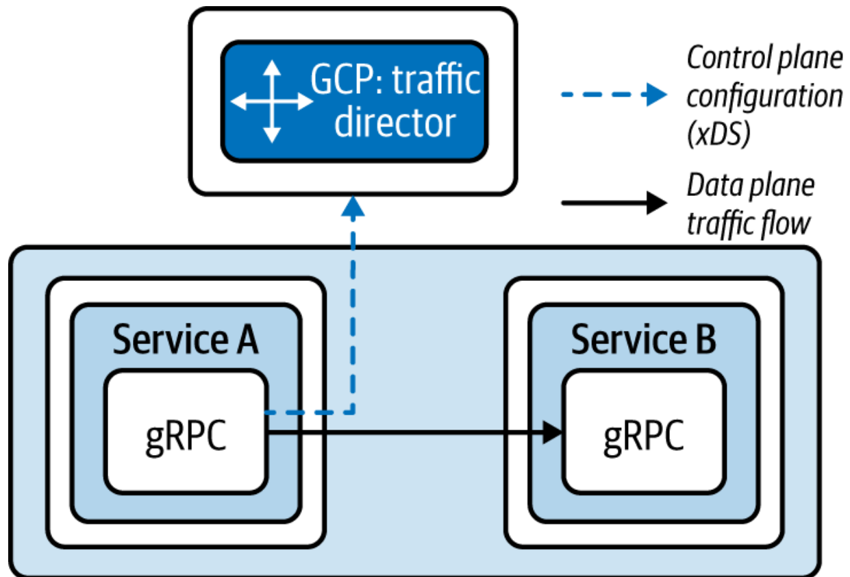
Figure 3-21. Sidecarless Service Mesh
