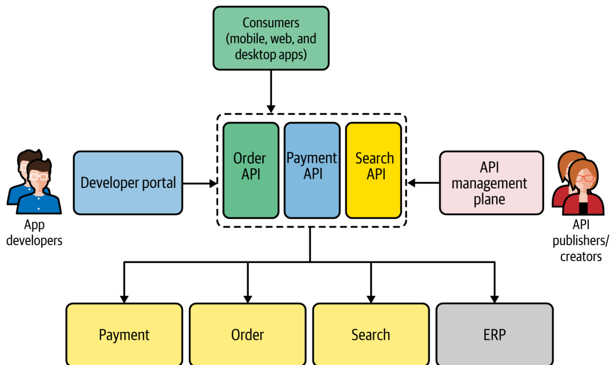
Figure 7-4. API microgateways in action
