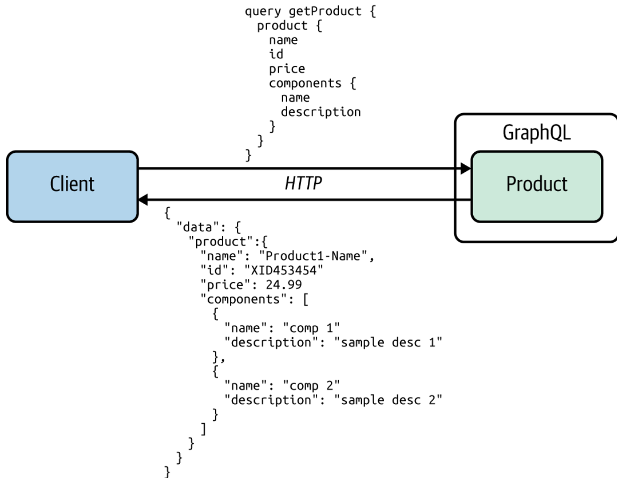
Figure 2-10. An example GraphQL service and its interactions
