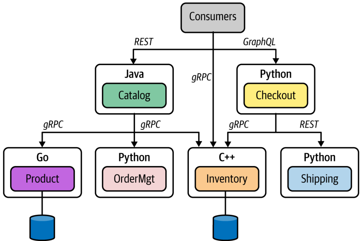
Figure 2-3. Using gRPC for microservice communication
