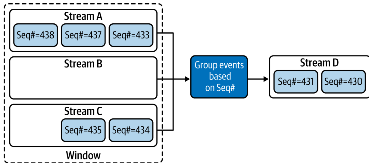
Figure 6-14. Grouping events based on event sequence number
