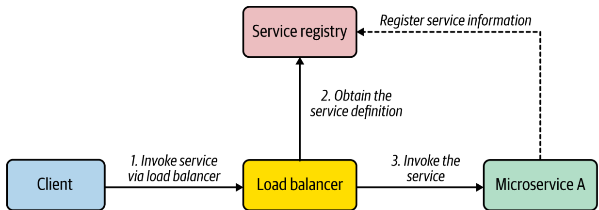
Figure 3-6. Service Registry and Discovery—server-side discovery
