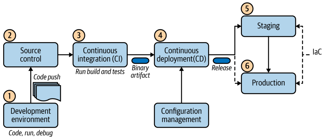
Figure 1-5. Cloud native application development life cycle
