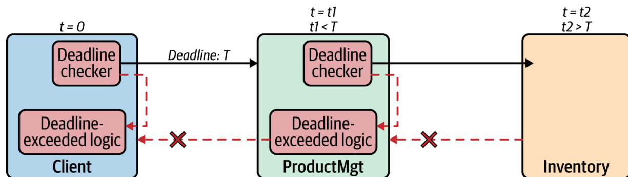
Figure 3-11. Deadlines
