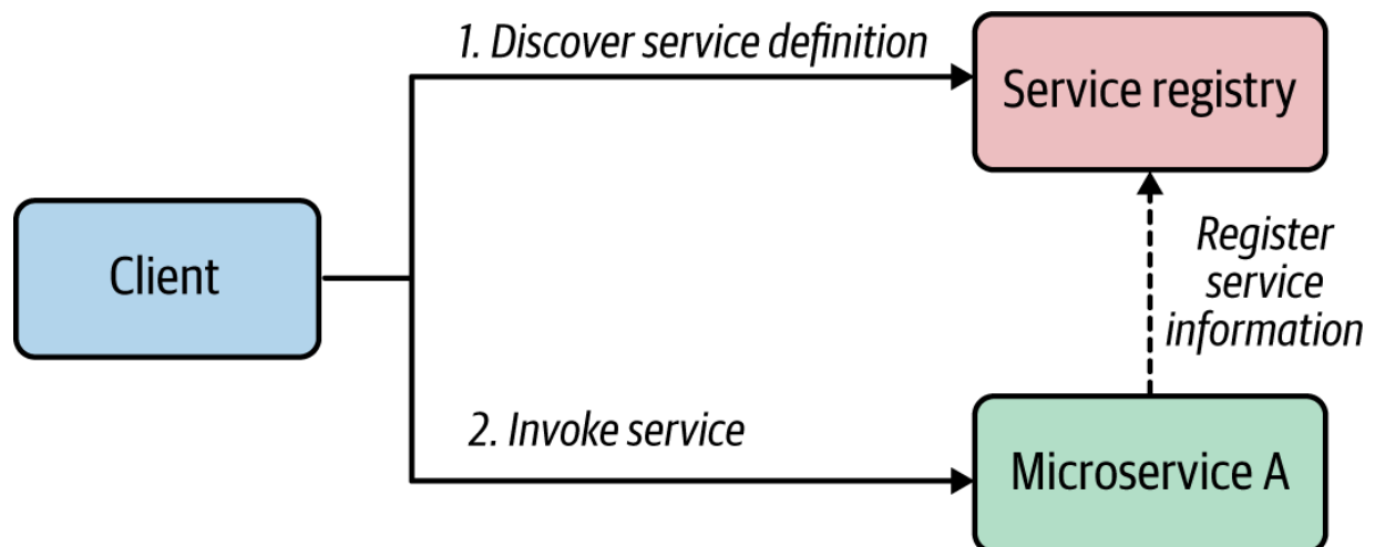
Figure 3-5. Service Registry and Discovery—client-side discovery
