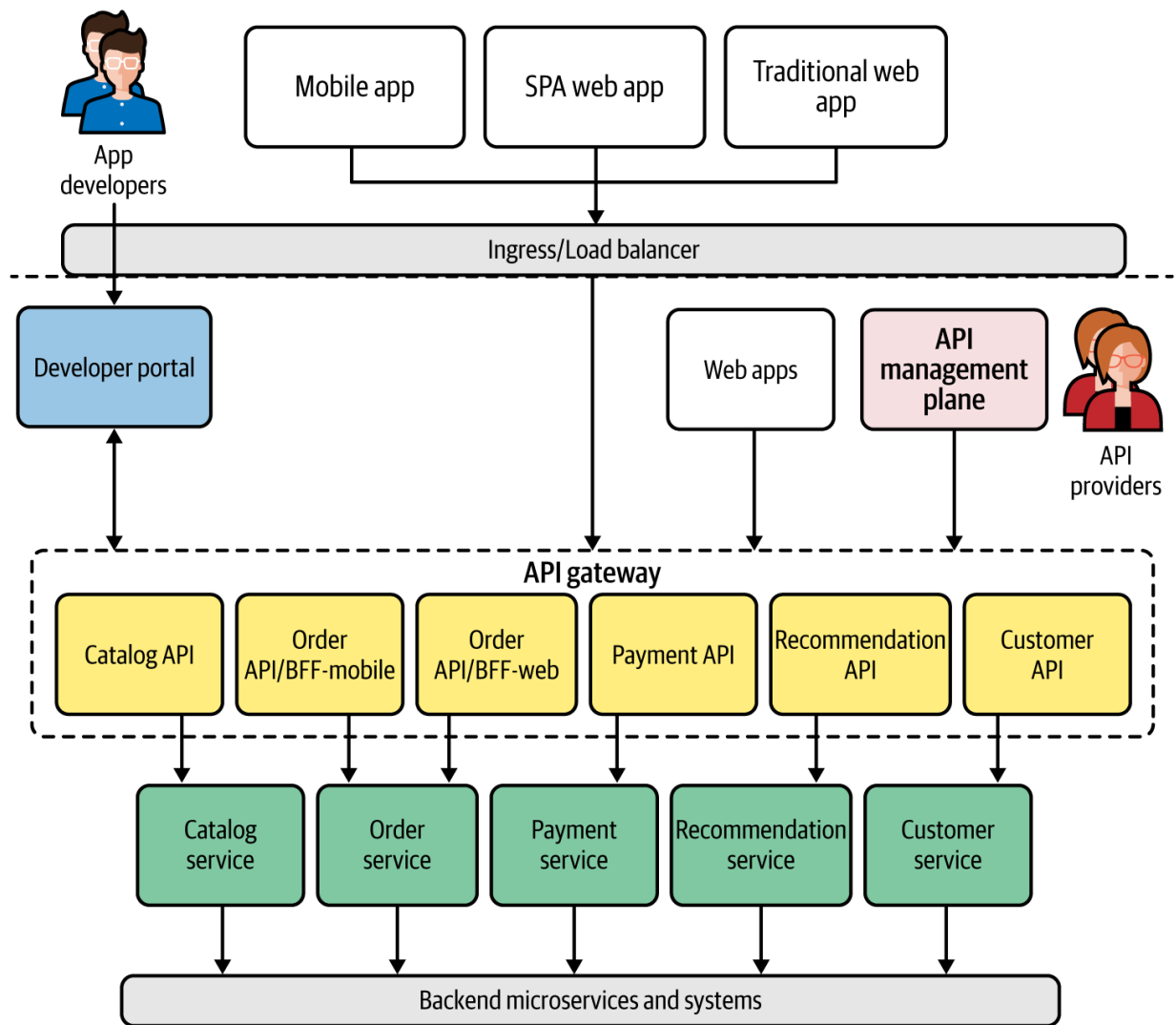
Figure 8-2. Designing APIs and frontend applications
