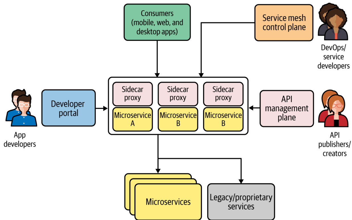
Figure 7-5. API management through service mesh sidecars
