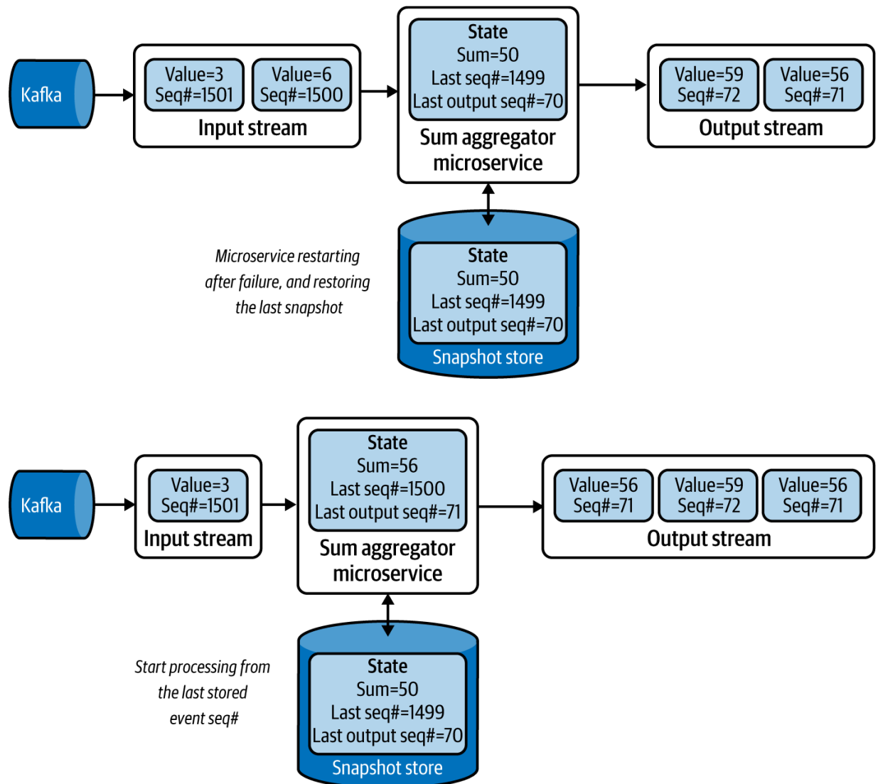
Figure 6-25. Microservice emitting the output sequence number for the dependent system to detect duplicate events
