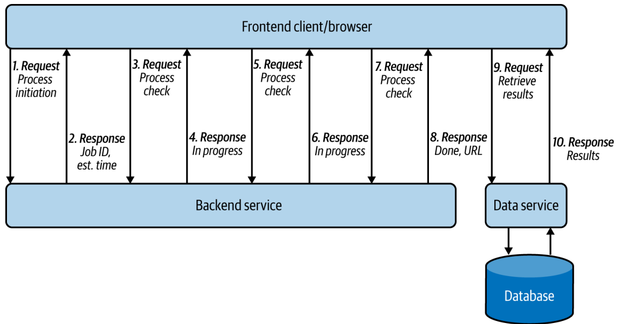
Figure 5-7. Frontend client/browser repeatedly calling backend service to retrieve asynchronous job results
