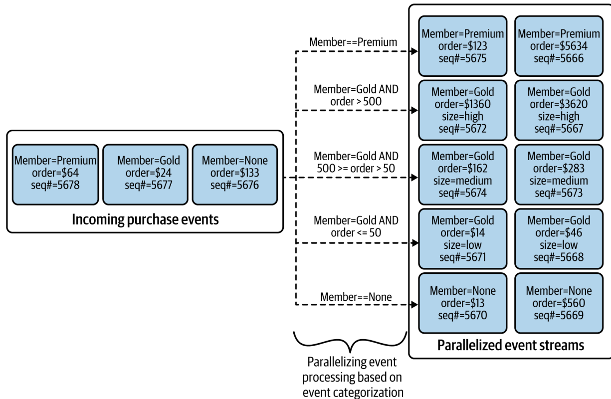
Figure 6-13. Partitioning and processing order events in parallel
