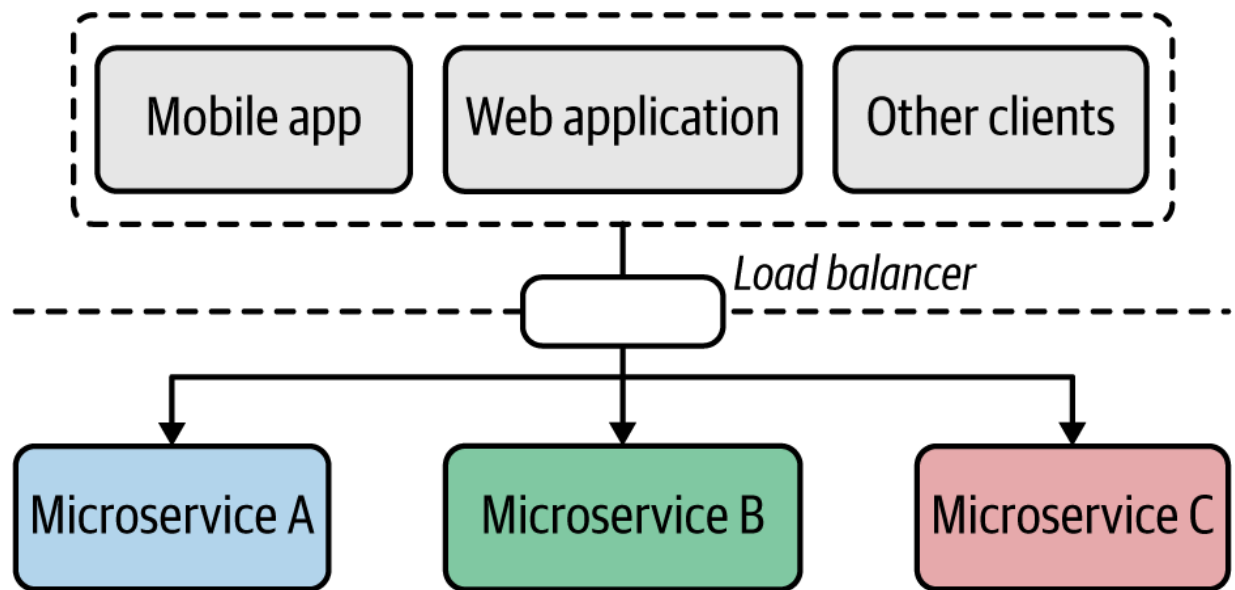
Figure 7-6. Directly exposing microservices to frontends
