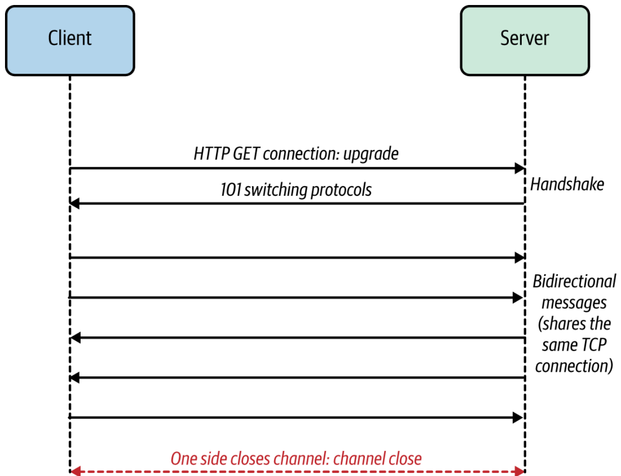
Figure 2-11. An example of WebSocket communication
