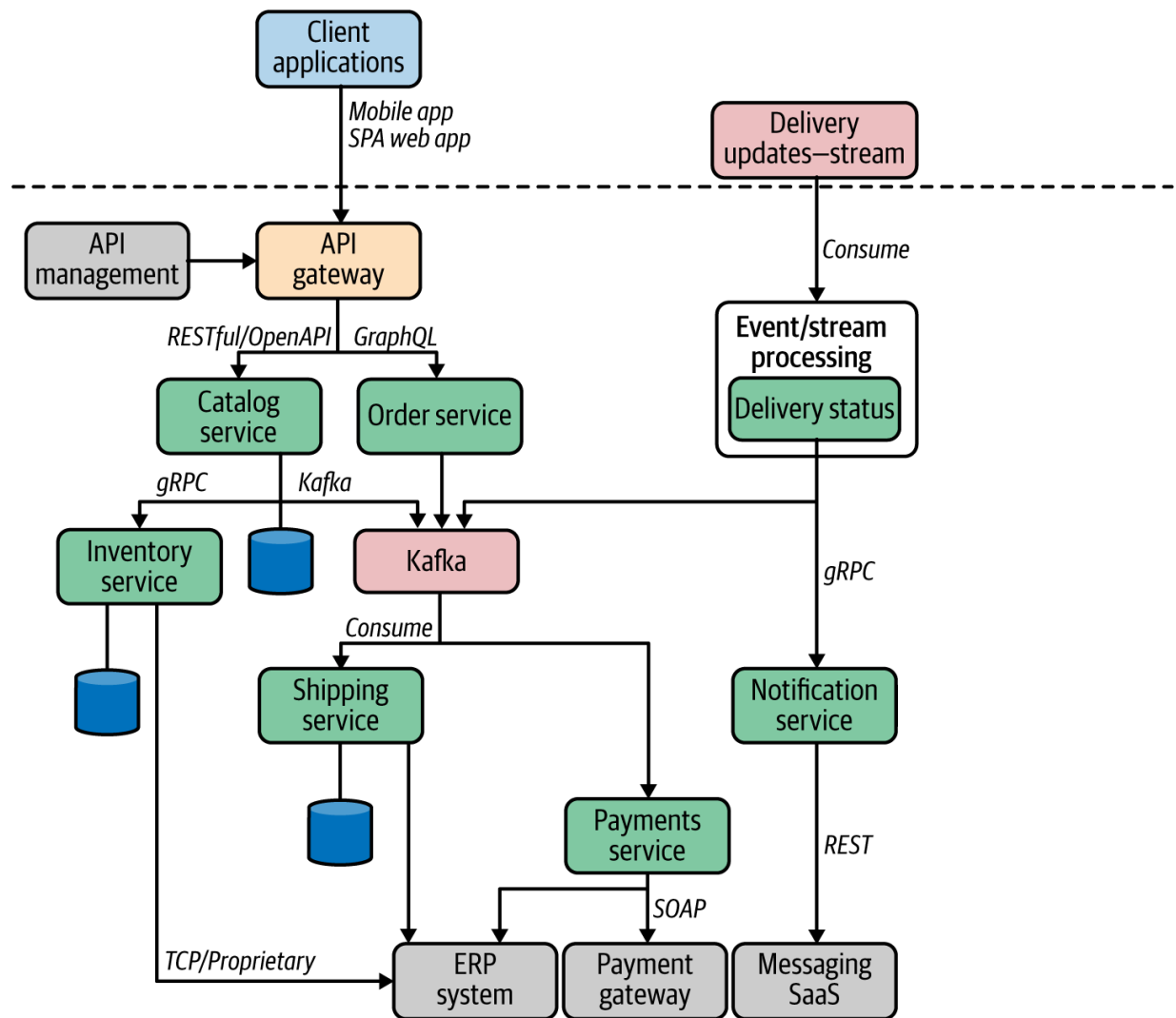
Figure 3-2. Using the Service Connectivity pattern in an online retail application
