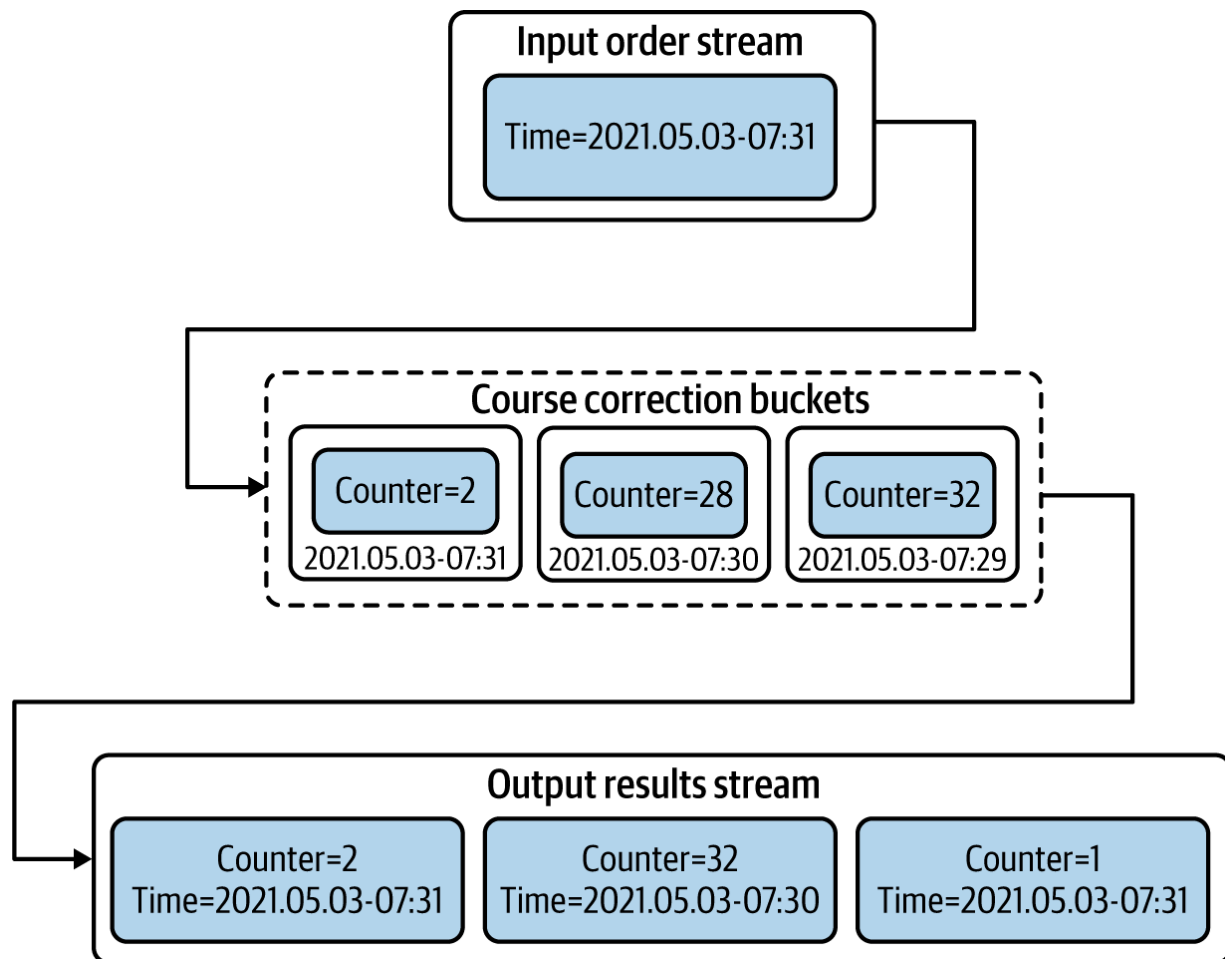
Figure 6-18. Aggregate events over multiple buckets to course-correct previous results
