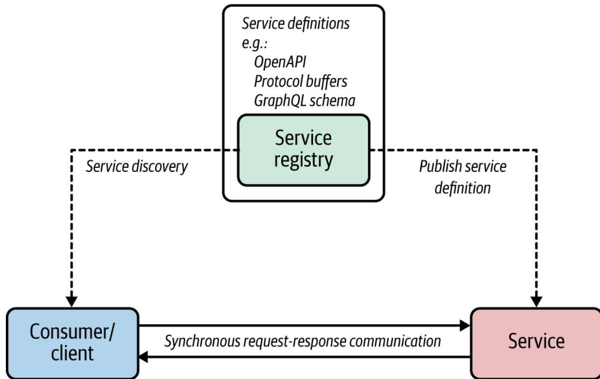
Figure 2-7. Using a service registry for storing service definitions and discovering them
