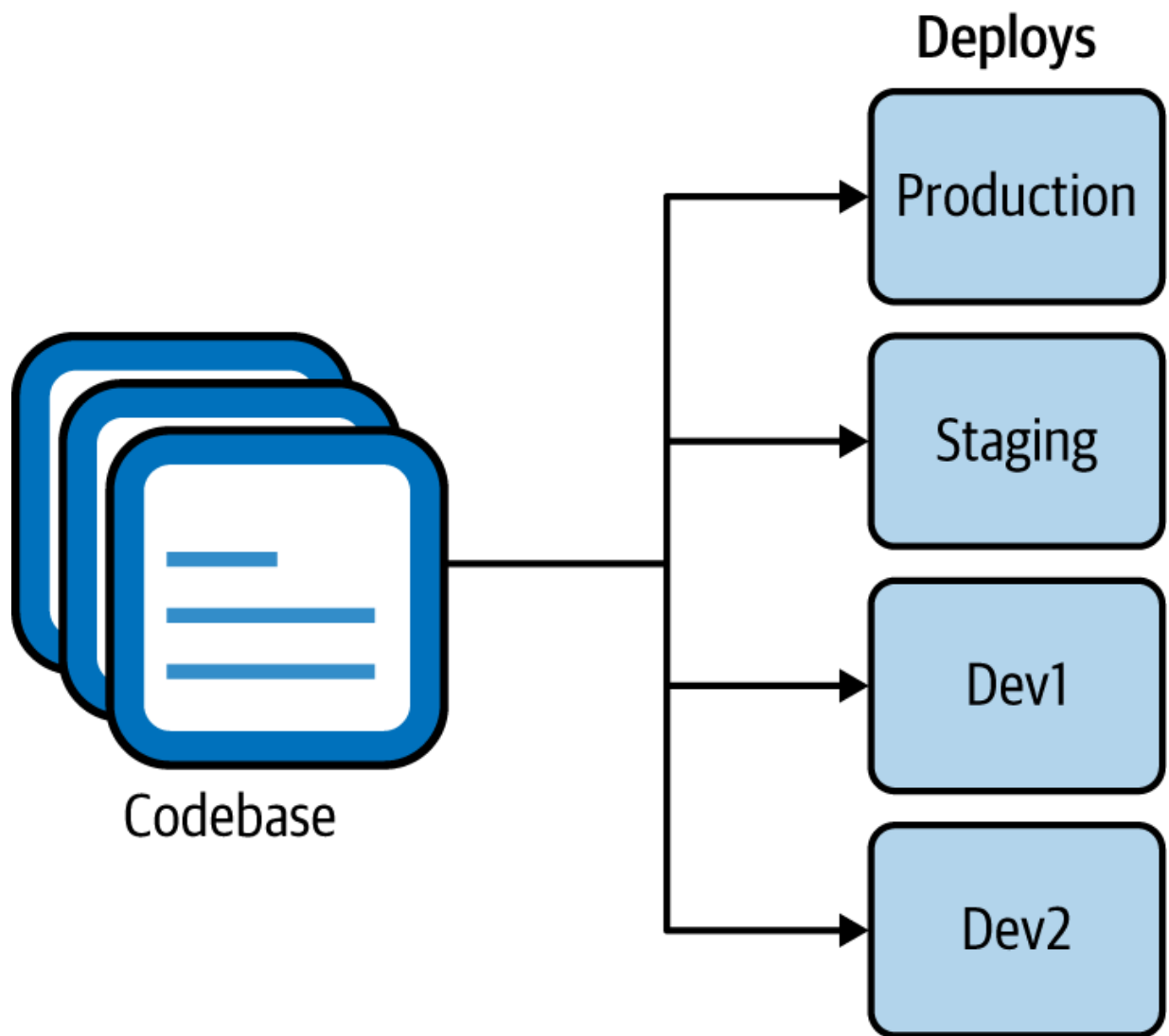
Figure 1-7. A single codebase with multiple deployments into different environments
