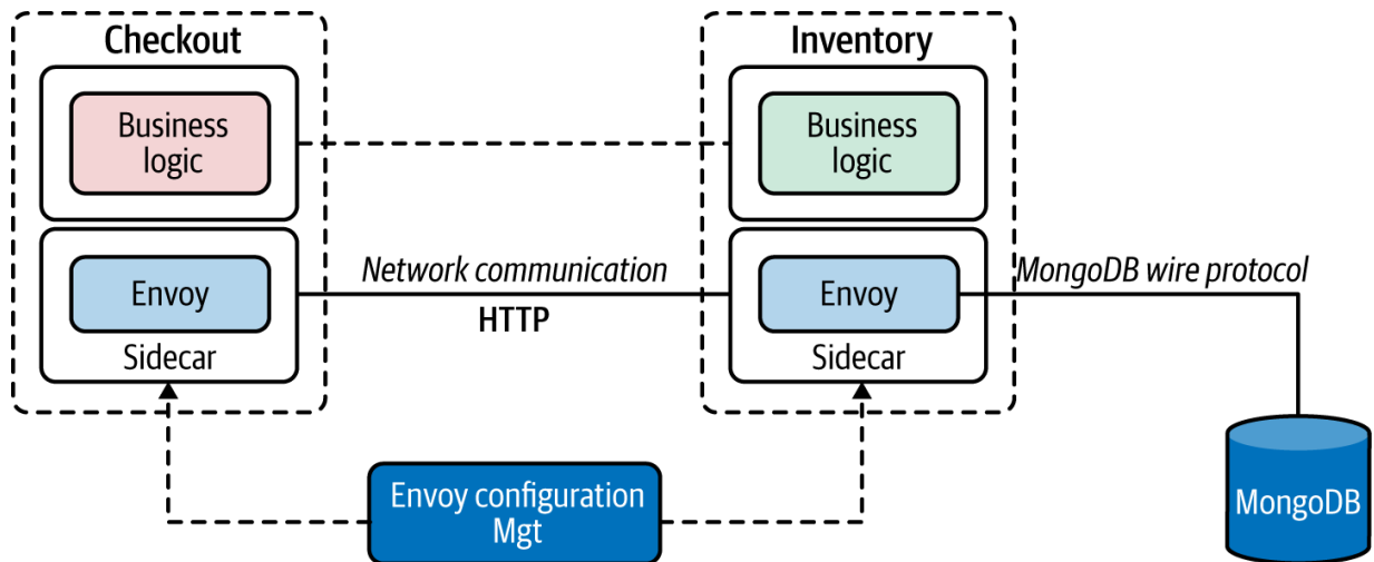
Figure 3-15. Using Envoy as a sidecar
