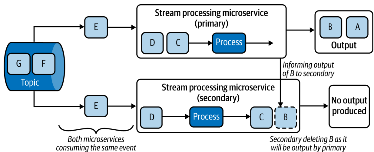
Figure 6-26. Running microservices as primary and secondary to enable failover
