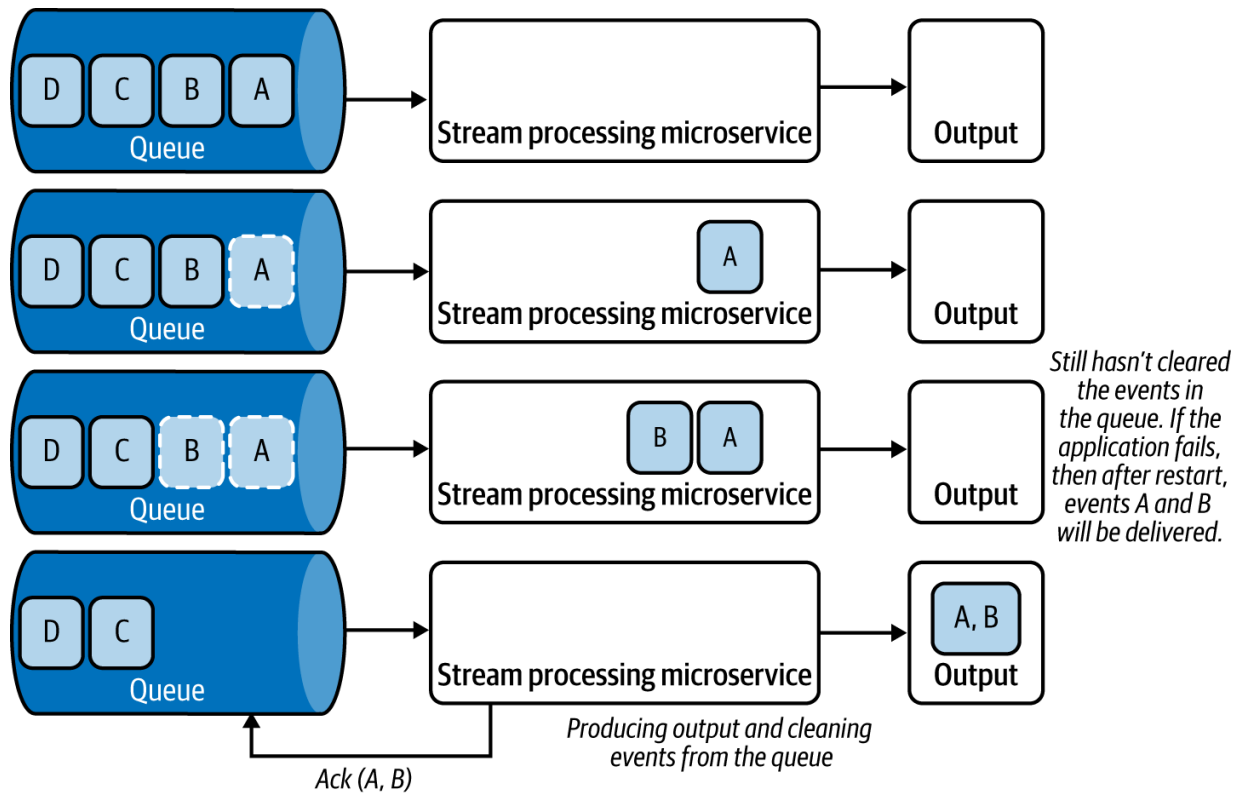
Figure 6-22. Deferring acknowledgment until after outputs are generated
