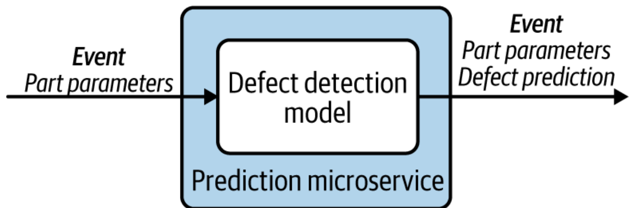
Figure 6-11. Running a prebuilt machine learning model to detect defects
