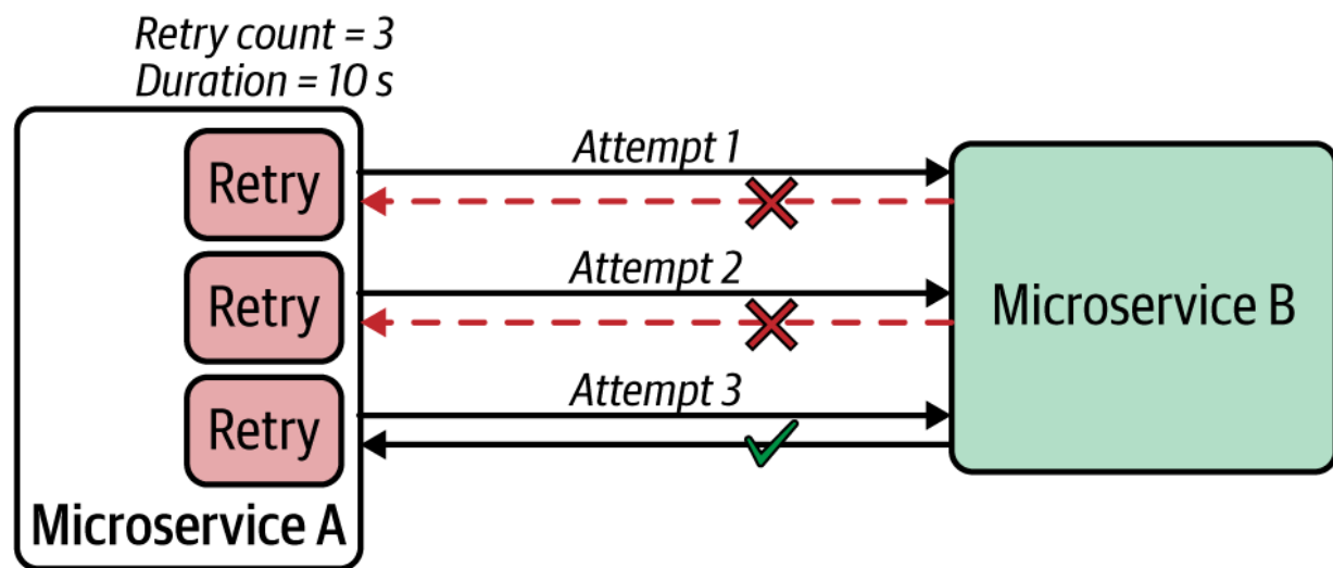
Figure 3-10. Retry logic trying to invoke the same service a specified number of times at given intervals
