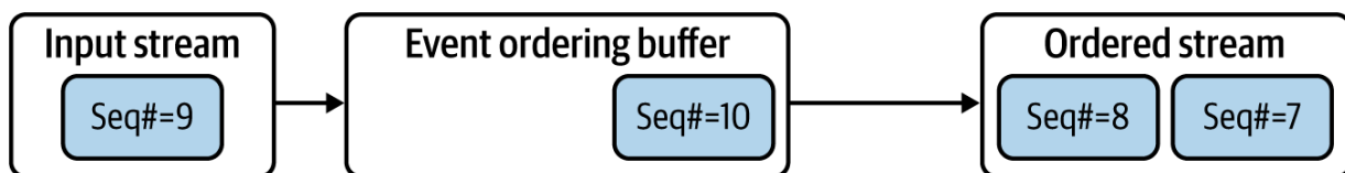
Figure 6-17. Ordering events based on sequence number
