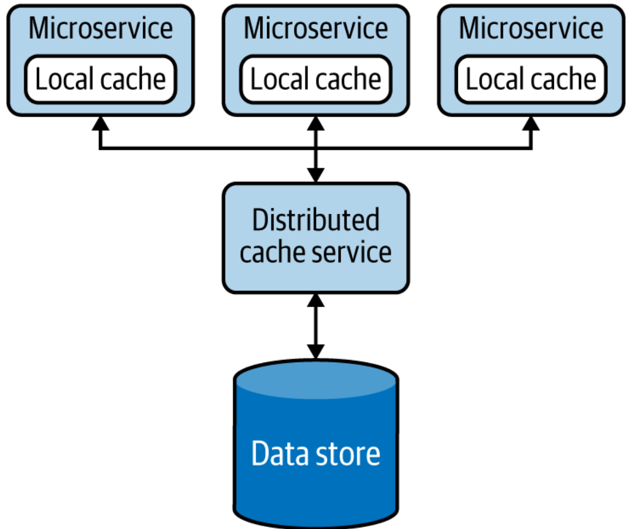
Figure 4-20. Multilayer cache fallback
