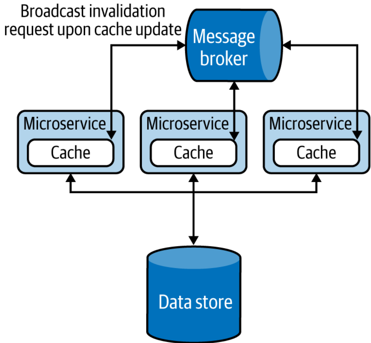
Figure 4-21. Using the message broker to invalidate cache in all services
