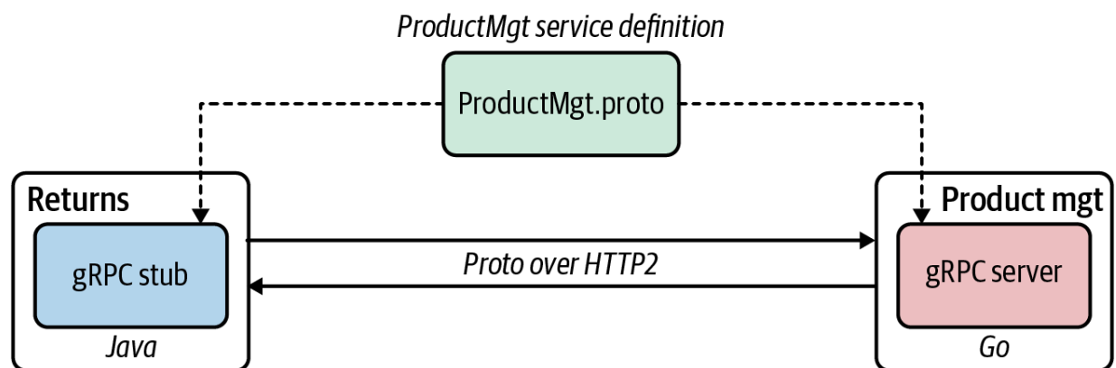
Figure 2-12. An example of microservices communication using gRPC
