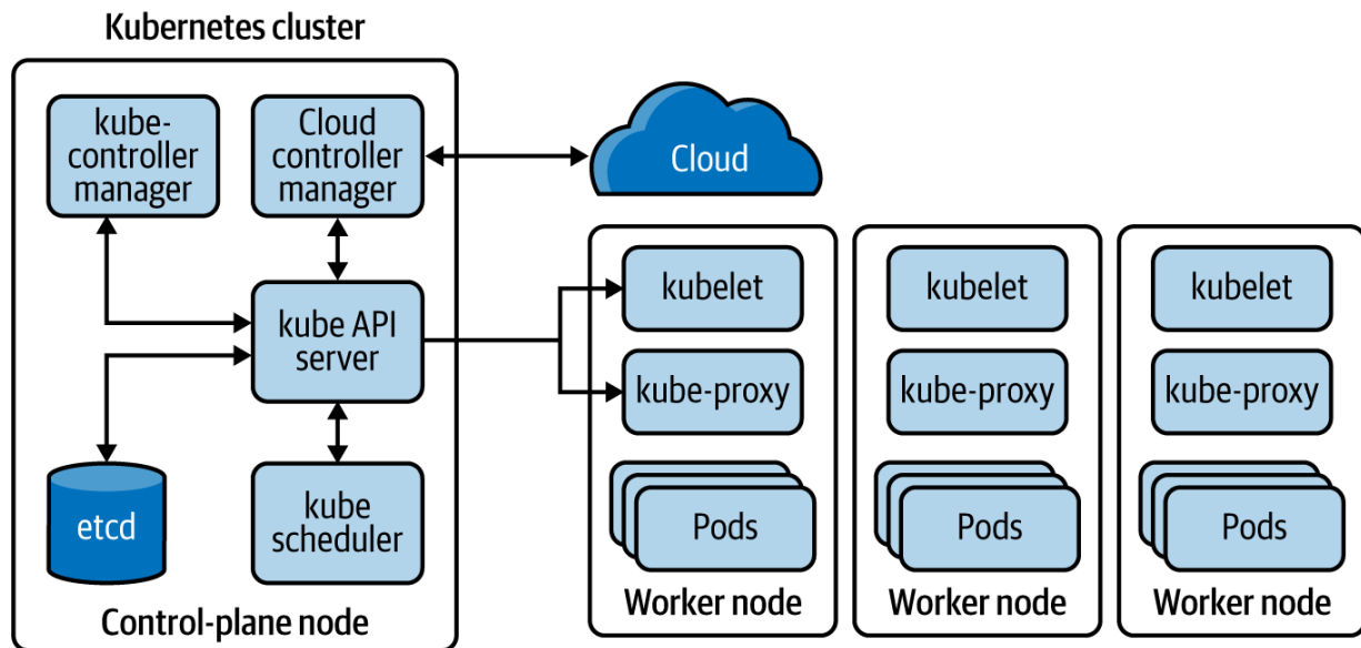
Figure 1-4. Fundamental components of a Kubernetes platform
