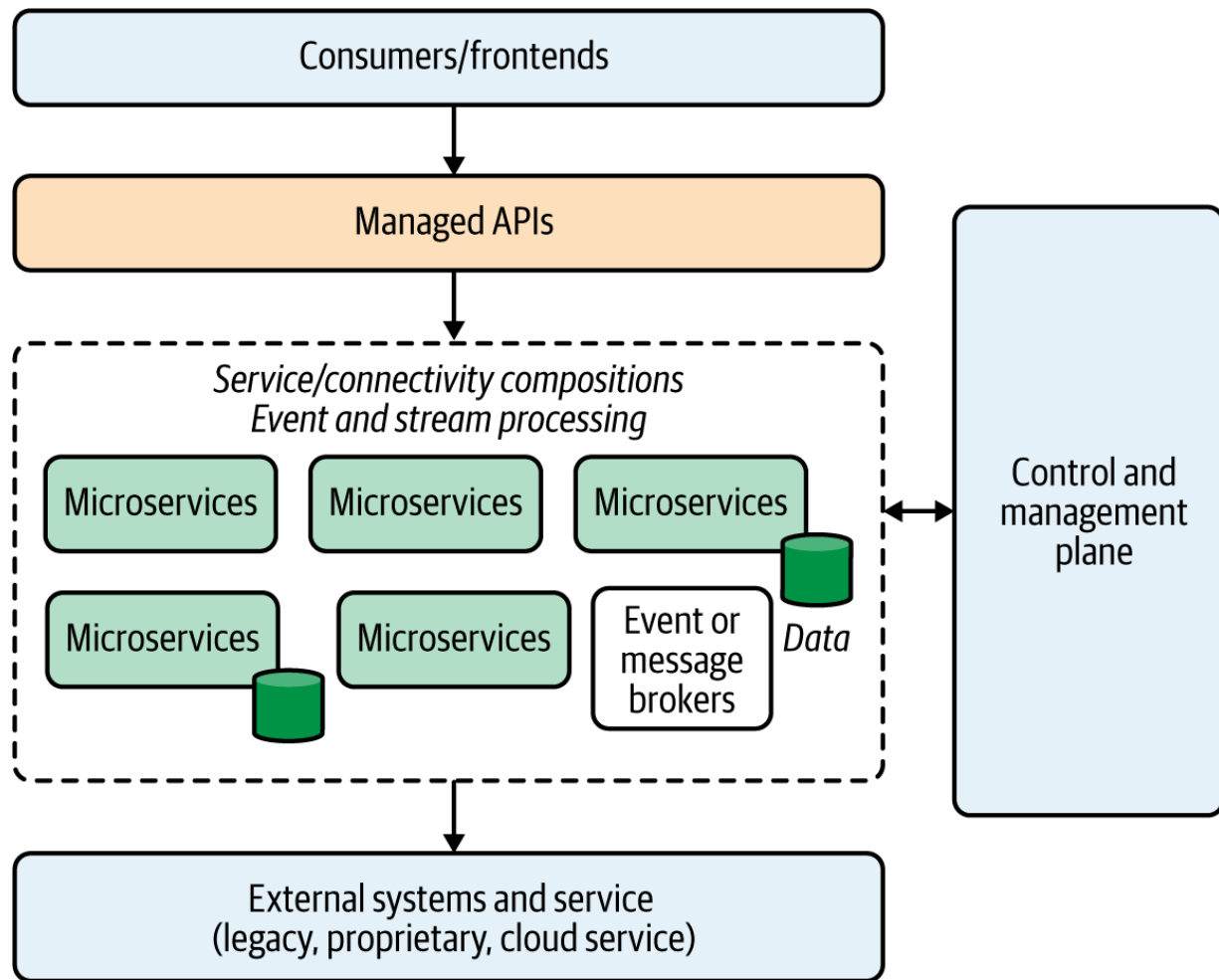
Figure 8-1. High-level architecture of the online retail cloud native application
