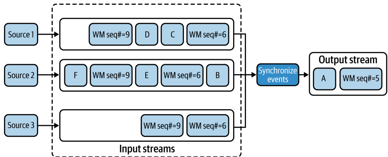
Figure 6-19. Generating watermark events and synchronizing events based on them
