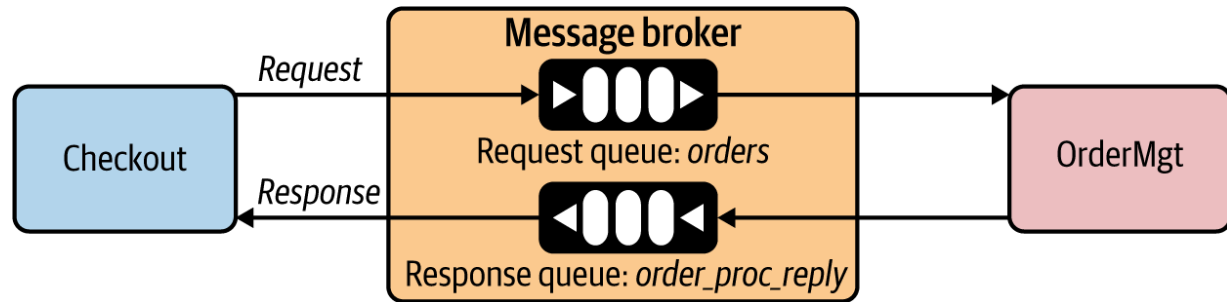
Figure 2-6. Asynchronous Request-Reply pattern implemented using a message broker
