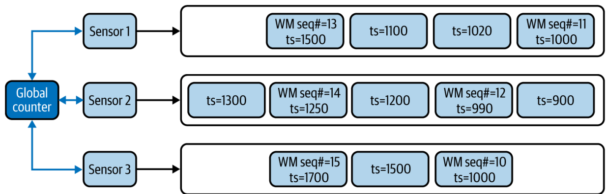
Figure 6-21. Ordering events based on continuous watermark events
