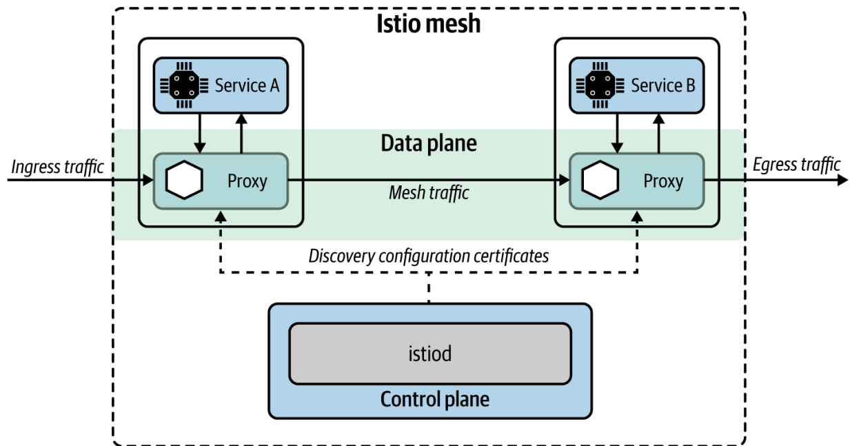
Figure 3-19. Component architecture of Istio service mesh
