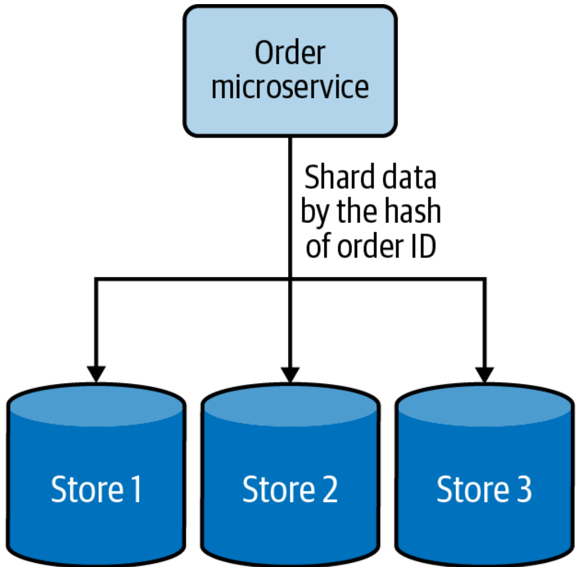
Figure 4-13. Horizontal data sharding using hashing
