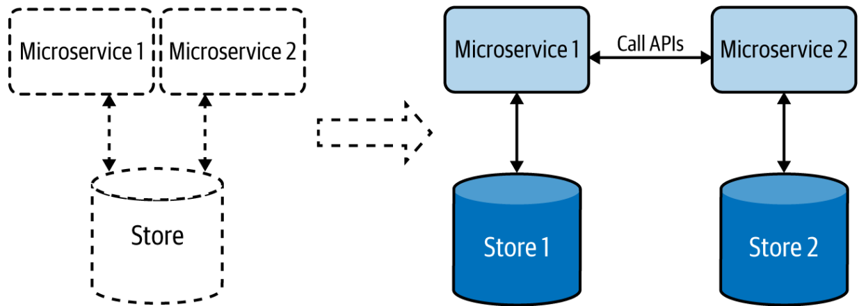
Figure 4-6. Cloud native applications, depicted at right, have a dedicated data store for each microservice.
