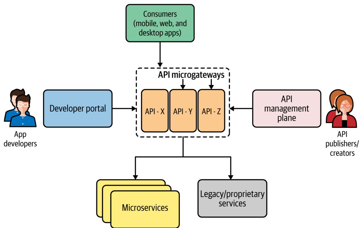
Figure 7-3. API management with microgateways
