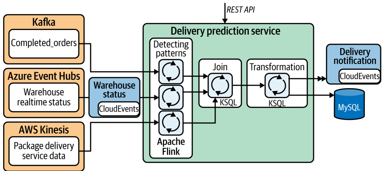
Figure 8-6. Processing multiple streams of data and predicting the delivery time
