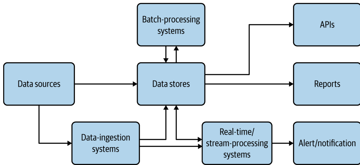
Figure 4-1. Data architecture for cloud native applications
