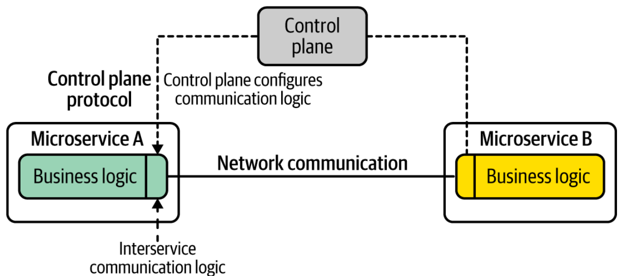
Figure 3-20. Sidecarless service mesh
