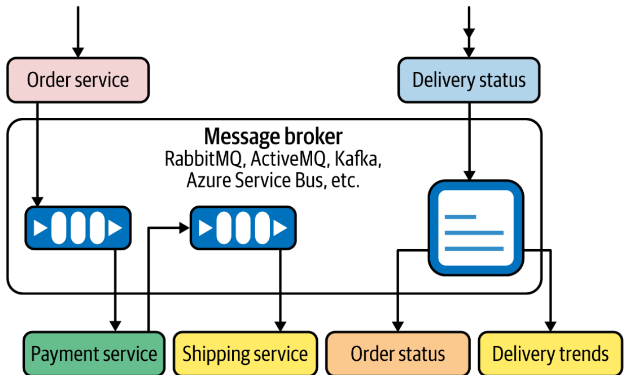
Figure 3-25. Service Choreography in action with queue- and topic-based asynchronous messaging
