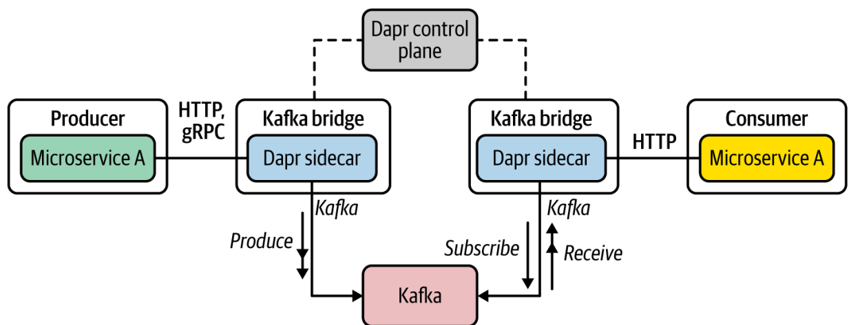
Figure 3-16. Using a Dapr sidecar as an HTTP-Kafka bridge
