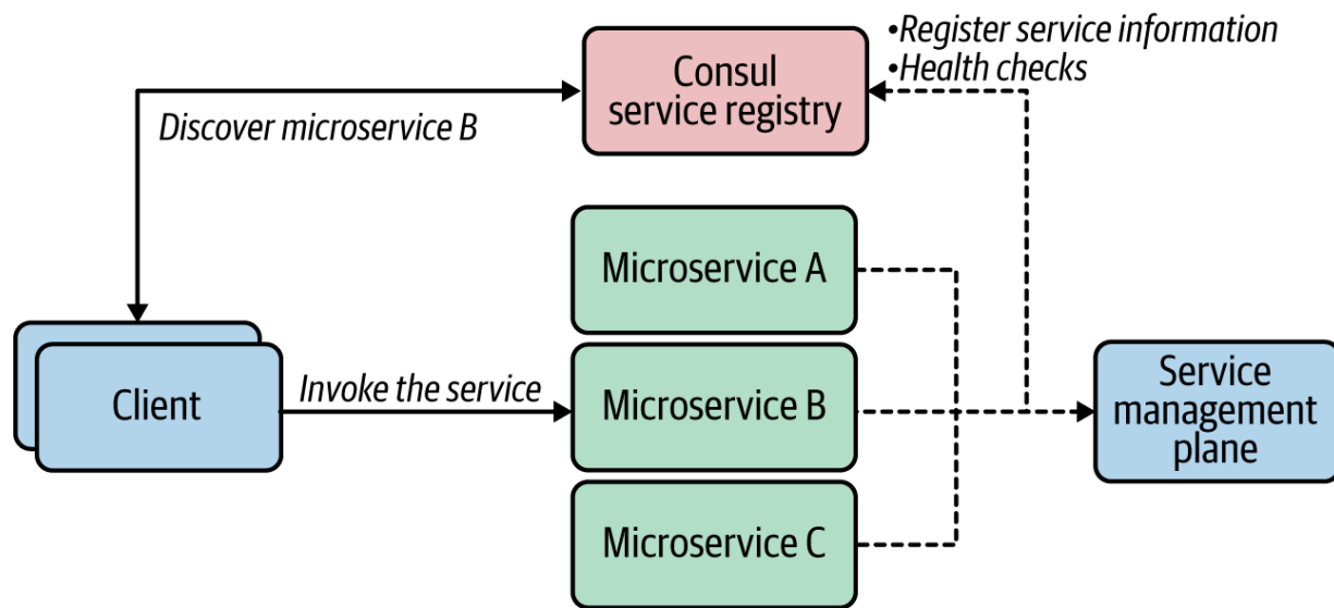
Figure 3-7. Service Registry and Discovery with Consul
