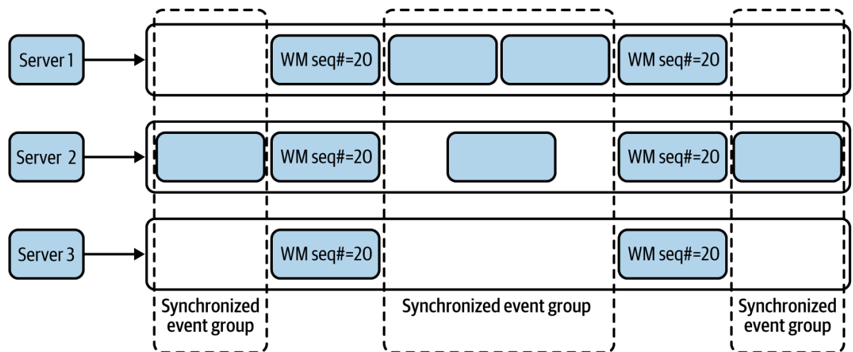
Figure 6-20. Aggregating events based on synchronized event groups generated between watermark events
