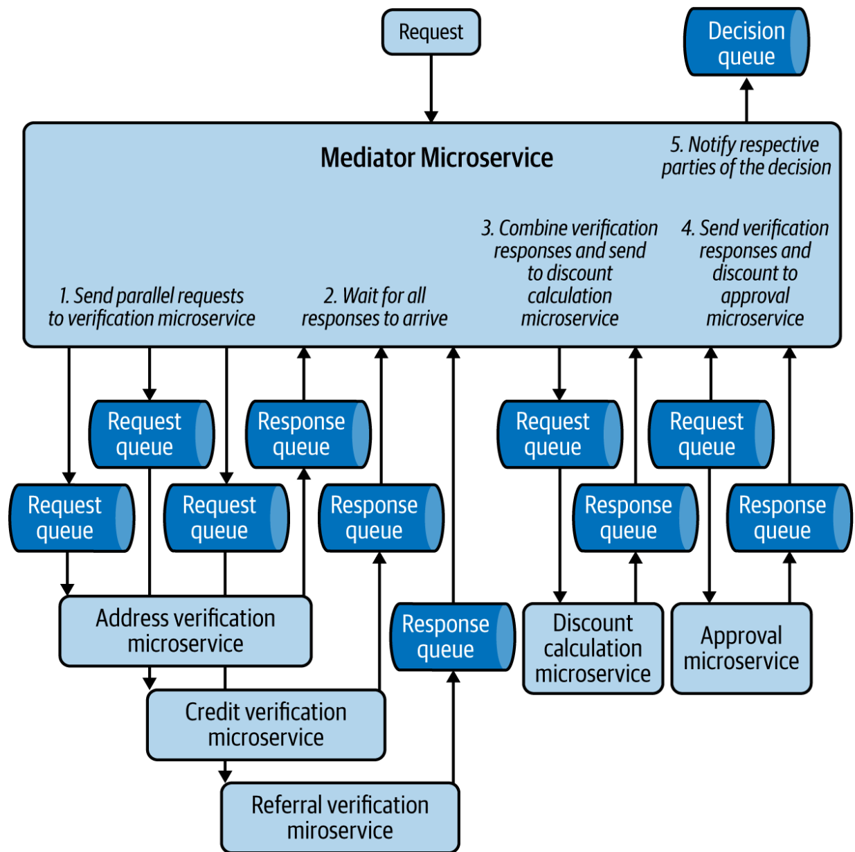
Figure 5-11. Mediator microservice orchestrating a new insurance request
