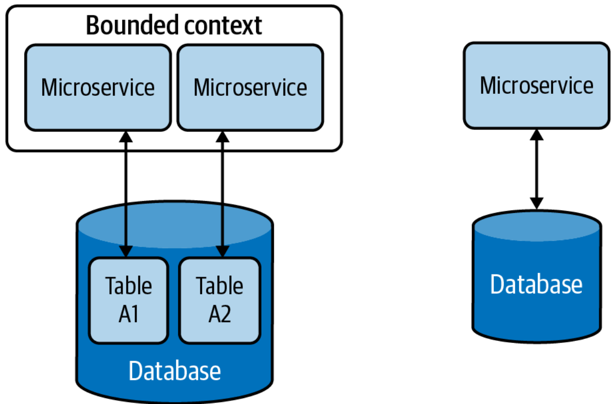
Figure 4-5. Hybrid data management
