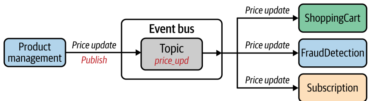
Figure 2-5. Multiple-Receiver pattern for implementing asynchronous message-based communication
