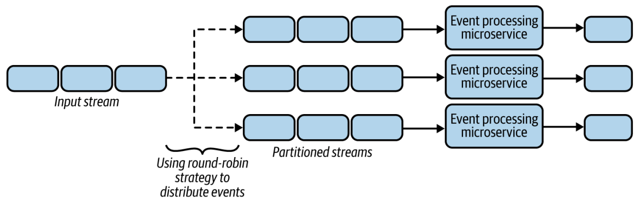
Figure 6-15. Using a simple round-robin strategy to partition events
