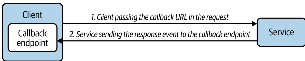
Figure 5-9. Client and server communicating via webhook
