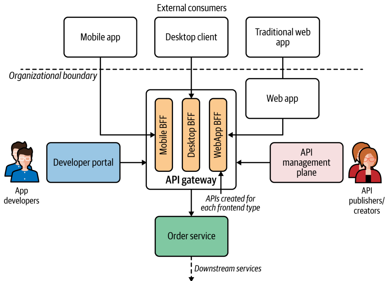
Figure 7-8. The Backend for Frontends pattern in action: each frontend application has a corresponding backend for frontend API/service at the API gateway
