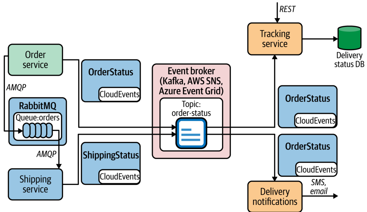
Figure 8-5. Event-driven communication with event sourcing and CloudEvents
