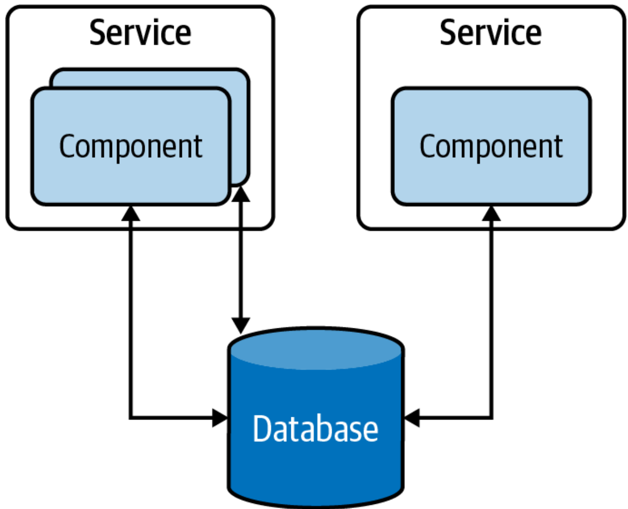
Figure 4-3. Centralized data management in a traditional data-centric application
