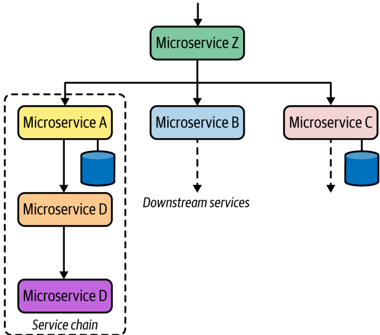
Figure 3-22. Service Orchestration logic implemented in Microservice Z
