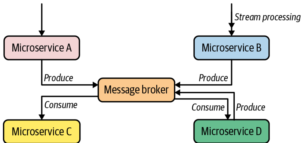
Figure 3-24. Service Choreography pattern
