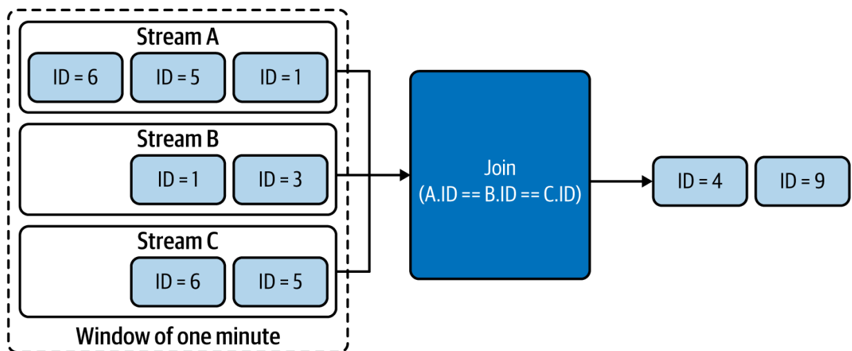
Figure 6-5. Stream Join based on events that have arrived during the last minute
