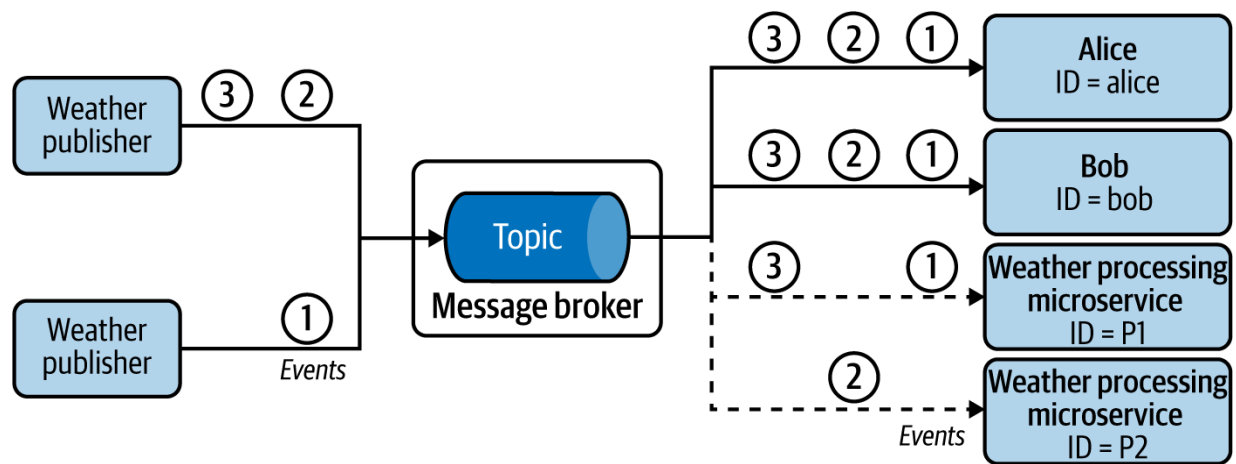
Figure 5-4. Replicating and distributing weather events across multiple microservices
