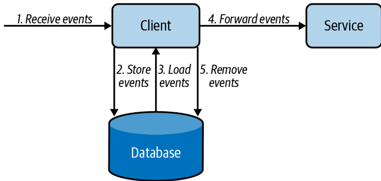
Figure 5-6. Store and Forward event delivery from client to service
