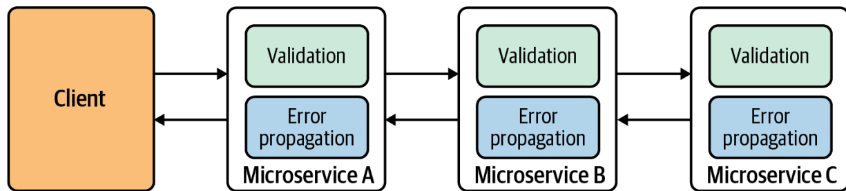
Figure 3-13. Validation of request to achieve fail-fast services
