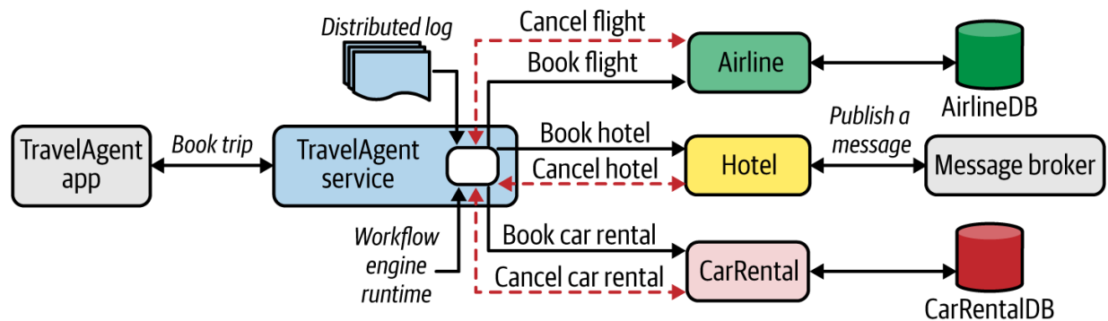
Figure 3-27. Application of Saga pattern in a travel-booking scenario
