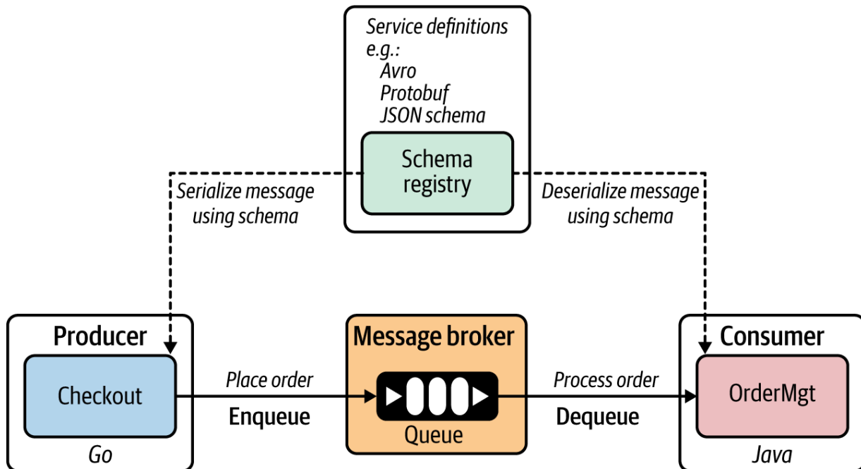
Figure 2-8. The service registry contains the service definitions and schemas for messages exchanged between producers and consumers.
