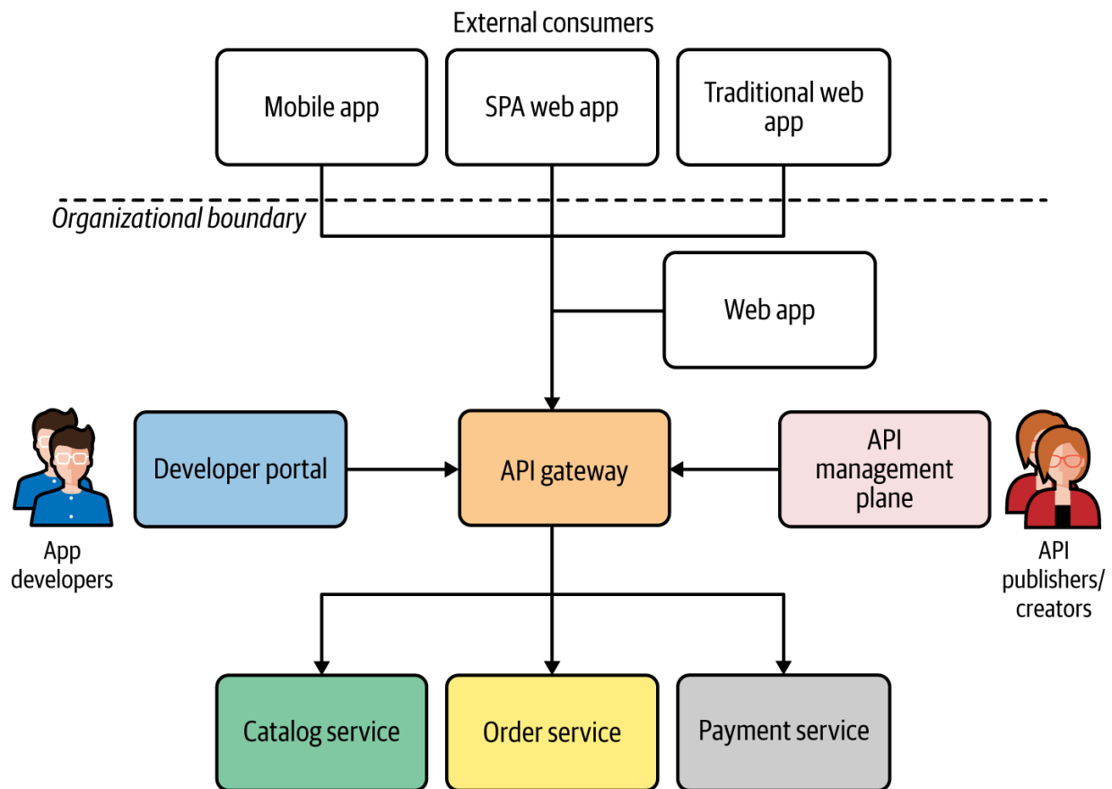
Figure 7-7. Frontends are consuming business capabilities via an API management layer
