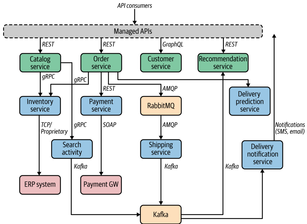
Figure 8-3. Connecting services and systems in our online retail application
