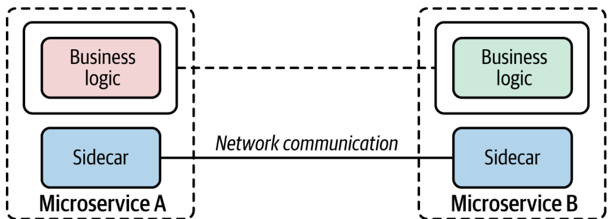
Figure 3-14. Using a sidecar to offload interservice communication
