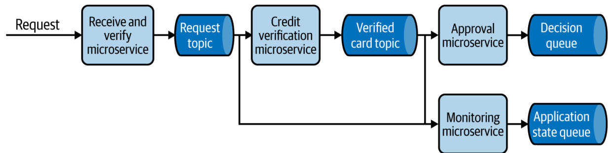
Figure 5-12. A credit card application processing flow using the Pipe and Filter pattern
