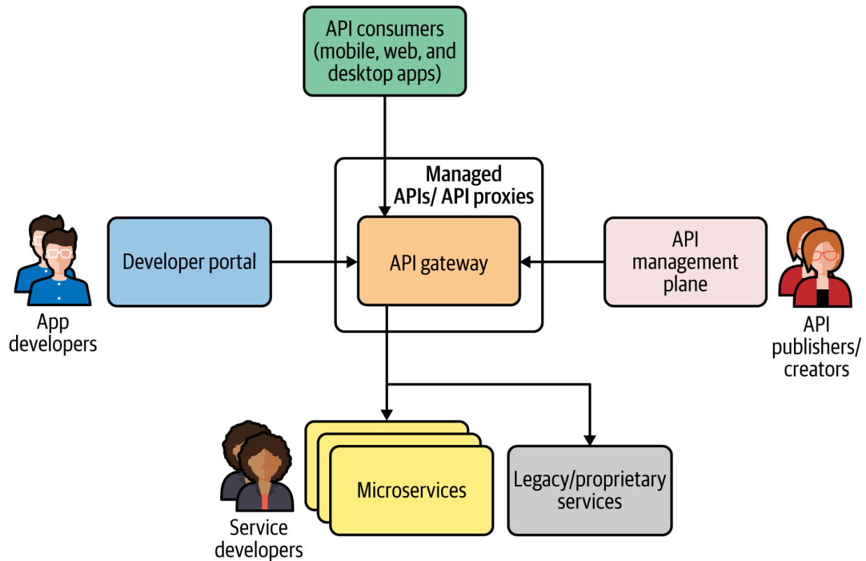
Figure 7-1. API management using API Gateway and associated roles
