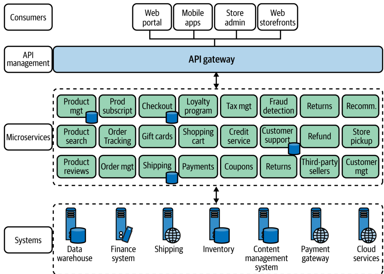
Figure 1-2. An online retail application built using microservices architecture
