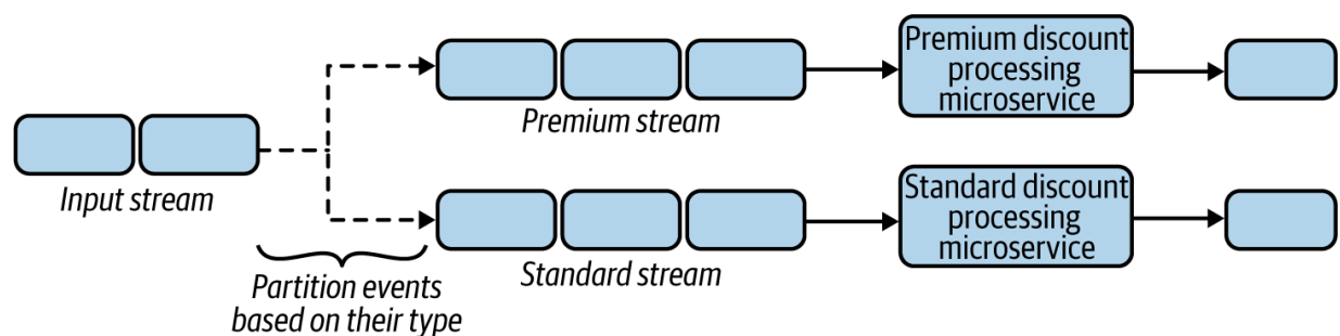
Figure 6-16. Generating different pipelines to process premium and standard events
