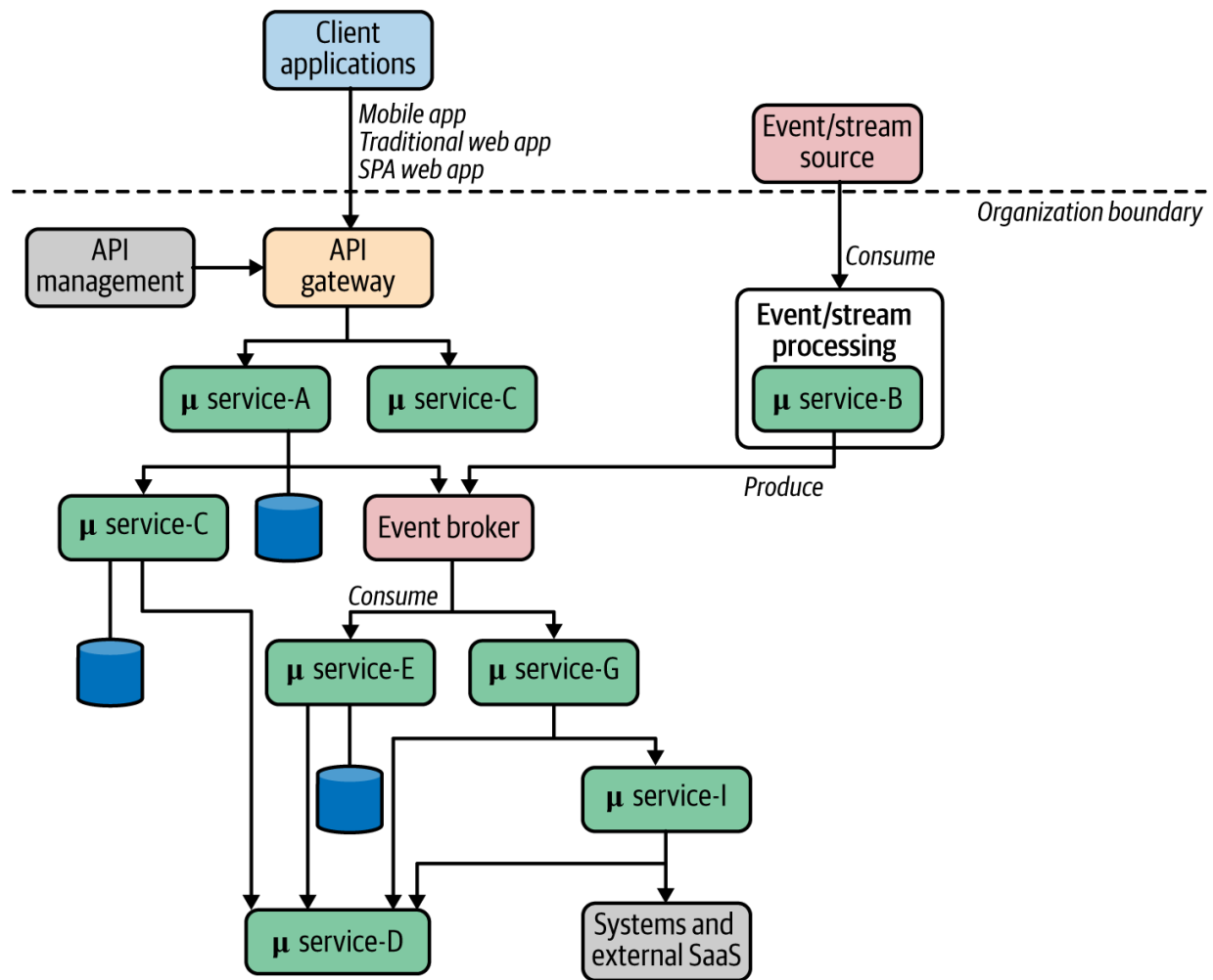
Figure 3-1. Service Connectivity pattern
