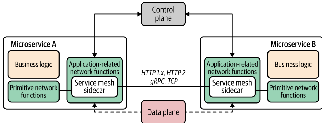
Figure 3-18. Service Mesh components
