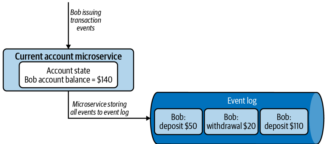
Figure 5-10. Current account microservice generating an event log while updating application state
