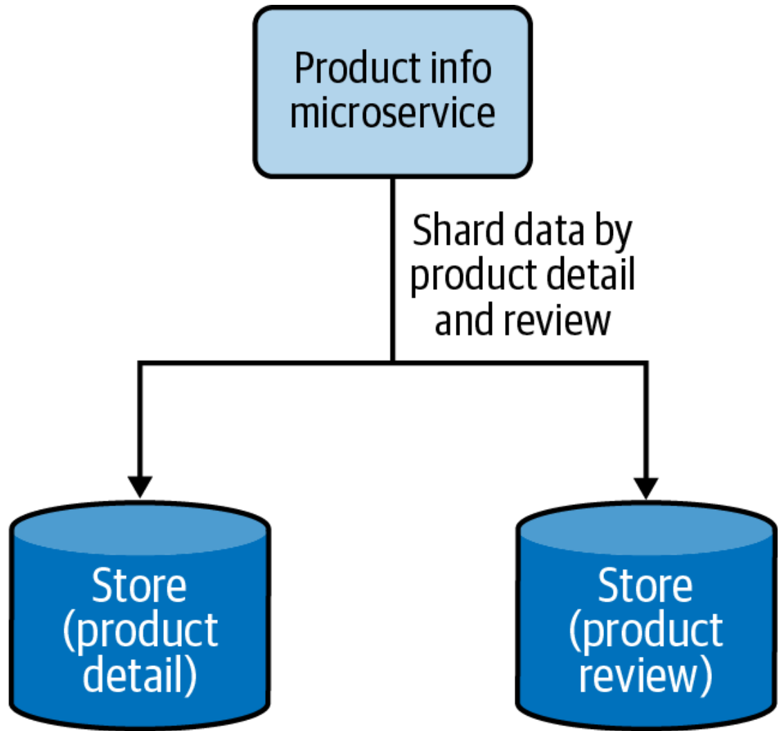
Figure 4-15. Functional data sharding by segregating product details and reviews into two data stores
