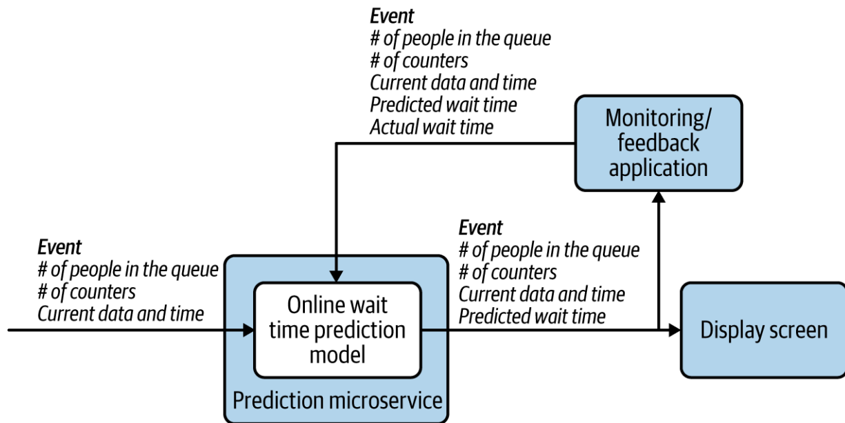
Figure 6-12. Emitting accurate wait-time predictions through feedback
