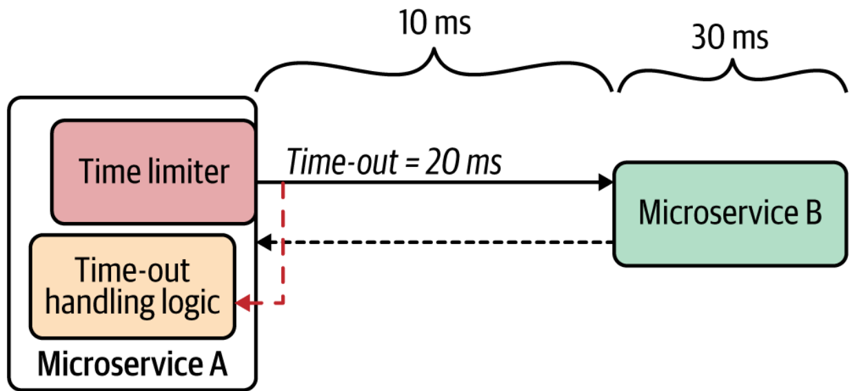
Figure 3-9. Resilient connectivity with time-outs
