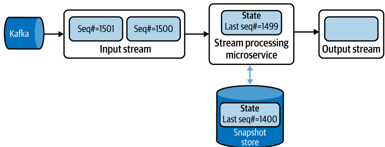
Figure 6-23. Storing periodic state snapshots with Kafka event sequence numbers
