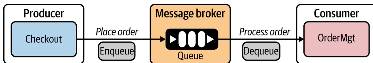
Figure 2-4. Single-Receiver pattern for implementing asynchronous message-based commands
