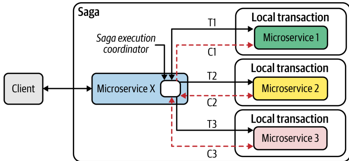
Figure 3-26. Service Composition with distributed transactions using the Saga pattern
