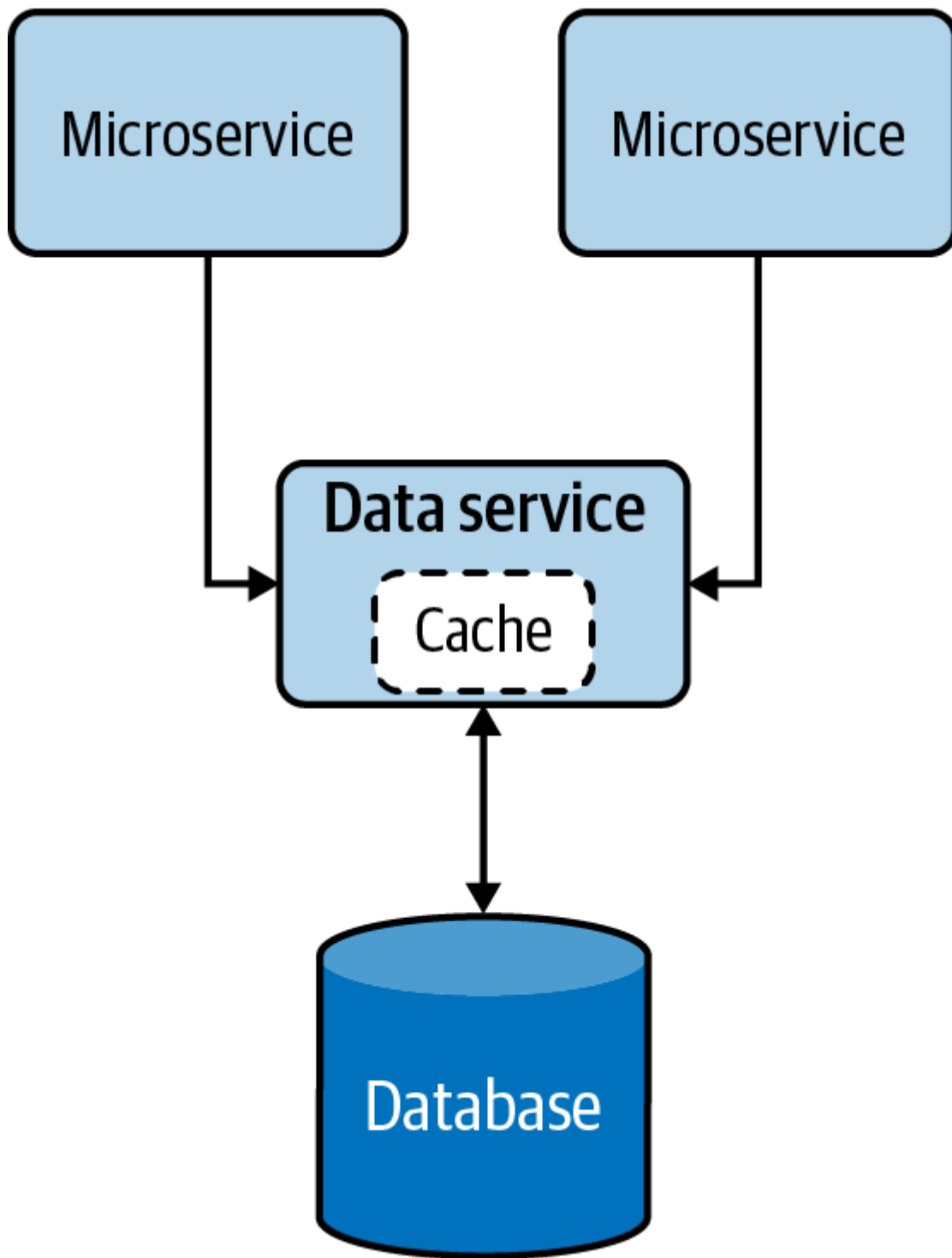
Figure 4-10. Data Service pattern
