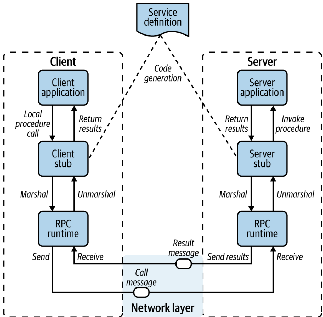
Figure 2-2. Implementation of Remote Procedure Calls pattern
