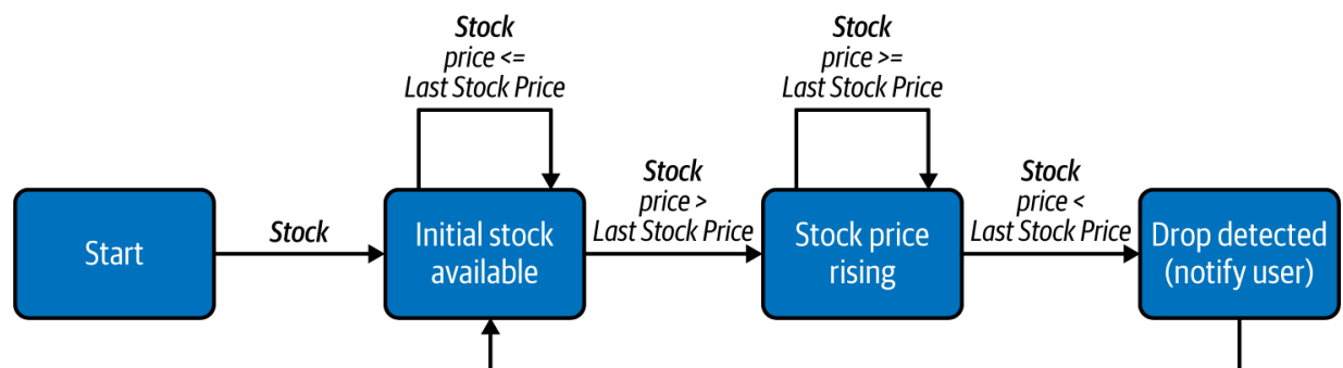
Figure 6-7. Using the Temporal Event Ordering pattern to detect a continuous stock price increase followed by a single drop
