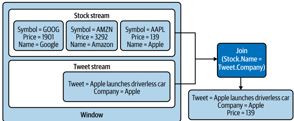
Figure 6-6. Joining stock prices with tweets based on company name
