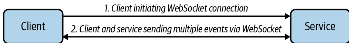
Figure 5-8. Client and service communicating via the WebSocket protocol
