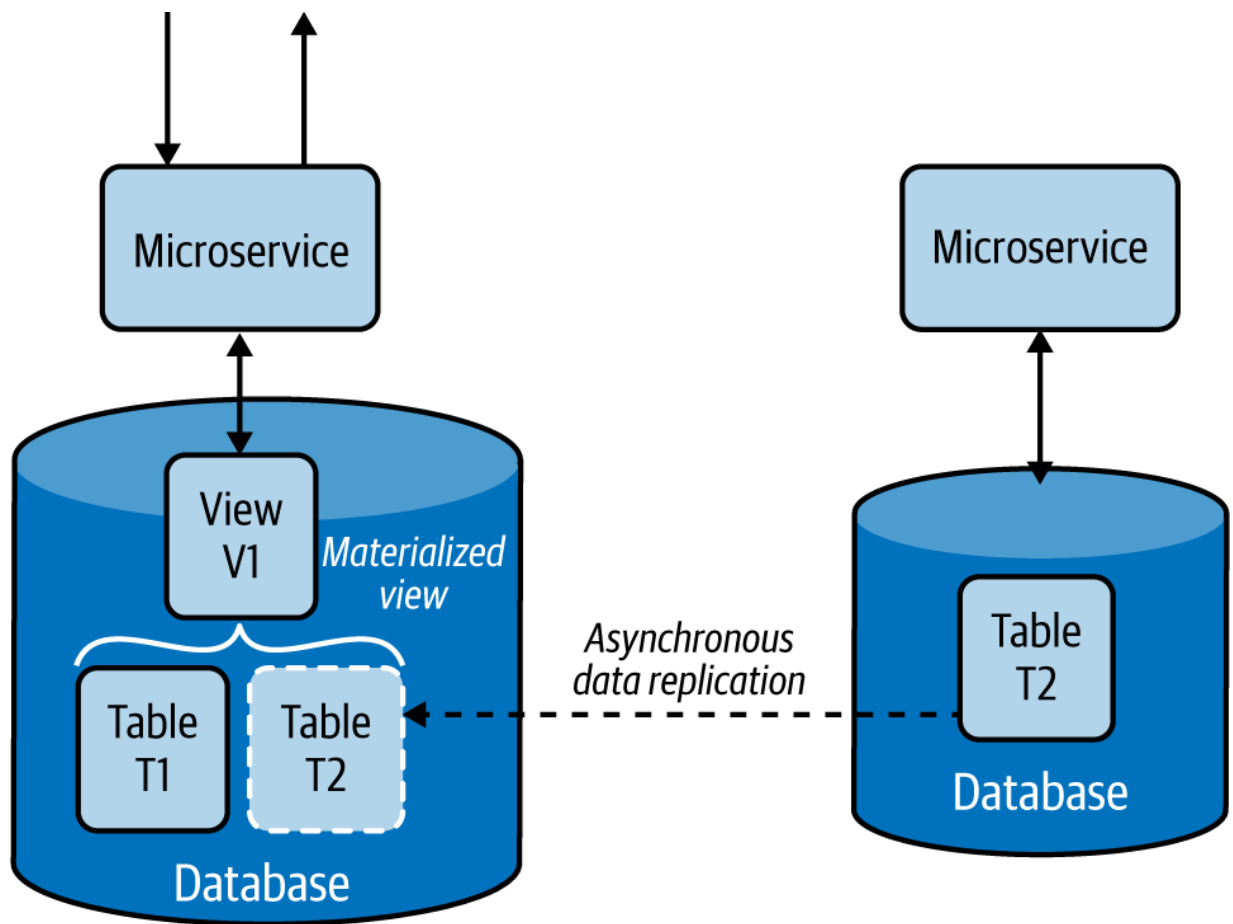
Figure 4-17. Service built with the Materialized View pattern
