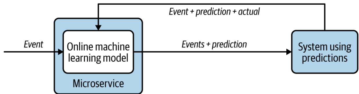
Figure 6-10. Microservice with an online machine learning model using a feedback loop to continuously learn
