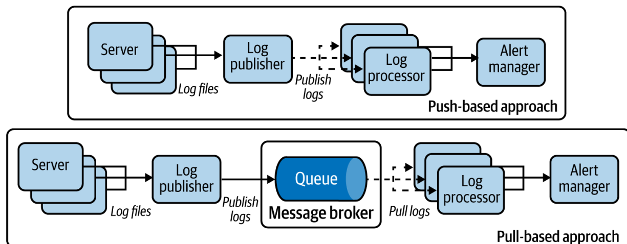
Figure 5-2. Handling bursts of logs with push- and pull-based approaches
