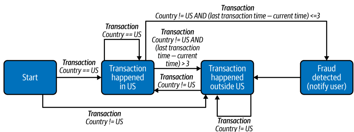
Figure 6-8. State machine for detecting transaction fraud
