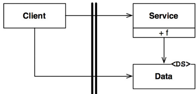
Figure 18.1 Flow of control crosses the boundary from a lower level to a higher level
