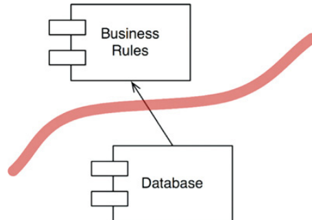
Figure 17.3 The business rules and database components
