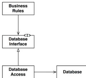
Figure 17.1 The database behind an interface
