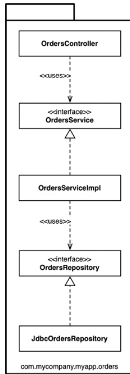
Figure 34.2 Package by feature
