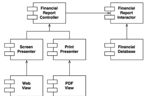
Figure 8.3 The component relationships are unidirectional
