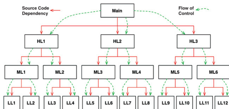
Figure 5.1 Source code dependencies versus flow of control
