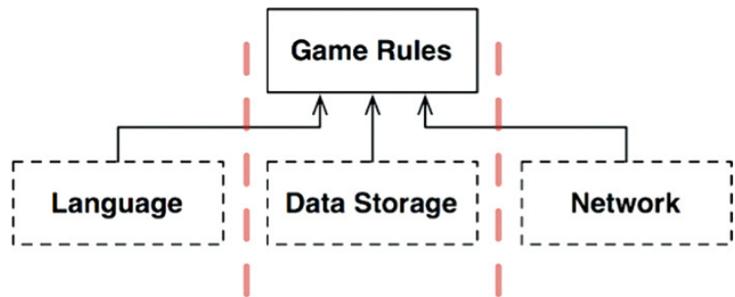
Figure 25.5 Adding a network component
