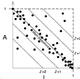
Figure 14.14 Scatterplot of the components
