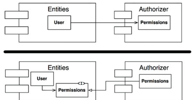
Figure 14.3 Inverting the dependency between Entities and Authorizer
