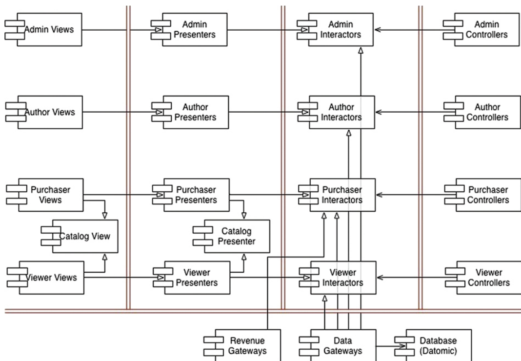
Figure 33.2 A preliminary component architecture
