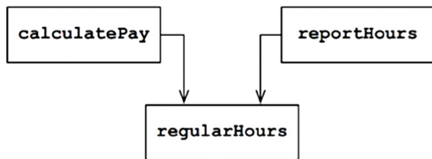
Figure 7.2 Shared algorithm
