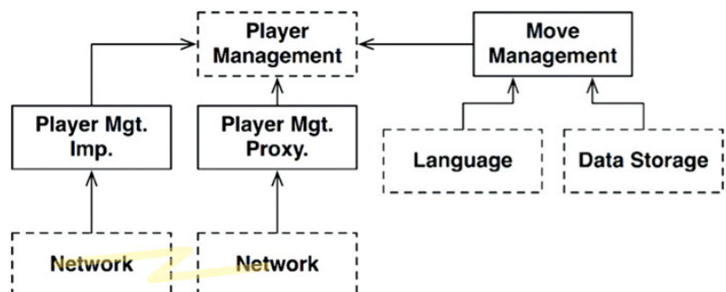
Figure 25.7 Adding a micro-service API
