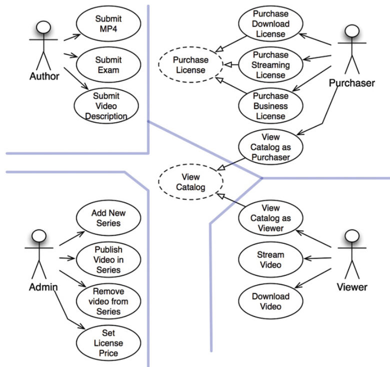
Figure 33.1 A typical use-case analysis
