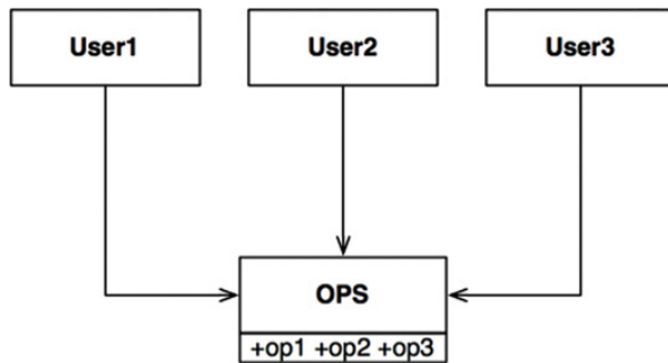
Figure 10.1 The Interface Segregation Principle
