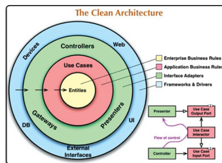
Figure 22.1 The clean architecture
