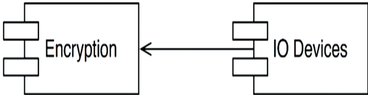
Figure 19.3 Lower-level components should plug in to higher-level components
