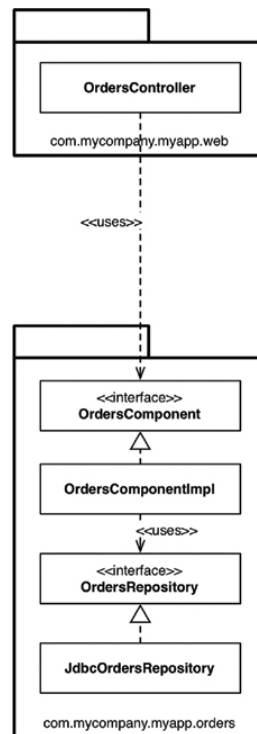
Figure 34.6 View orders use case
