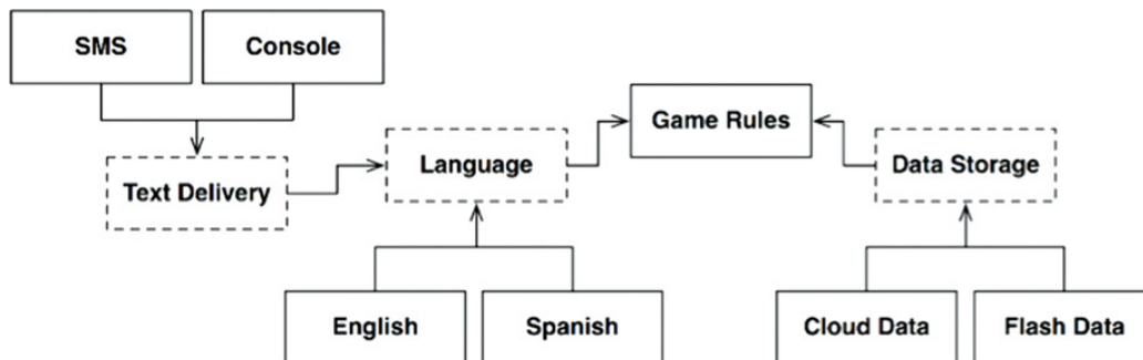
Figure 25.3 The revised diagram
