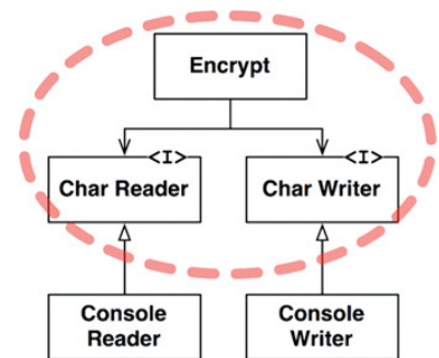
Figure 19.2 Class diagram showing a better architecture for the system
