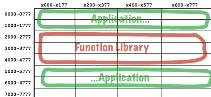
Figure 12.2 Splitting the application into two address segments
