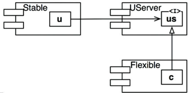
Figure 14.11 C implements the interface class US
