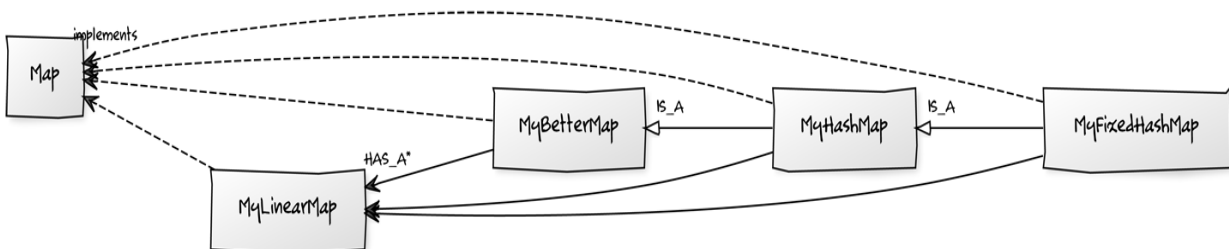
Figure 11-2. UML diagram for the classes in this chapter.
