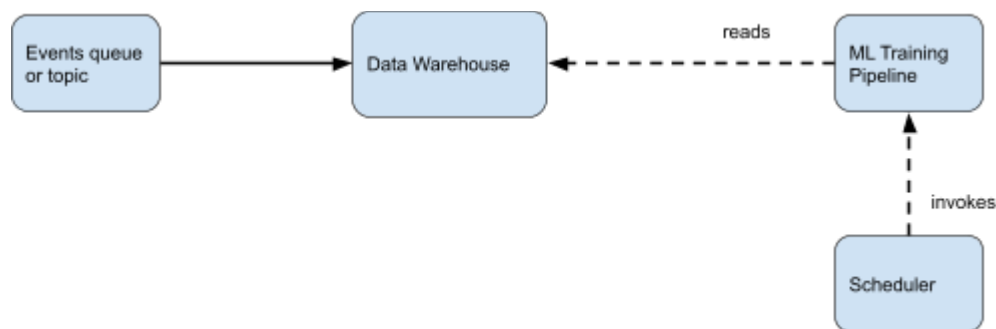
Figure 9-14. Scheduled Training.
