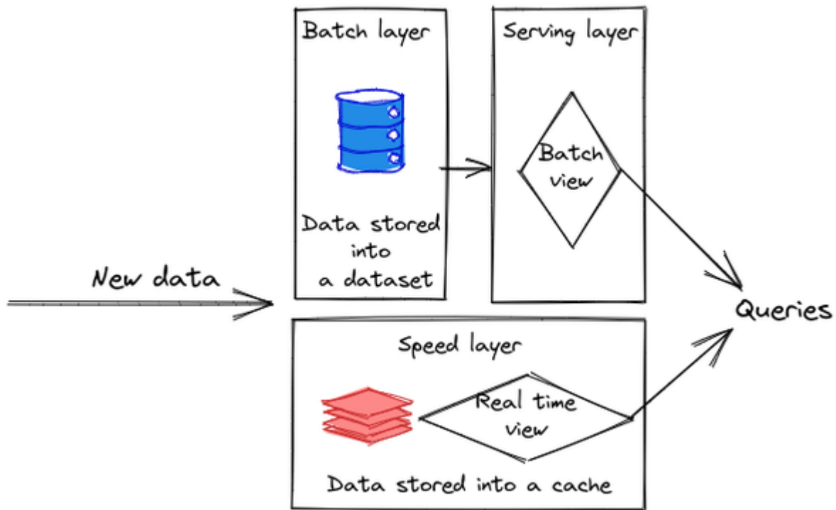
Figure 6-3. Lambda architecture
