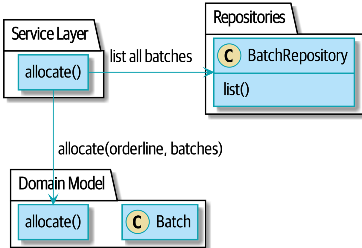
Figure 7-2. Before: allocate against all batches using the domain service
