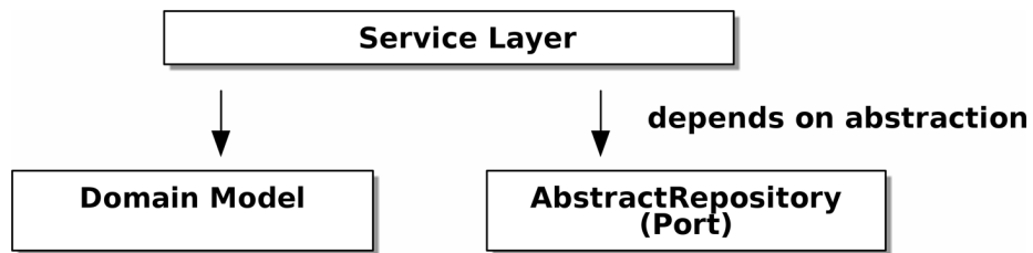
Figure 4-3. Abstract dependencies of the service layer
