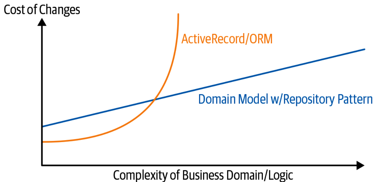
Figure 2-6. Domain model trade-offs as a diagram
