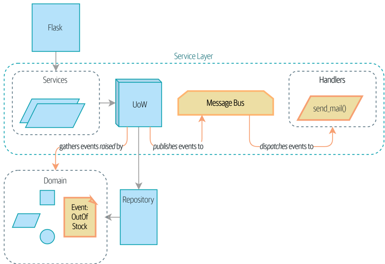
Figure 8-1. Events flowing through the system
