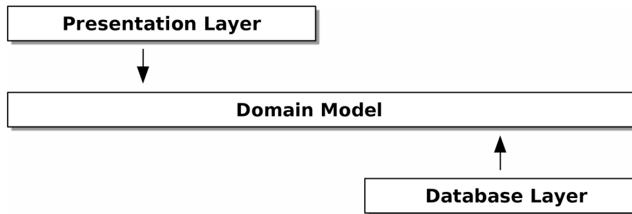
Figure 2-3. Onion architecture
