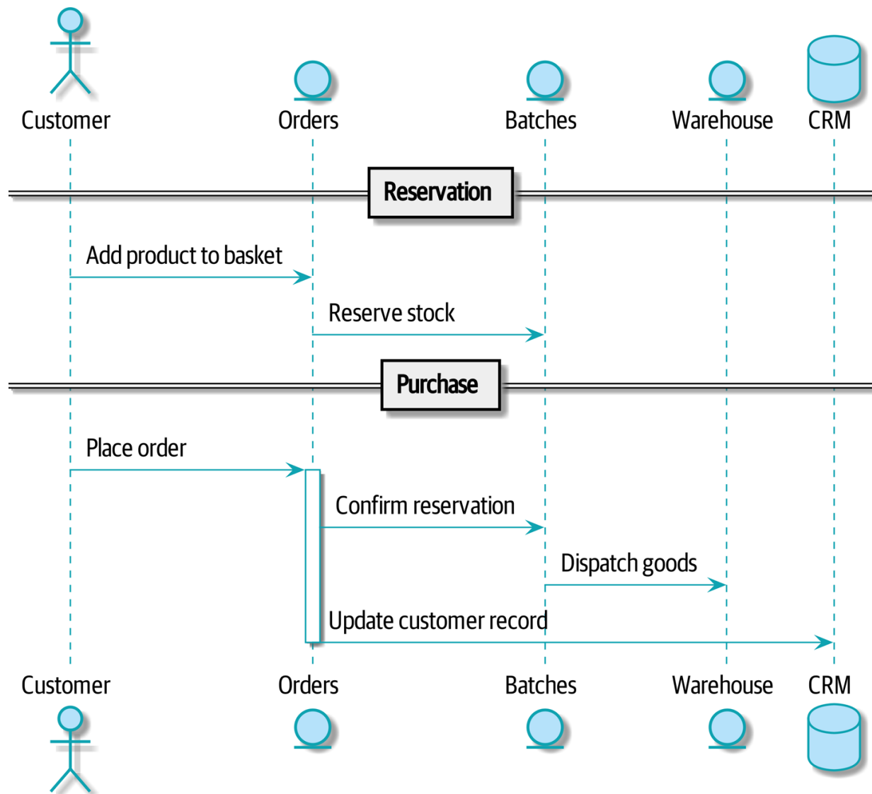
Figure 11-3. Command flow 1
