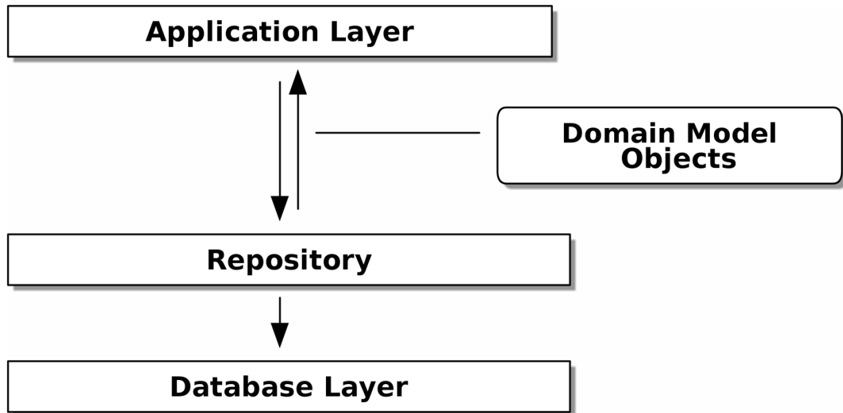
Figure 2-5. Repository pattern
