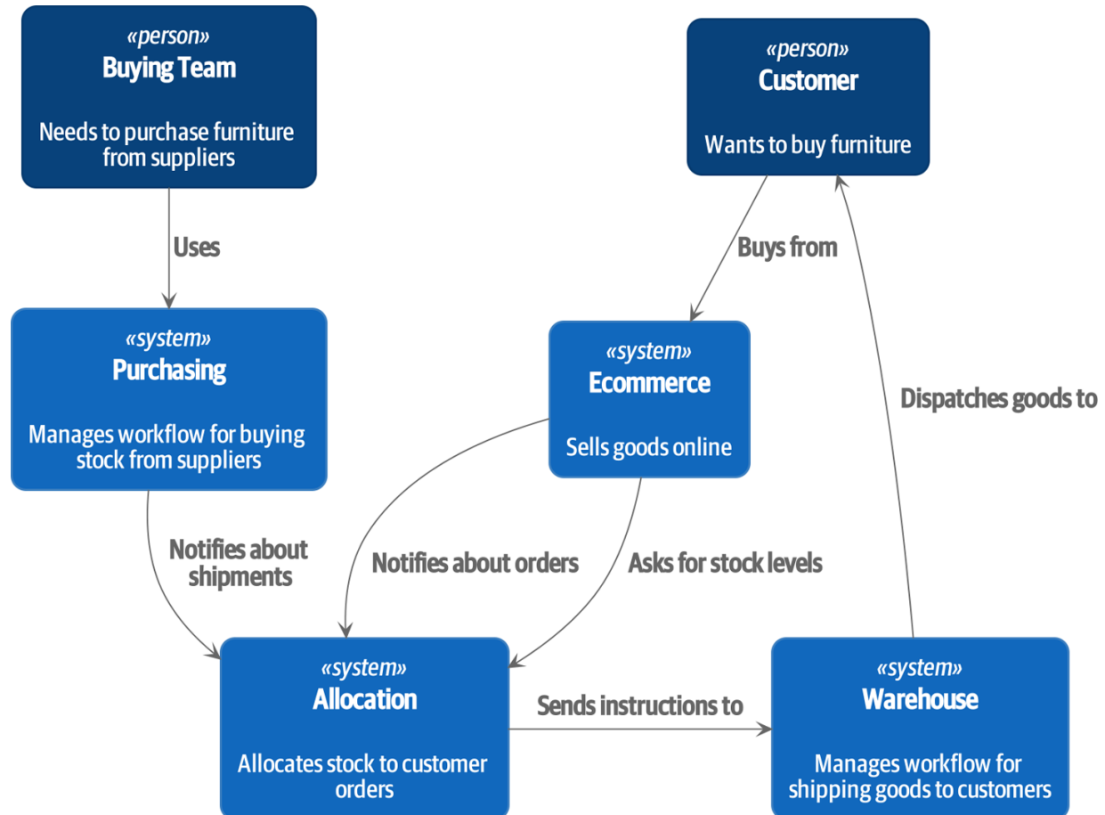
Figure 1-2. Context diagram for the allocation service
