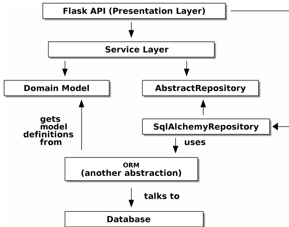
Figure 4-5. Dependencies at runtime
