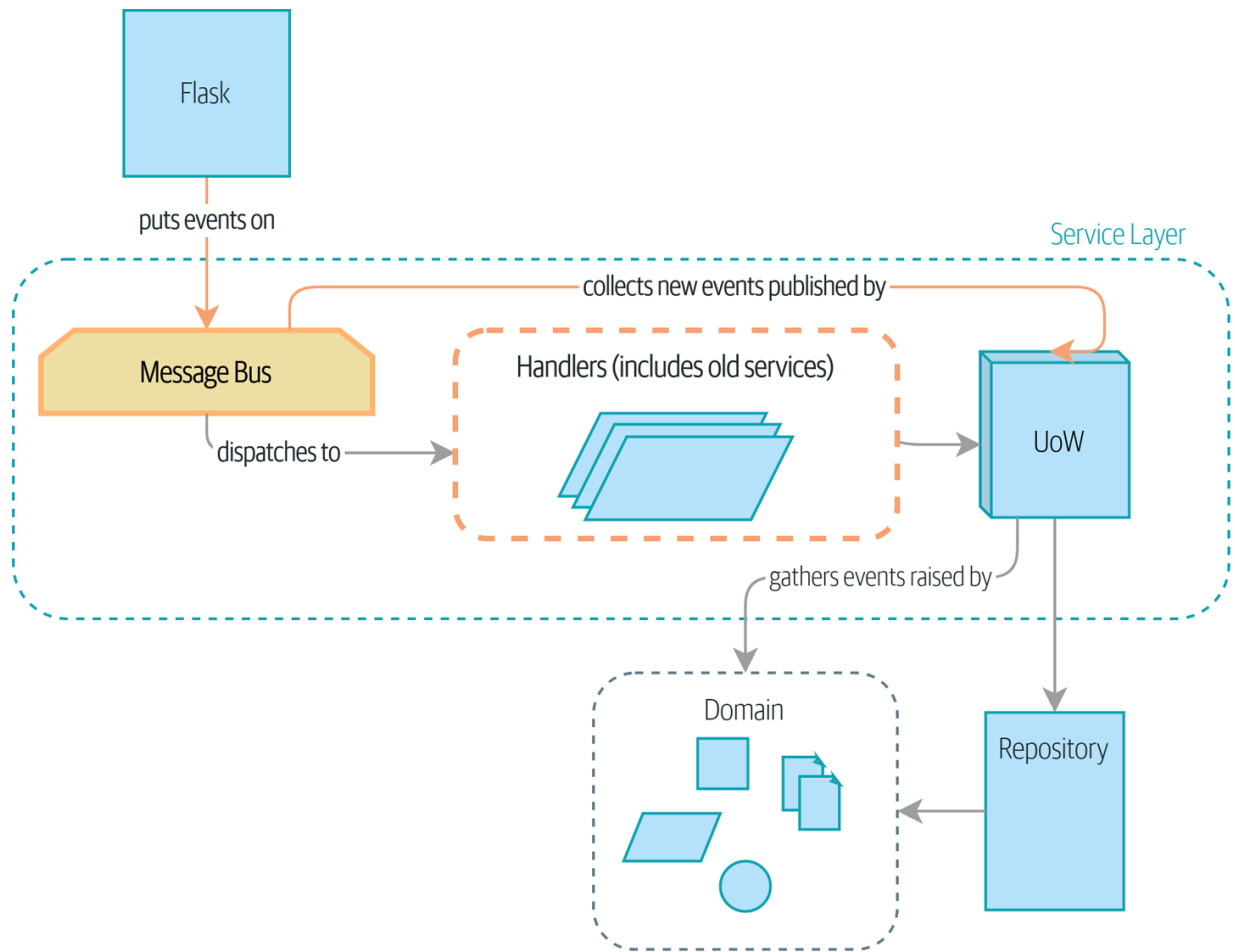
Figure 9-2. The message bus is now the main entryptpoint to the service layer
