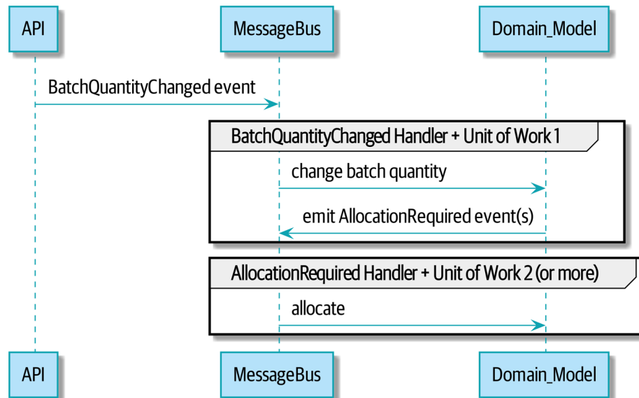
Figure 9-4. Sequence diagram for reallocation flow
