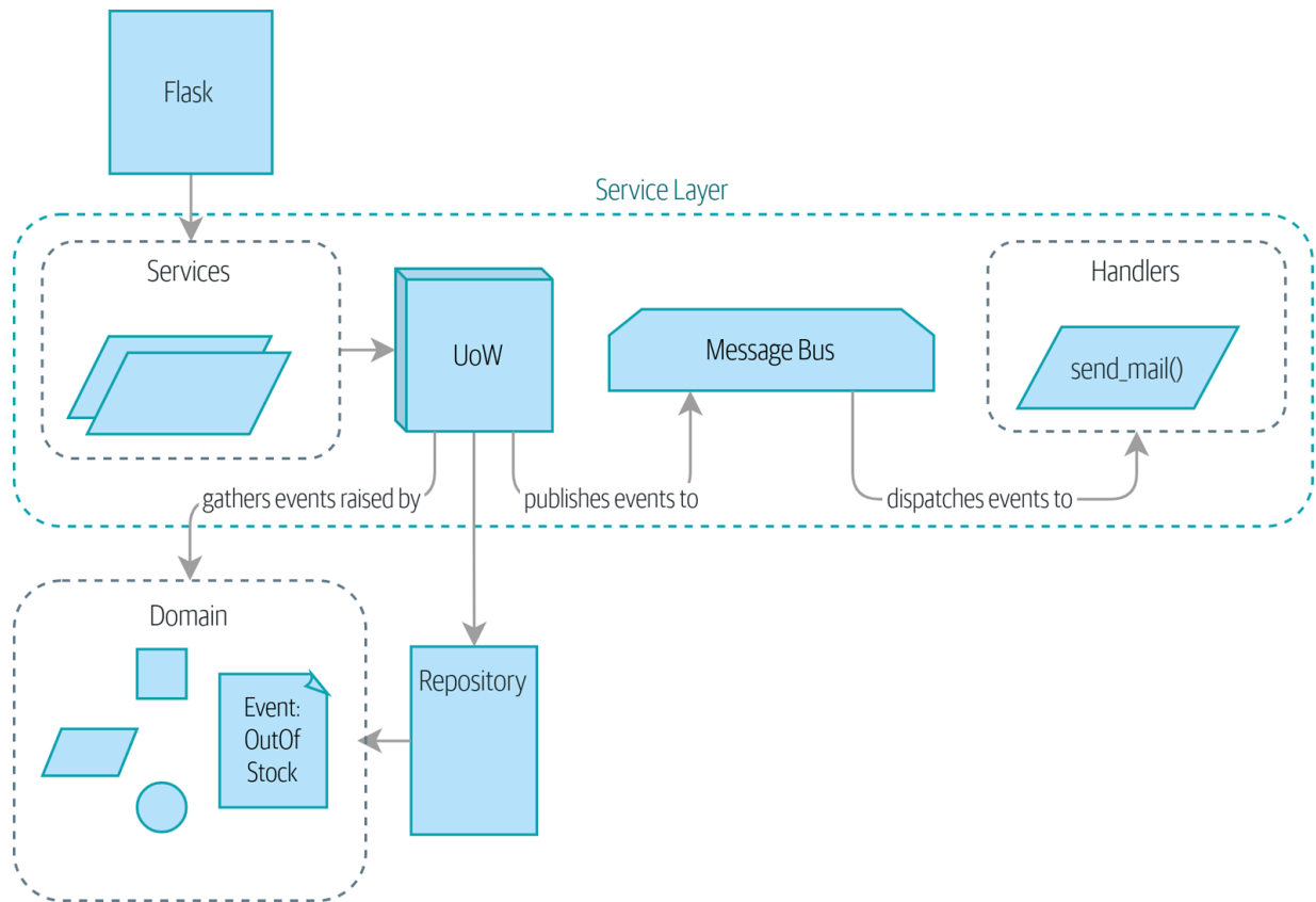
Figure 9-1. Before: the message bus is an optional add-on
