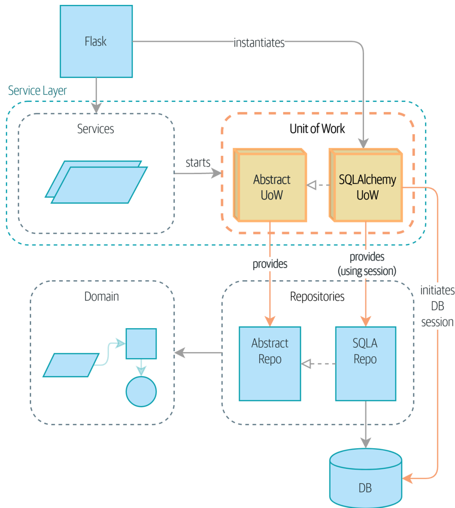
Figure 6-2. With UoW: UoW now manages database state
