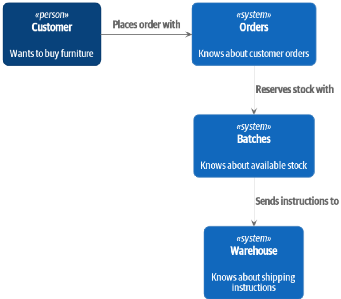
Figure 11-2. Context diagram with noun-based services
