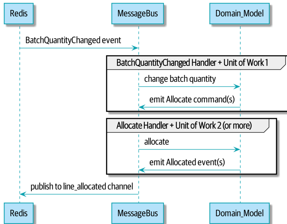
Figure 11-6. Sequence diagram for reallocation flow
