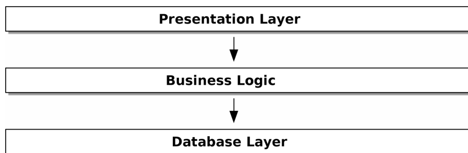
Figure 2-2. Layered architecture
