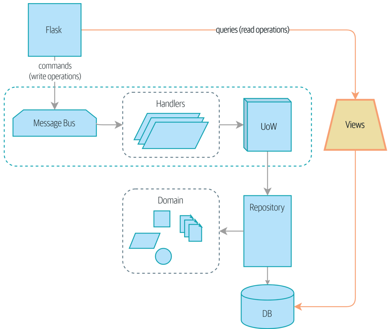
Figure 12-1. Separating reads from writes
