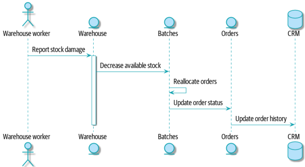
Figure 11-4. Command flow 2
