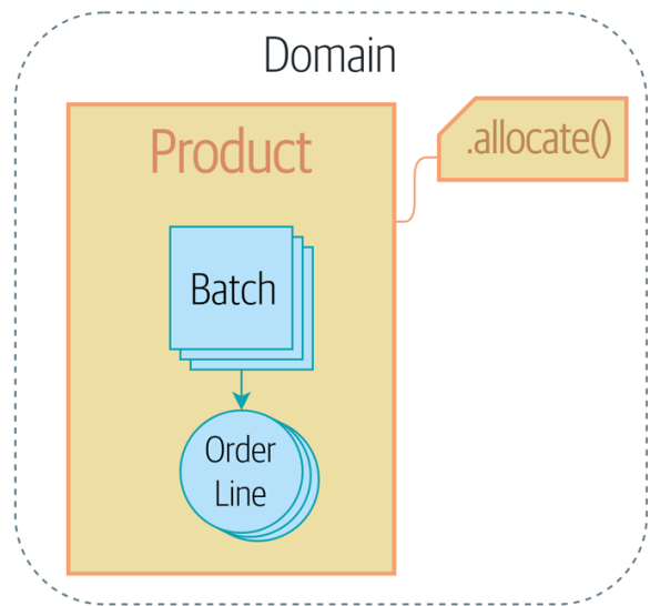
Figure 7-1. Adding the Product aggregate
