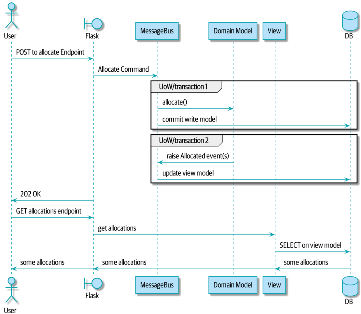
Figure 12-2. Sequence diagram for read model
