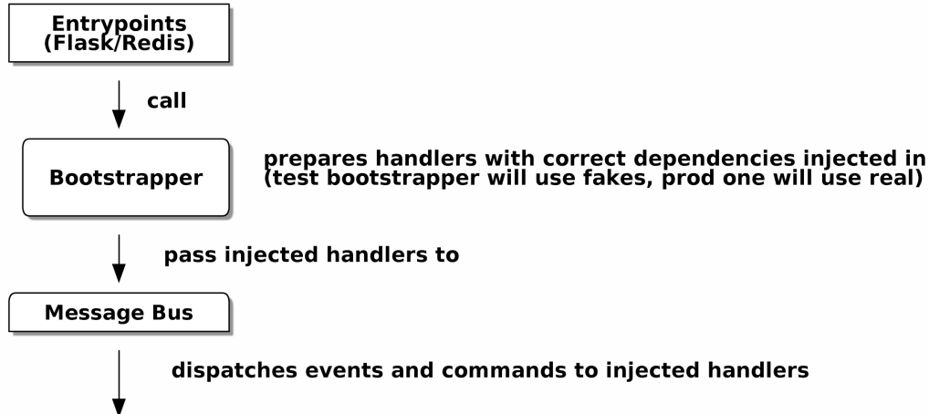
Figure 13-3. Bootstrapper between entrypoints and message bus
