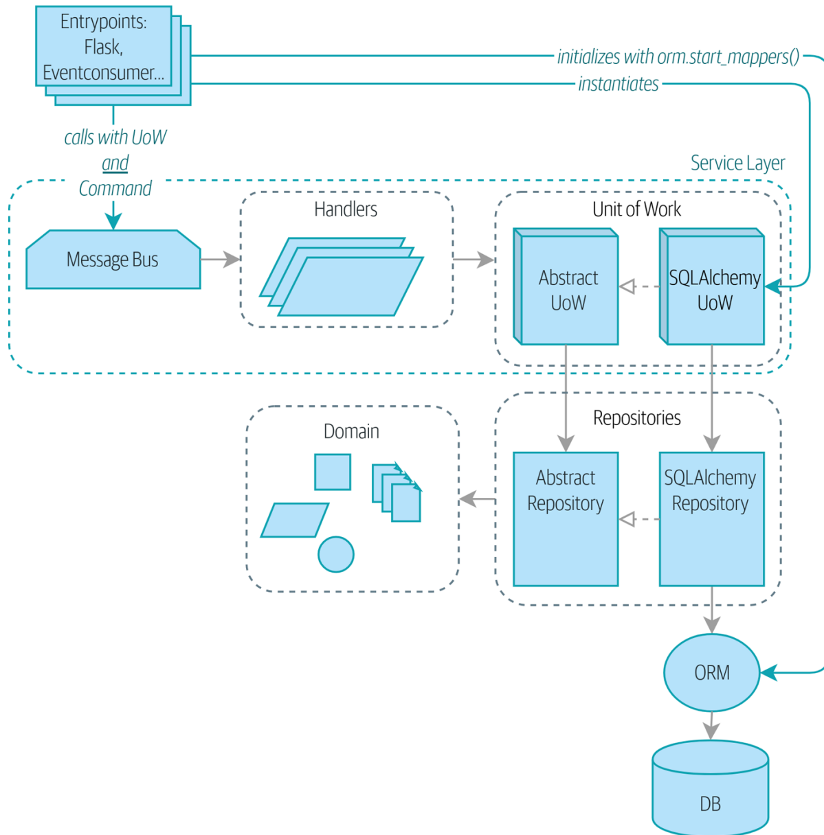
Figure 13-1. Without bootstrap: entrypoints do a lot
