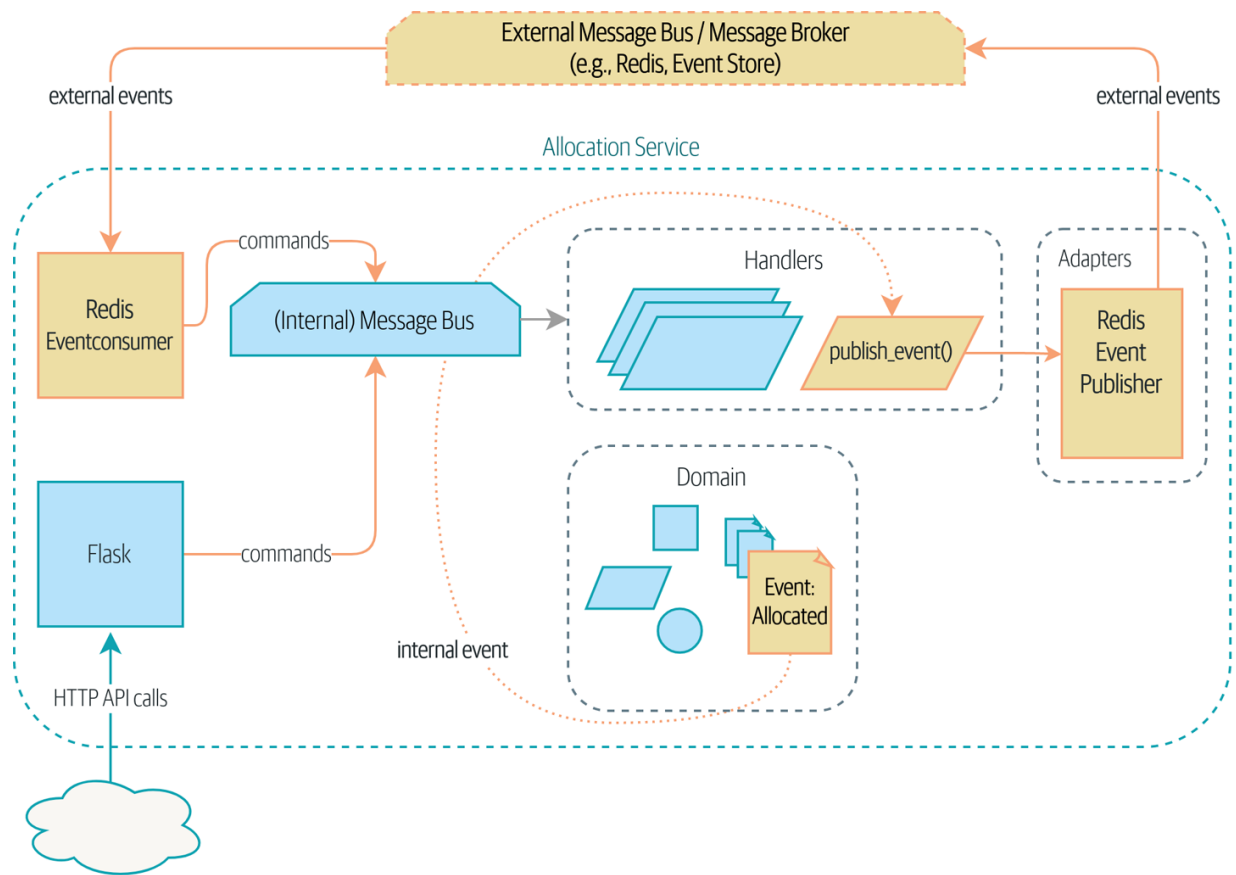
Figure 11-1. Our application is a message processor
