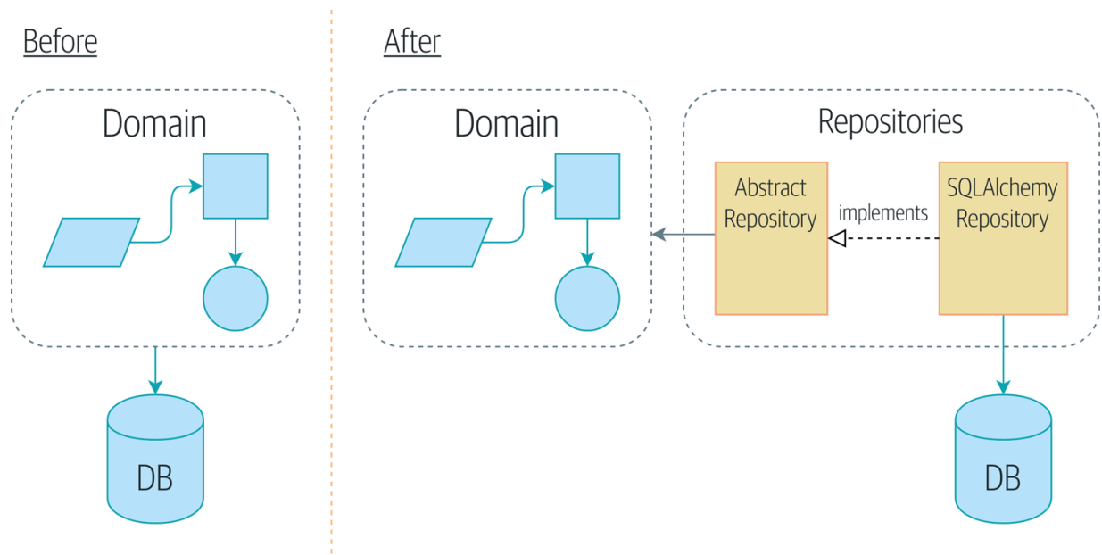
Figure 2-1. Before and after the Repository pattern
