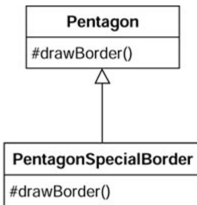
Figure 8-2 PentagonSpecialBorder derives from Pentagon
