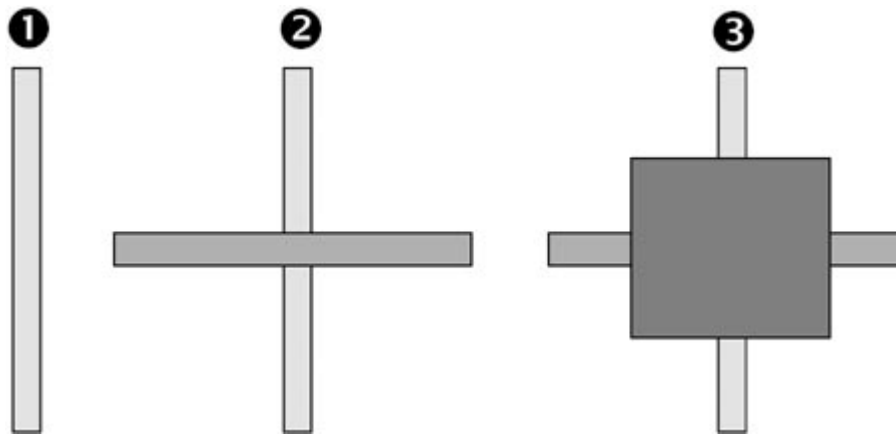
Figure 3-3 A bad approach to cutting out the openings. This sequence results in weakened, bent sheet metal.
