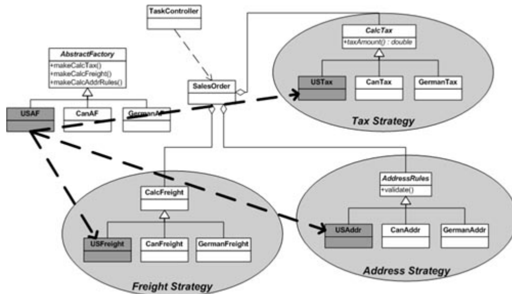
Figure 16.1 High-level application design
