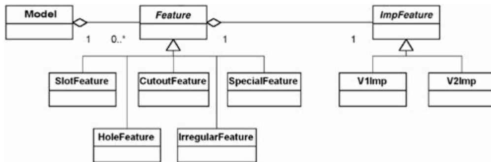
Figure 13-9 Applying the Bridge pattern to the problem.
