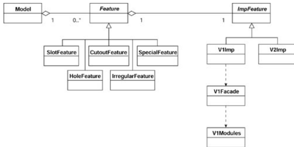
Figure 13-10 After applying the Bridge and Facade patterns.
