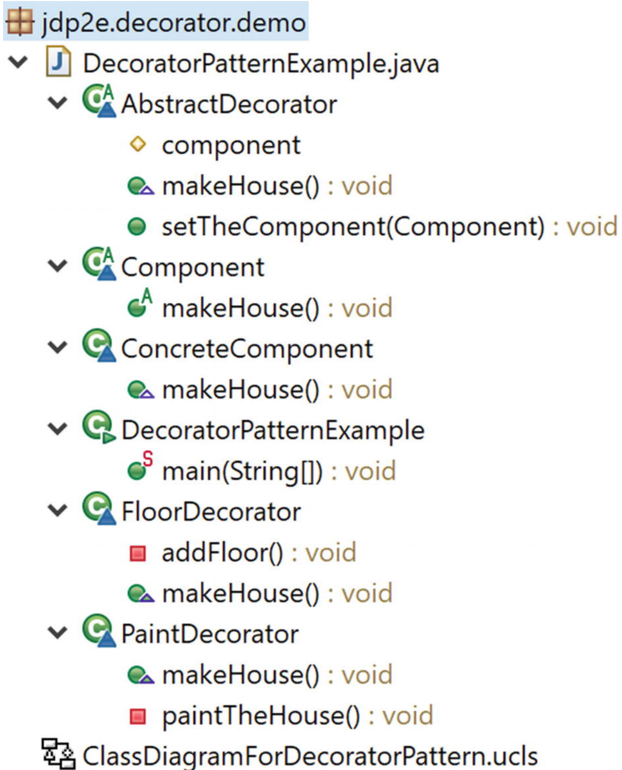
Figure 7-5 Package Explorer view
