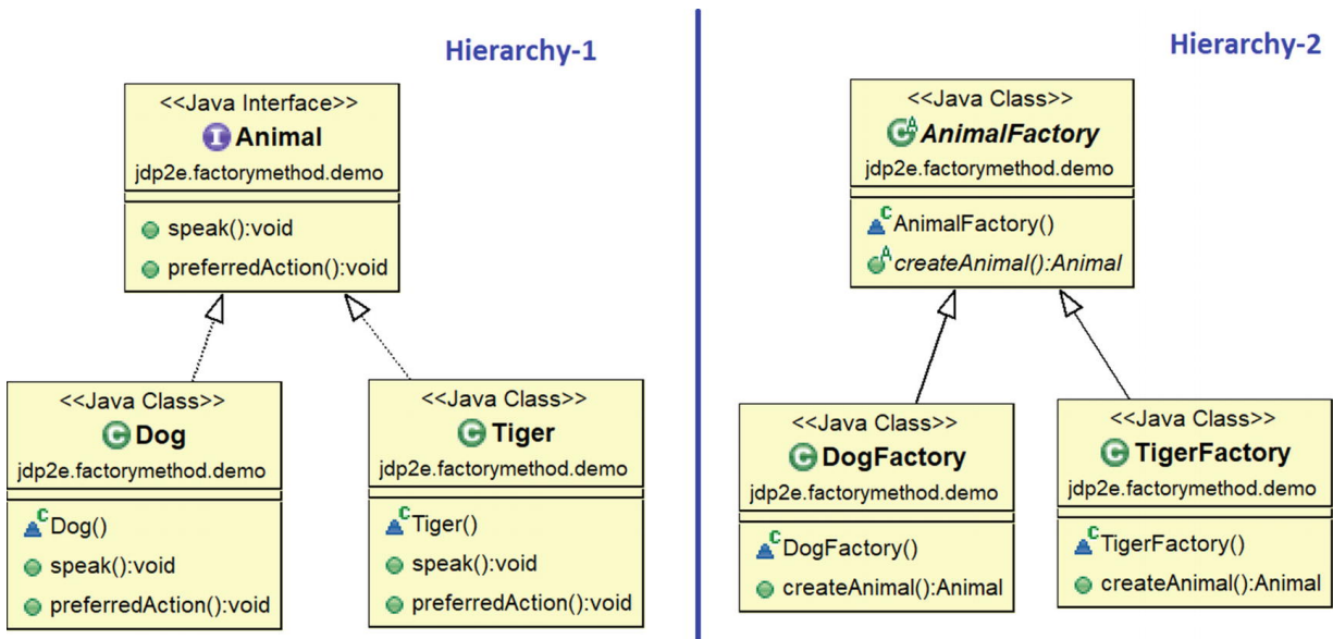
Figure 4-3 The two class hierarchies in our example
