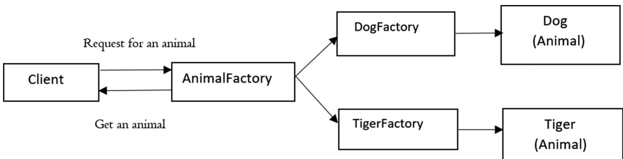
Figure 5-5 Factory method pattern
