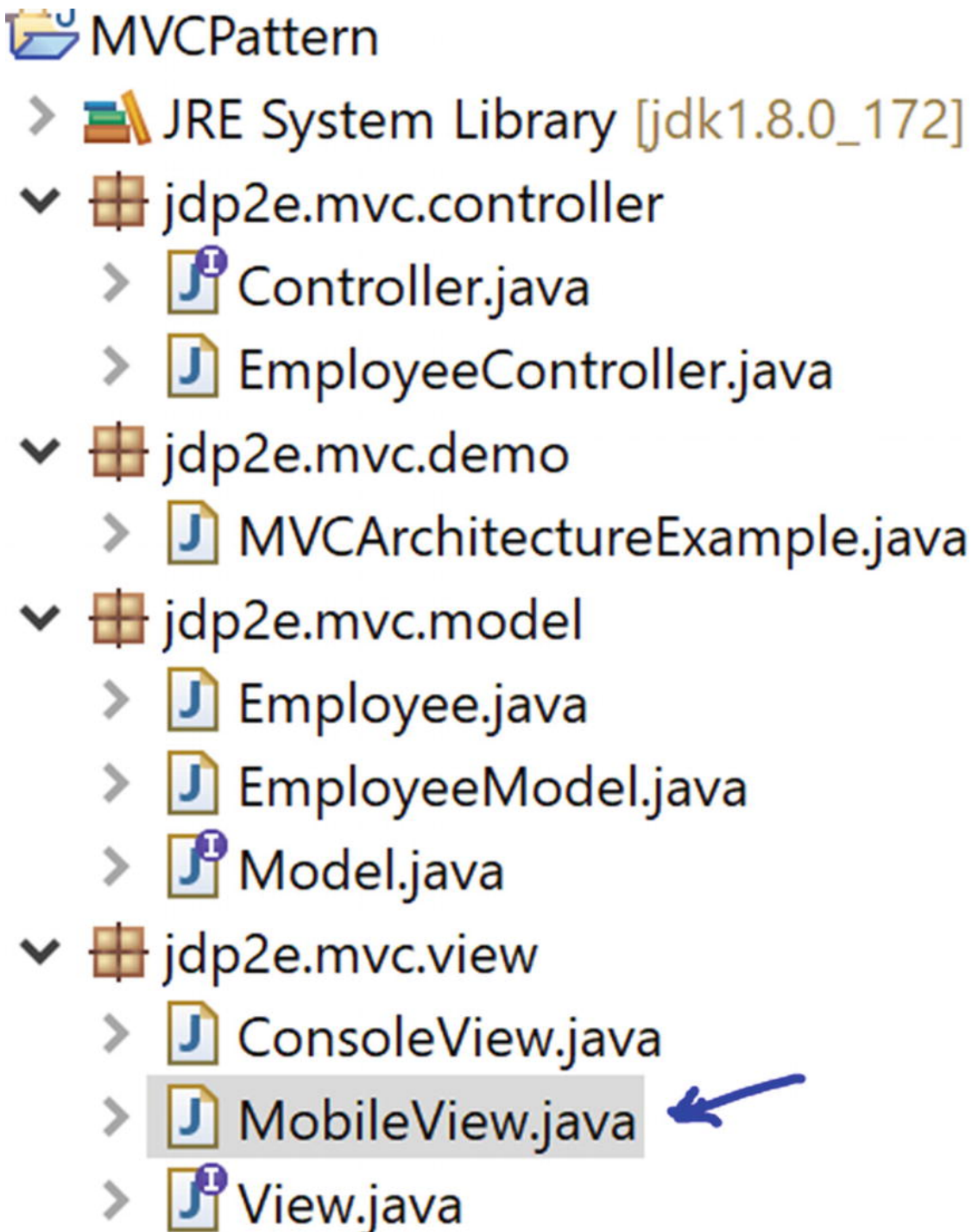
Figure 26-8 Modified Package Explorer view
