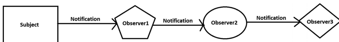
Figure 14-9 The basic workflow of a chain of responsibility pattern
