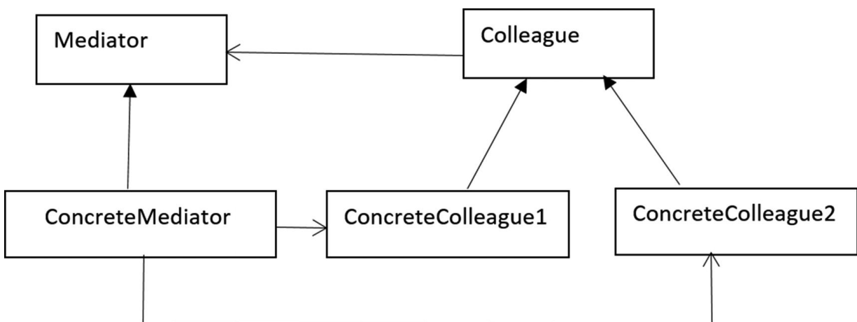
Figure 21-1 Mediator pattern example
