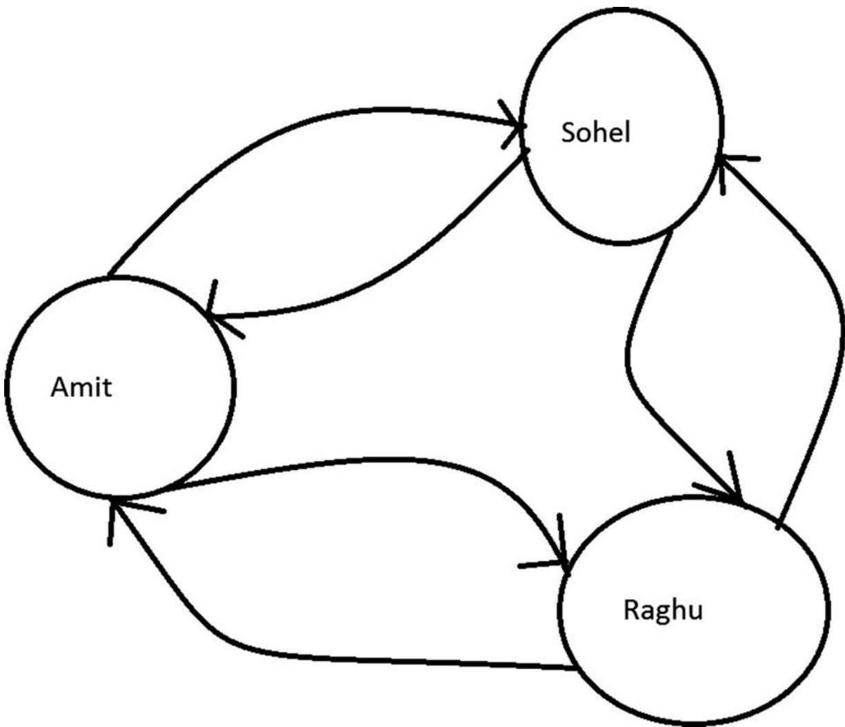
Figure 21-6 Communication without using a mediator
