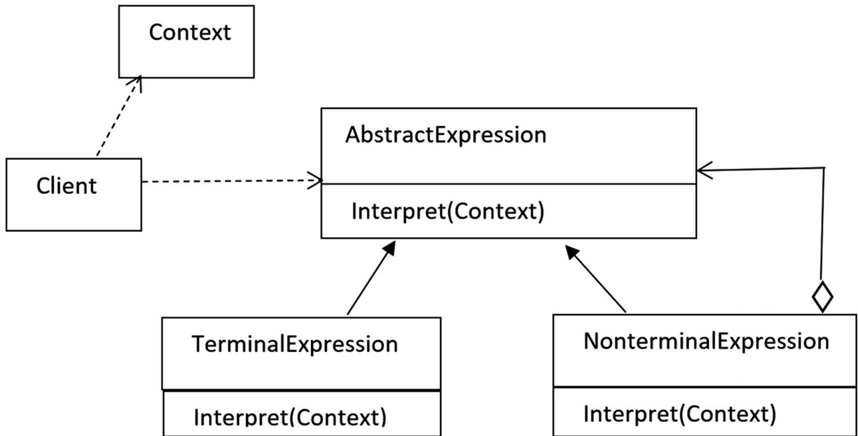
Figure 23-1 Structure of a typical interpreter pattern
