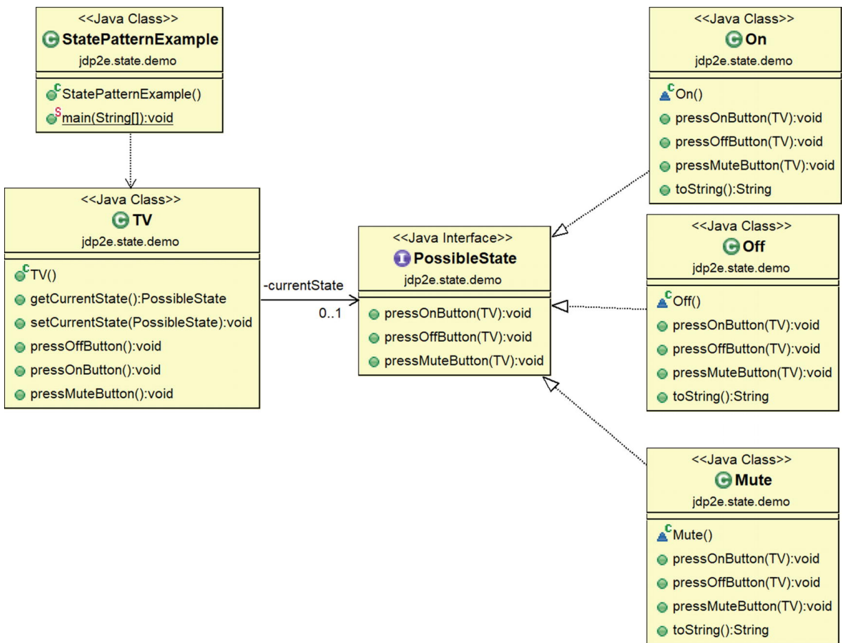
Figure 20-2 Class diagram
