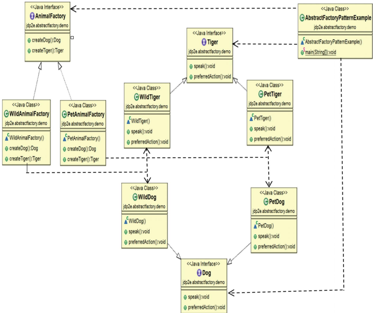
Figure 5-2 Class diagram
