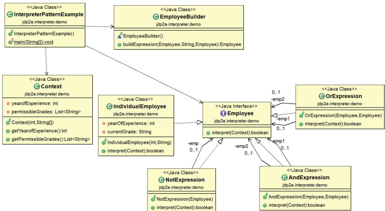
Figure 23-2 Class diagram
