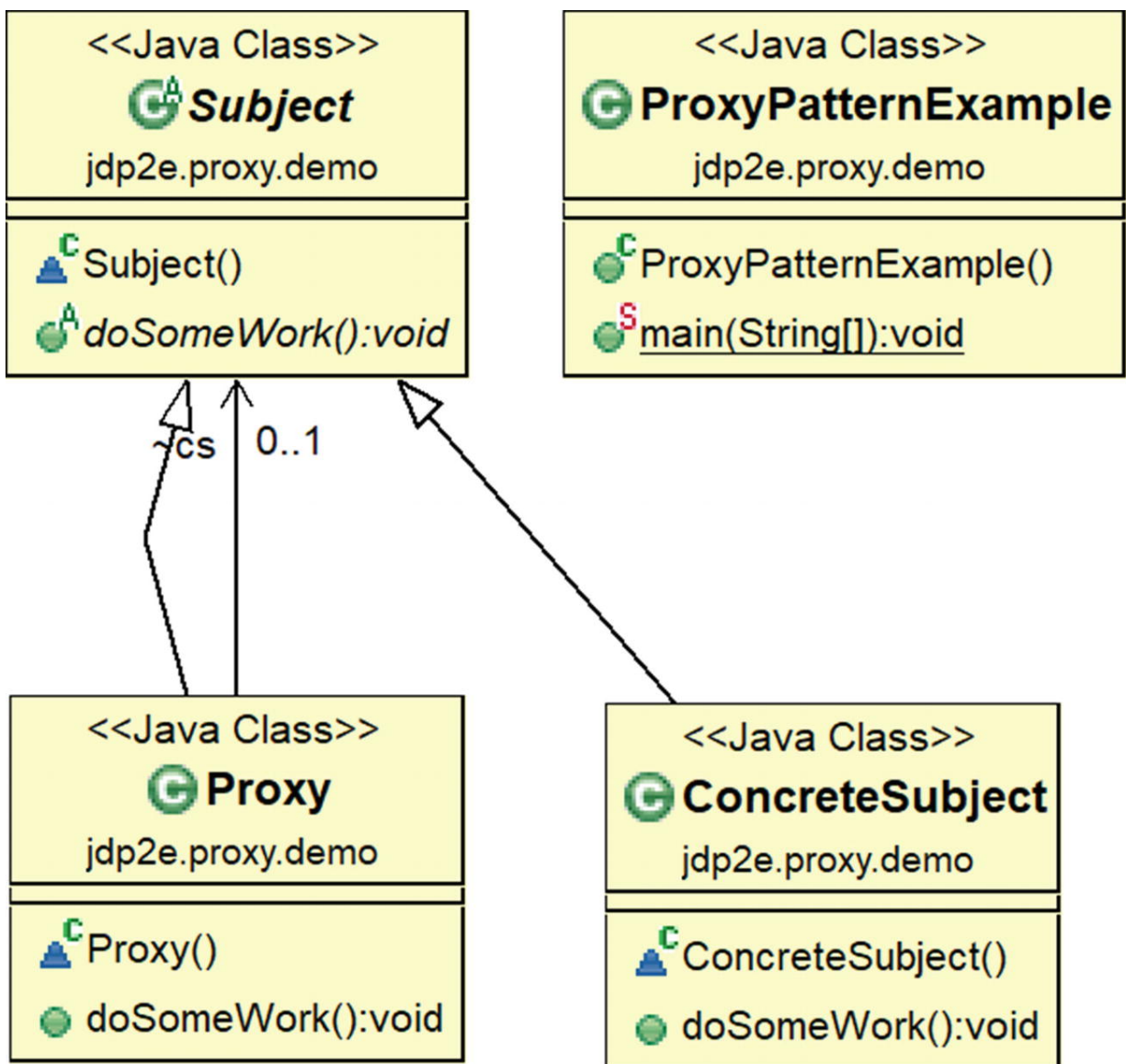
Figure 6-1 Class diagram
