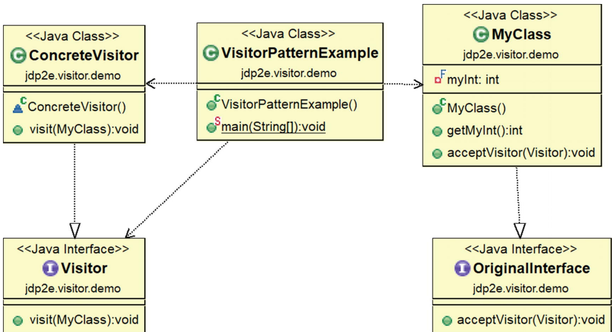
Figure 13-1 Class diagram
