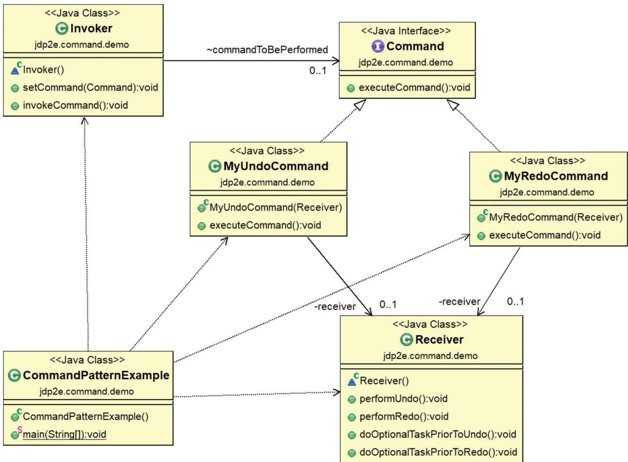
Figure 17-1 Class diagram
