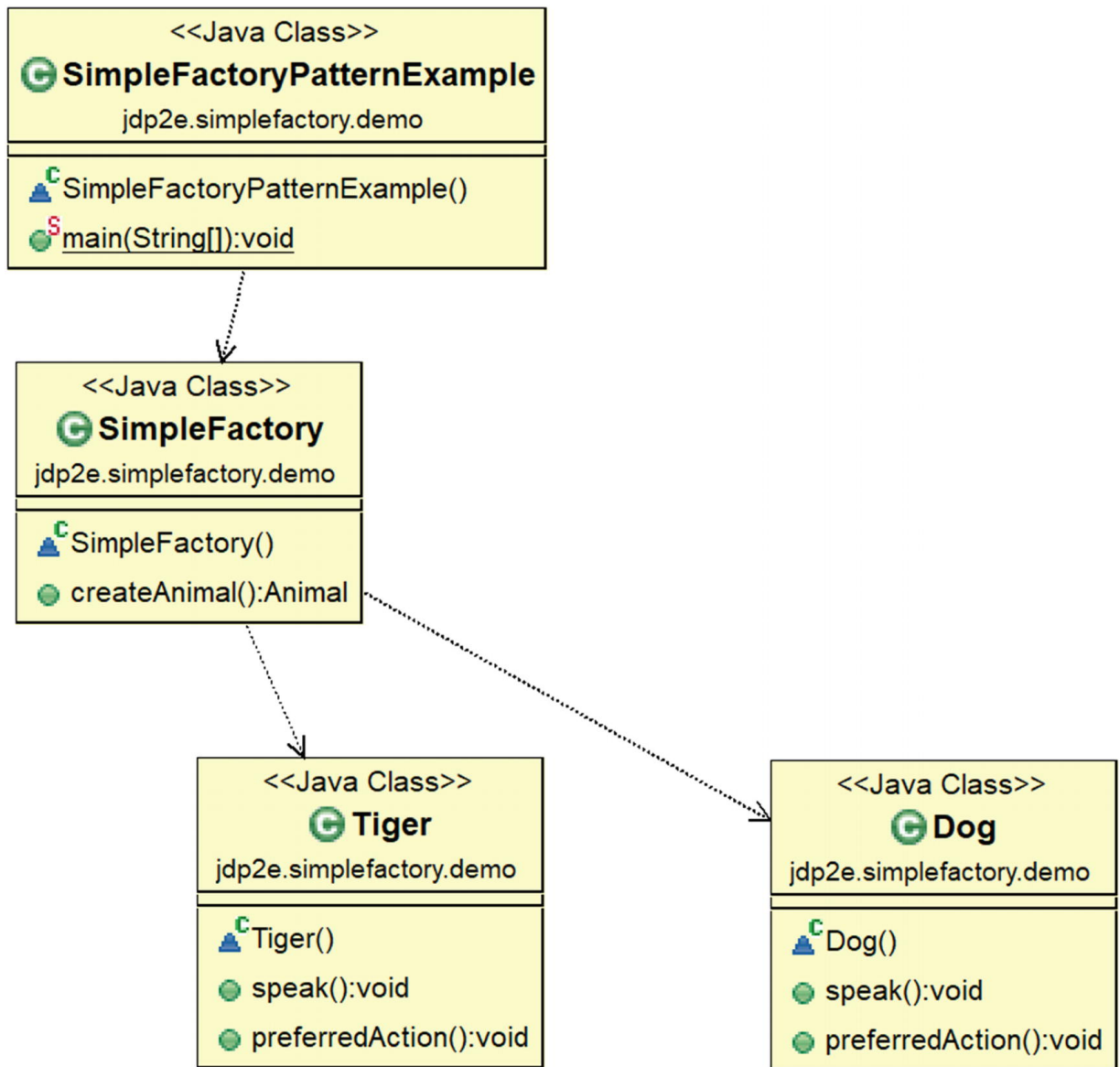
Figure 24-1 Class diagram
