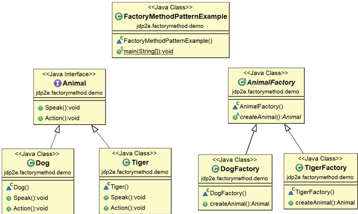
Figure 4-1 Class diagram
