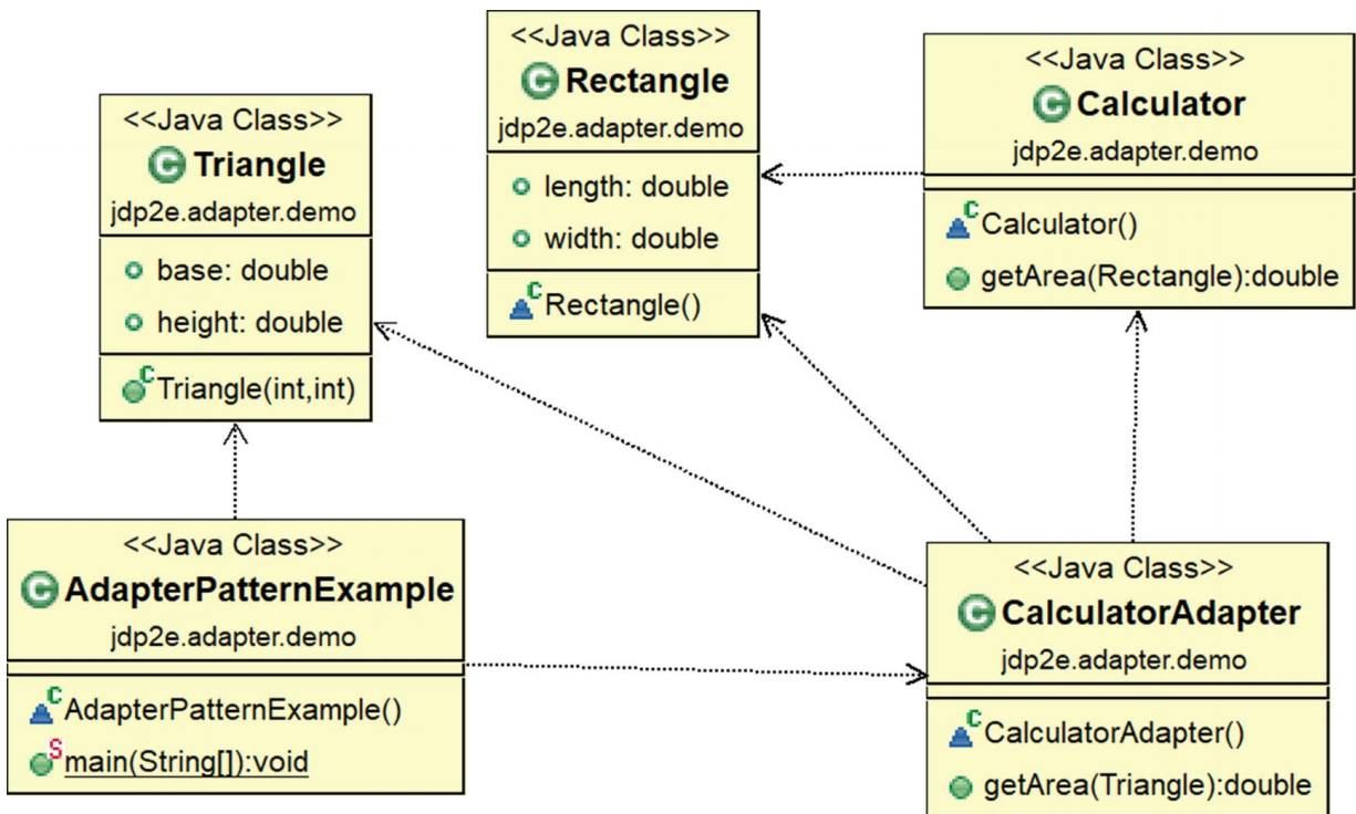
Figure 8-3 Class diagram
