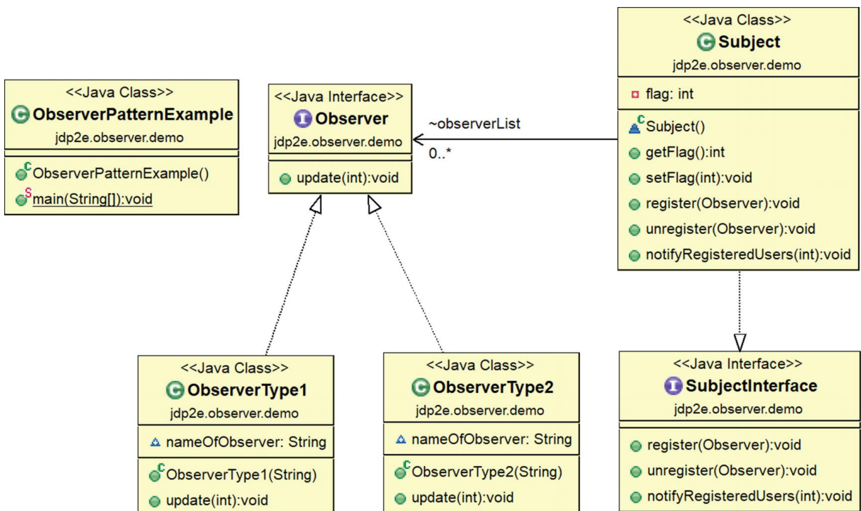
Figure 14-6 Class diagram
