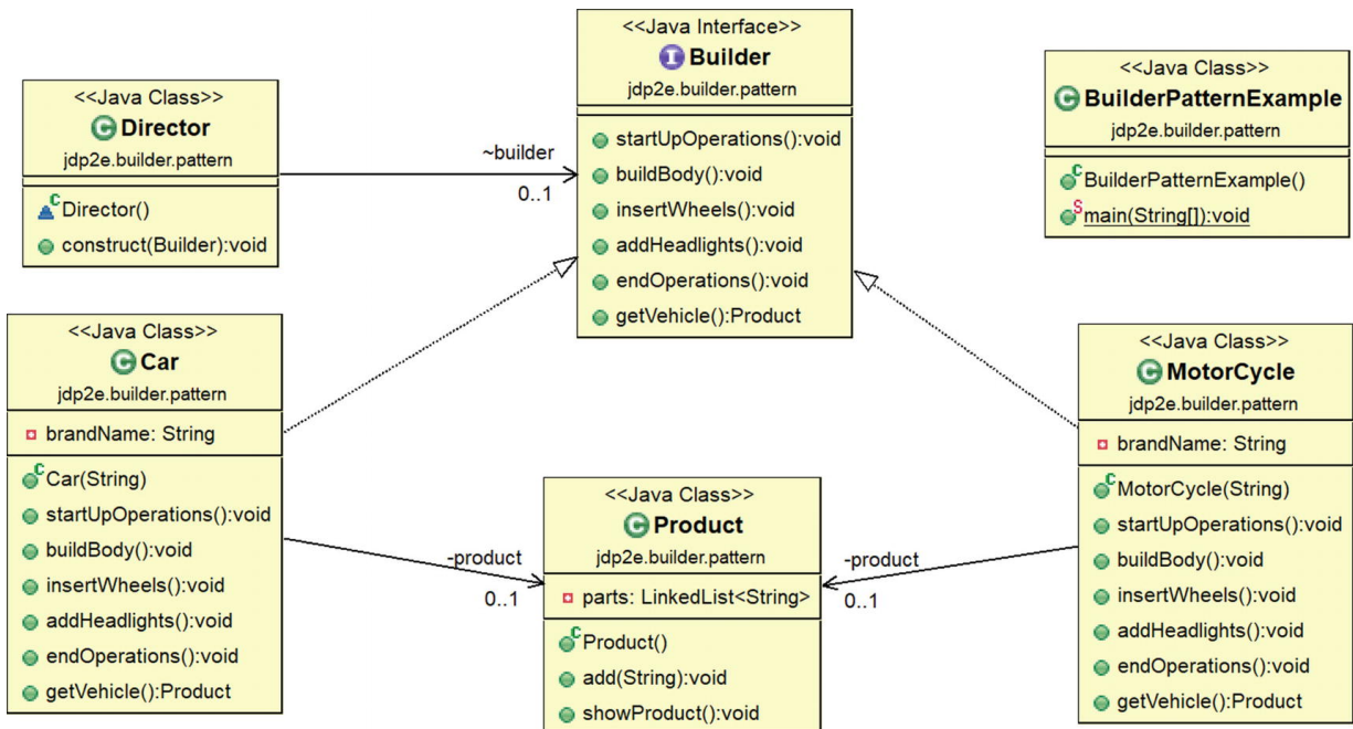
Figure 3-2 Class diagram
