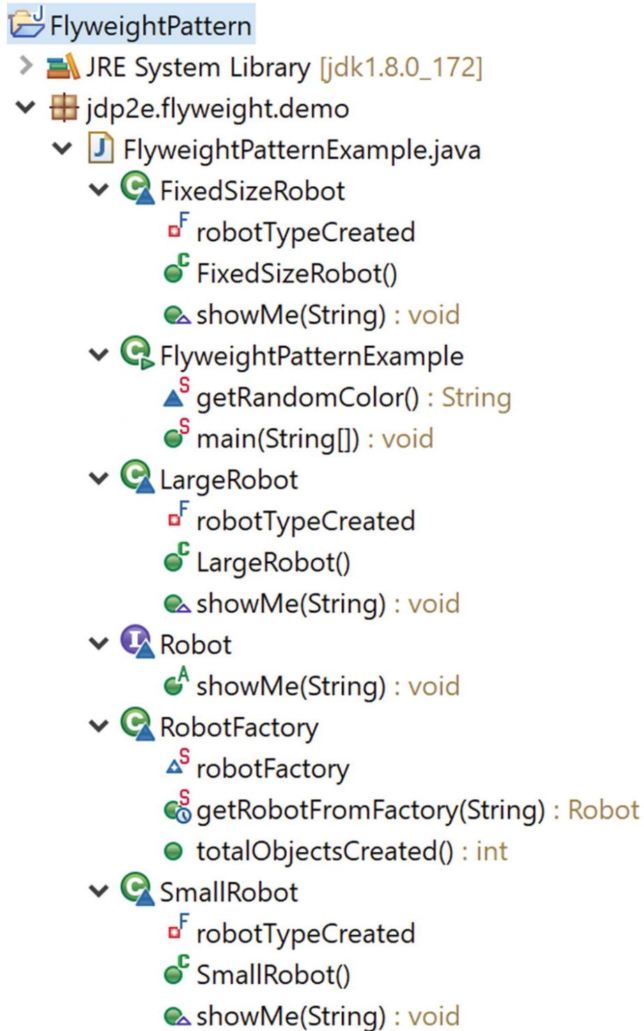
Figure 10-2 Package Explorer view
