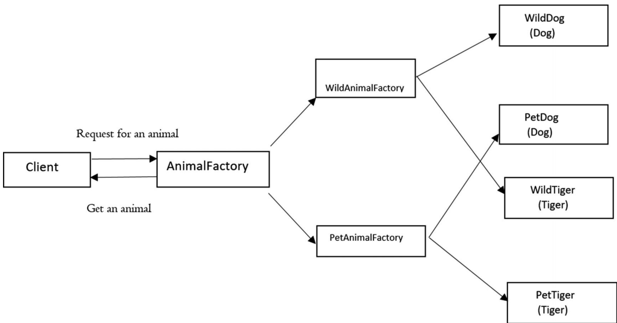
Figure 5-6 Abstract factory method pattern
