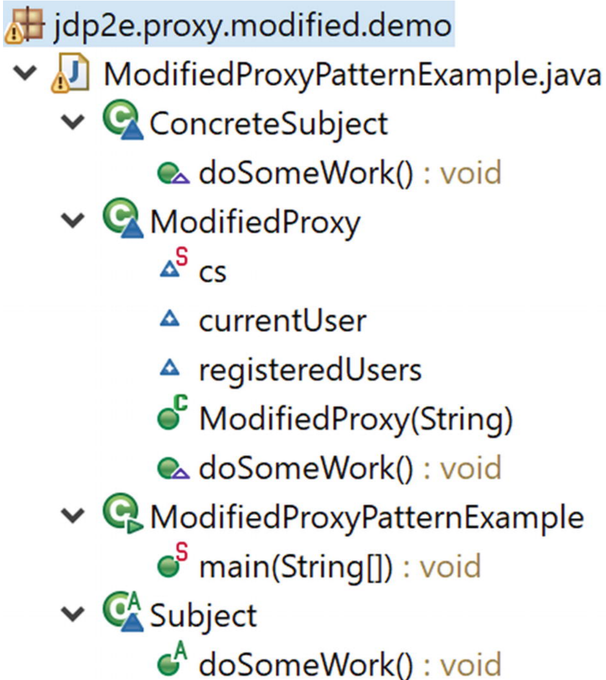
Figure 6-4 Modified Package Explorer view
