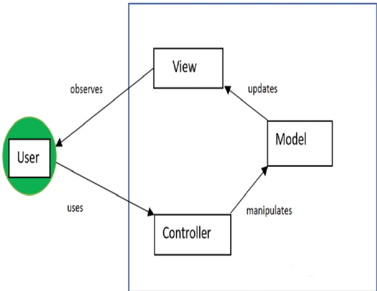
Figure 26-2 A typical MVC framework
