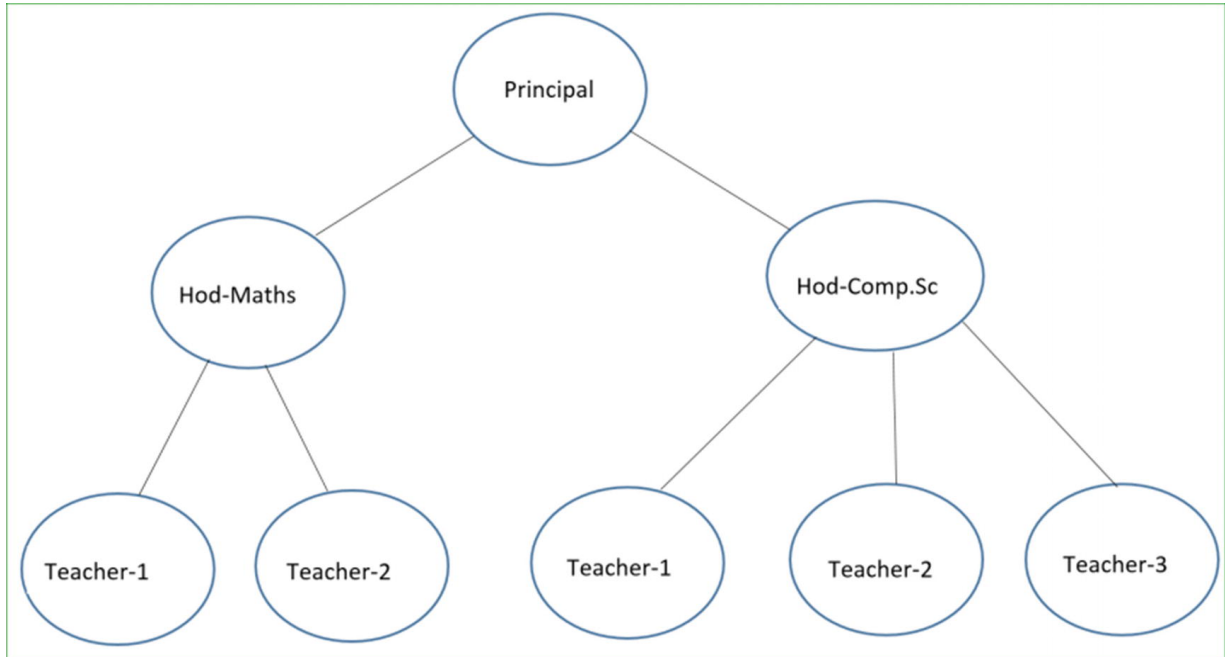
Figure 13-3 Tree structure of a composite design example
