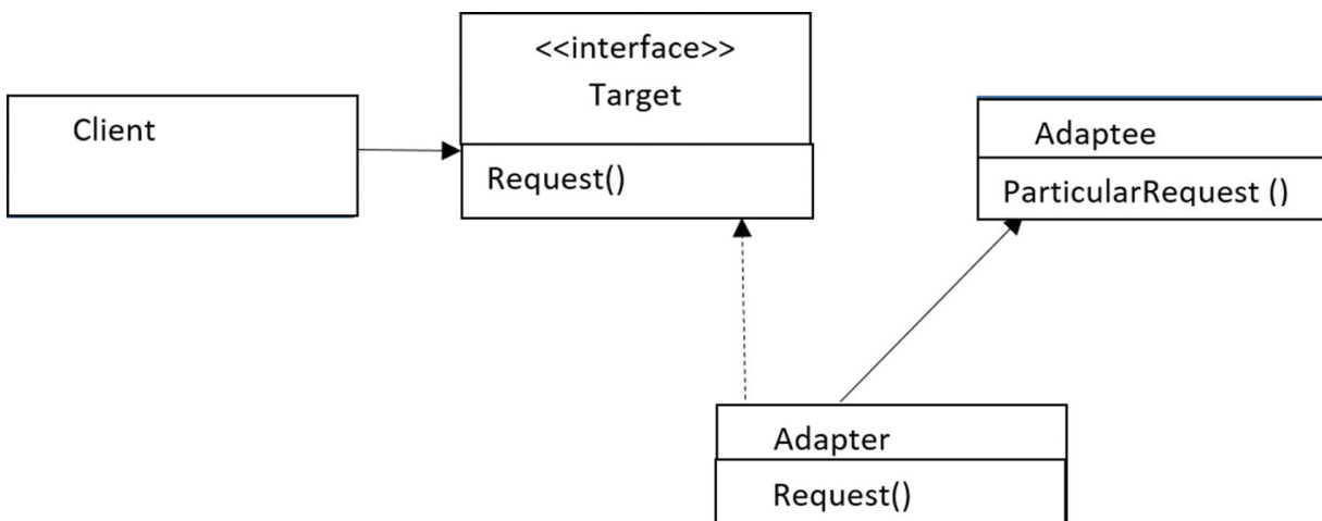
Figure 8-6 A typical object adapter
