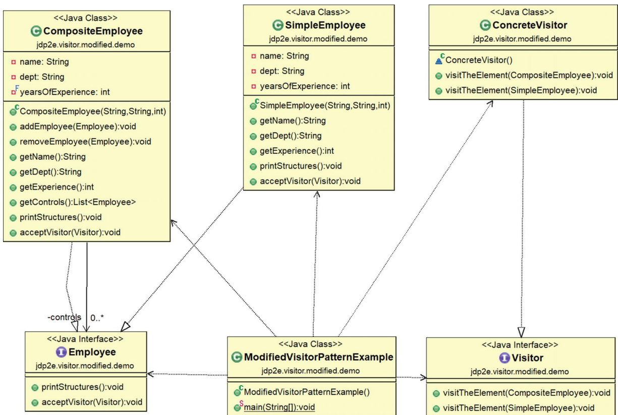
Figure 13-9 Modified class diagram
