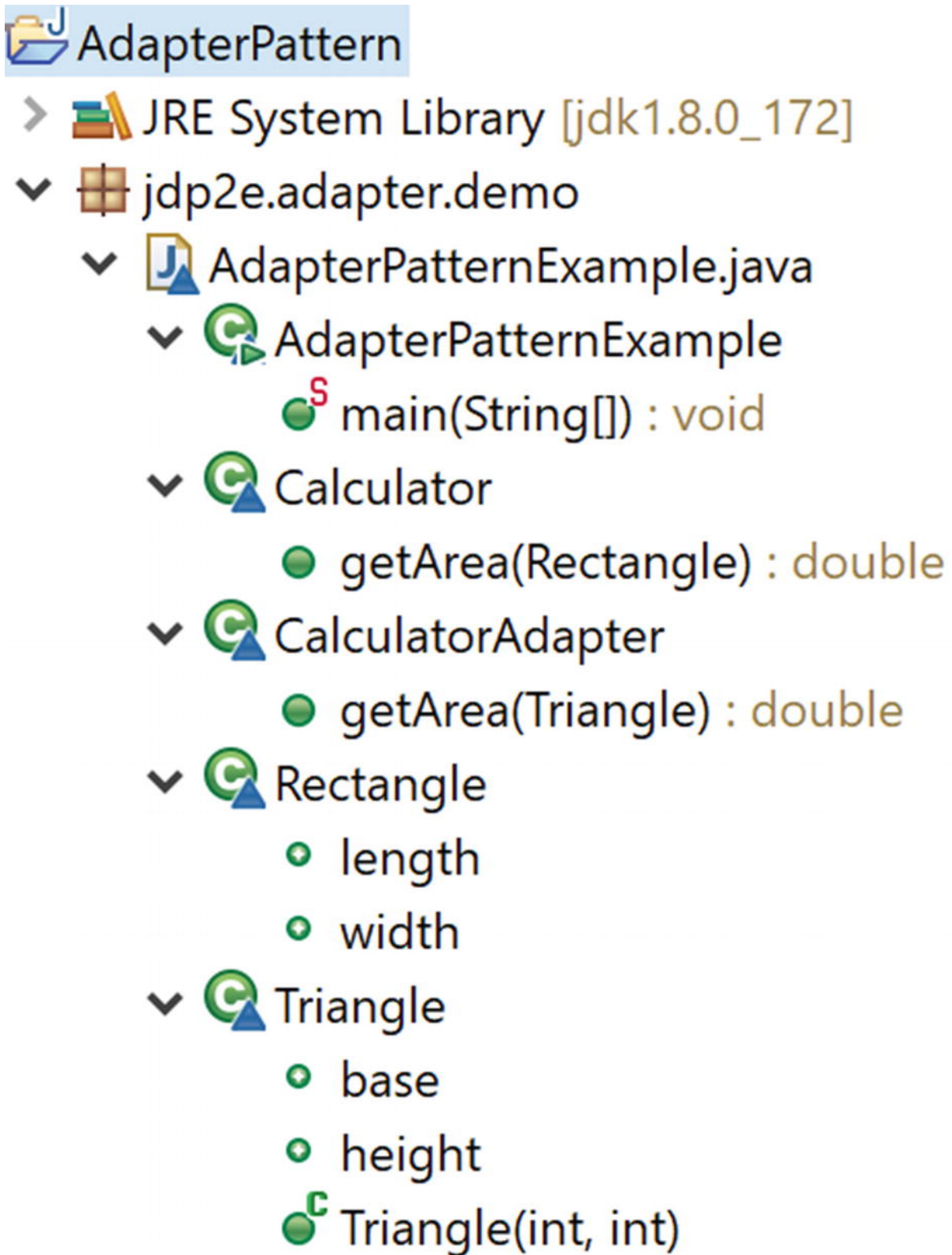
Figure 8-4 Package Explorer view
