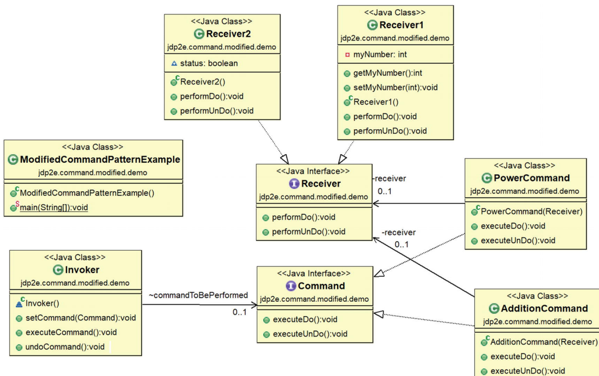
Figure 17-3 Modified class diagram
