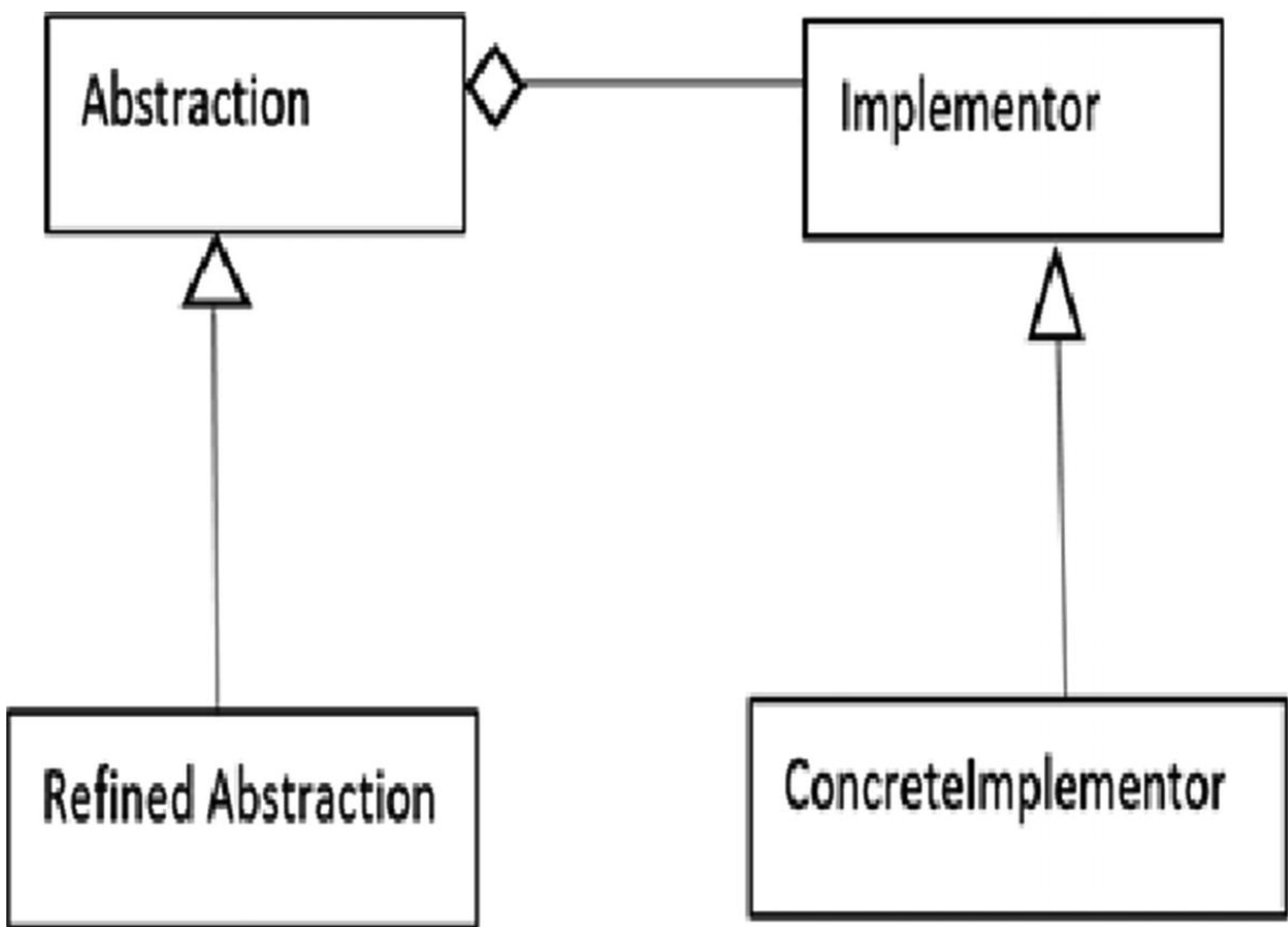
Figure 12-3 A classic bridge pattern
