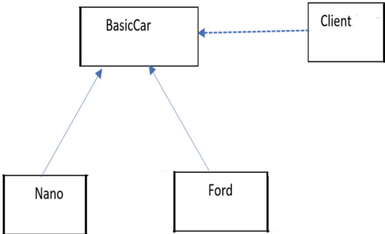
Figure 2-1 A sample prototype structure
