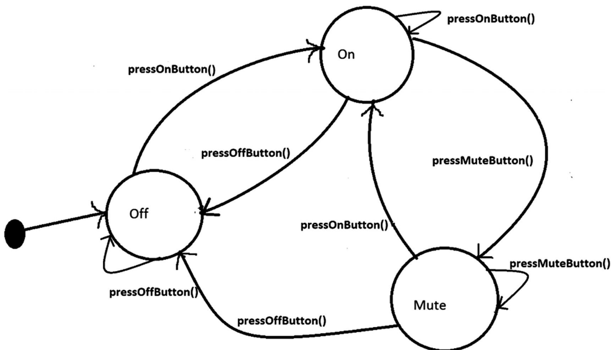
Figure 20-1 Different states of a TV
