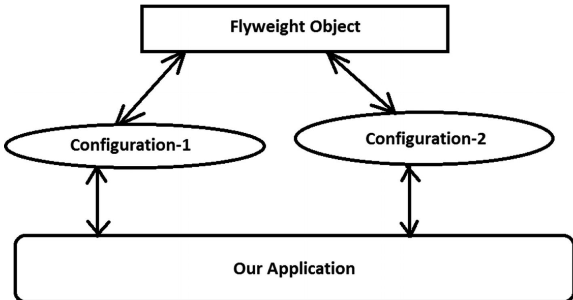
Figure 10-4 After using flyweights
