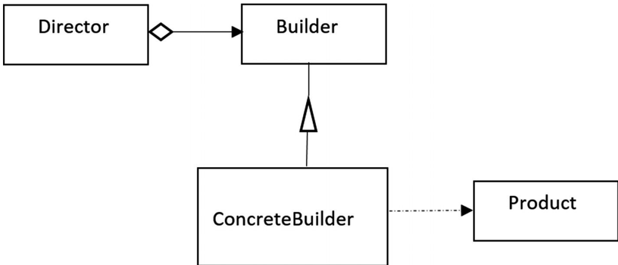
Figure 3-1 An example of the builder pattern
