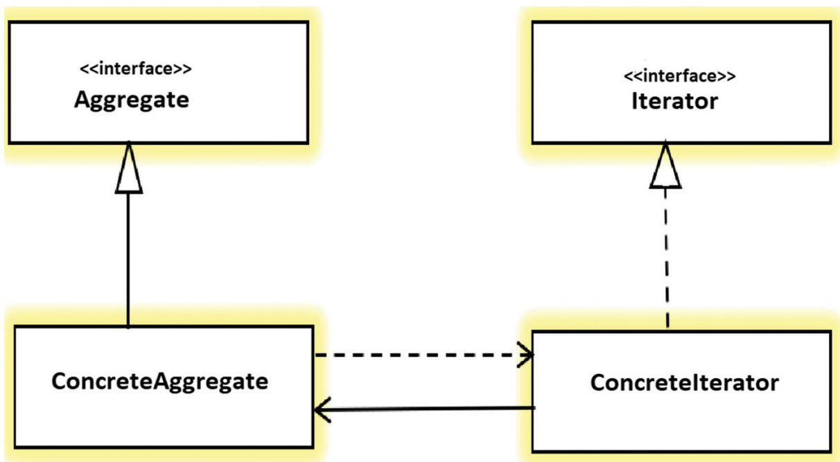
Figure 18-1 A sample diagram for an iterator pattern
