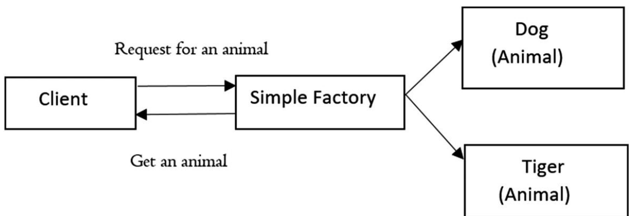
Figure 5-4 Simple factory pattern
