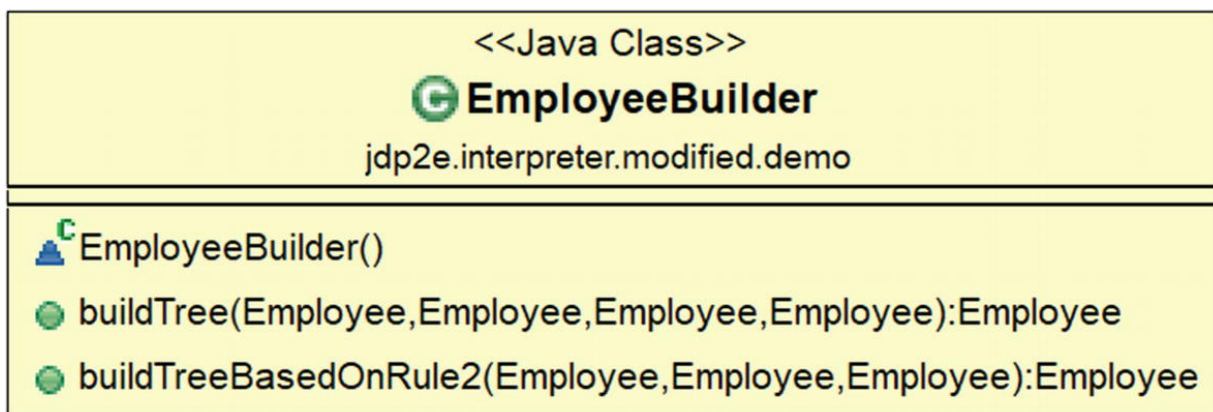
Figure 23-4 Modified Class diagram for EmployeeBuilder class
