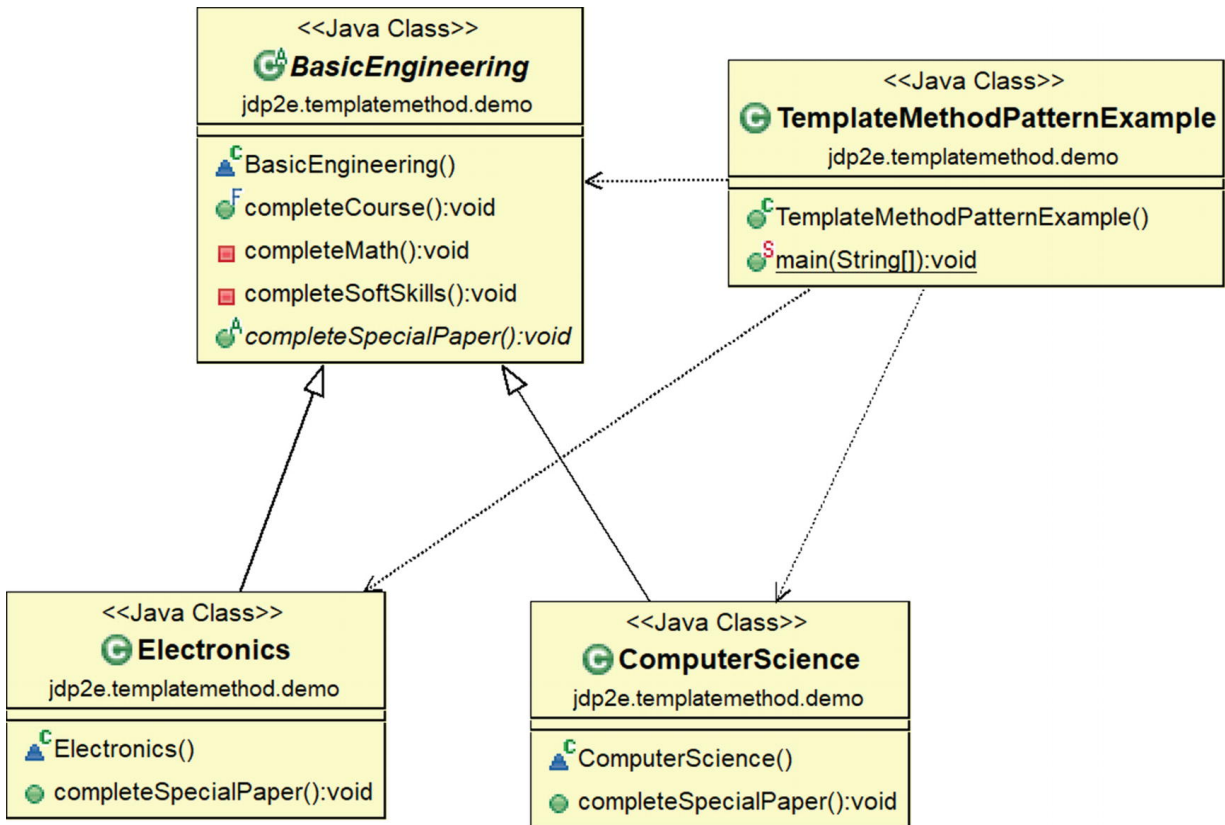
Figure 16-1 Class diagram
