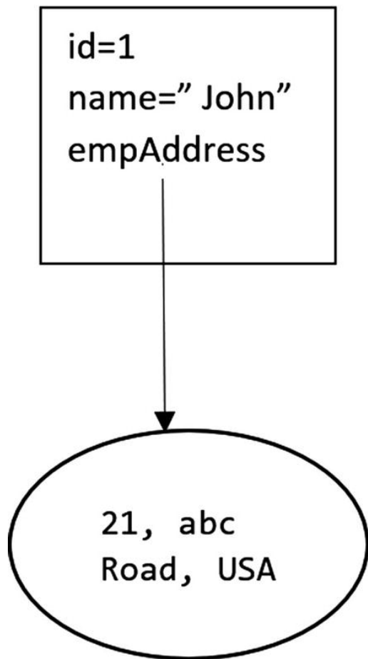
Figure 19-4 Deep copy
