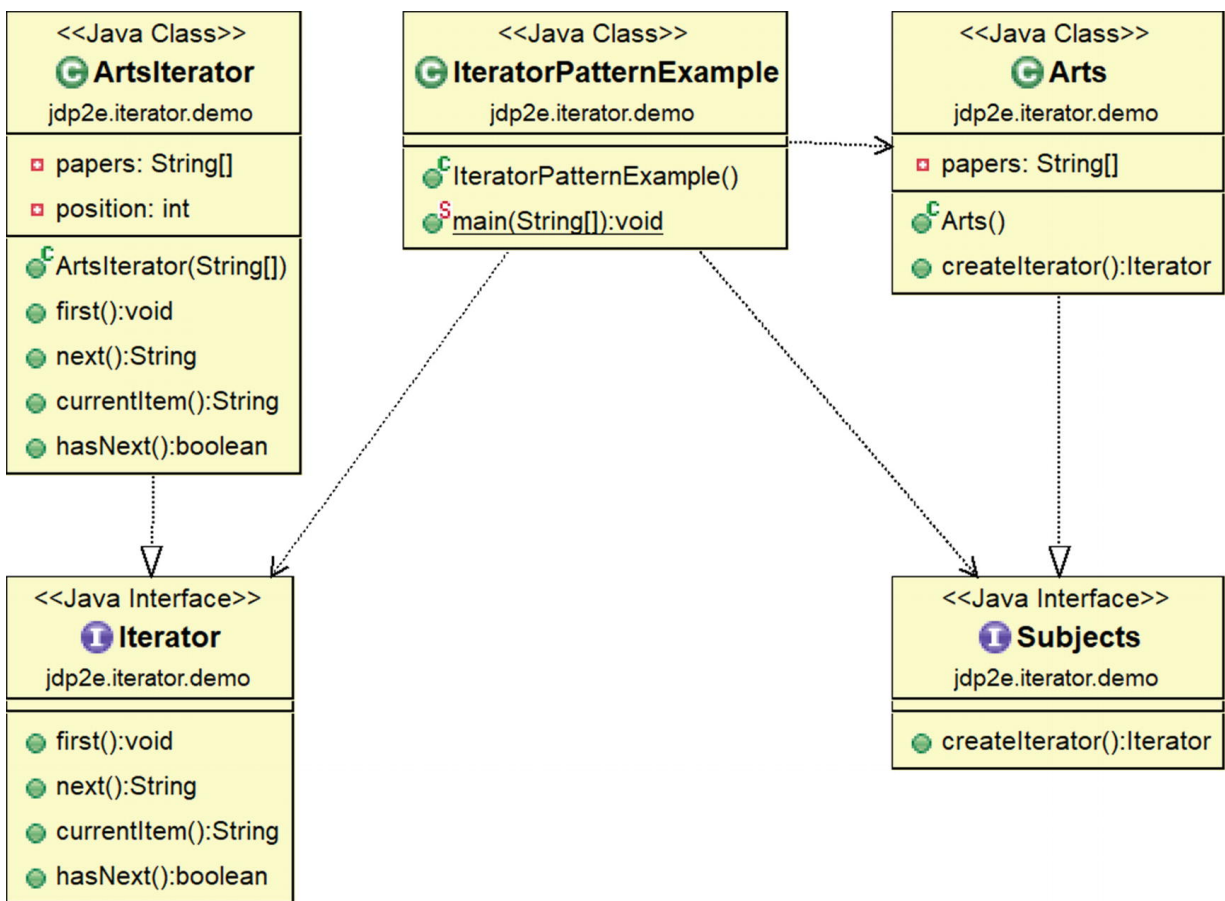
Figure 18-2 Class diagram
