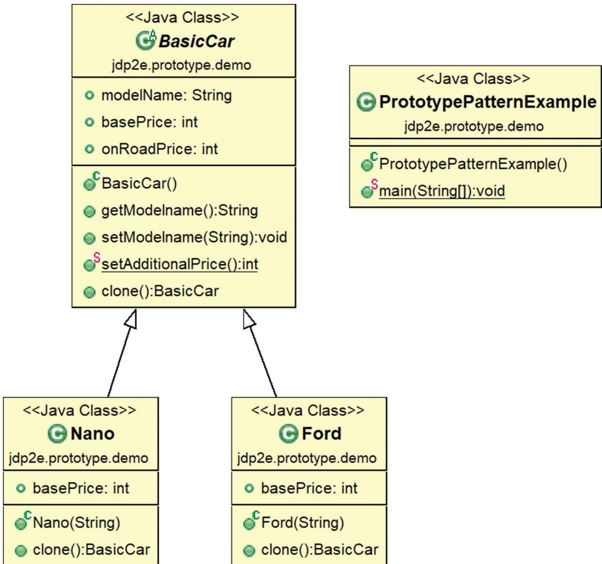
Figure 2-2 Class diagram
