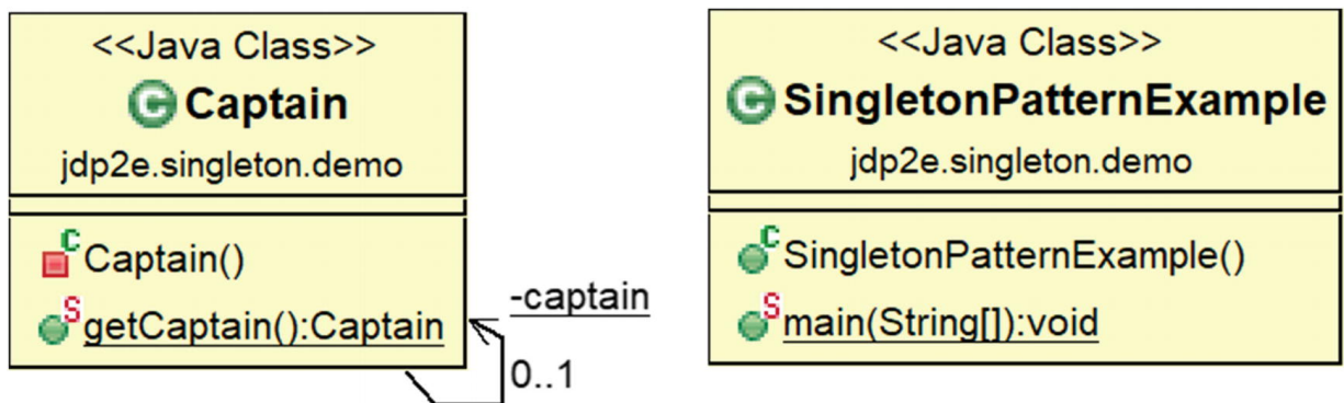
Figure 1-1 Class diagram
