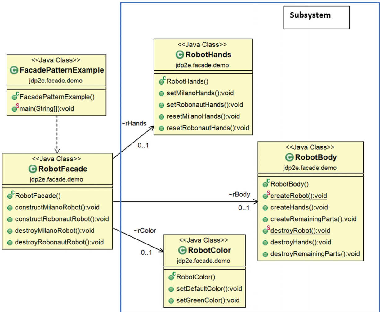
Figure 9-1 Class diagram
