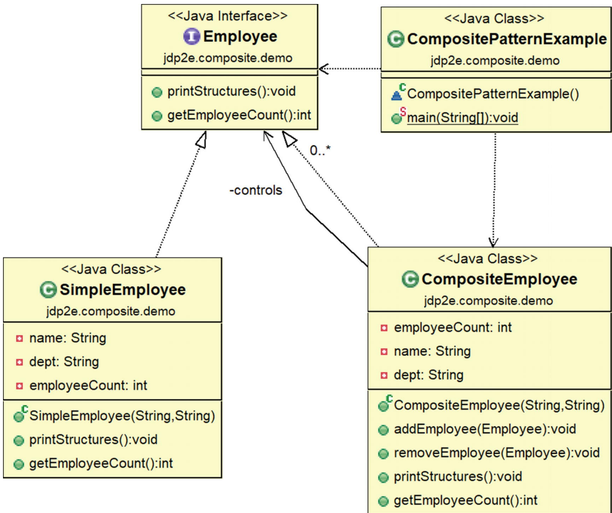
Figure 11-2 Class diagram
