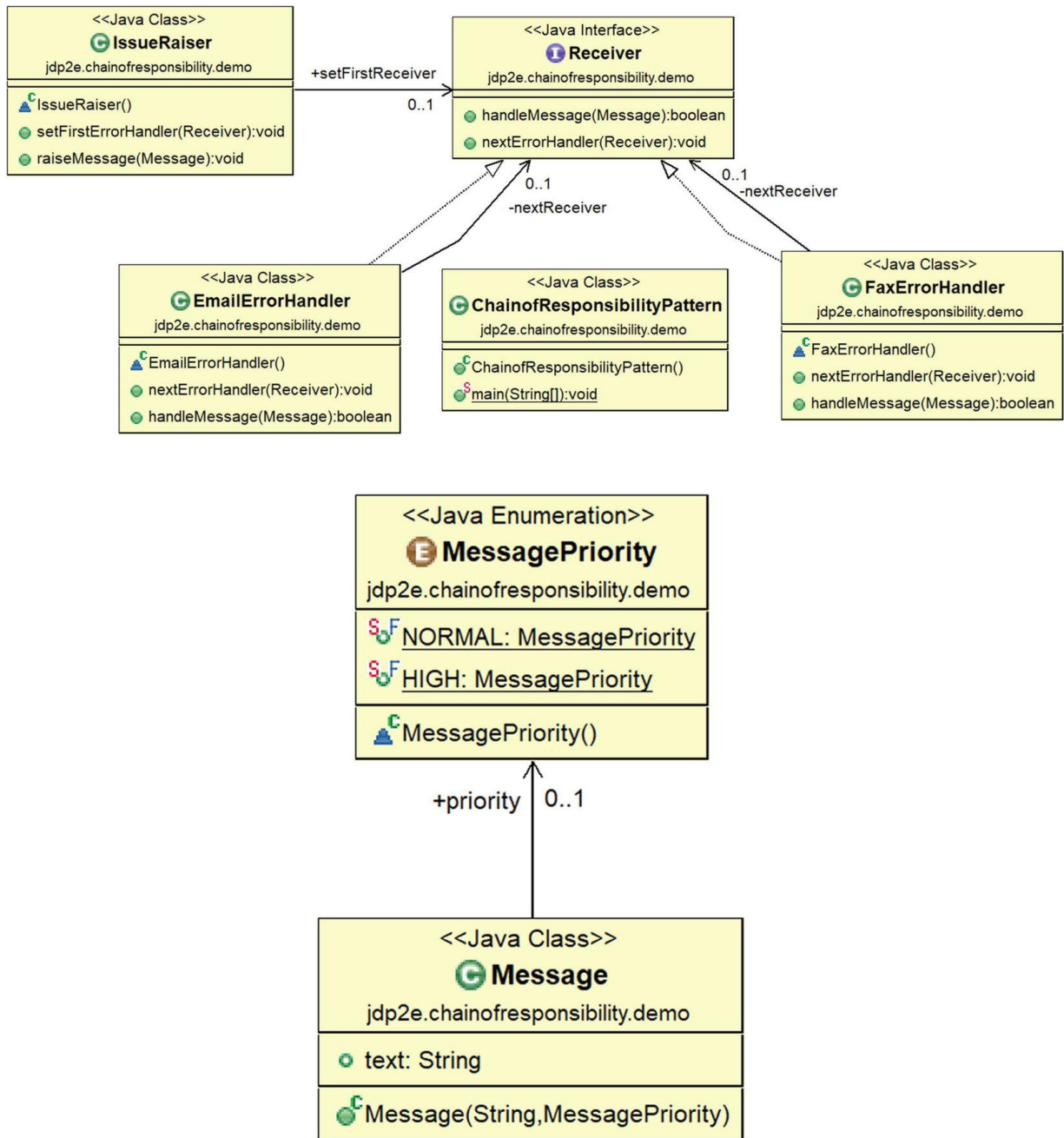
Figure 22-2 Class diagram
