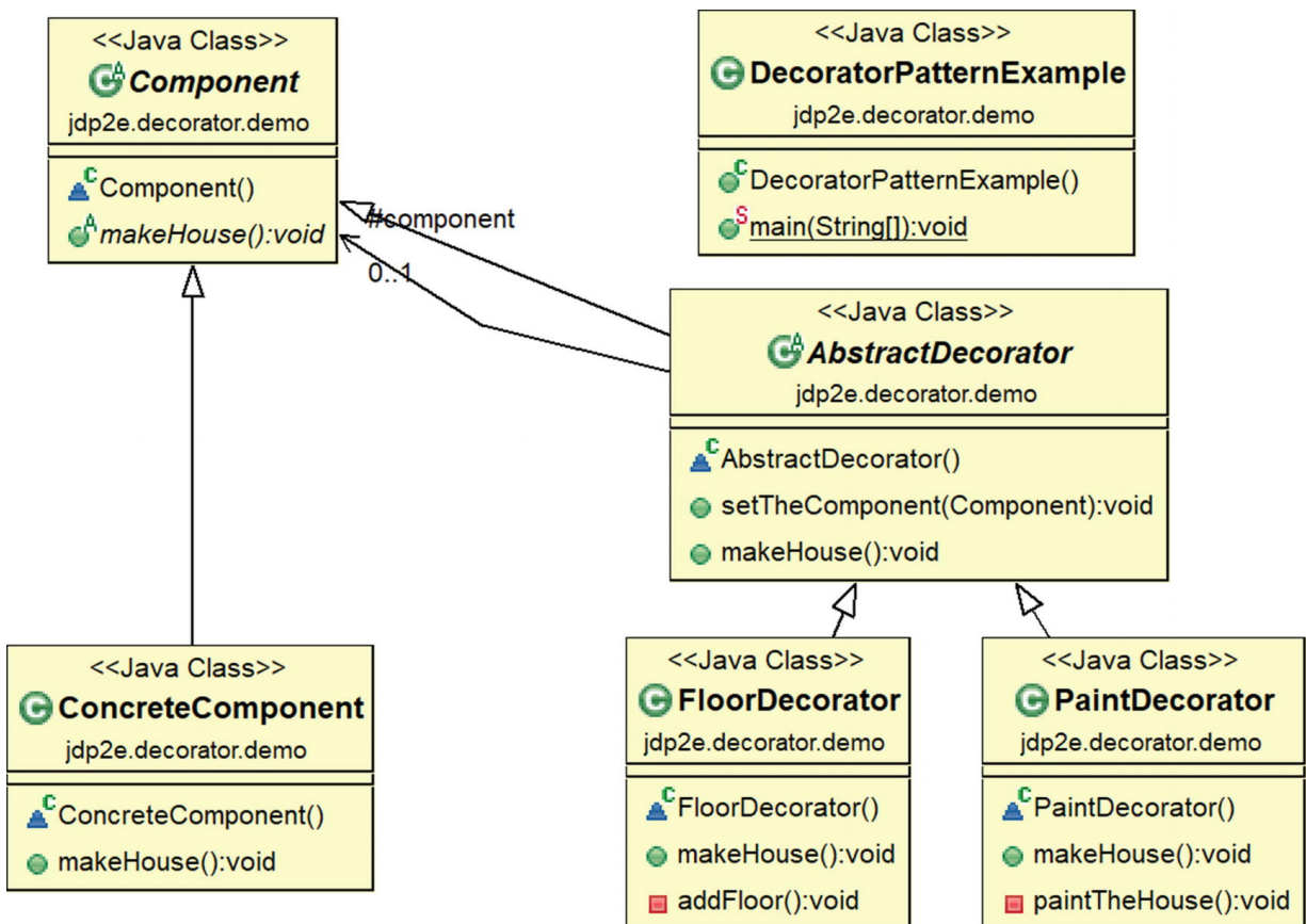
Figure 7-4 Class diagram
