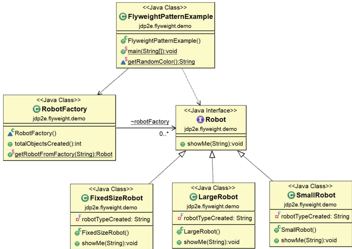
Figure 10-1 Class diagram
