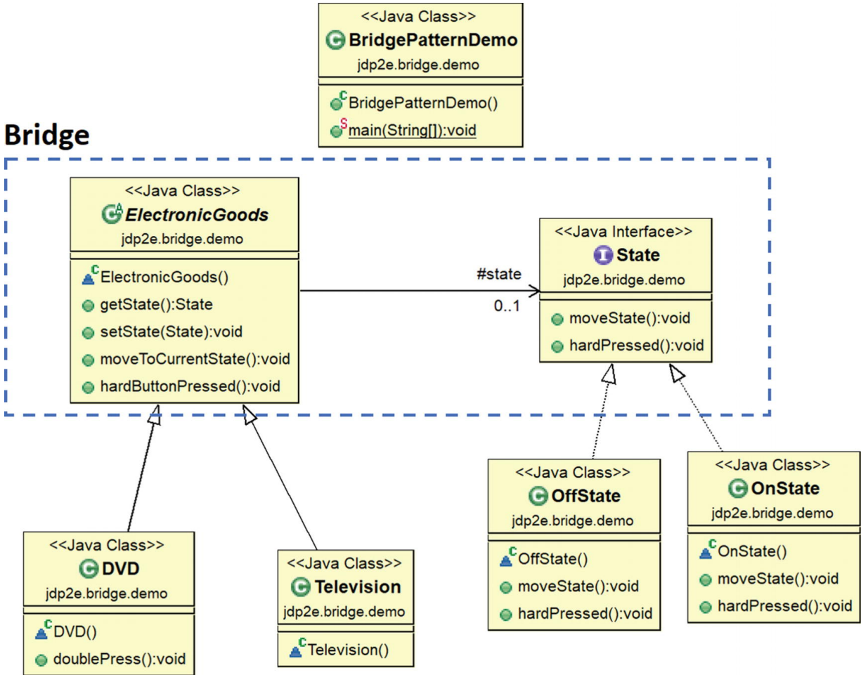
Figure 12-4 Class diagram
