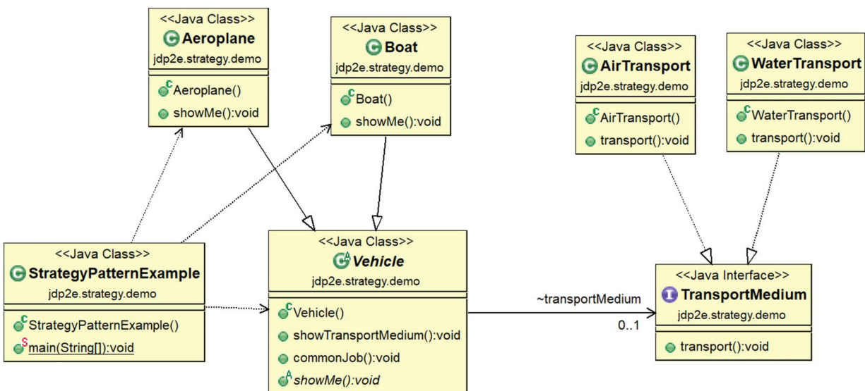
Figure 15-1 Class diagram
