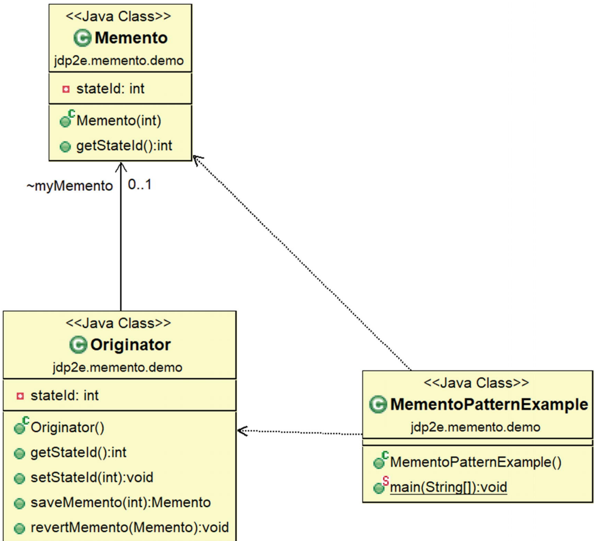
Figure 19-1 Class diagram
