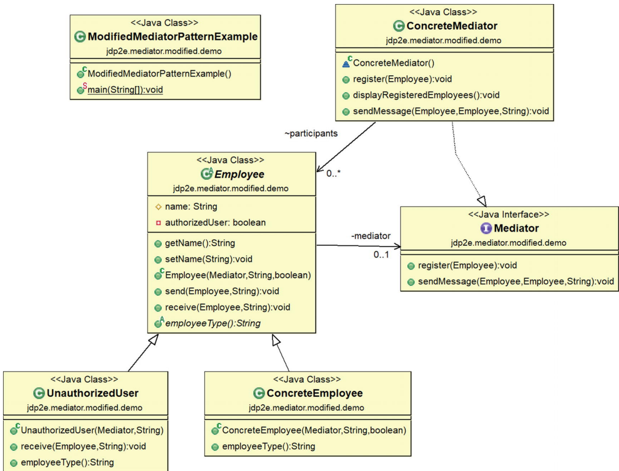
Figure 21-4 Class diagram
