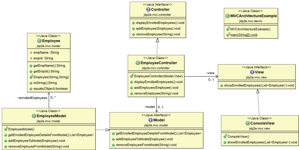
Figure 26-6 Class diagram
