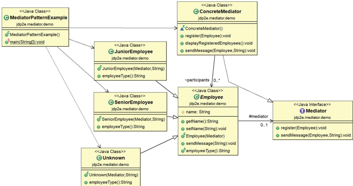
Figure 21-2 Class diagram
