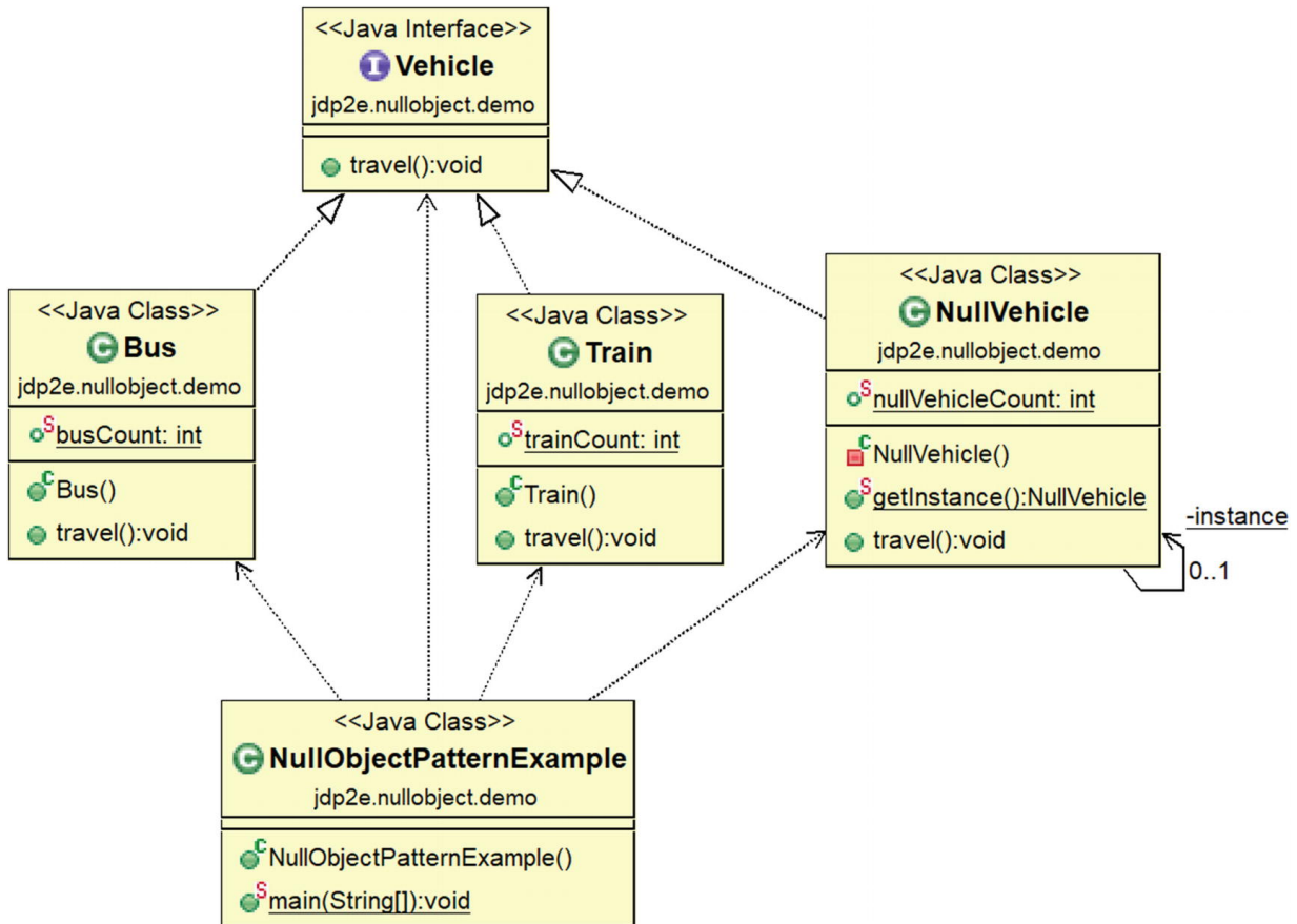
Figure 25-1 Class diagram
