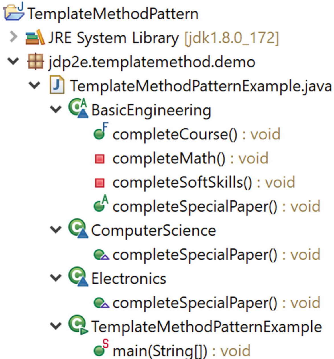
Figure 16-2 Package Explorer View
