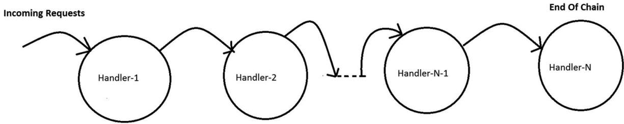
Figure 22-1 The concept of a chain-of-responsibility pattern
