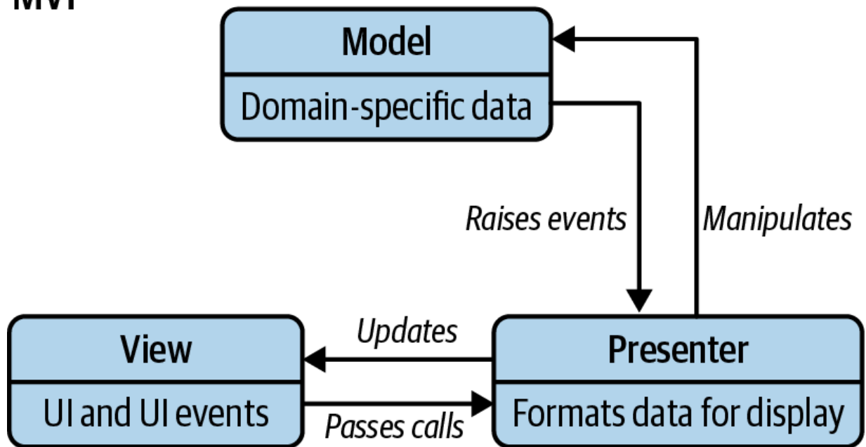
Figure 8-2. MVP pattern
