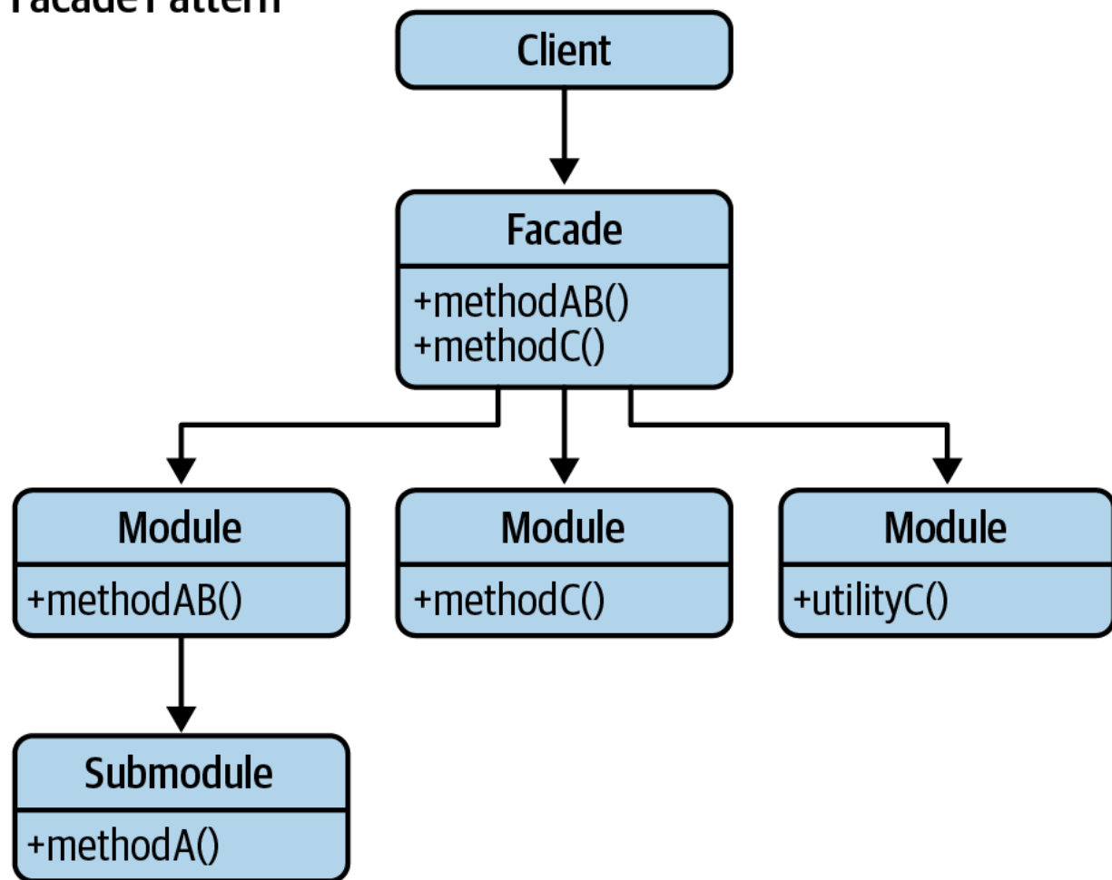
Figure 7-5. Facade pattern
