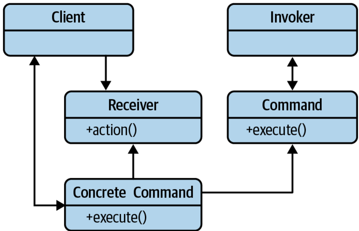
Figure 7-12. Command pattern
