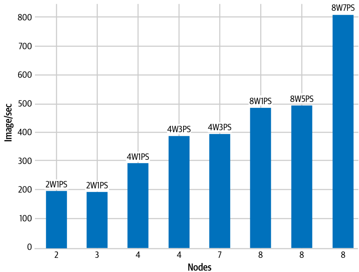
Figure 4-17. Comparison of throughput between different distribution setups. Here, 2W1PS indicates two workers and one parameter server.
