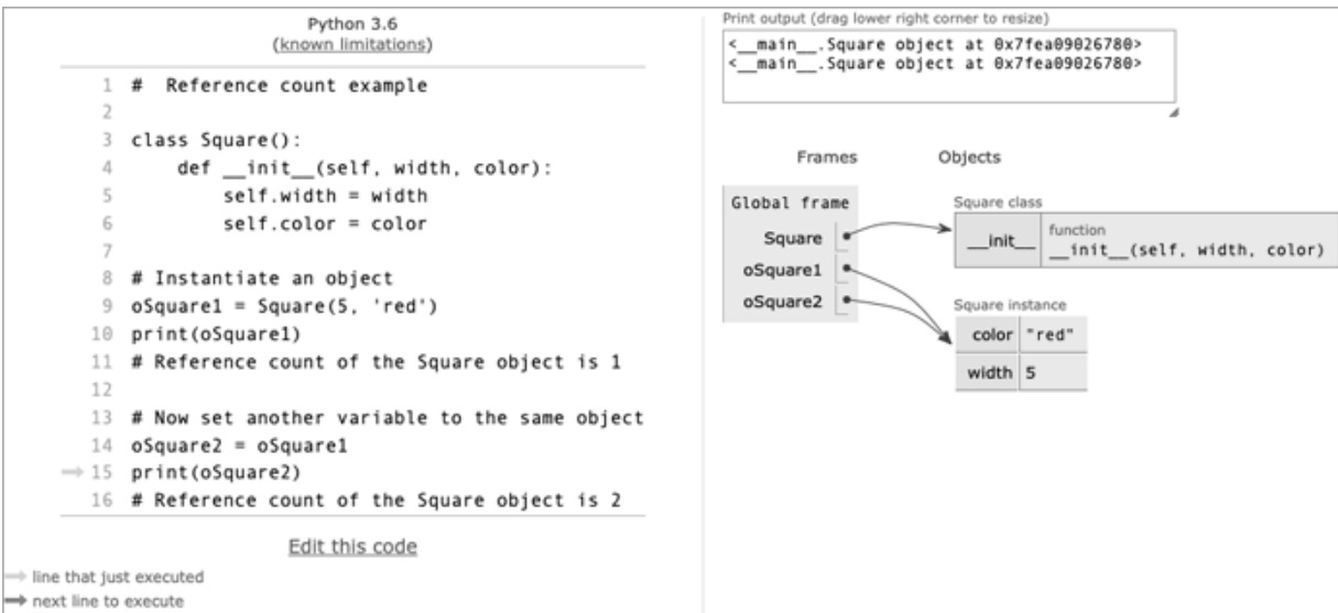
Figure 11-2: Two variables referring to the same object
