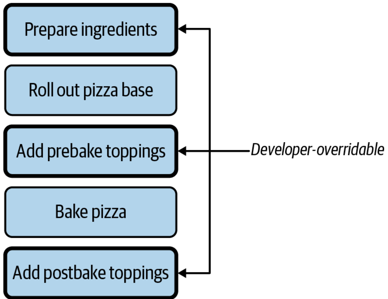
Figure 19-2. Pizza-making algorithm
