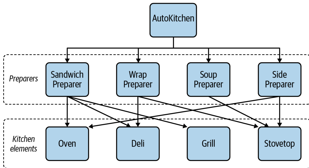
Figure 17-2. AutoKitchen design
