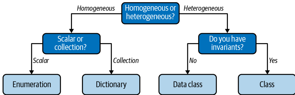
Figure 10-1. Picking the appropriate abstraction
