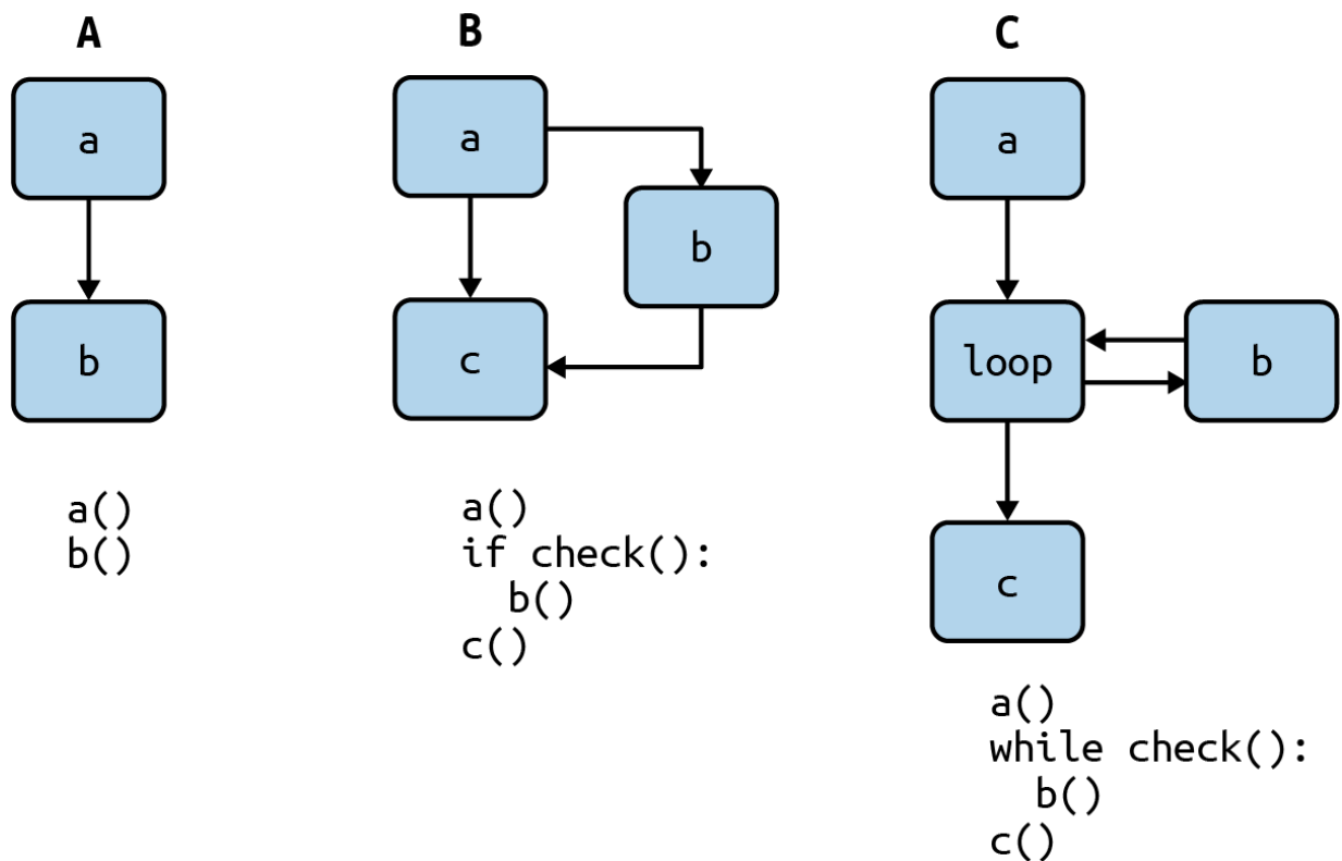
Figure 20-1. Cyclomatic complexity examples
