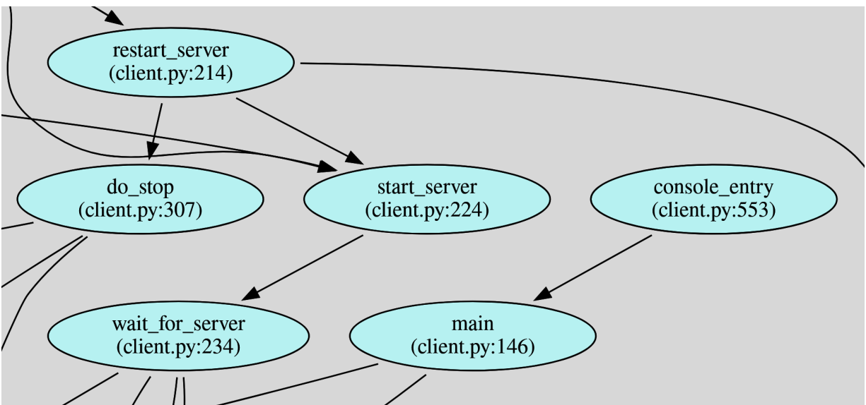
Figure 16-7. Visualizing function calls statically
