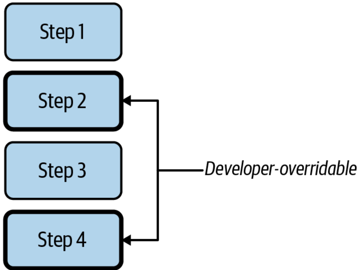
Figure 19-1. The Template Method Pattern
