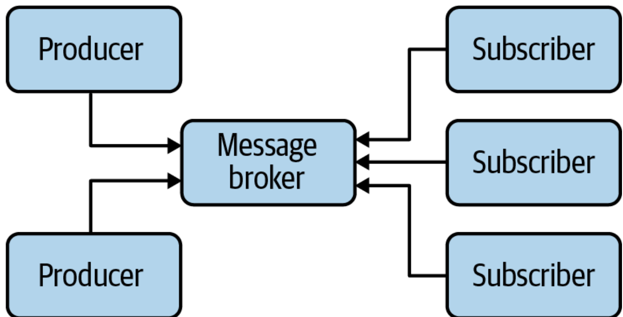
Figure 18-2. A hypothetical message broker–based architecture
