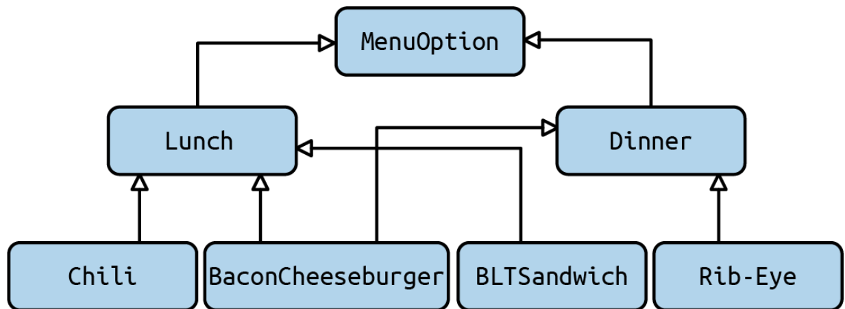
Figure 13-2. A more complicated type hierarchy
