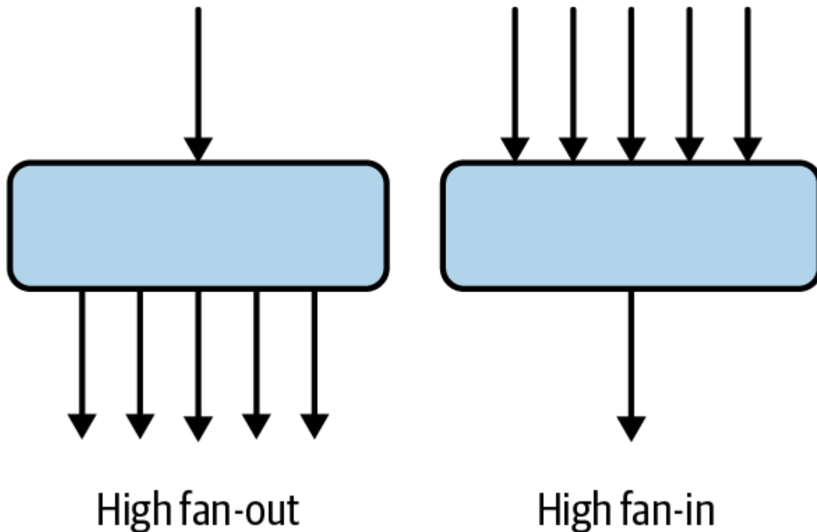
Figure 16-9. The difference between fan-in and fan-out
