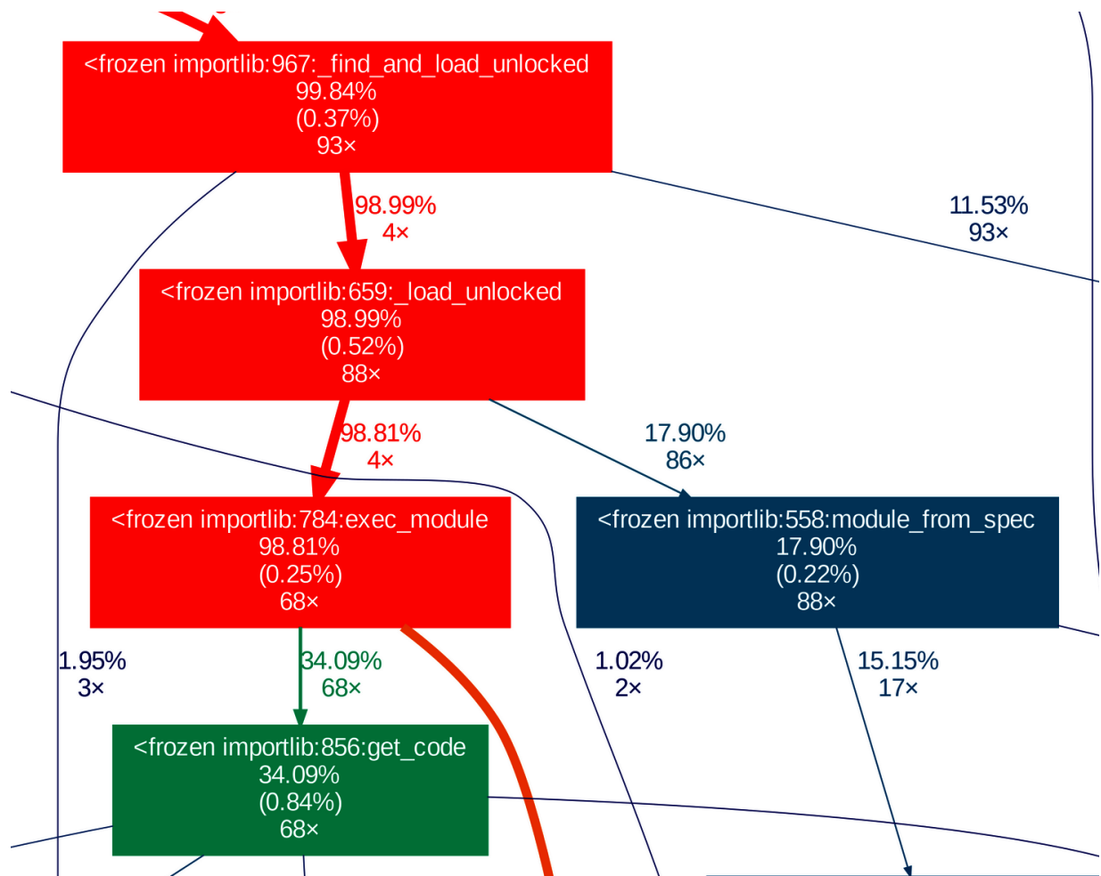
Figure 16-8. Visualizing function calls dynamically
