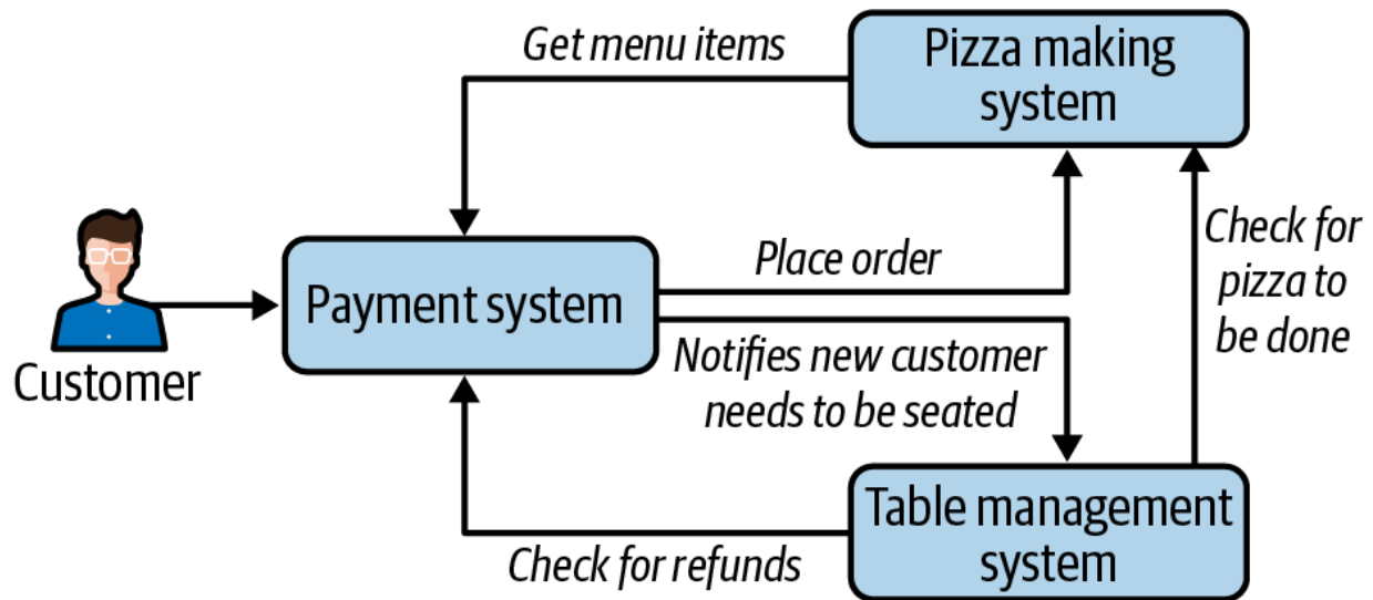
Figure 16-4. More sensible dependencies
