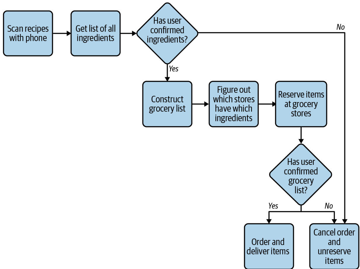
Figure 11-1. Workflow for automated grocery delivery app
