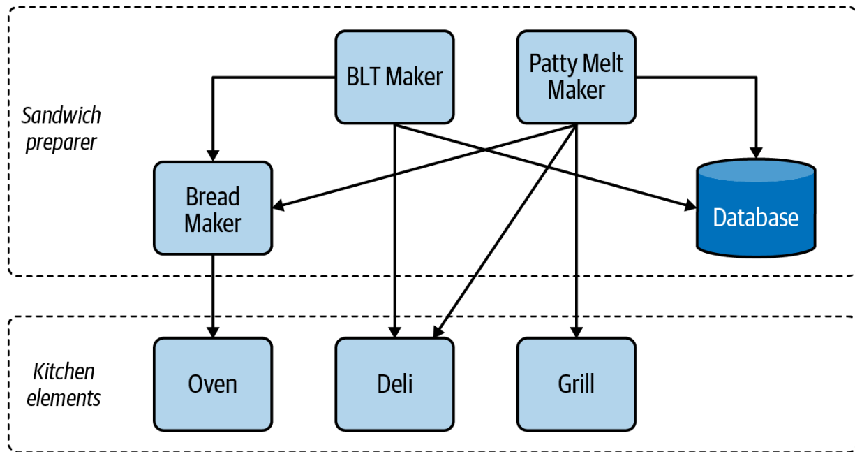
Figure 17-3. Sandwich Preparer
