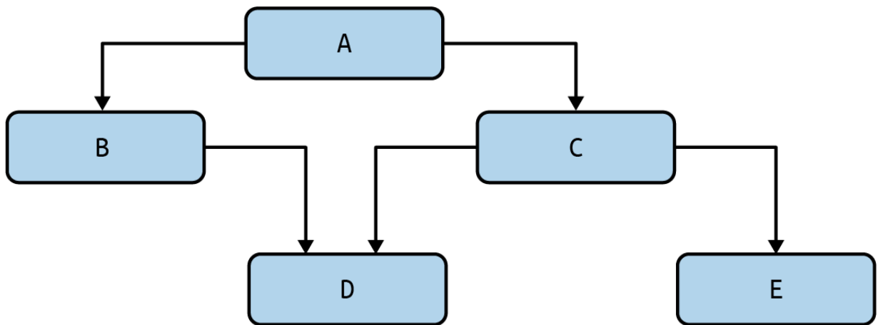
Figure 16-1. Box-and-arrows diagram
