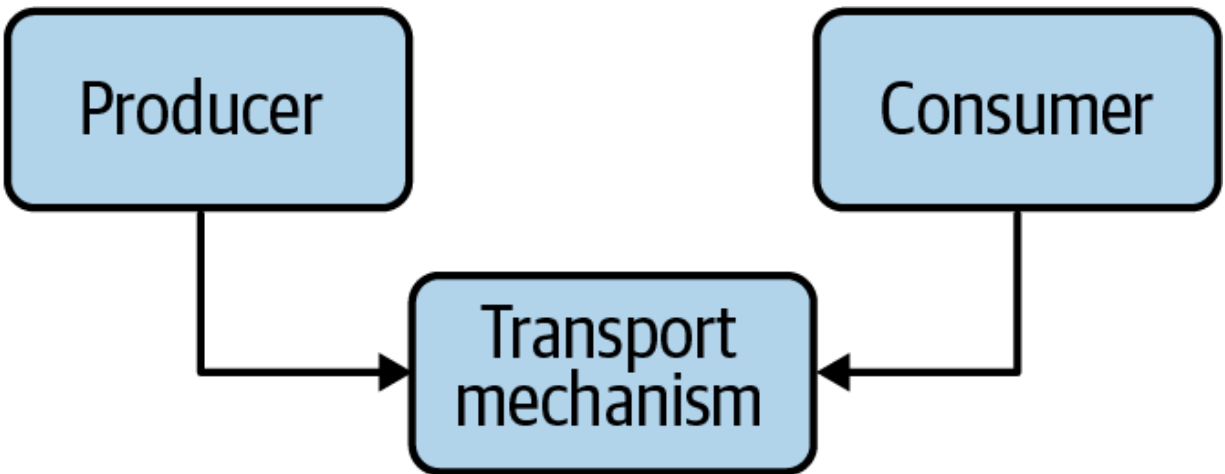
Figure 18-1. Producer–consumer relationship
