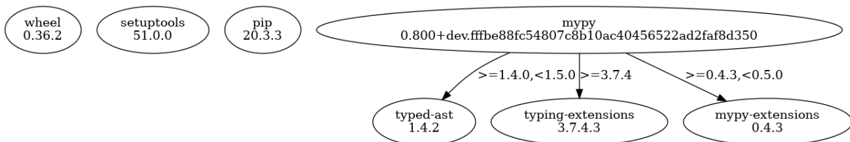
Figure 16-5. Visualizing packages
