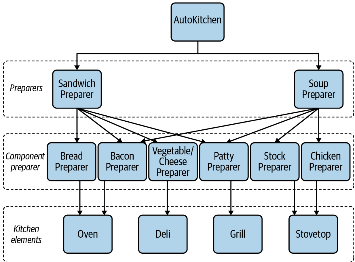
Figure 17-4. Composable architecture
