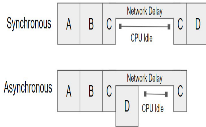
Figure 2.1: Sync versus async timing diagram
