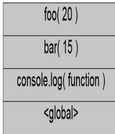
Figure 2.3: Call stack
