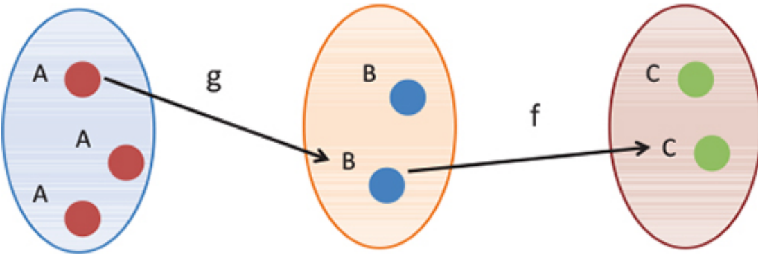
Figure 4.11. The composition of two functions is a new function directly mapping the inputs of the first function to the output of the second. The composition is also a referentially transparent mapping between inputs and outputs.
