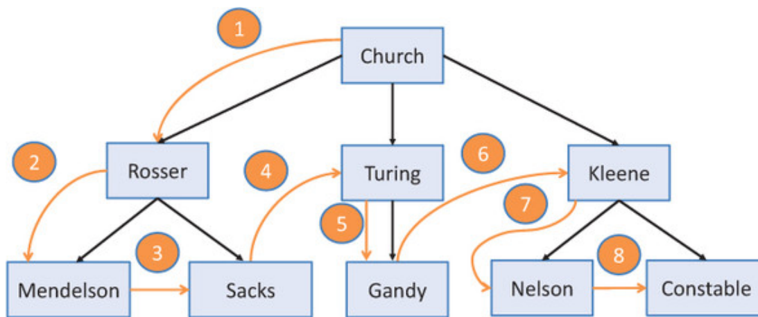
Figure 3.9. Recursive preorder traversal, starting with the root and descending all the way to the left before going to the right
