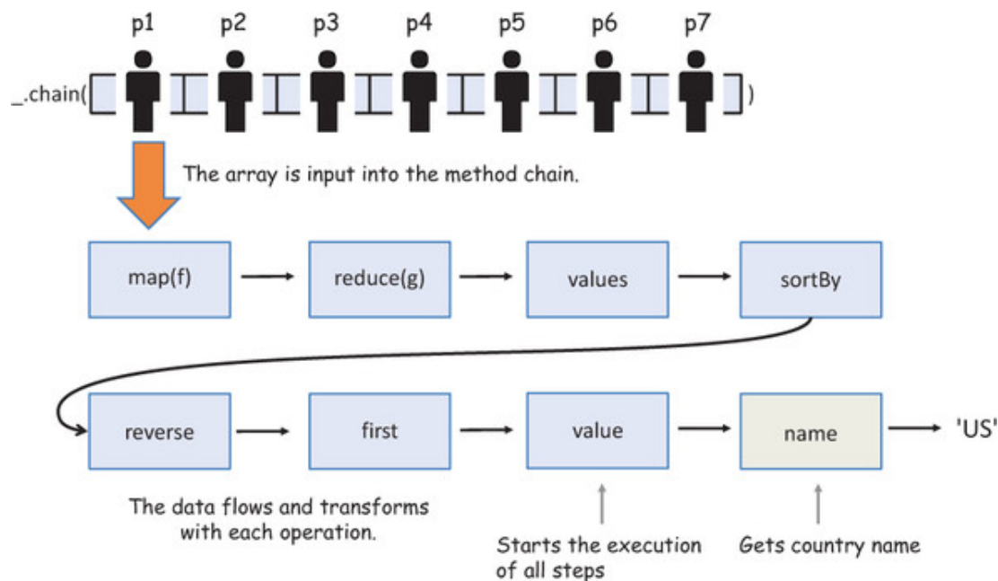
Figure 3.7. Control of a program built using Lodash function chains. The array of person objects is processed through a series of operations. Along the way, the data flows and is finally transformed into a single value.
