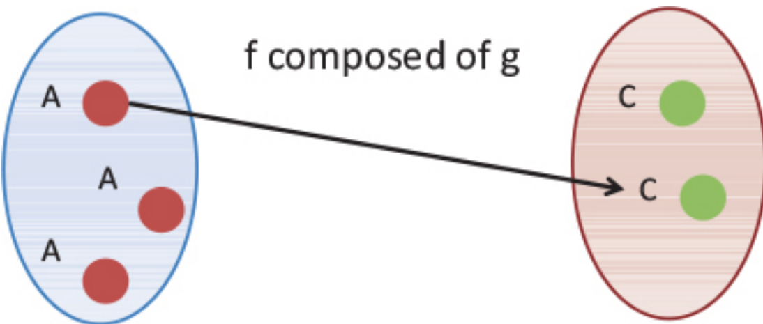
Figure 4.11. The composition of two functions is a new function directly mapping the inputs of the first function to the output of the second. The composition is also a referentially transparent mapping between inputs and outputs.
