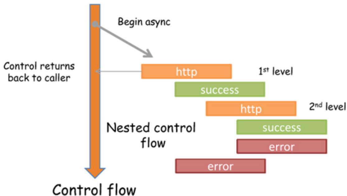
Figure 8.2. A program’s simple linear control flow breaks down on a remote call and degenerates into a waterfall of nested function calls—a pyramid that grows horizontally like a “Christmas tree of doom.”
