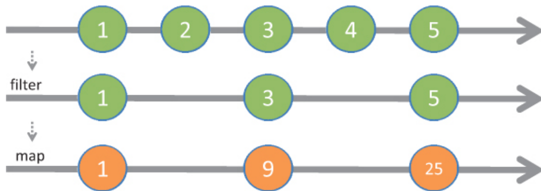
Figure 8.12. The process of applying functions filter and map from an observable sequence of numbers
