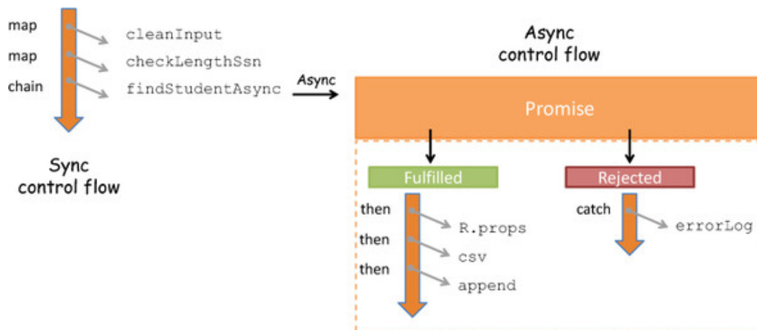
Figure 8.9. When composing synchronous code with asynchronous behavior, there's a point of inflexion in the program where the code shifts into a time-bound adjacent sequence of events that happen within the confines of the promise type.
