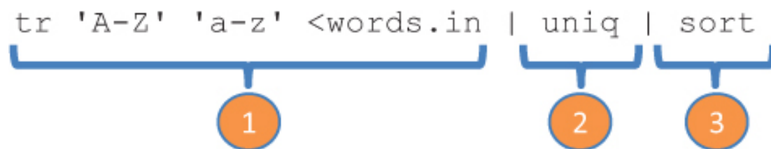
Figure 4.13. A simple Unix shell program, piping together a sequence of functions or programs
