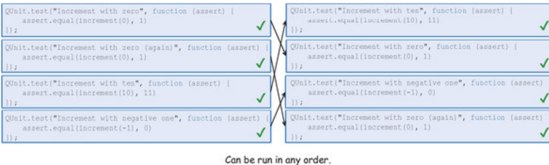
Figure 6.5. Tests against the functional increment function, which can be repeated or run in a different order without altering their outcome
