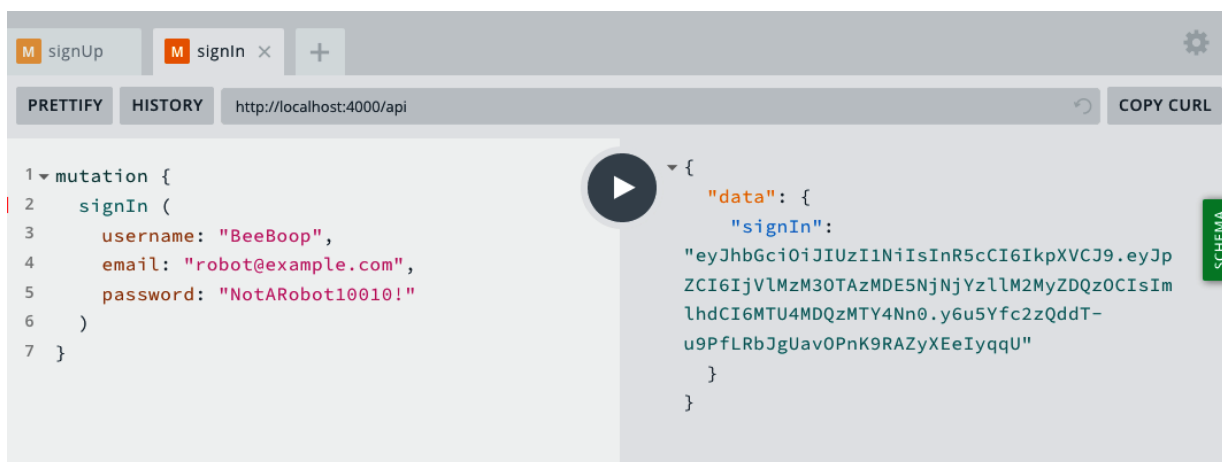
Figure 7-2. The signIn mutation in the GraphQL Playground
