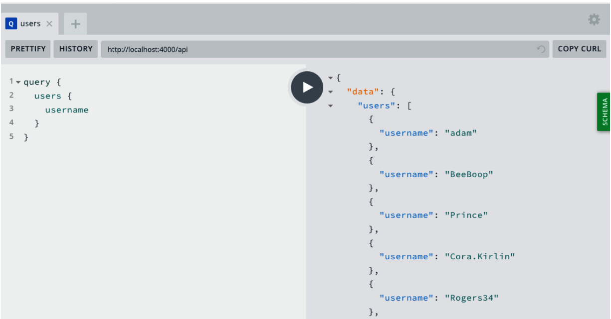
Figure 15-2. We can also see a list of users by performing a users query in the GraphQL Playground
