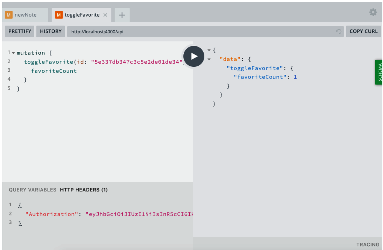
Figure 8-6. The toggleFavorite mutation
