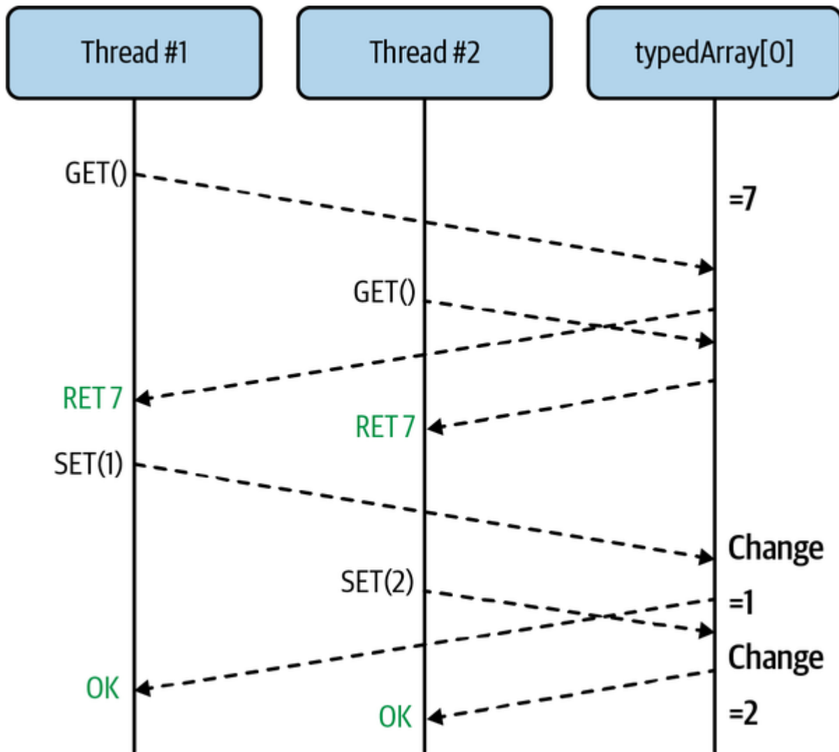
Figure 4-3. Nonatomic form of Atoms.compareExchange()
