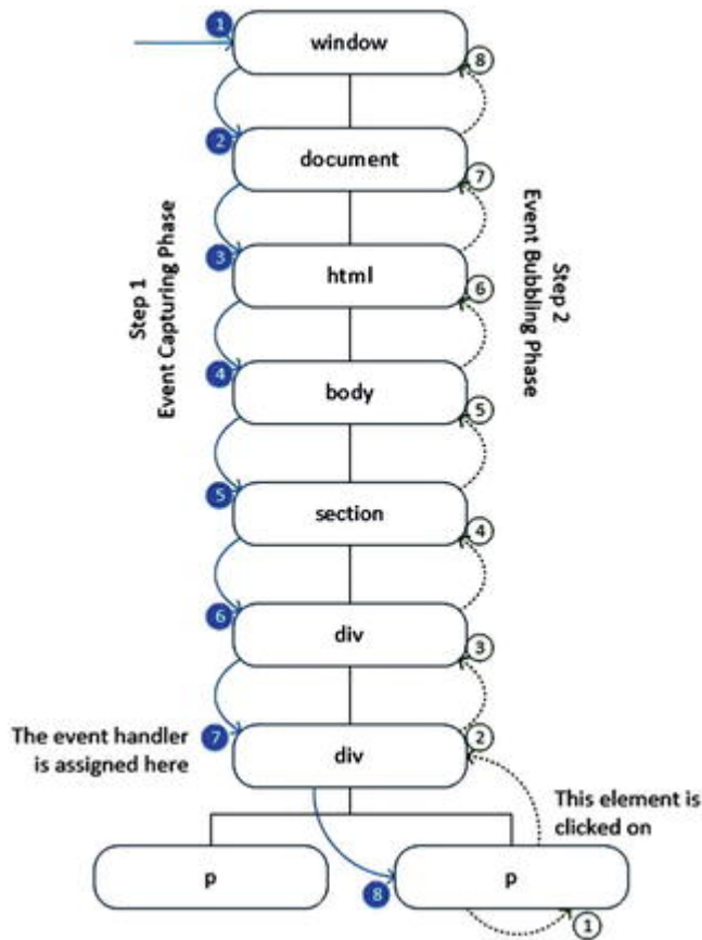
Figure 20-2. Event propagation
