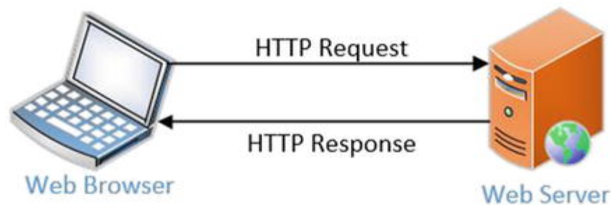
Figure 8-1. Client/Server Architecture
