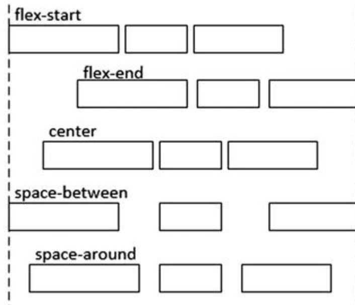
Figure 14-4. Justification along the main axis
