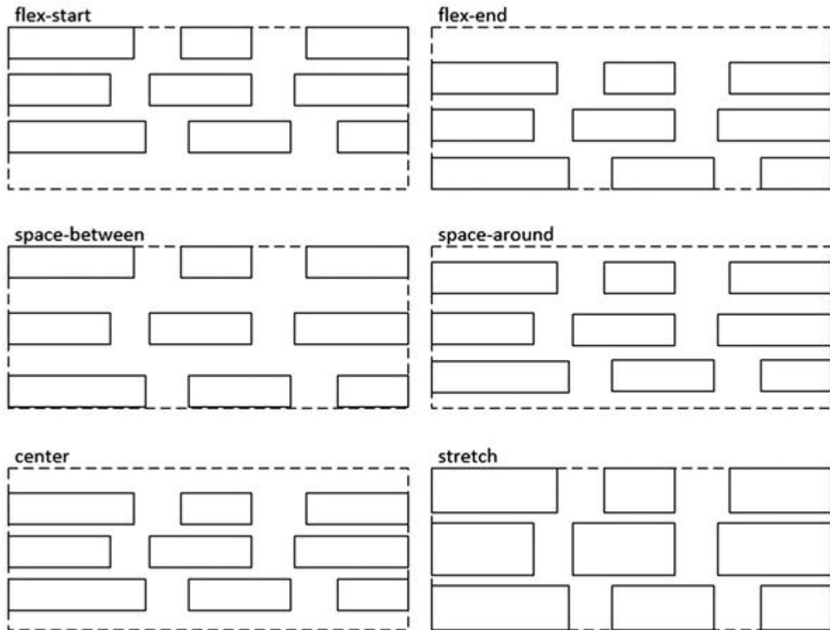
Figure 14-5. Justification along the cross axis
