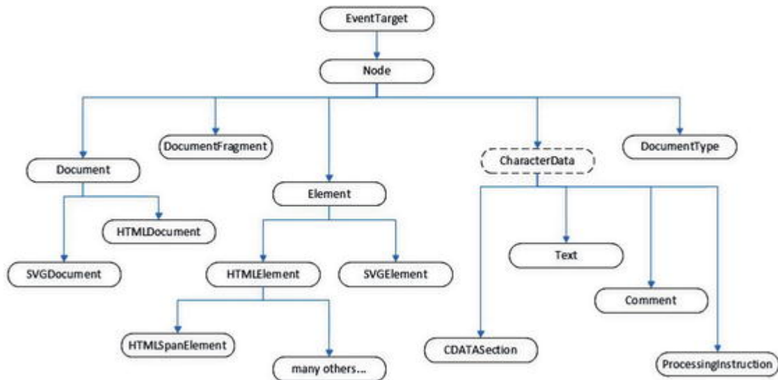
Figure 18-2. The inheritance hierarchy
