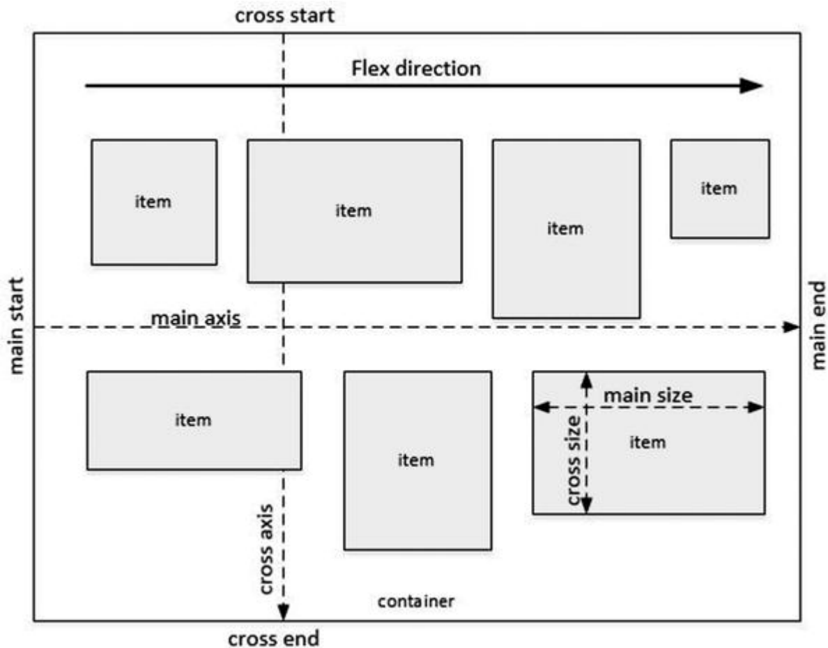
Figure 14-1. Illustrating flexbox terminology
