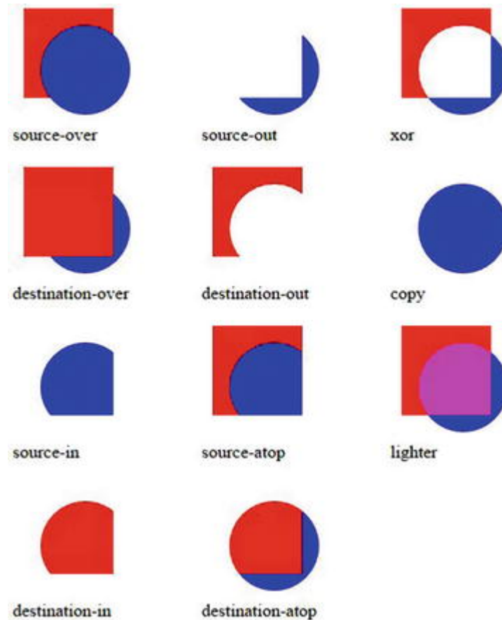
FIGURE 23-13. DEMONSTRATING THE COMPOSITING OPTIONS
