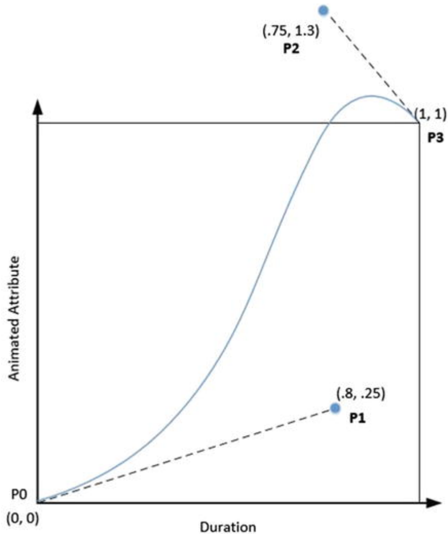
Figure 15-1. Cubic Bézier
