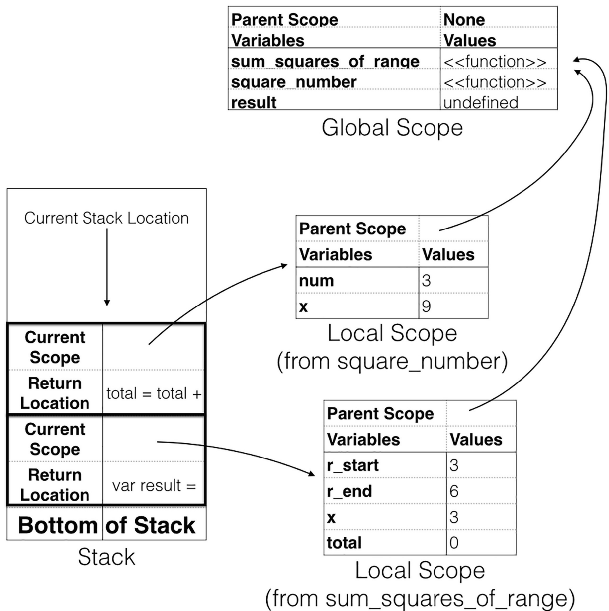
Figure 13-10 Stack Frame with Two Functions Active
