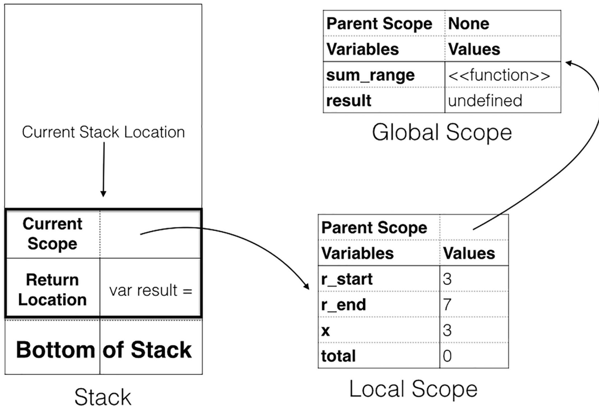
Figure 13-8 Conceptual Layout of Computer Memory in a Function Call
