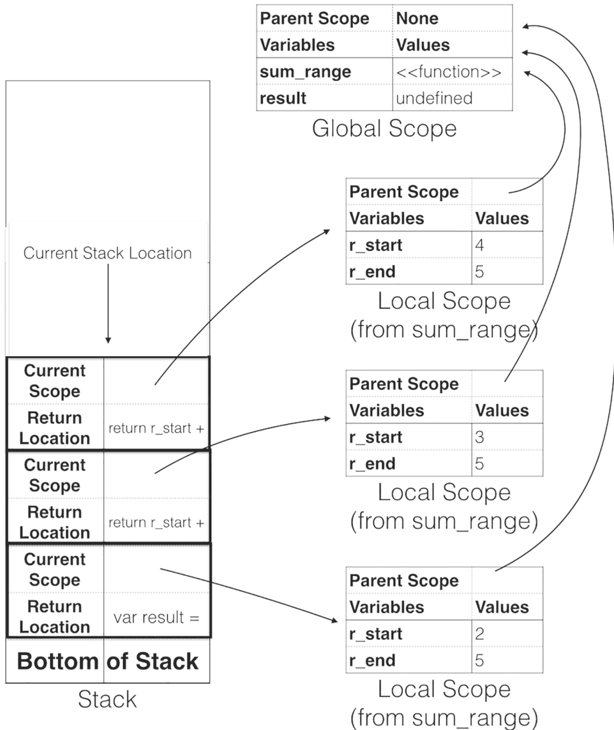
Figure 13-13 Stack Frame for Recursive Function Call
