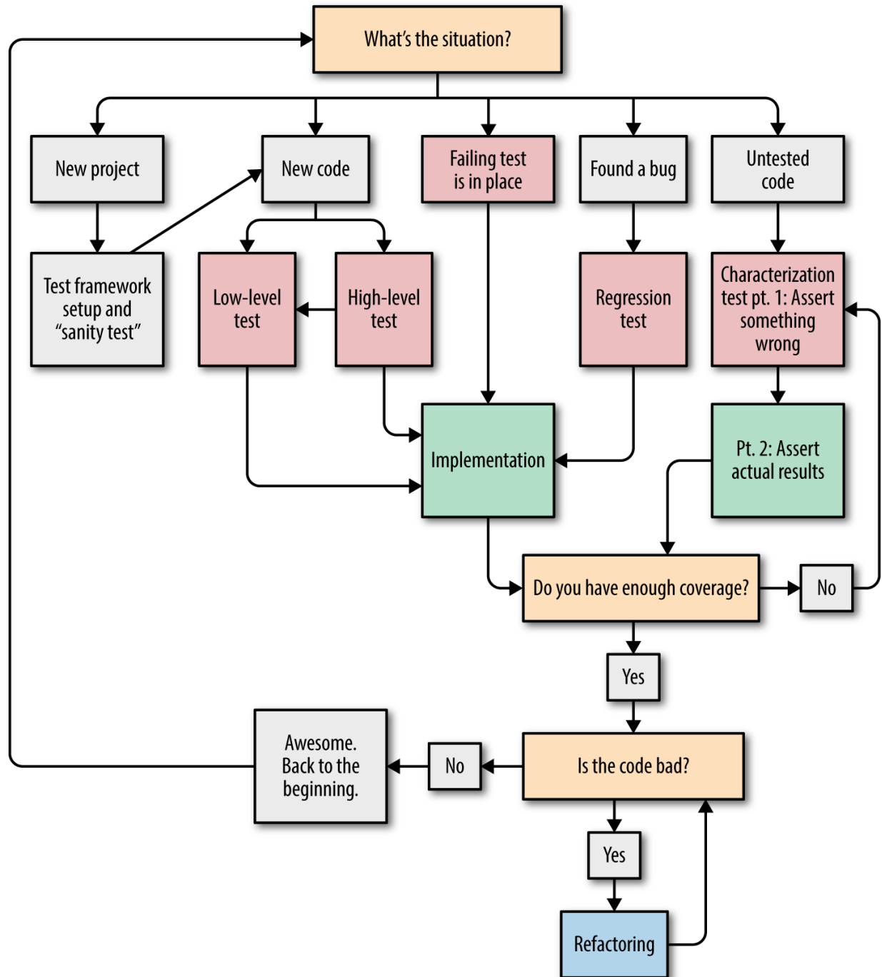
Figure 5-1. Testing and refactoring flow chart
