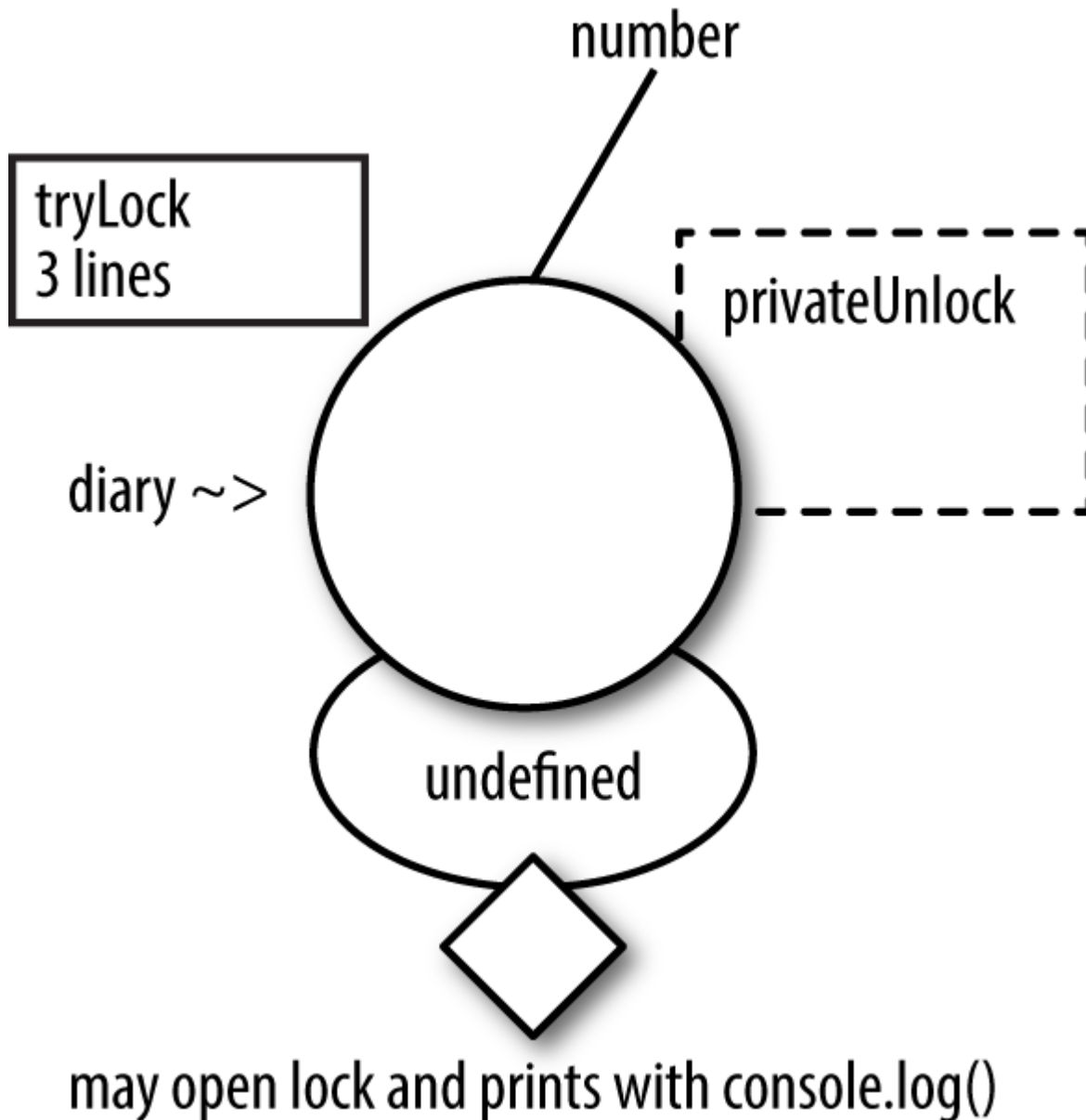
Figure 5-19. The tryLock function of diary
