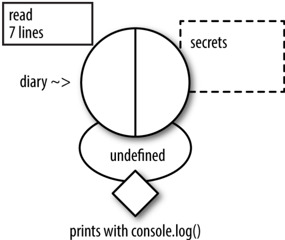
Figure 5-18. The read function of diary
