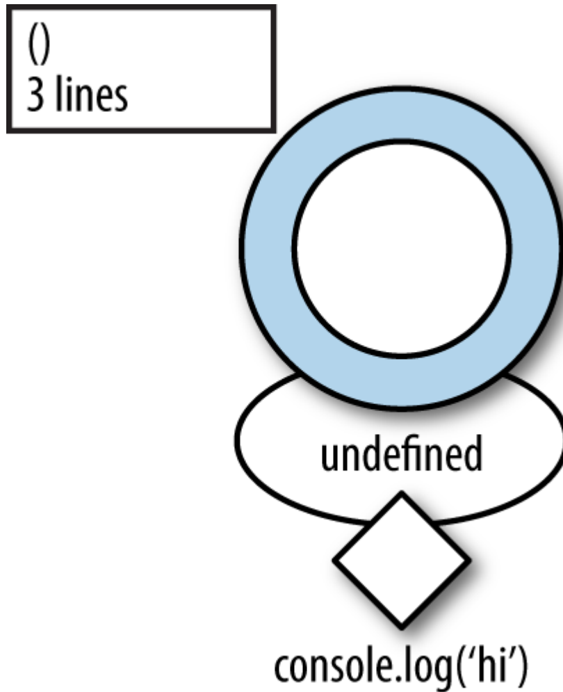
Figure 5-17. A “private” anonymous function
