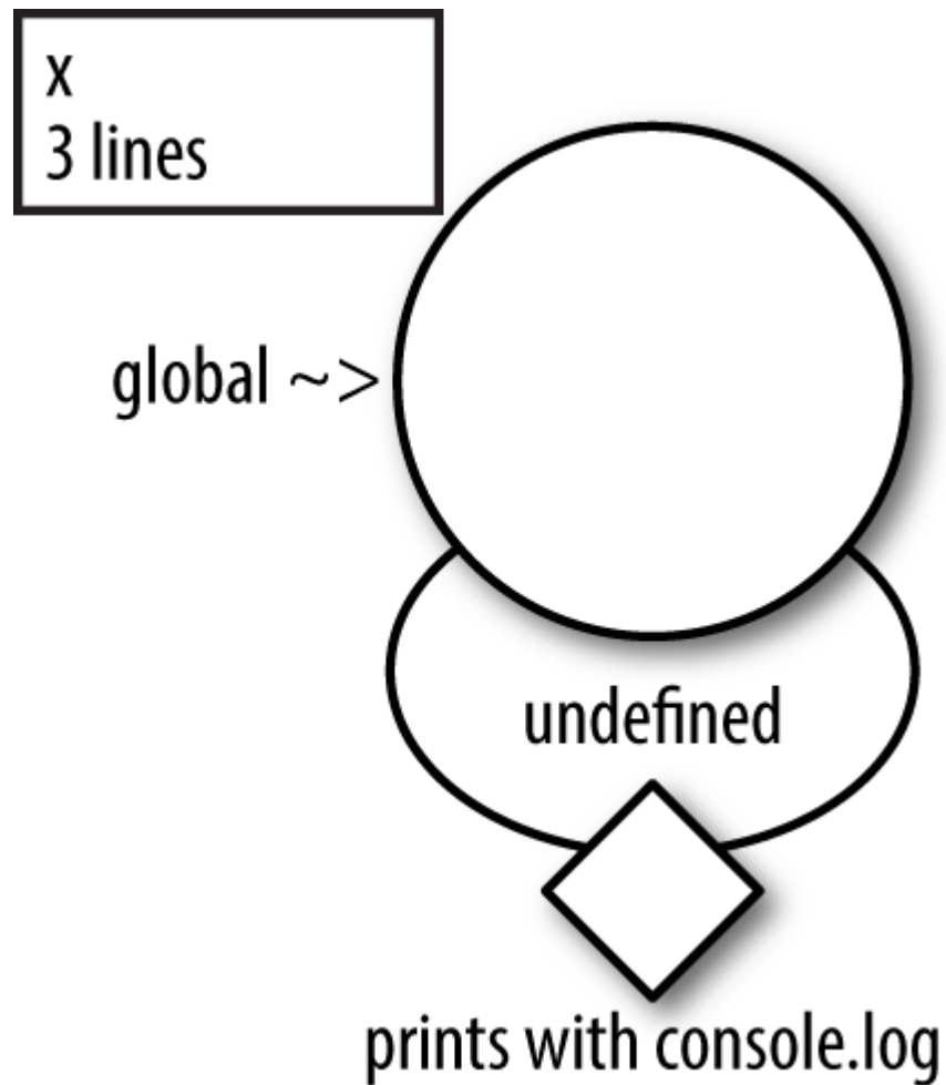
Figure 5-12. This function has the global object as its “this” value
