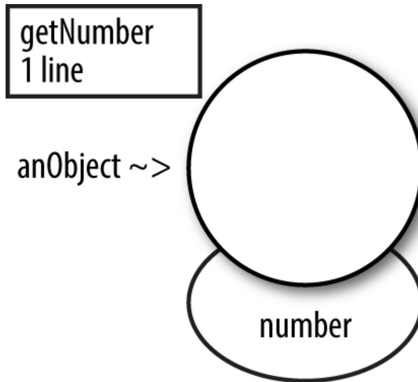
Figure 5-14. getNumber attached to a this of anObject
