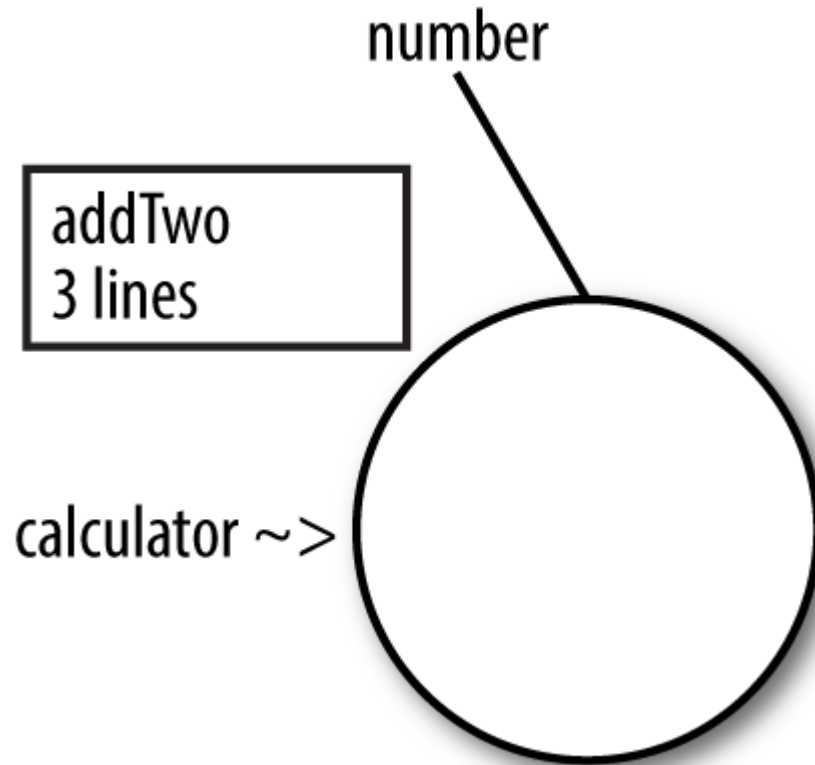
Figure 5-6. addTwo function with explicit input ( number ) and implicit input ( calculator )
