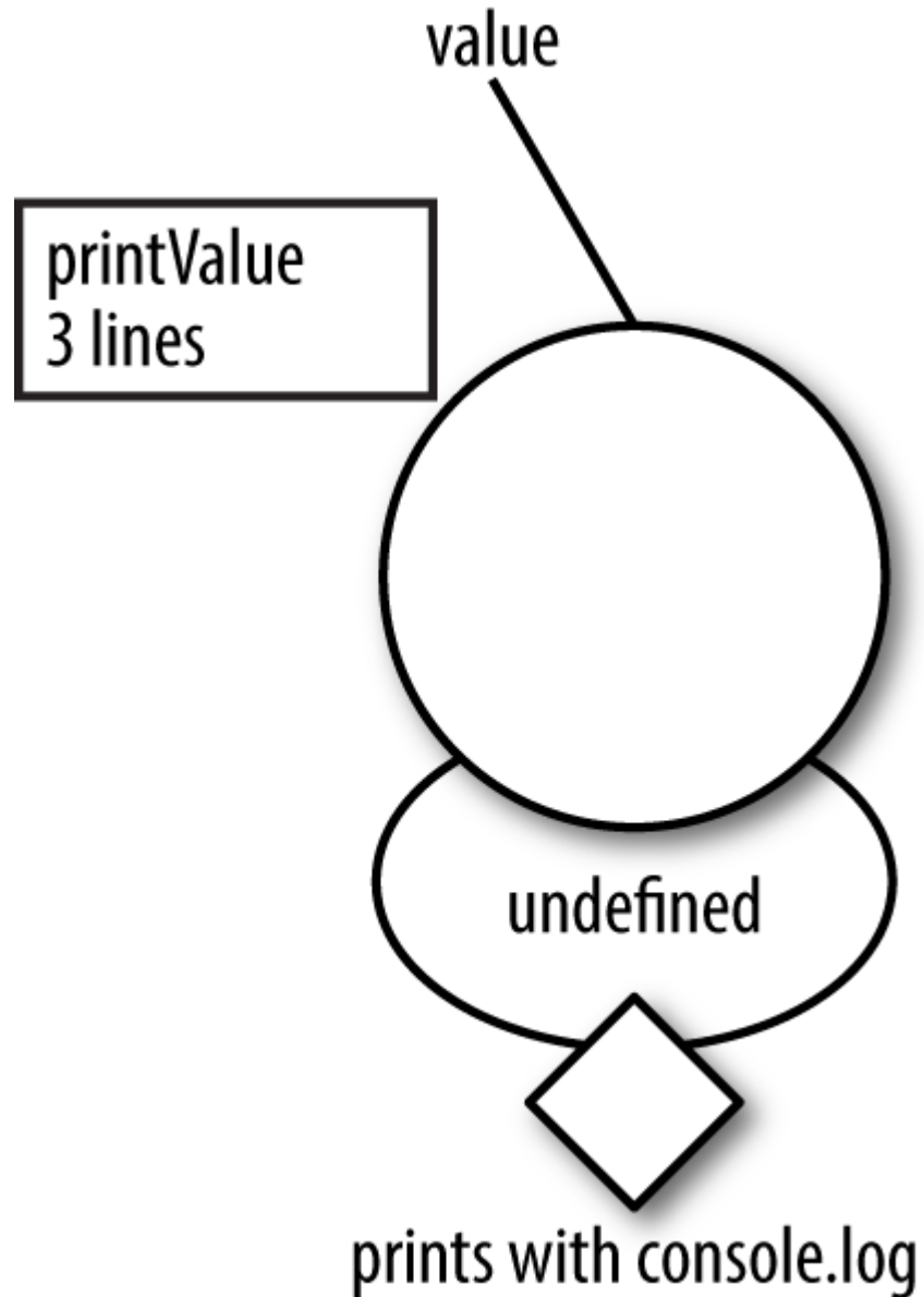
Figure 5-11. A function with a very common side effect: logging
