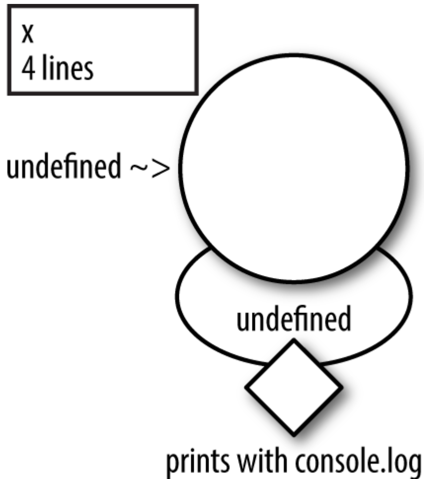
Figure 5-13. A function with a this value of undefined
