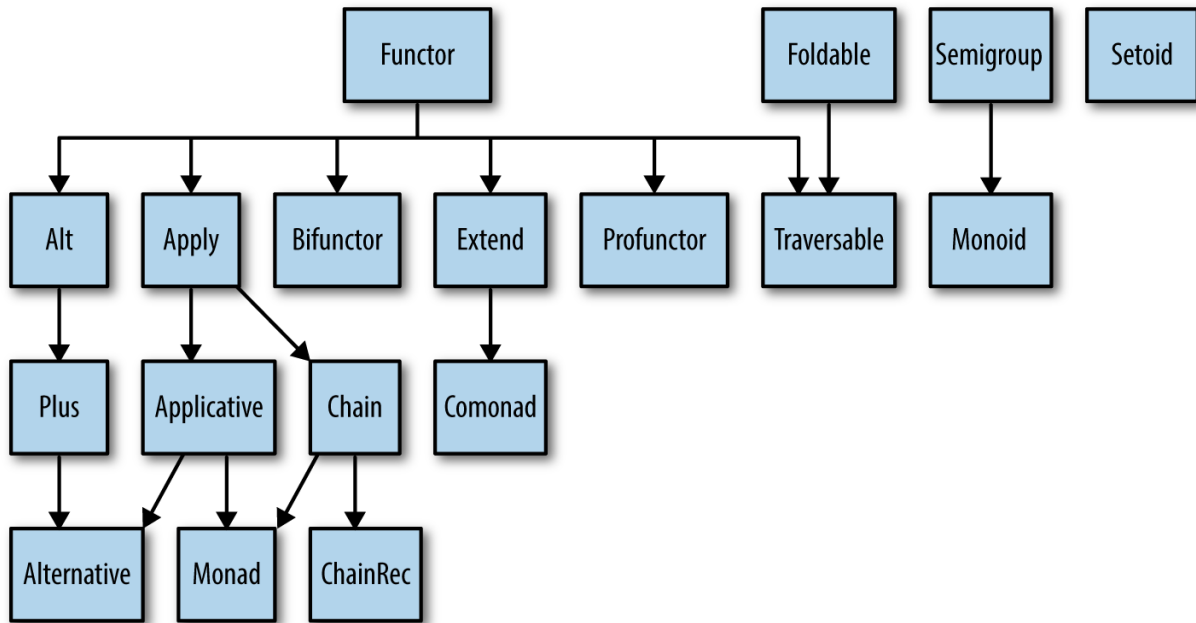
Figure 11-2. The Fantasy Land specification for burritos in JS
