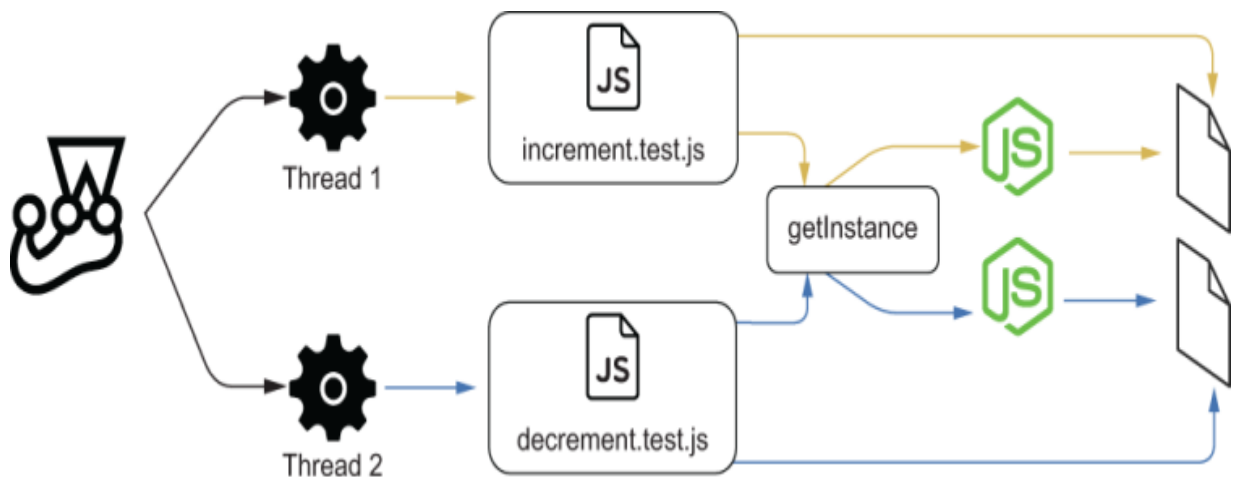
Figure 5.2 Each test obtains a different instance of the module through getInstance and checks a different underlying resource.
