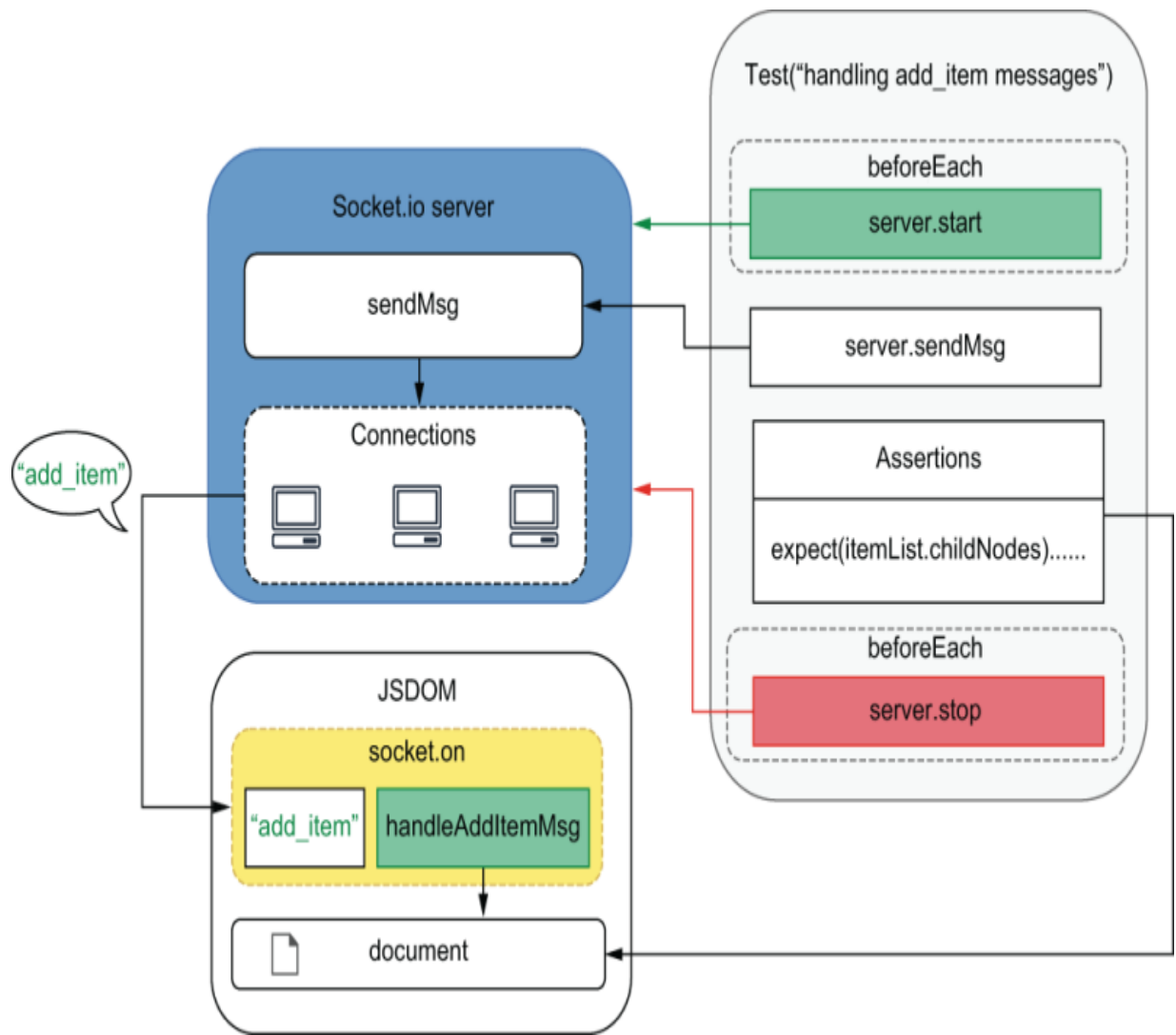
Figure 6.9 How your tests communicate with your Socket.io server, causing it to update the document so that they can perform assertions
