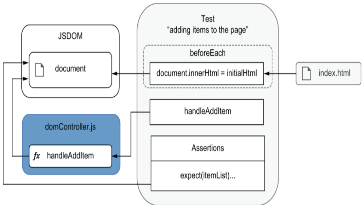
Figure 6.4 The test for handleAddItem invokes it directly, causing it to update the document.
