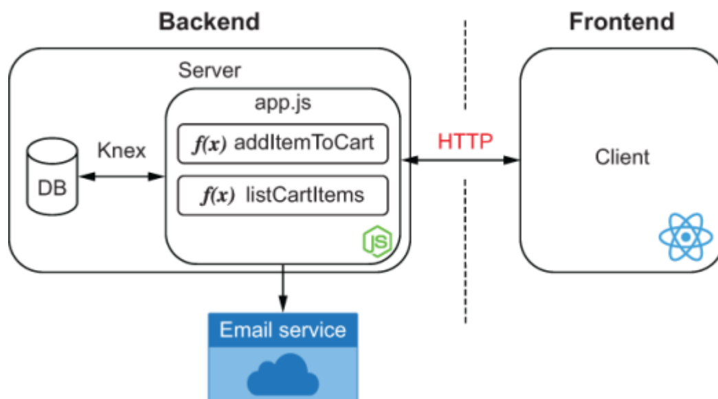
Figure 2.3 The bakery's website infrastructure
