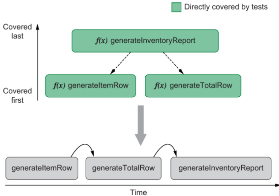
Figure 9.10 When taking a bottom-up approach to writing tests, you validated the most granular pieces of software first and the most coarse later.
