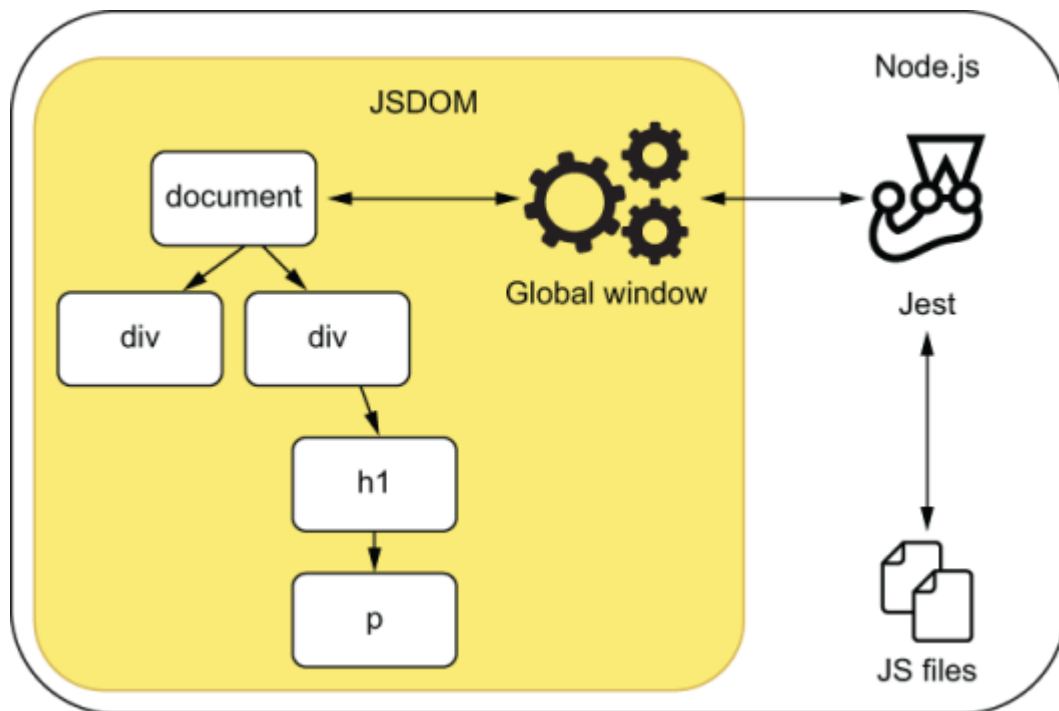
Figure 6.2 The JavaScript environment within Node.js
