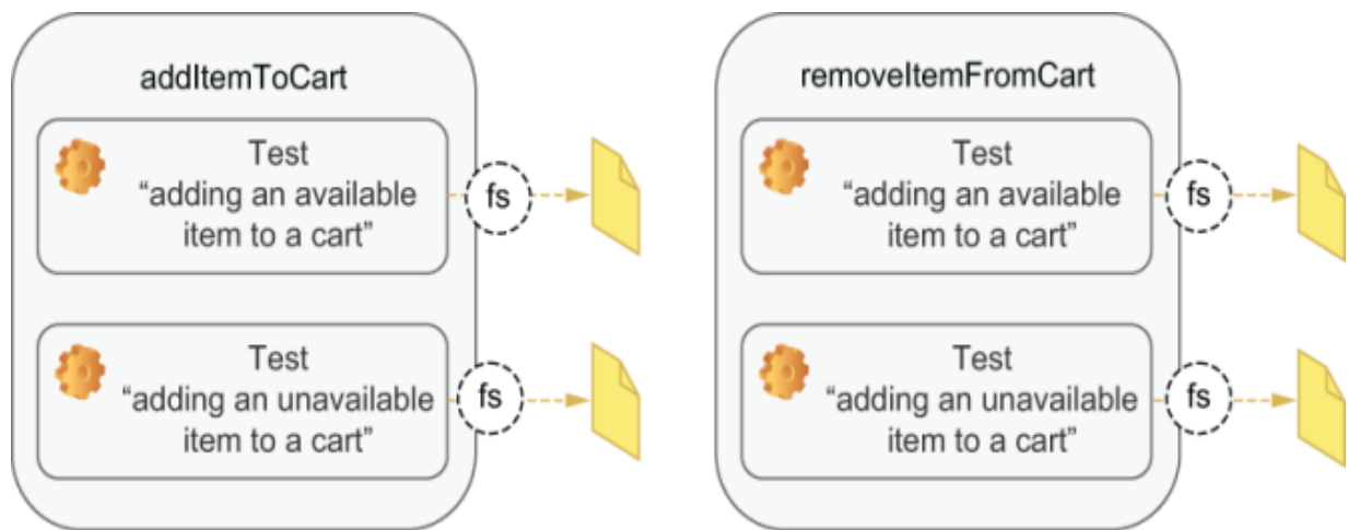
Figure 5.7 In each test that depends on the logger, you will repeat the same code to read the log file and perform similar assertions.
