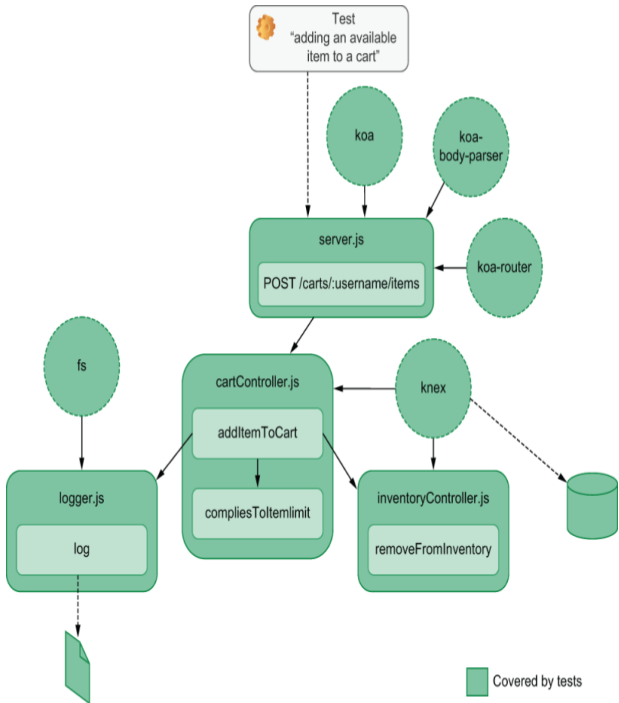
Figure 5.3 An end-to-end test that sends a request to this route will cause functions like addItemToCart , compliesToItemLimit , removeFromInventory , and log to be executed.
