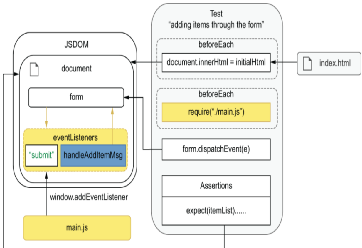
Figure 6.5 By dispatching events through the form, the application triggers the event listener attached by main.js .
