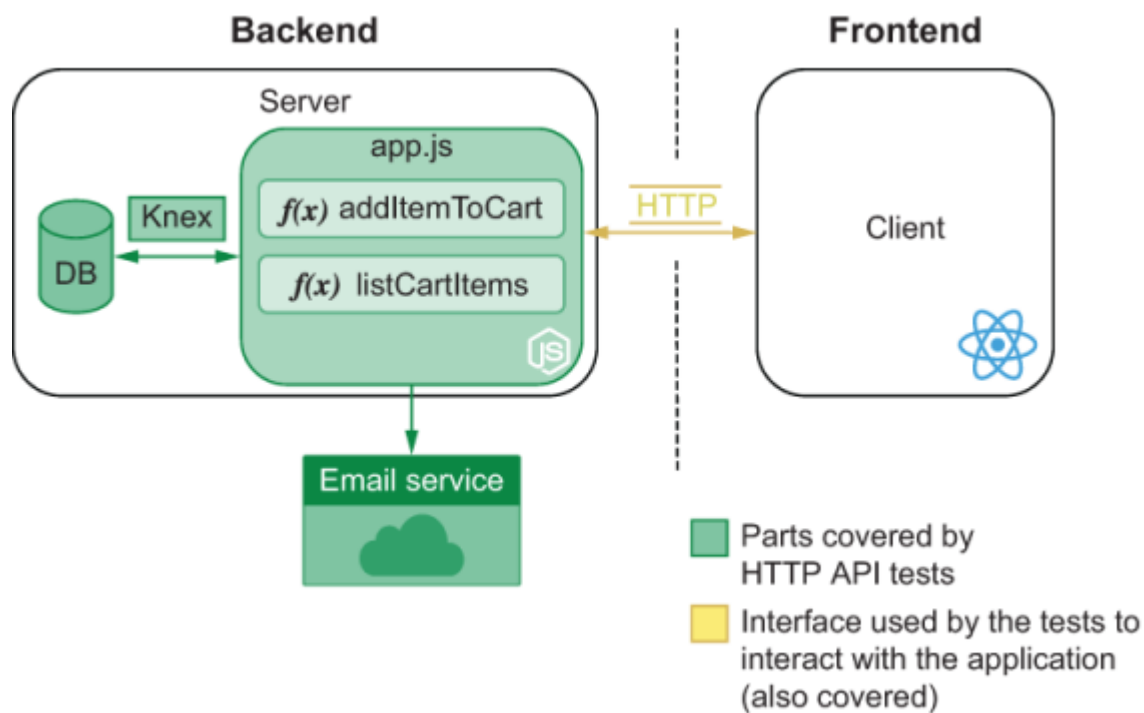
Figure 2.10 The scope of tests that address your backend through its HTTP API
