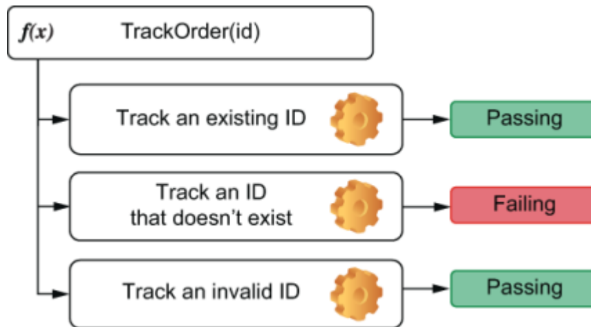
Figure 1.7 The tests for the trackOrder function can call that function directly, so you don't have to touch other parts of the application.
