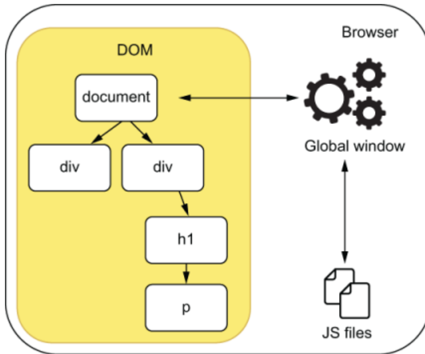
Figure 6.1 The JavaScript environment within a browser
