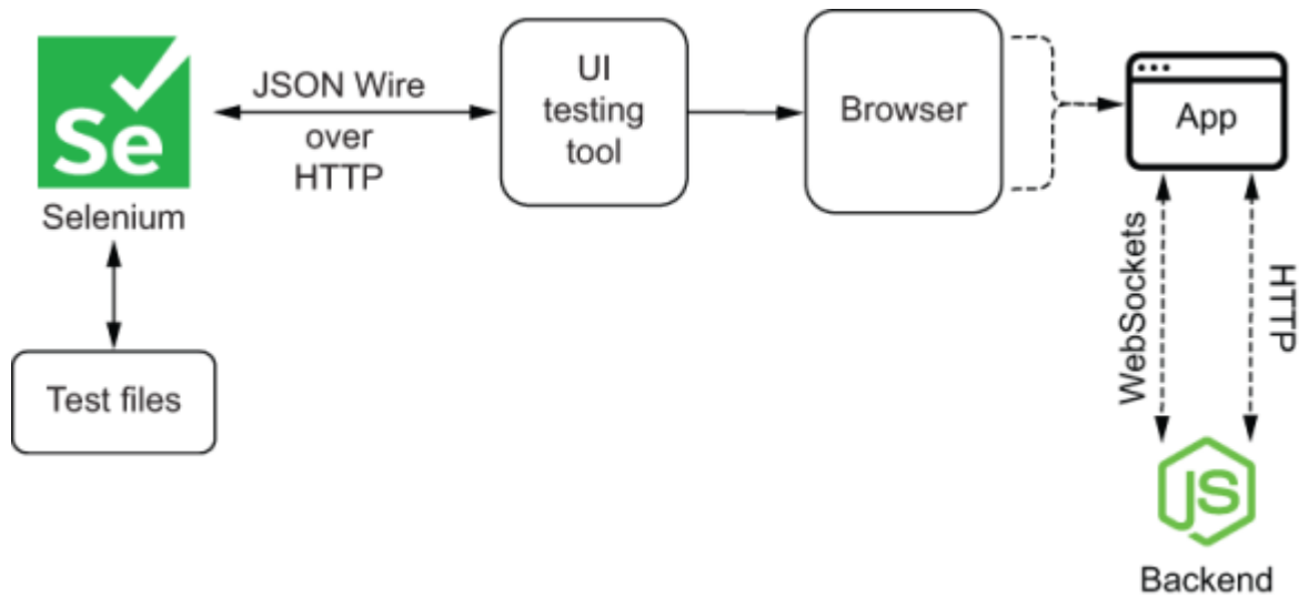
Figure 10.5 Selenium sends HTTP requests to the Webdrivers that control browsers. These requests adopt the JSON Wire protocol.
