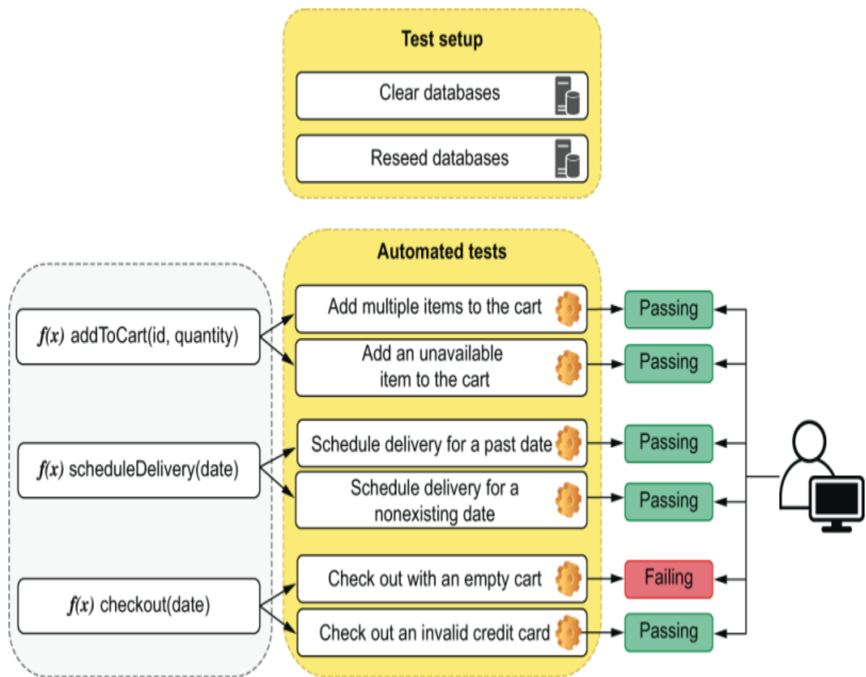
Figure 1.8 Automated tests can check parts of your code individually and give you precise feedback on what's broken as soon as you break it.
