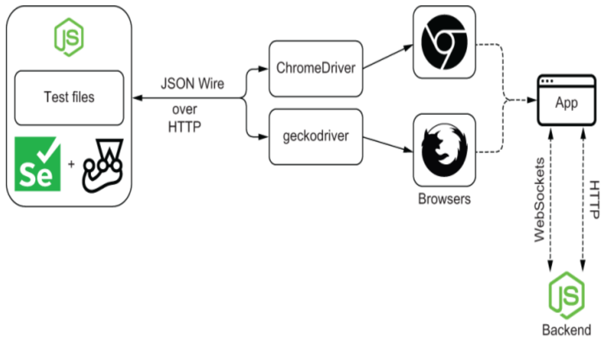
Figure 10.7 If you want to use Selenium for testing, you must pair it with a testing framework, such as Jest.
