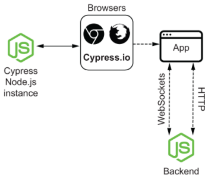
Figure 10.10 Cypress spawns a Node.js process that communicates with the tests that run within browsers themselves.
