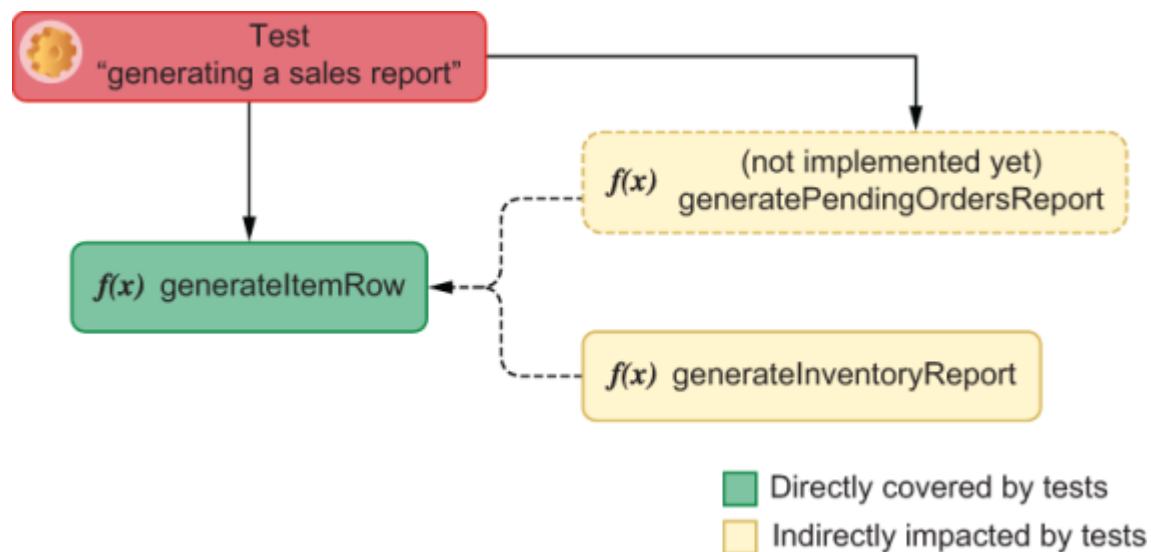
Figure 9.15 To avoid adding a new function and extra tests for it, you can update the generateItemRow function's tests and reuse them in multiple places.
