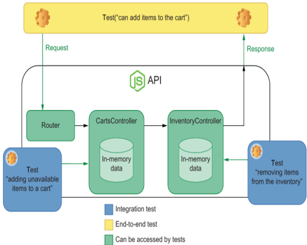
Figure 4.4 Which parts of your application each end-to-end and integration test has access to
