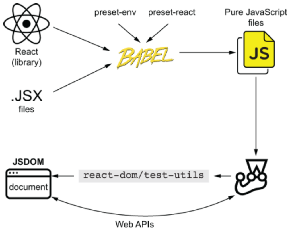
Figure 7.3 Testing components by using react-dom/test-utils to render components to the DOM and Web APIs to find and inspect the rendered elements
