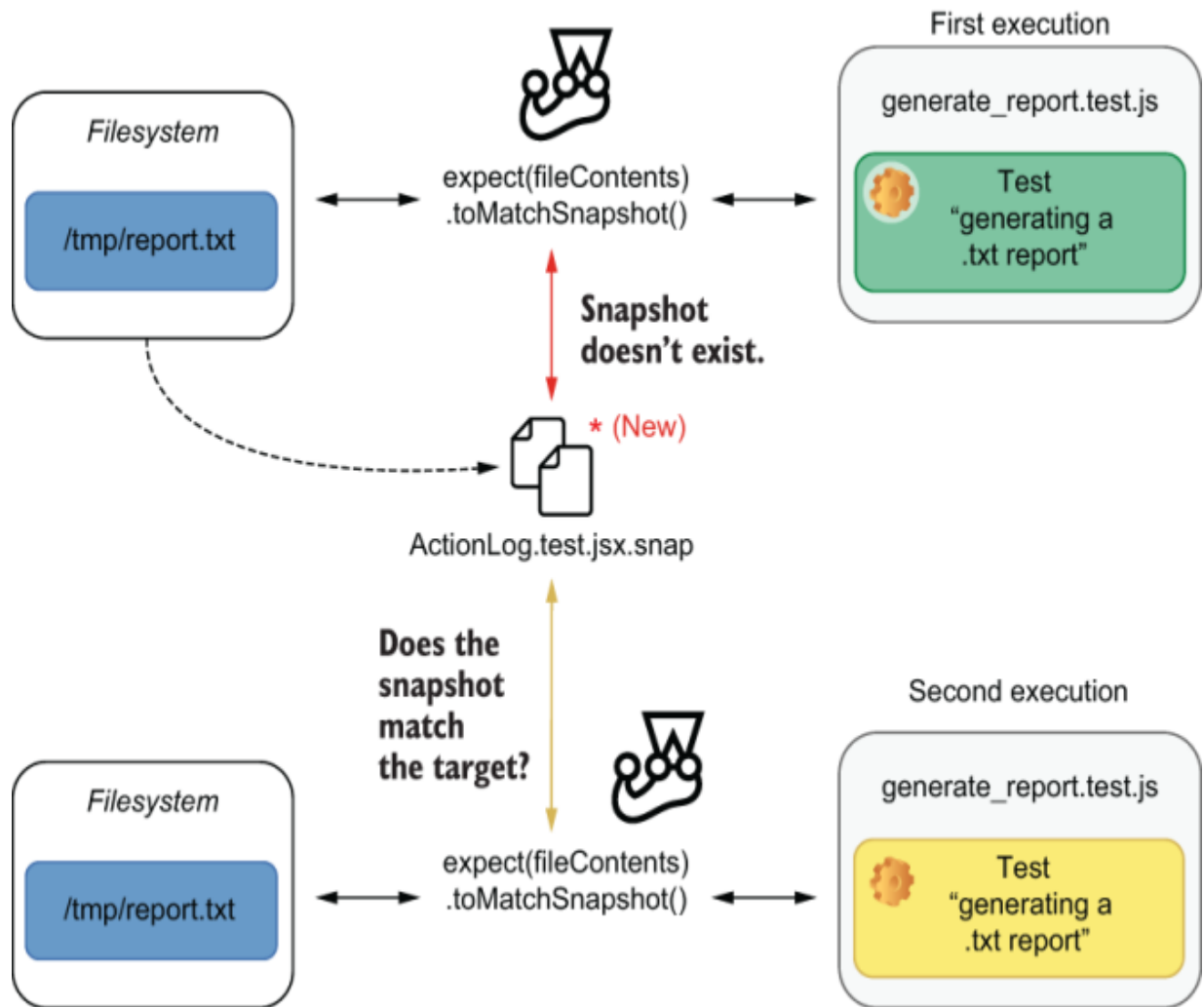
Figure 8.8 Jest creates a snapshot with the report's contents the first time it runs. The second time it runs, it will compare the report's actual content with what it had saved in the snapshot file.
