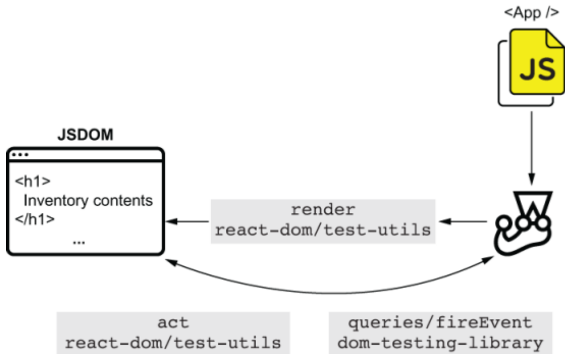
Figure 7.4 What happens when using react-dom/test-utils to render components but using dom-testing-library to find rendered elements and interact with them
