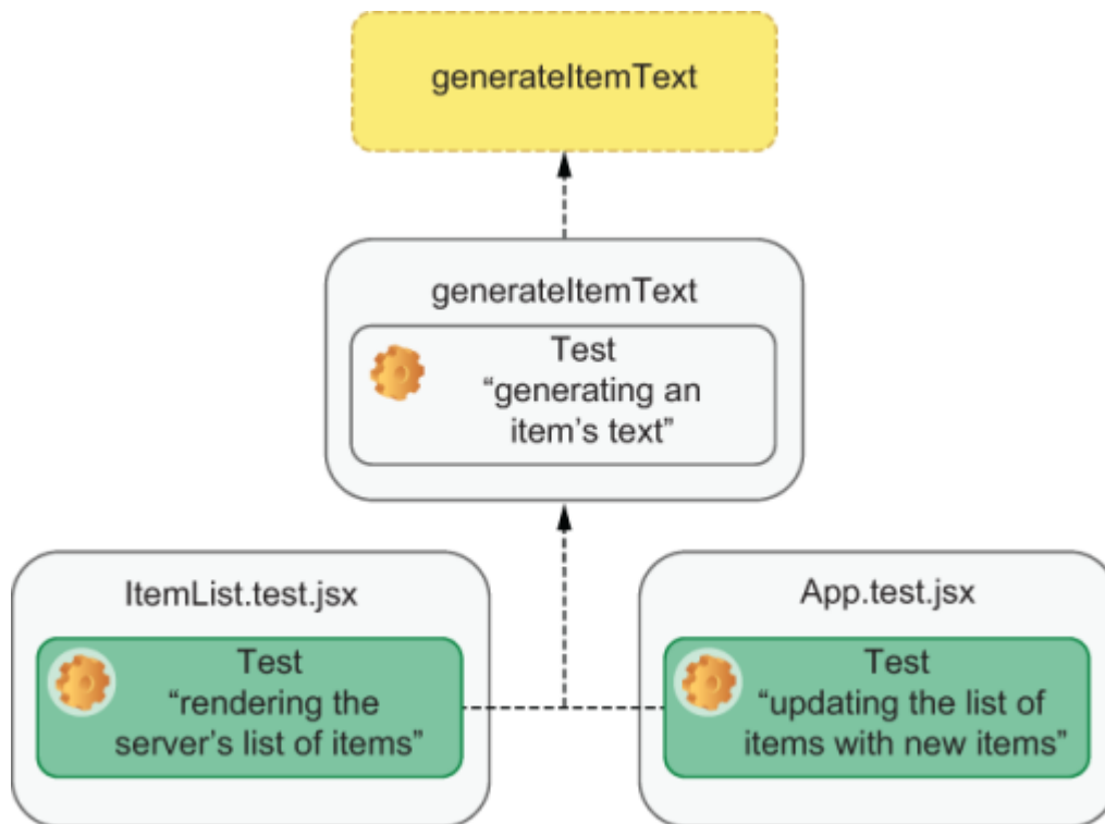
Figure 8.4 How centralizing the dependency on generateItemText creates a transitive guarantee
