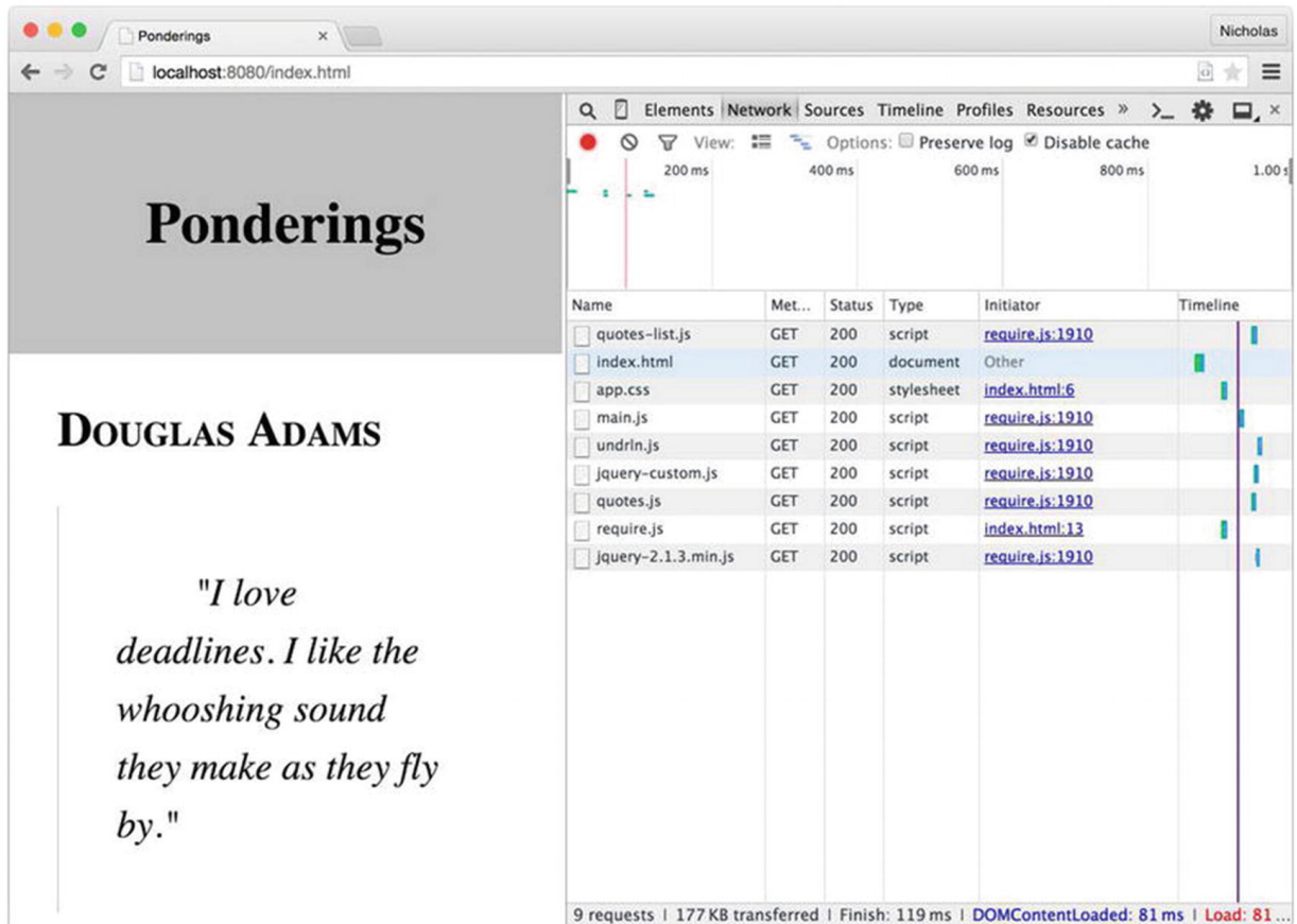
Figure 4-2 RequireJS modules shown loaded in Chrome
