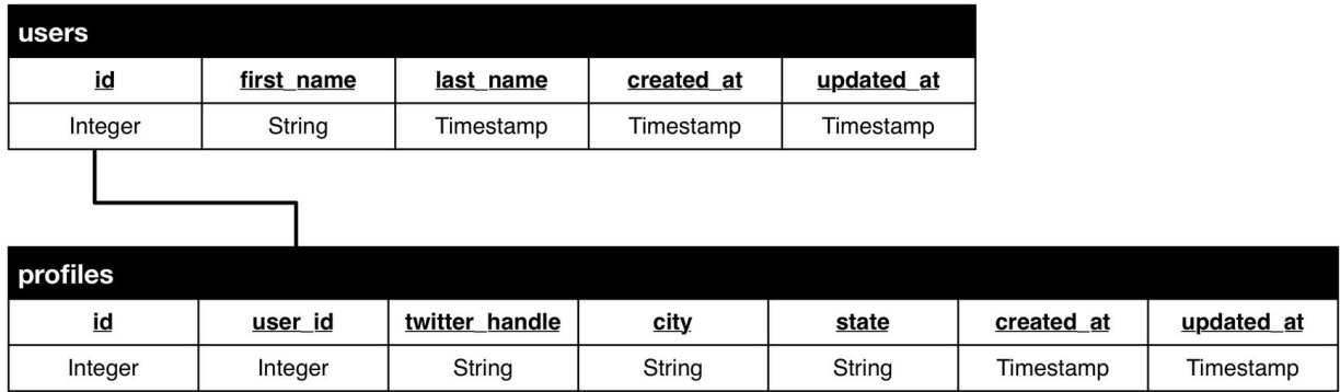
Figure 10-3 The database schema behind our one-to-one relationships
