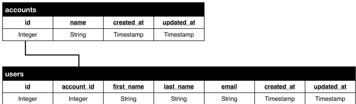
Figure 10-2 Here, the relationship between users and accounts (an account has one or more users, users belong to accounts) is described via the account_id foreign key column within the users table
