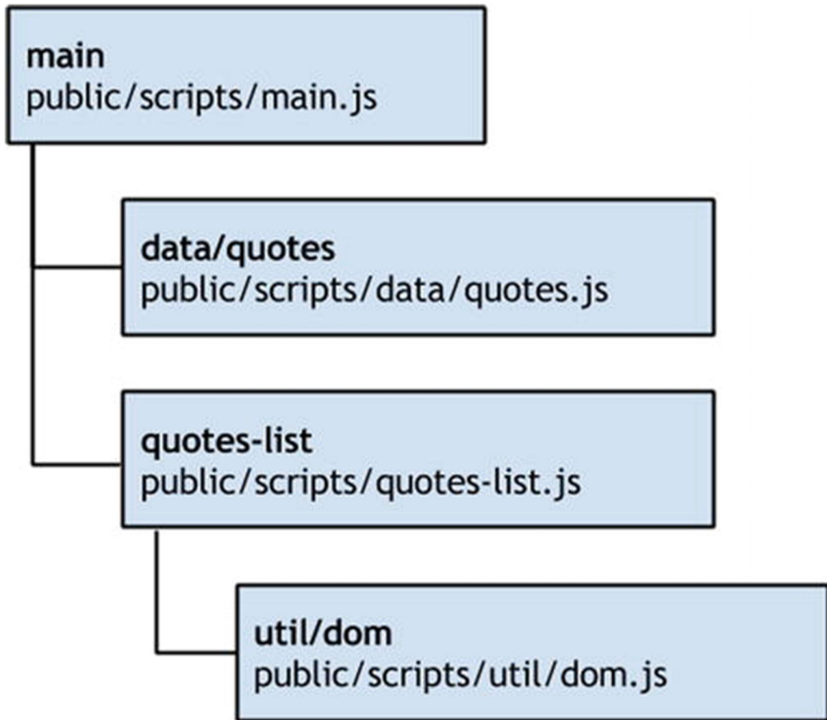
Figure 4-1 RequireJS dependency tree
