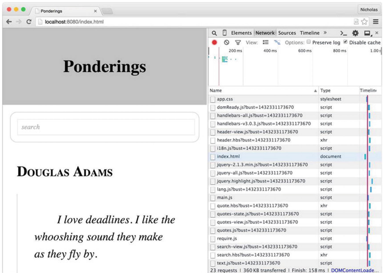
Figure 4-4 The bust parameter is appended to each RequireJS request
