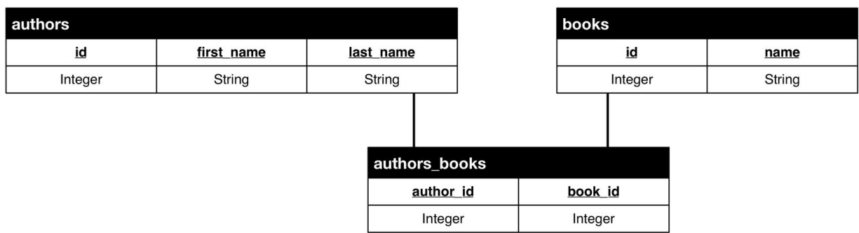
Figure 10-5 A many-to-many association made possible through the use of a third join table. In this example, an author can write multiple books, and a book can have multiple authors.
