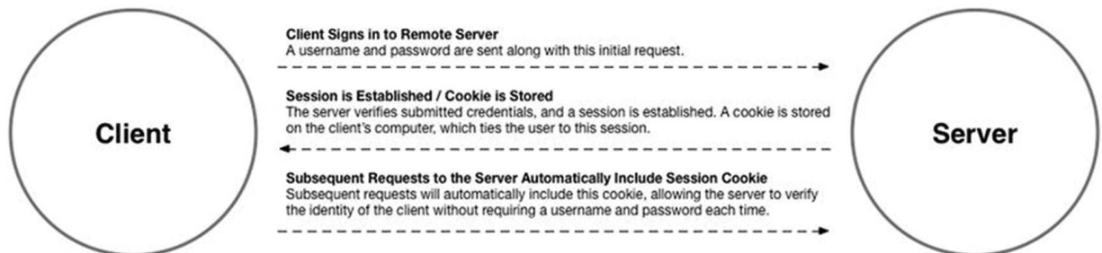
Figure 8-10 Cookie-based authentication
