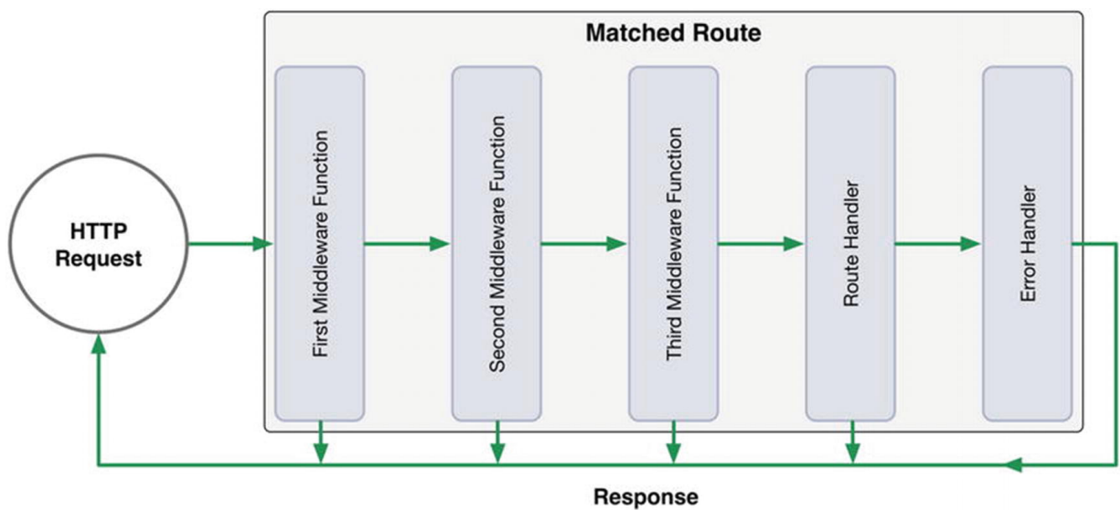
Figure 8-2 Series of Express middleware calls
