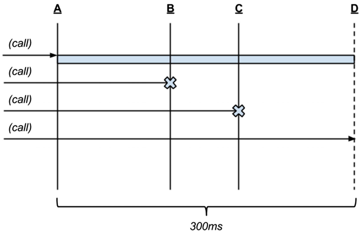
Figure 12-2 A throttled function invoked multiple times
