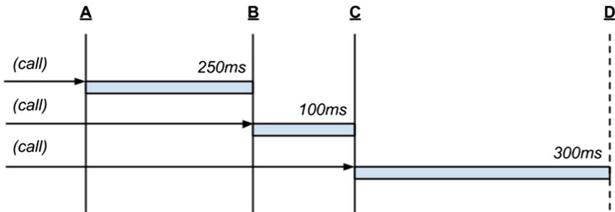
Figure 12-1 A debounced function invoked multiple times
