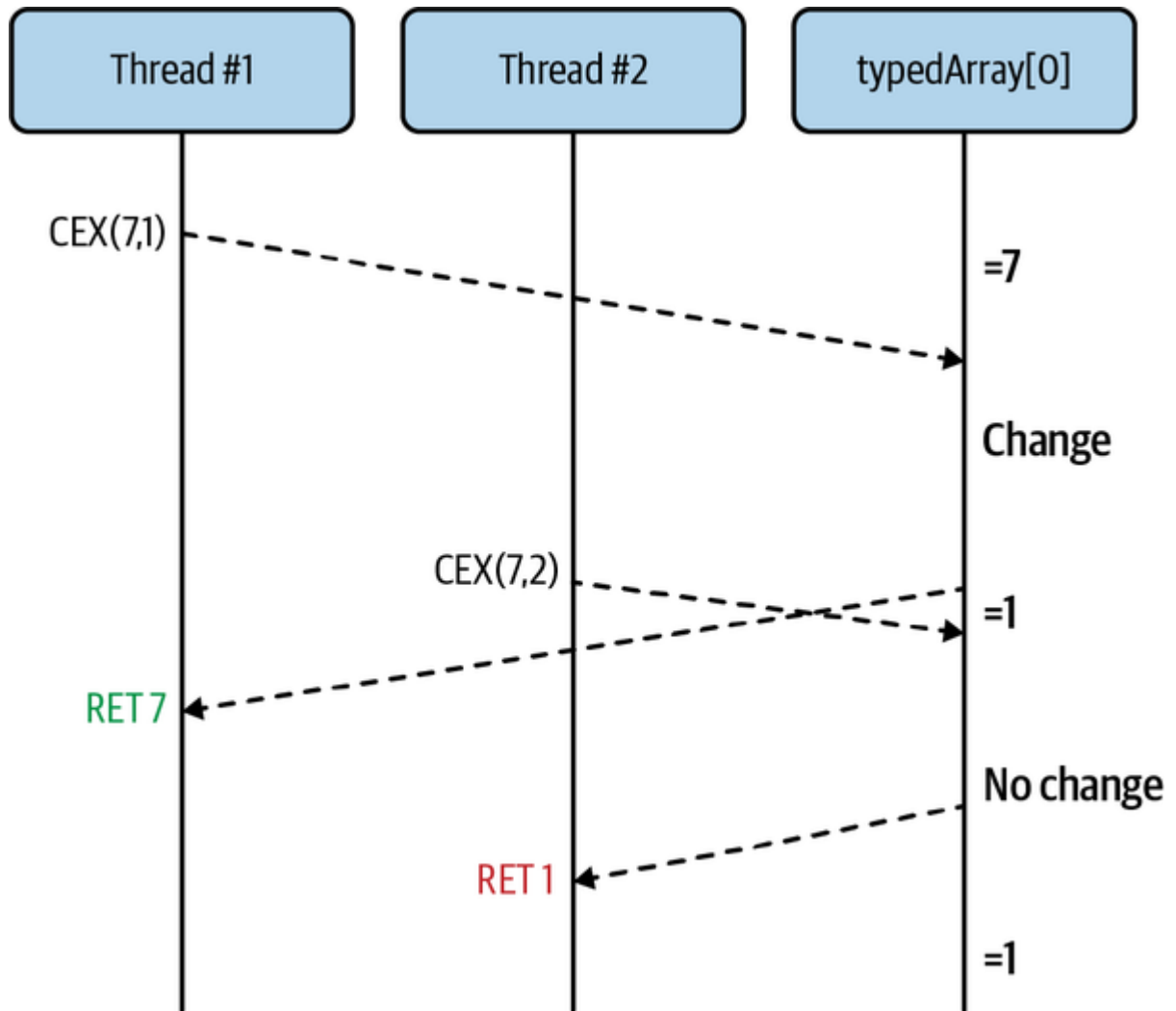
Figure 4-2. Atomic form of Atoms.compareExchange()
