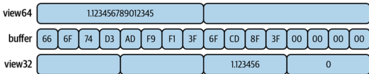
Figure 4-1. Single ArrayBuffer and multiple TypedArray views
