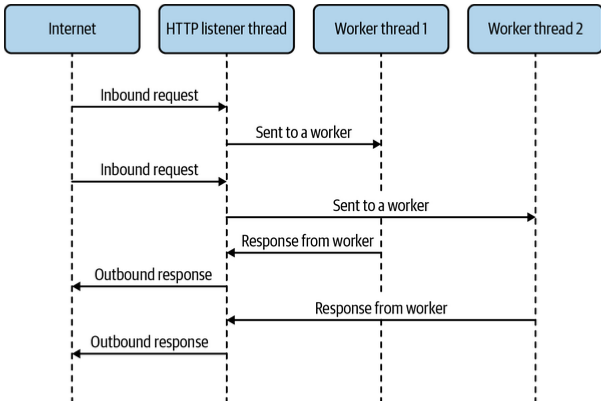
Figure 1-1. Worker threads as they might be used in an HTTP server
