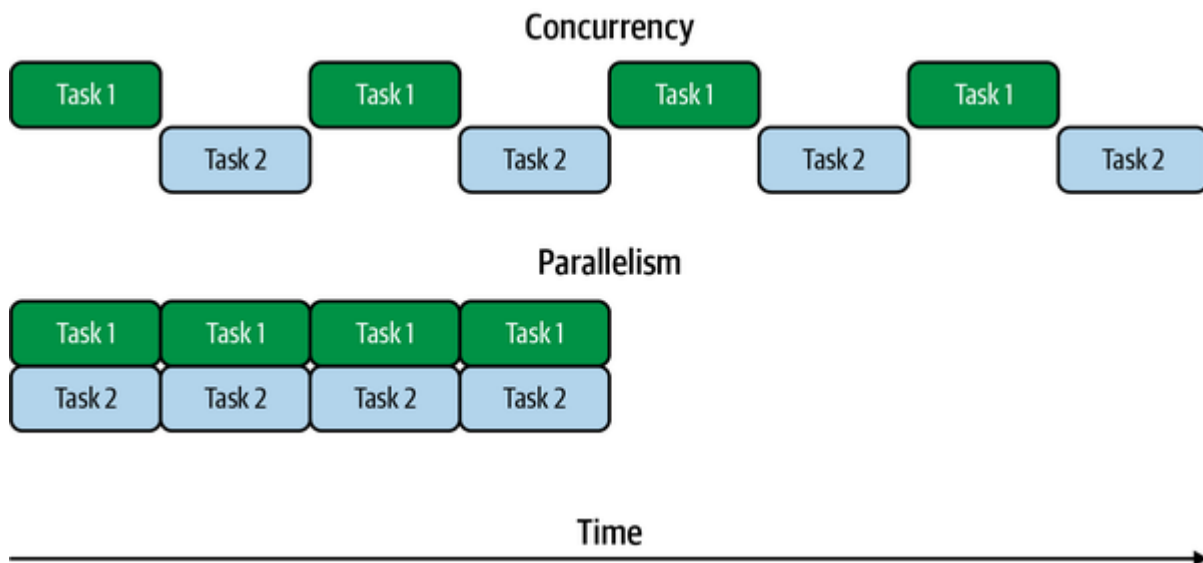
Figure 1-2. Concurrency versus parallelism
