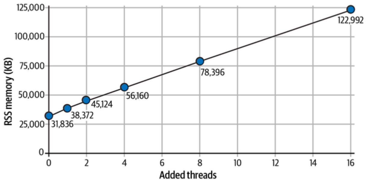
Figure 8-1. Memory usage increases with each additional thread
