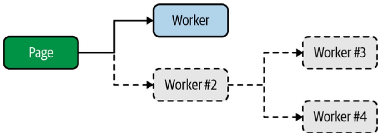
Figure 2-1. Dedicated worker relationship
