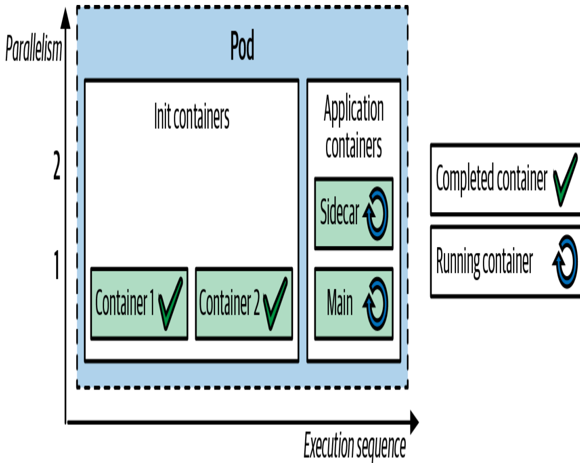
Figure 15-1. Init and application containers in a Pod
