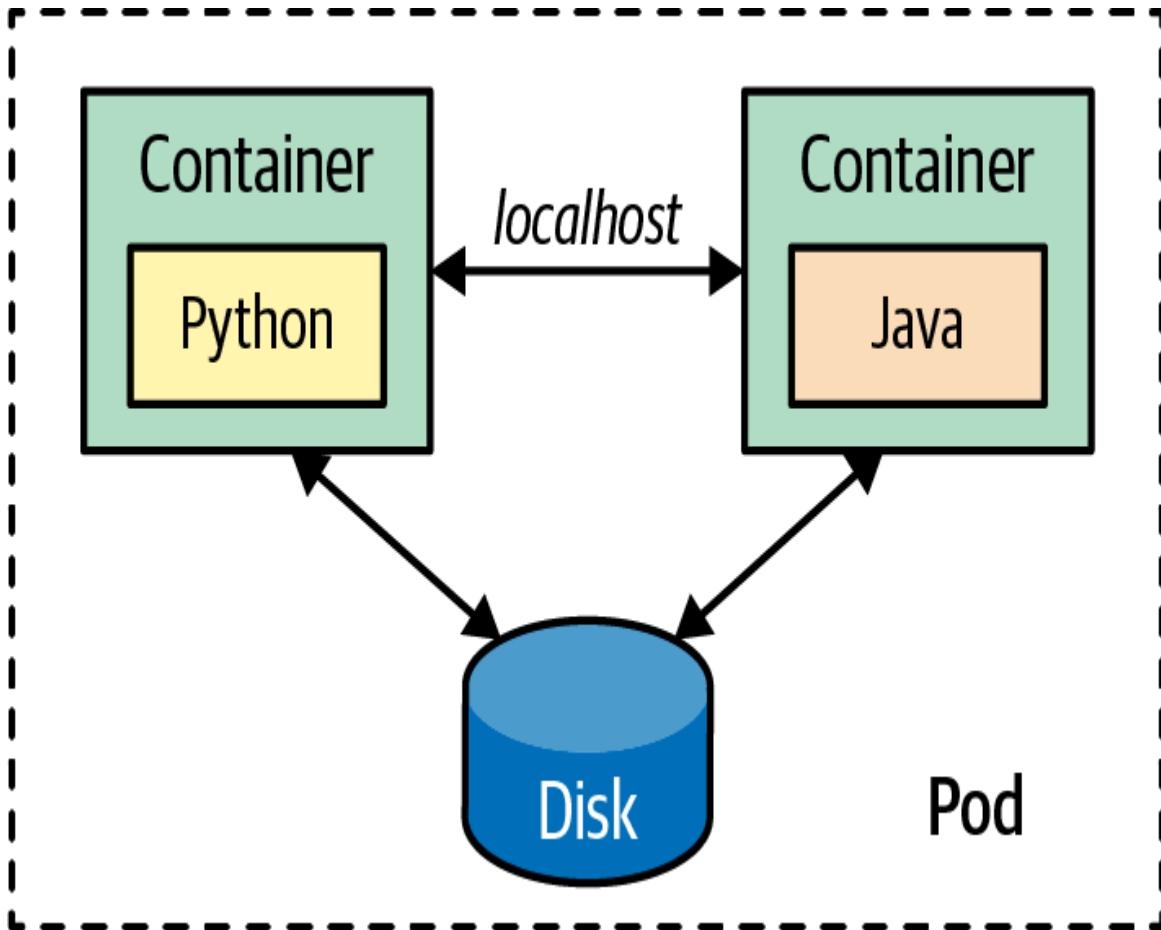
Figure 1-2. A Pod as the deployment and management unit
