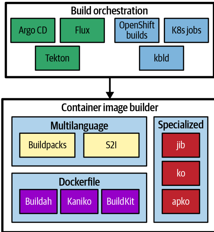
Figure 30-1. Container image builds within Kubernetes
