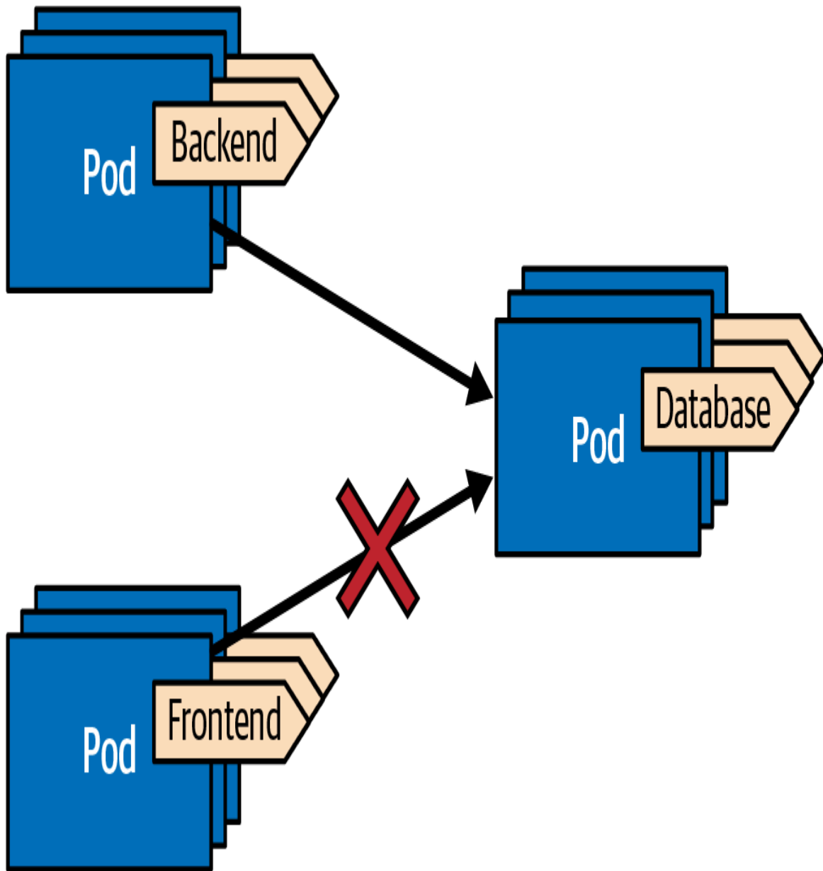
Figure 24-1. NetworkPolicy for ingress traffic
