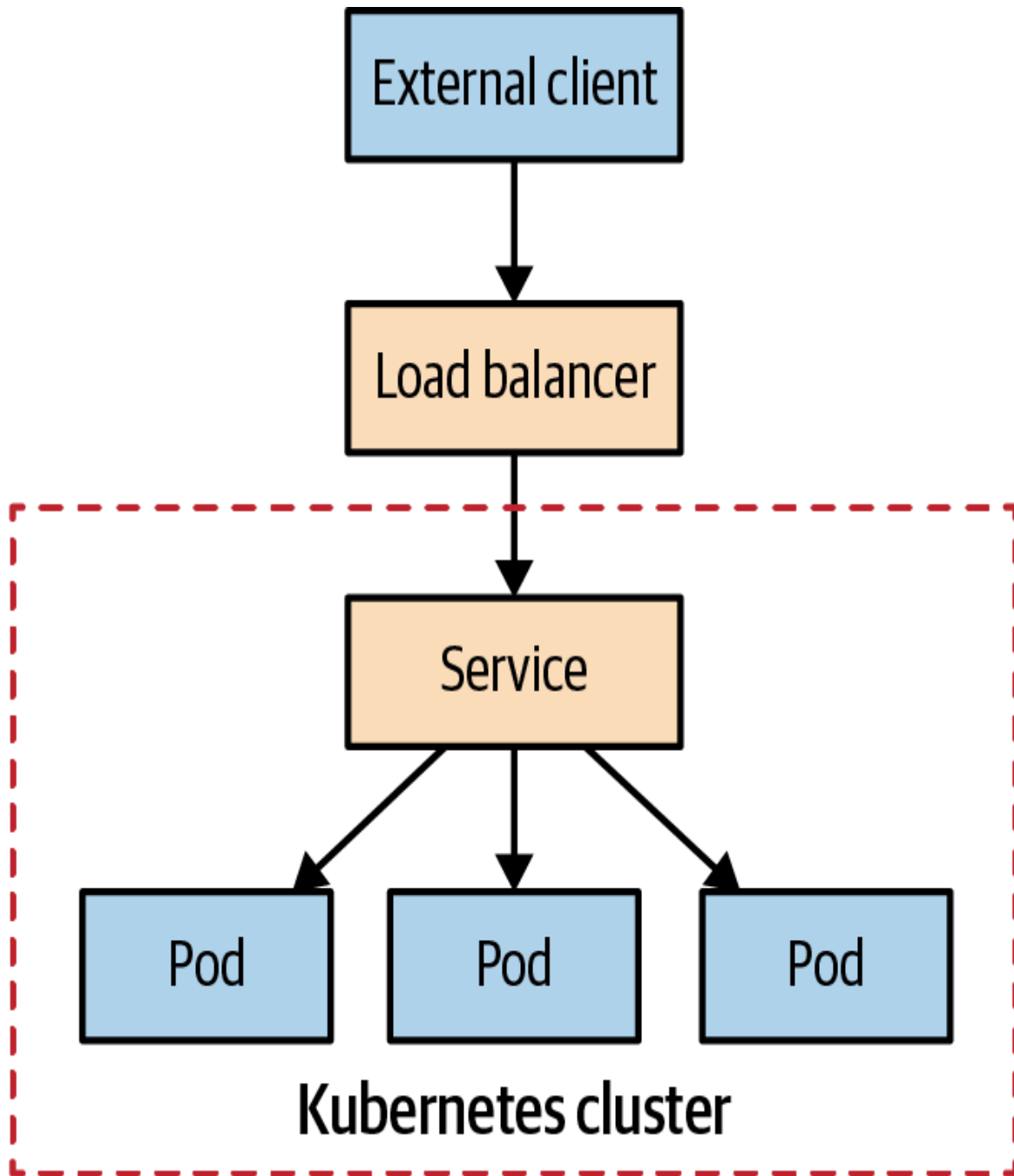
Figure 13-6. Load balancer service discovery
