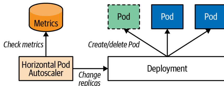
Figure 29-1. Horizontal Pod autoscaling mechanism
