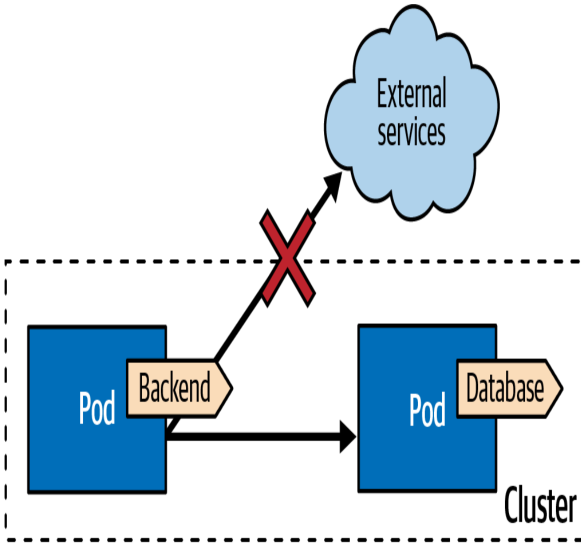
Figure 24-2. NetworkPolicy that allows only internal egress traffic
