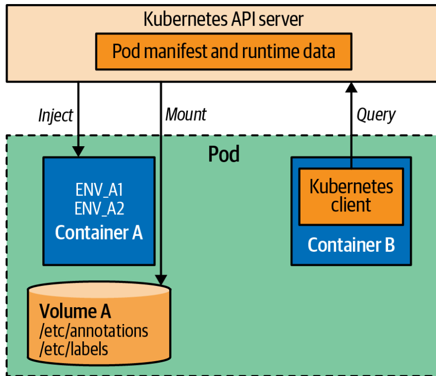
Figure 14-1. Application introspection mechanisms
