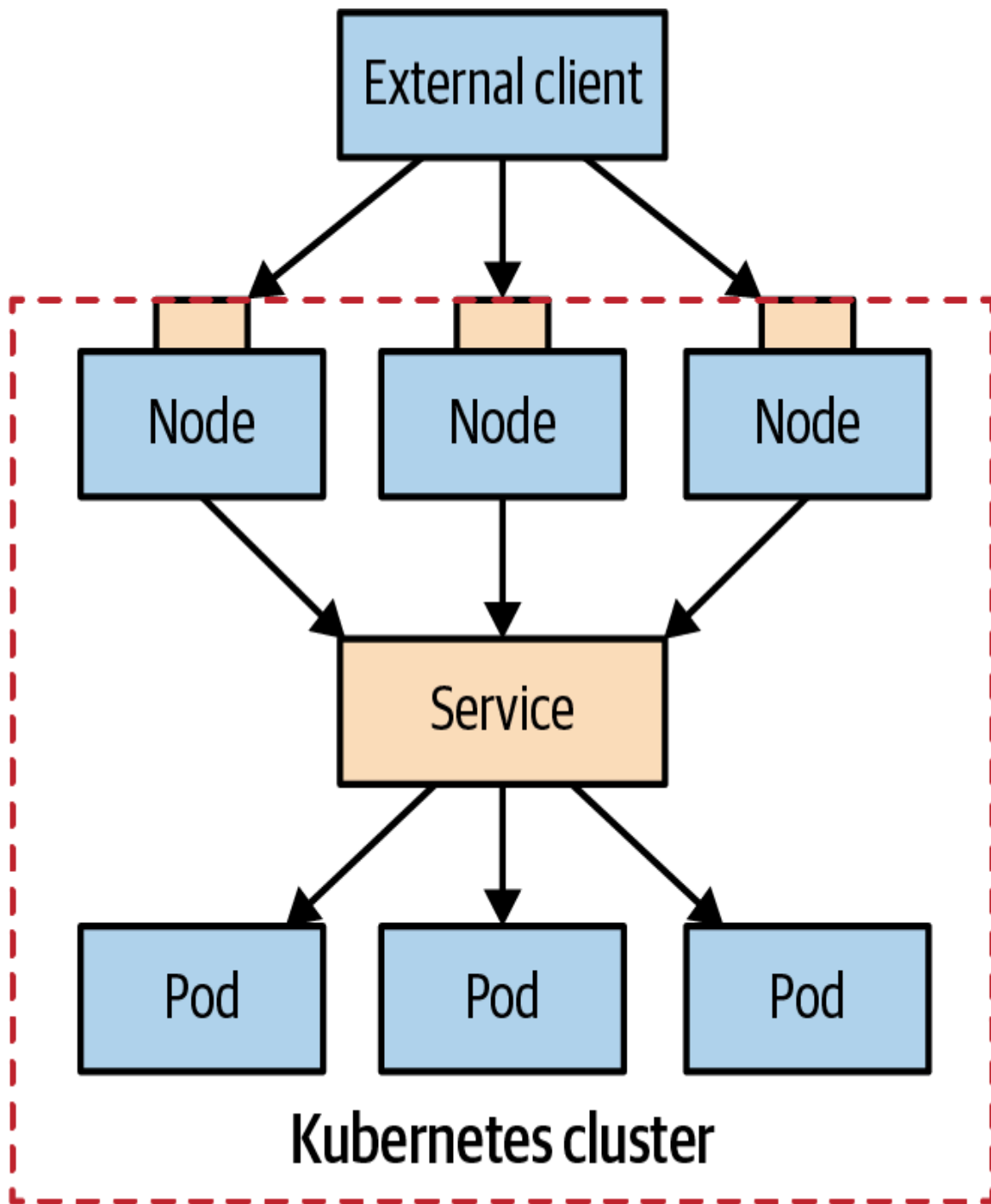
Figure 13-5. Node port service discovery
