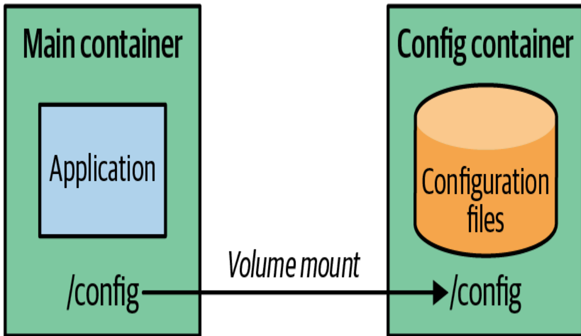
Figure 21-1. Immutable configuration with Docker volume
