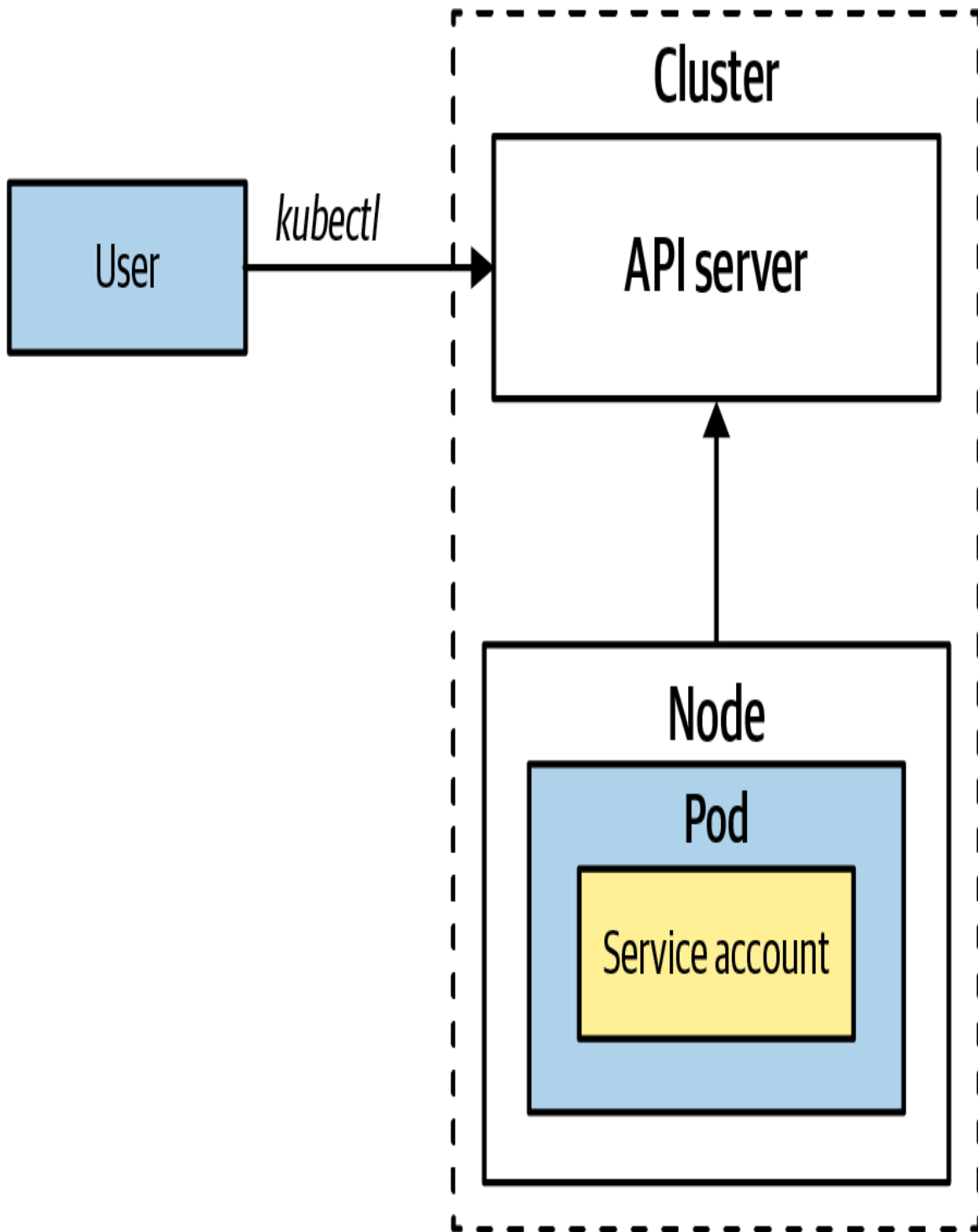
Figure 26-2. Subject (user or service account) requests to API Server
