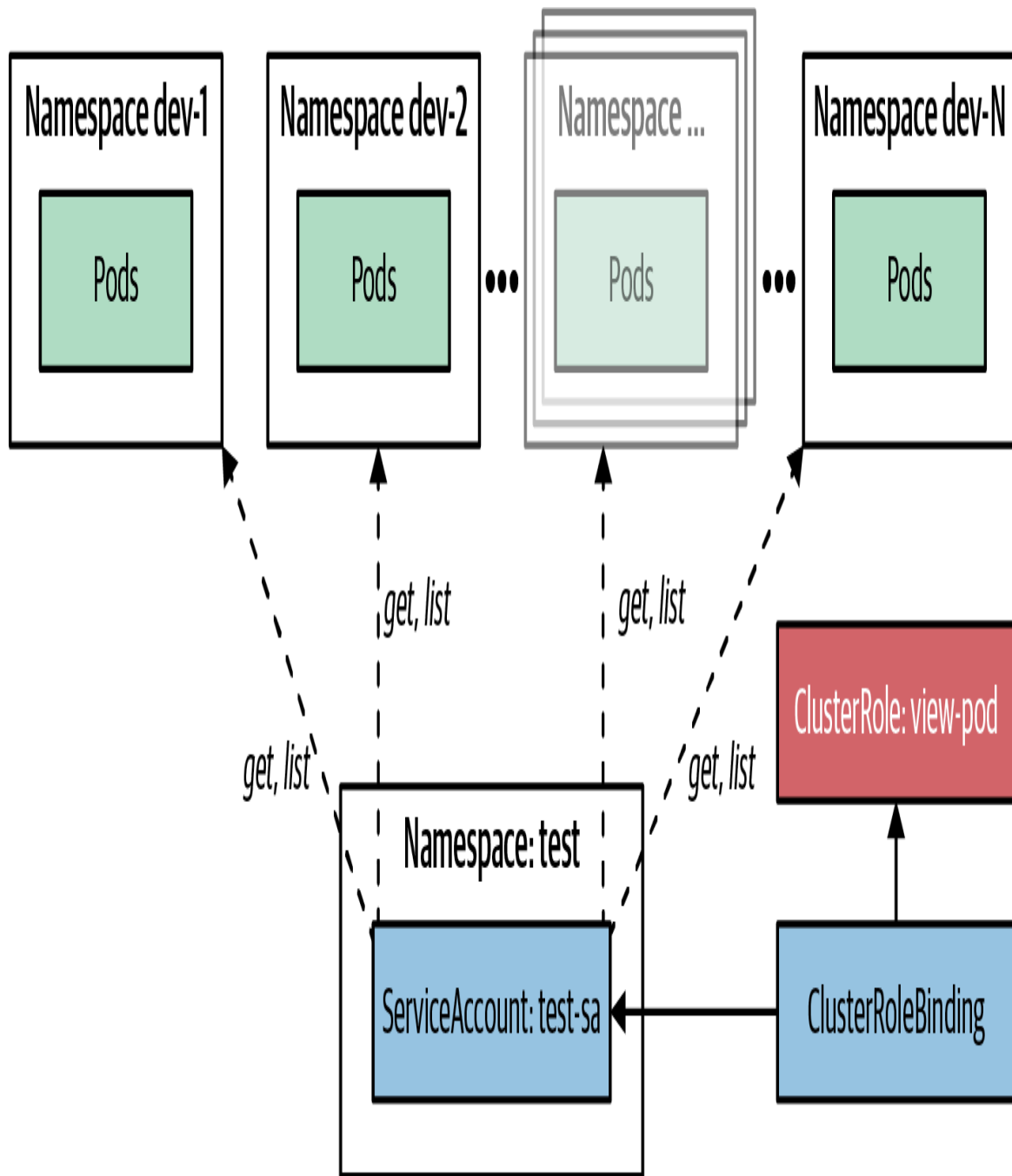
Figure 26-5. ClusterRoleBinding for reading all Pods
