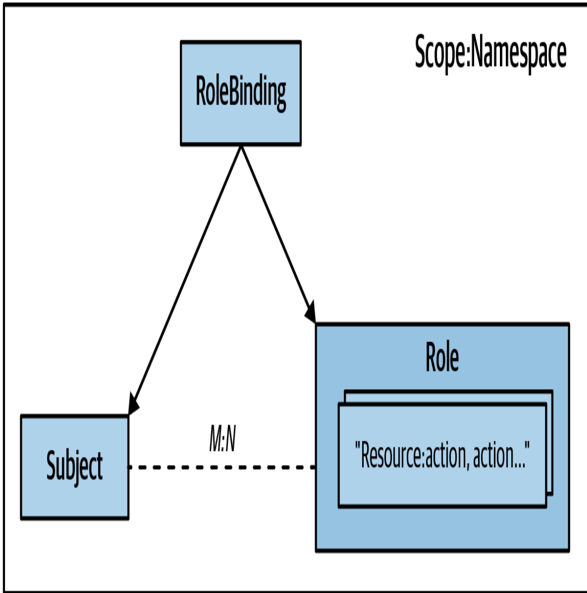
Figure 26-3. Relationship between Role, RoleBinding, and subjects
