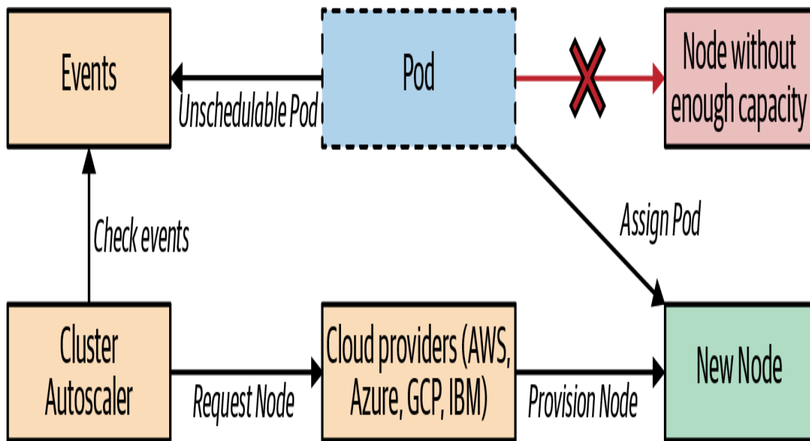
Figure 29-5. Cluster autoscaling mechanism
