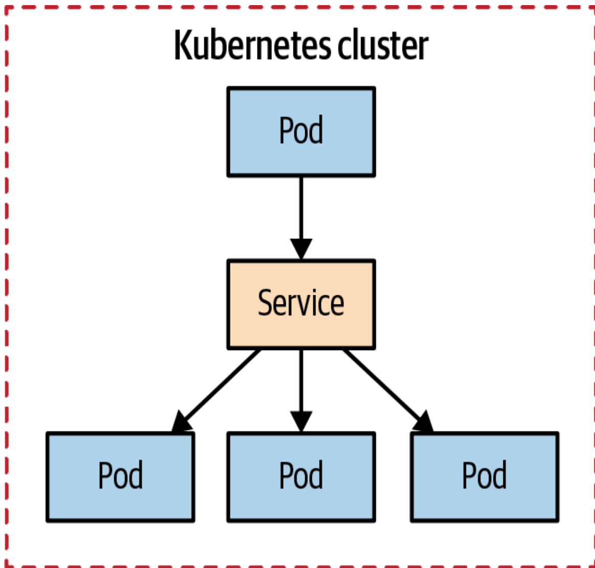
Figure 13-3. Internal service discovery
