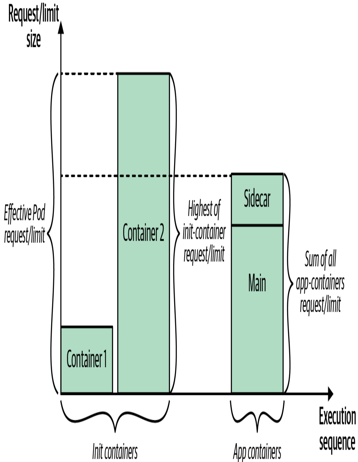
Figure 15-2. Effective Pod request/limit calculation
