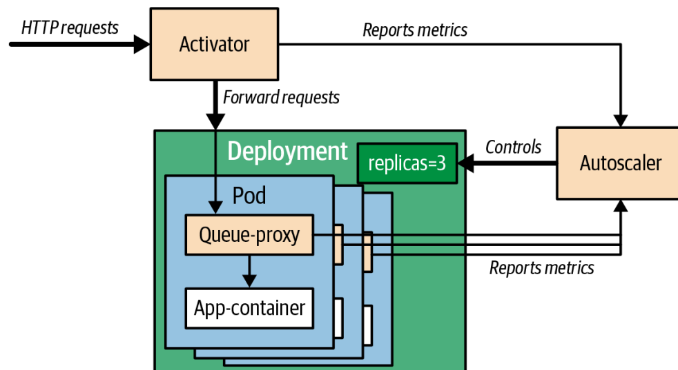
Figure 29-2. Knative Pod Autoscaler
