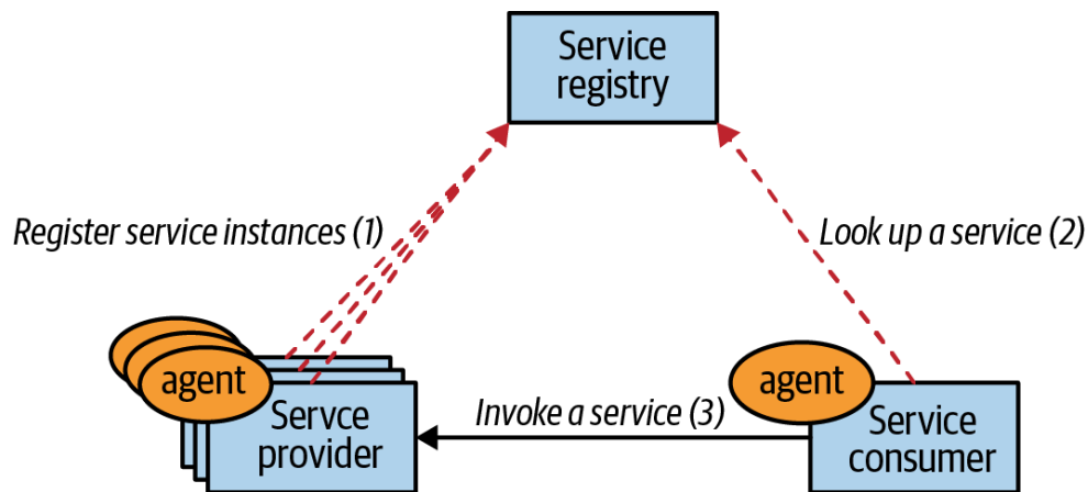
Figure 13-1. Client-side service discovery
