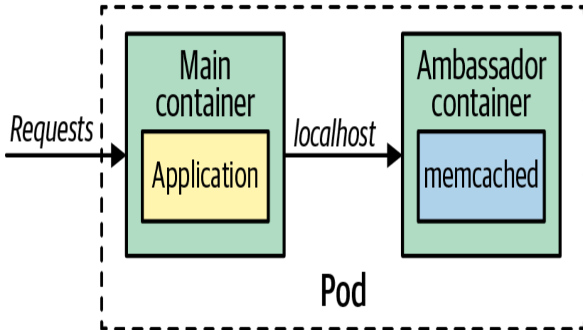
Figure 18-2. Ambassador for accessing a local cache
