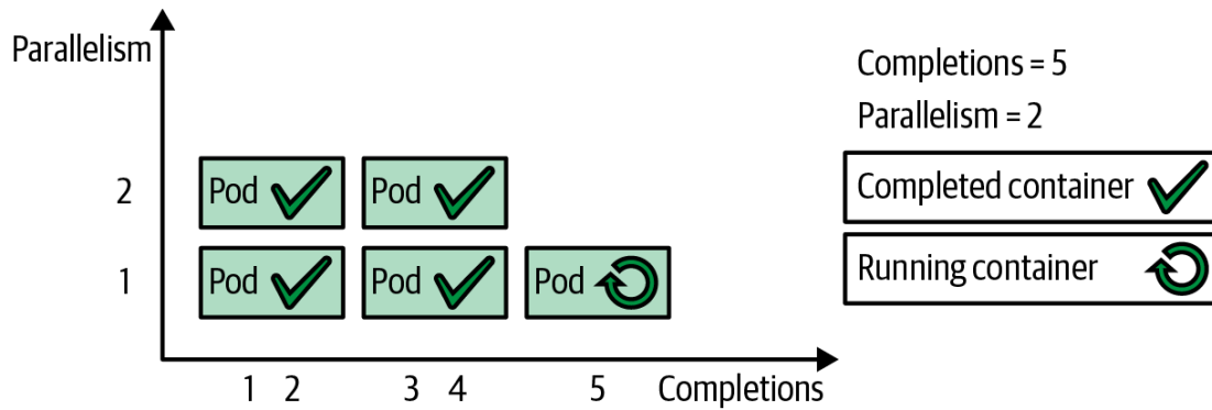
Figure 7-1. Parallel Batch Job with a fixed completion count
