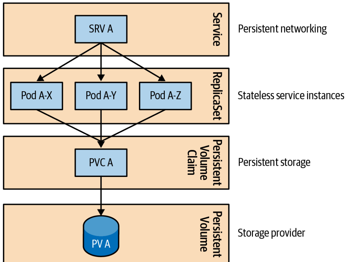
Figure 11-1. A distributed stateless application on Kubernetes
