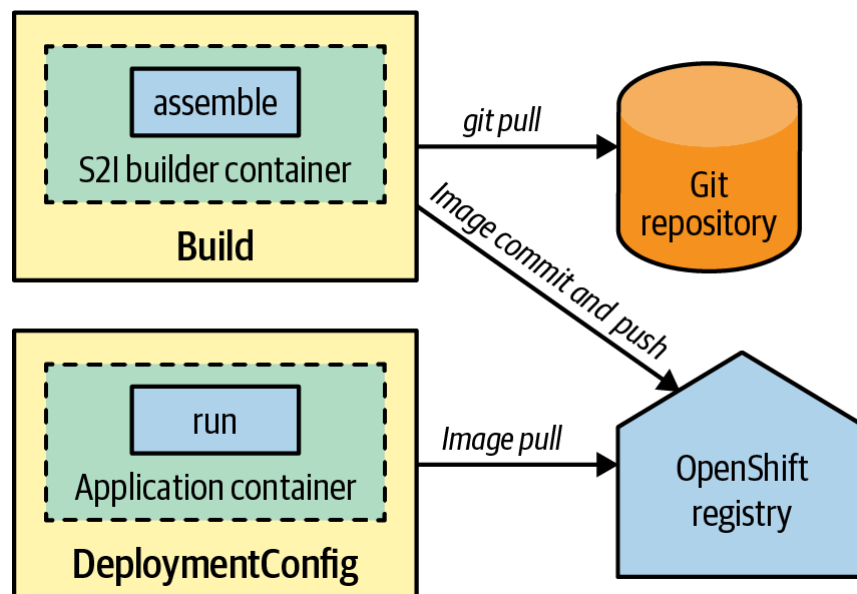
Figure 30-3. S2I build with Git source as input
