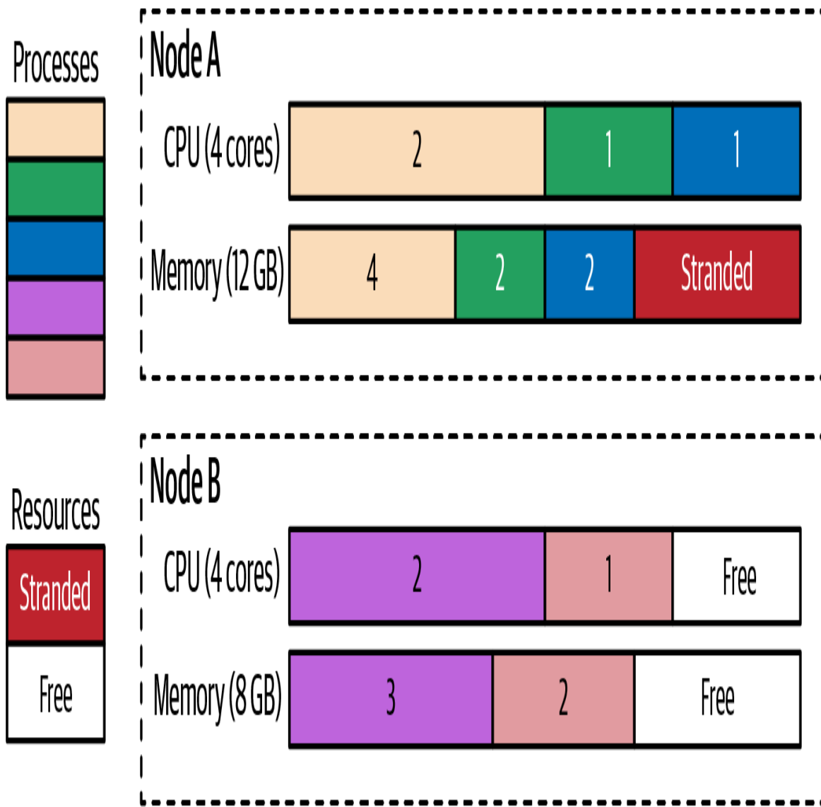
Figure 6-2. Processes scheduled to nodes and stranded resources
