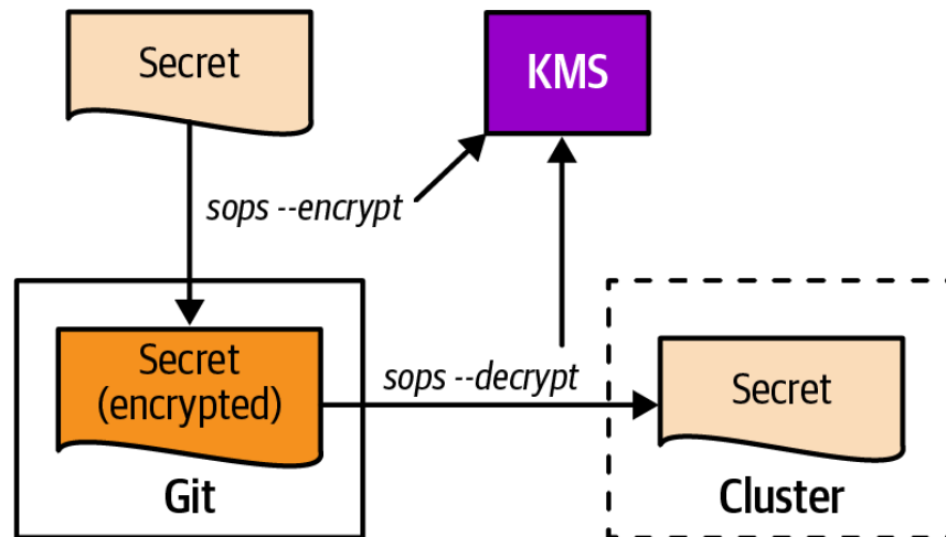
Figure 25-3. Sops for decrypting and encrypting resource files
