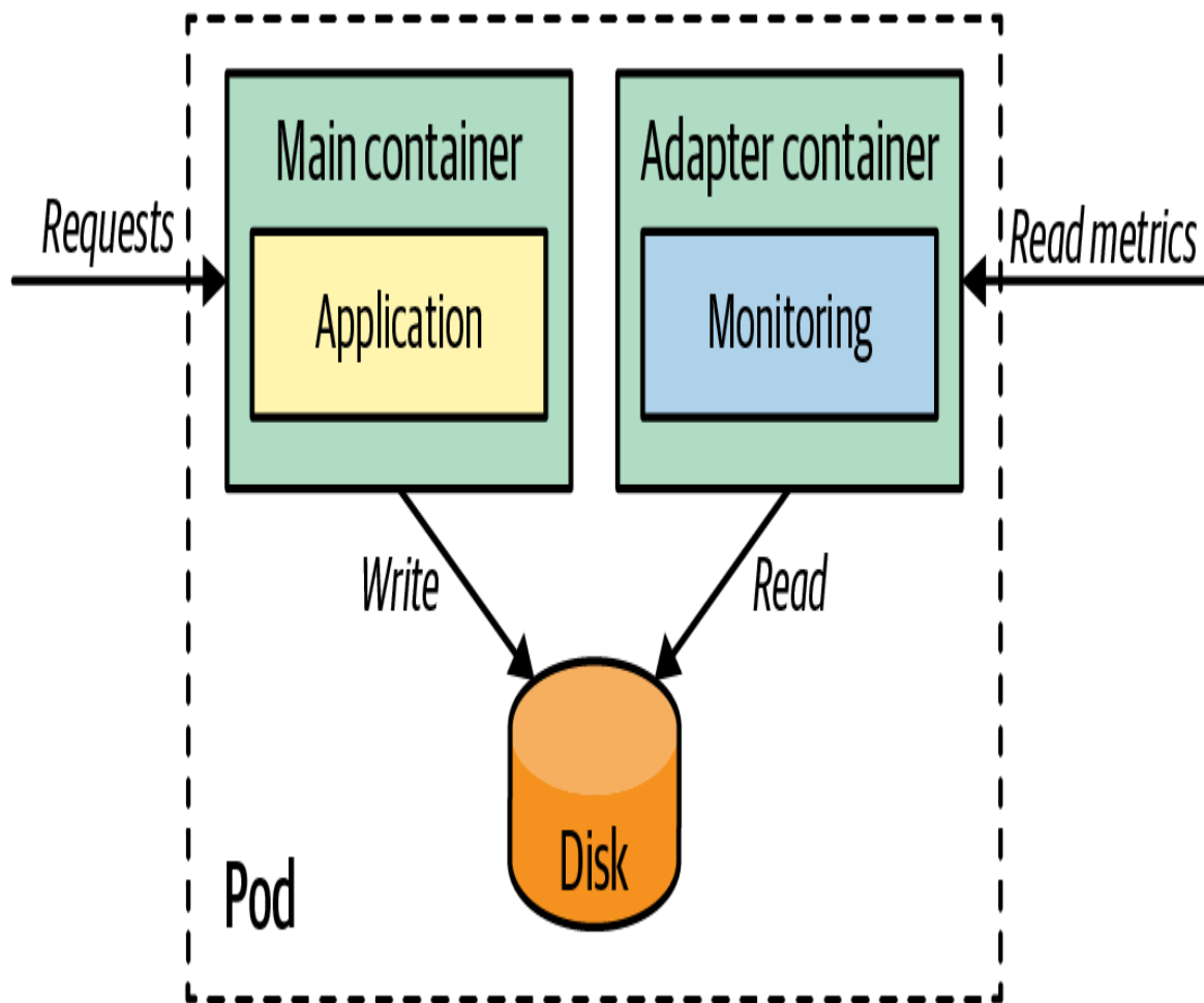
Figure 17-1. Adapter pattern
