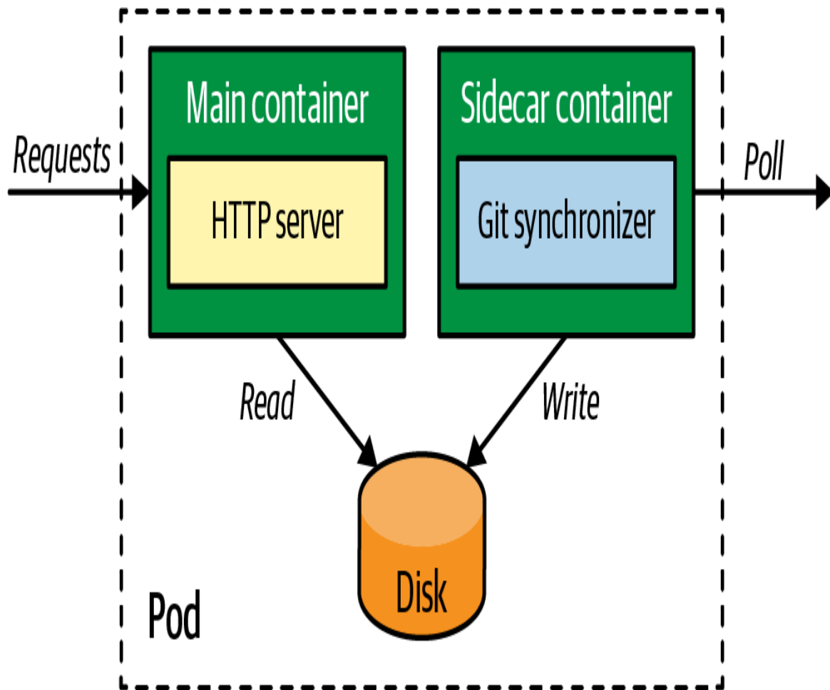
Figure 16-1. Sidecar pattern
