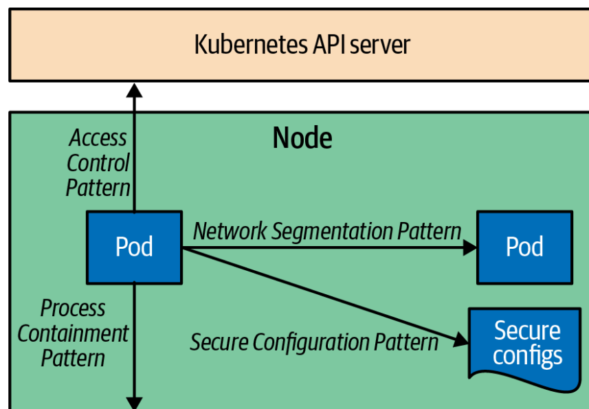
Figure V-1. Security patterns
