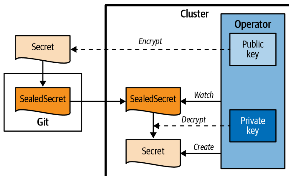
Figure 25-1. Sealed Secrets
