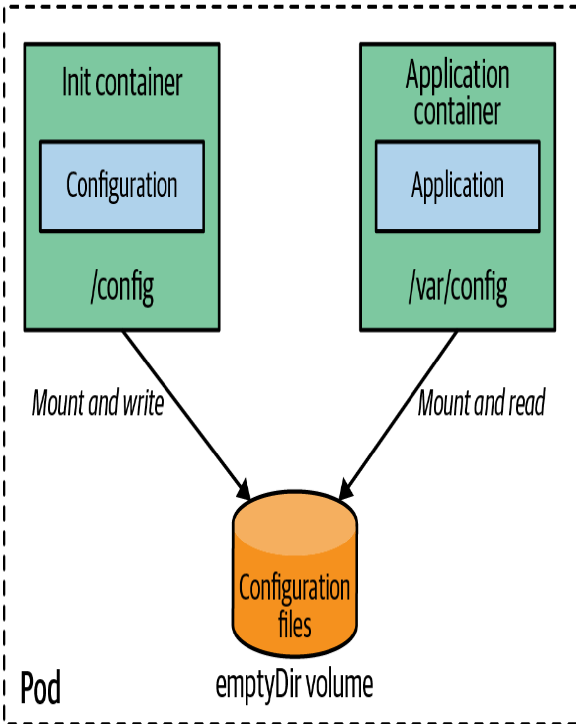
Figure 21-2. Immutable configuration with an init container
