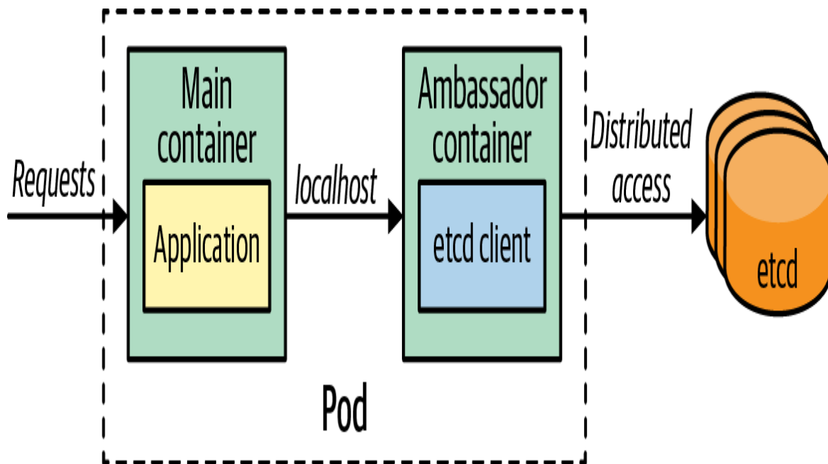
Figure 18-1. Ambassador for accessing a remote distributed cache
