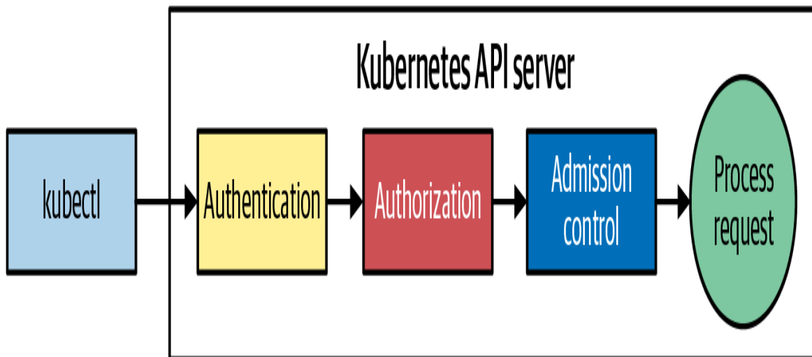
Figure 26-1. A request to the Kubernetes API server must pass through these stages
