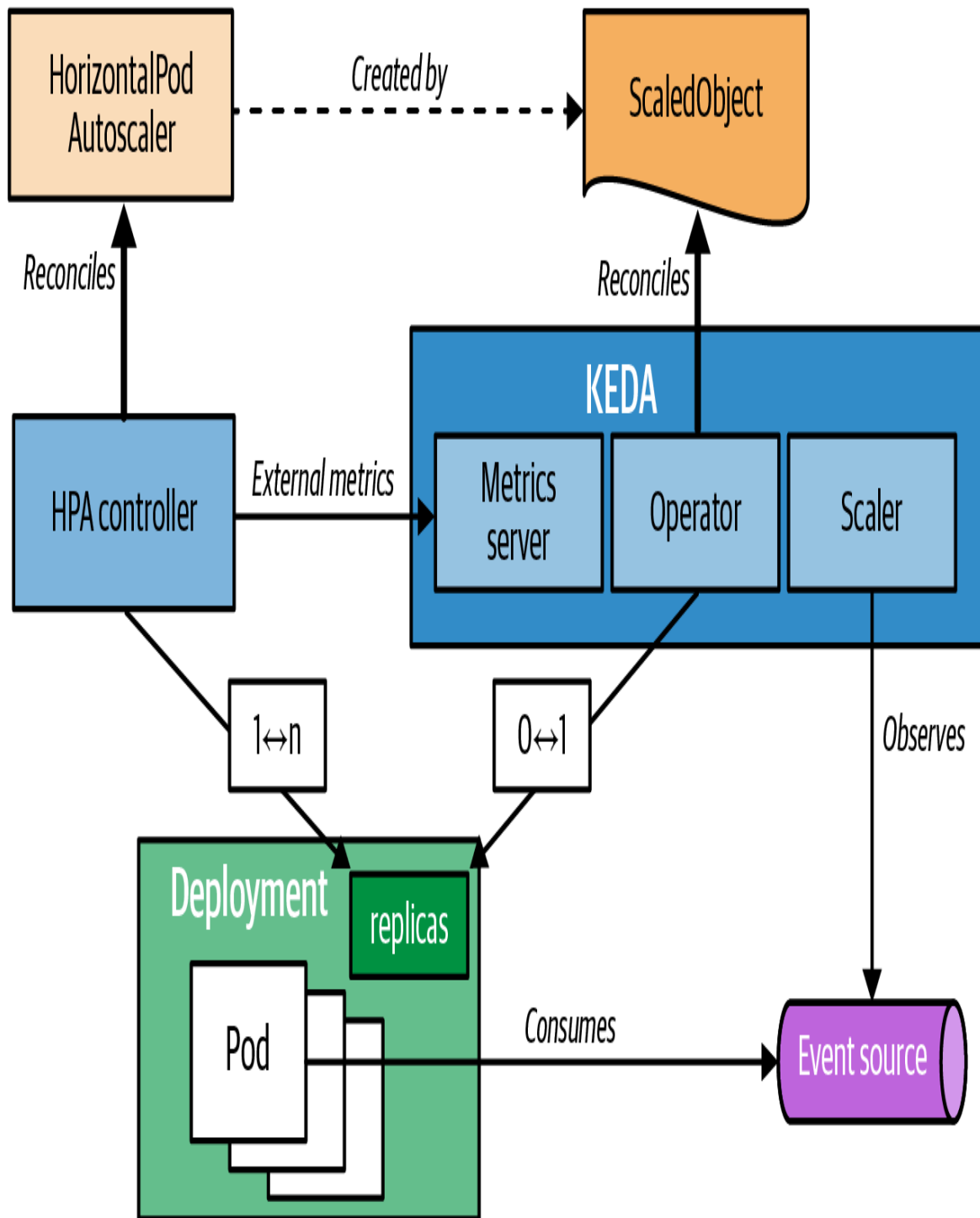
Figure 29-3. KEDA autoscaling components
