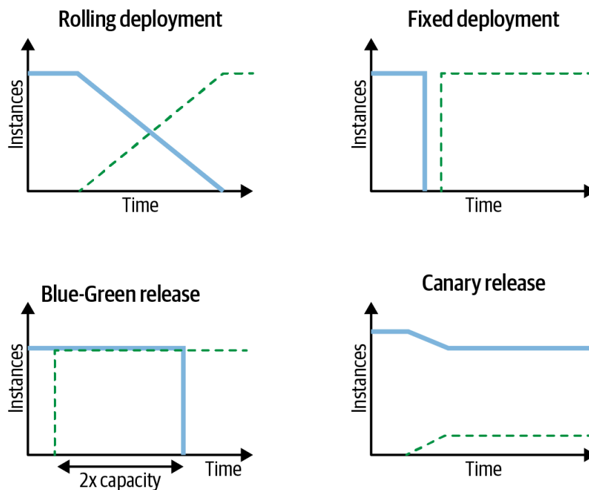
Figure 3-5. Deployment and release strategies
