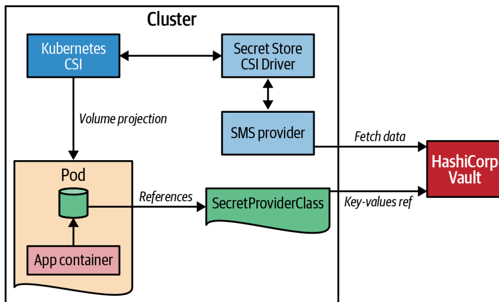
Figure 25-4. Secrets Store CSI Driver
