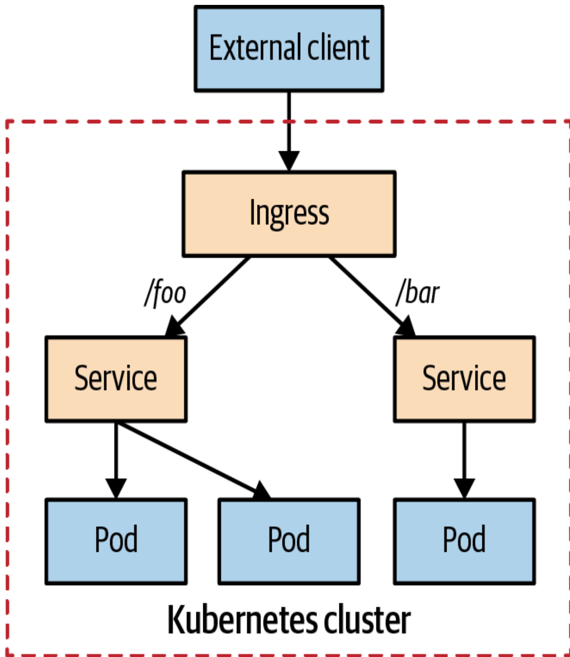
Figure 13-7. Application layer service discovery
