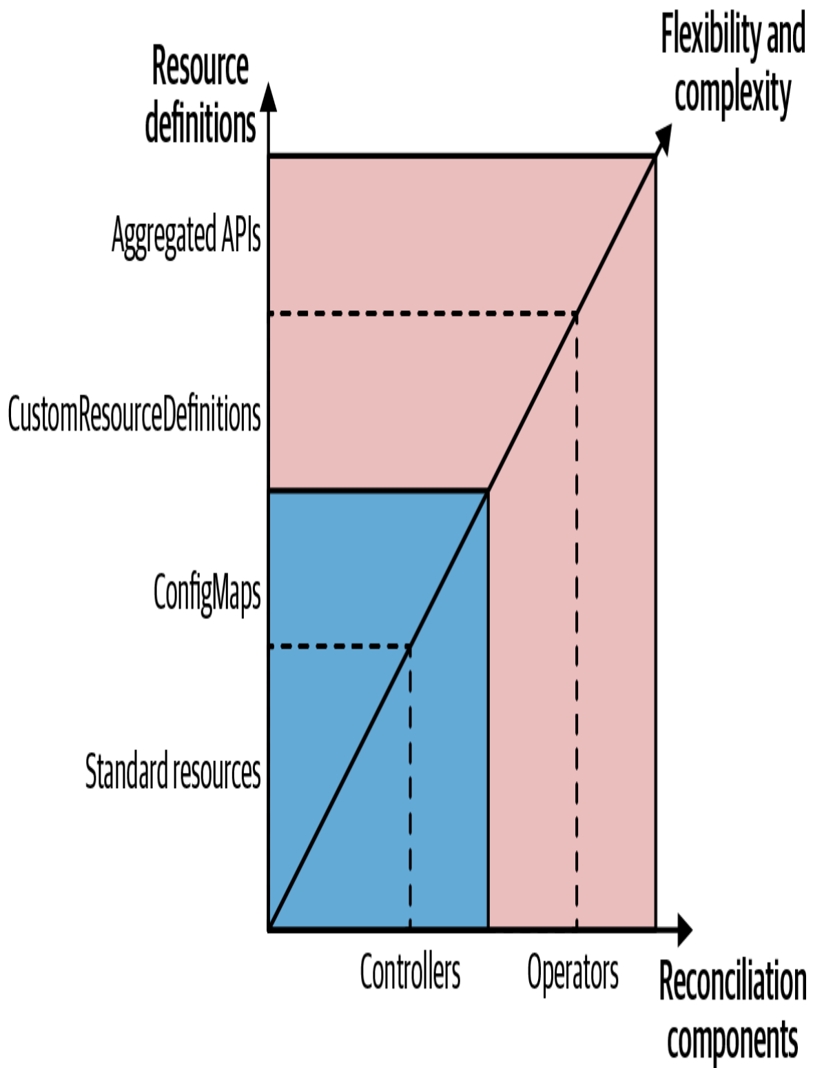
Figure 28-1. Spectrum of controllers and operators
