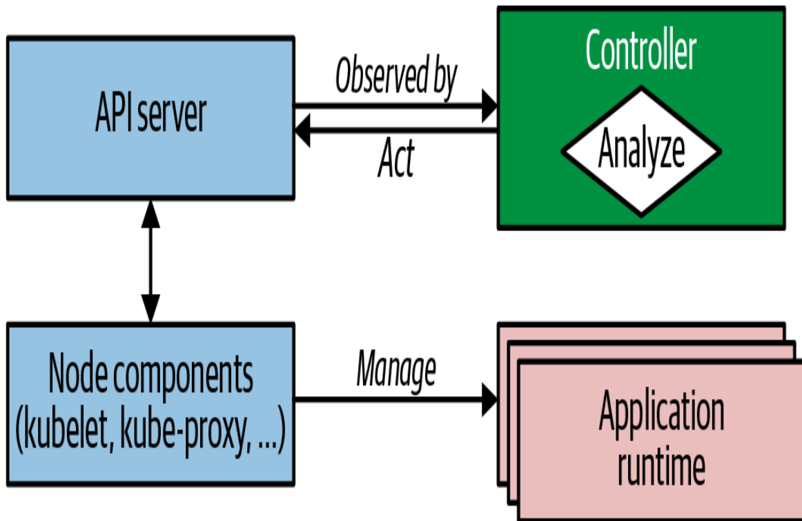
Figure 27-1. Observe-Analyze-Act cycle
