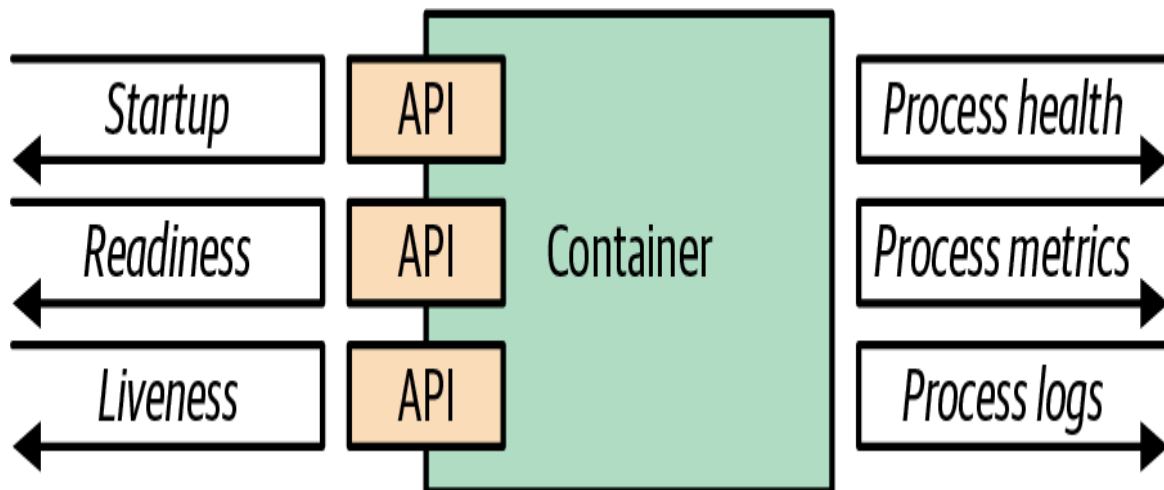
Figure 4-1. Container observability options
