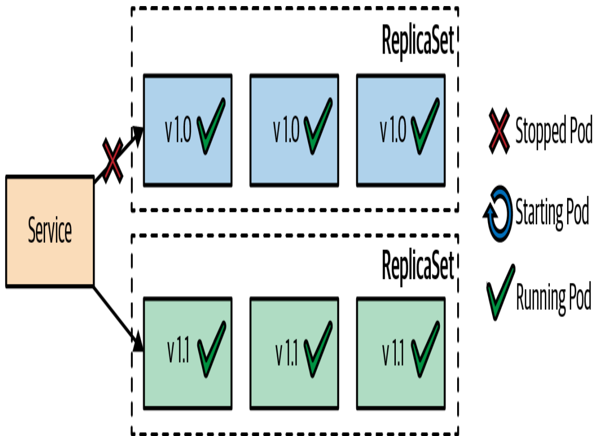
Figure 3-3. Blue-Green release
