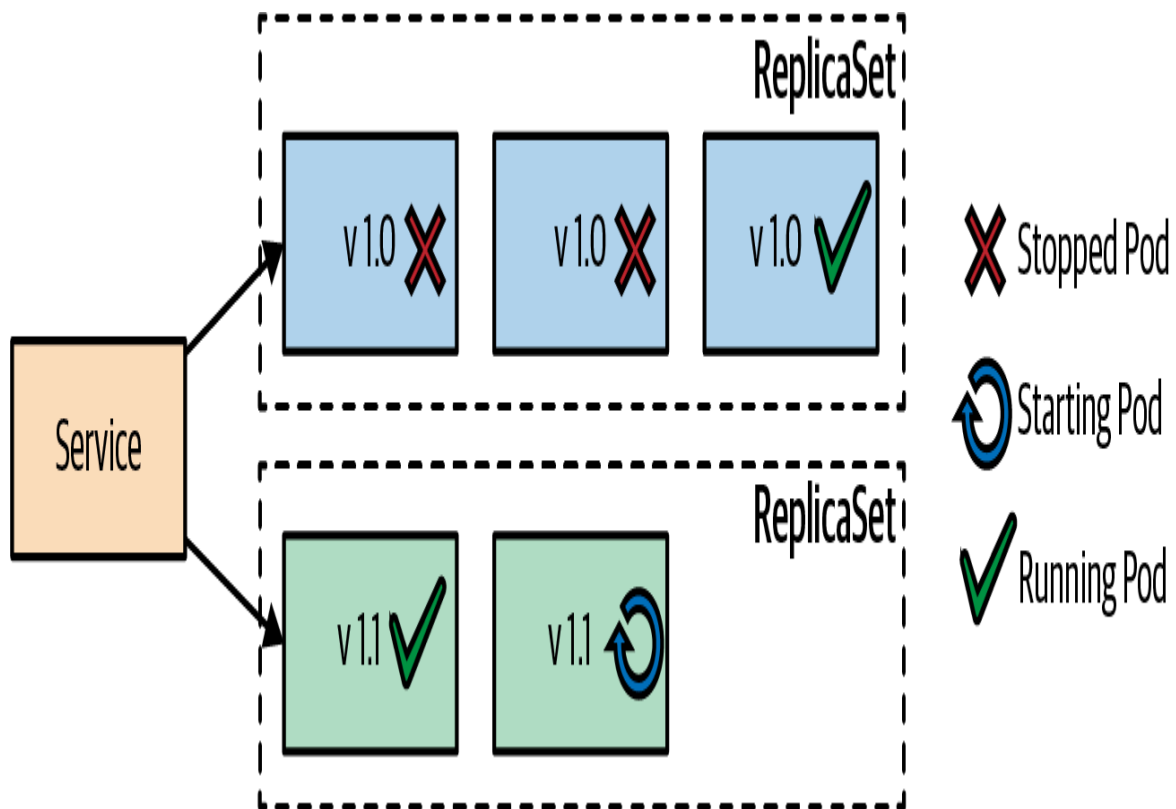
Figure 3-1. Rolling deployment
