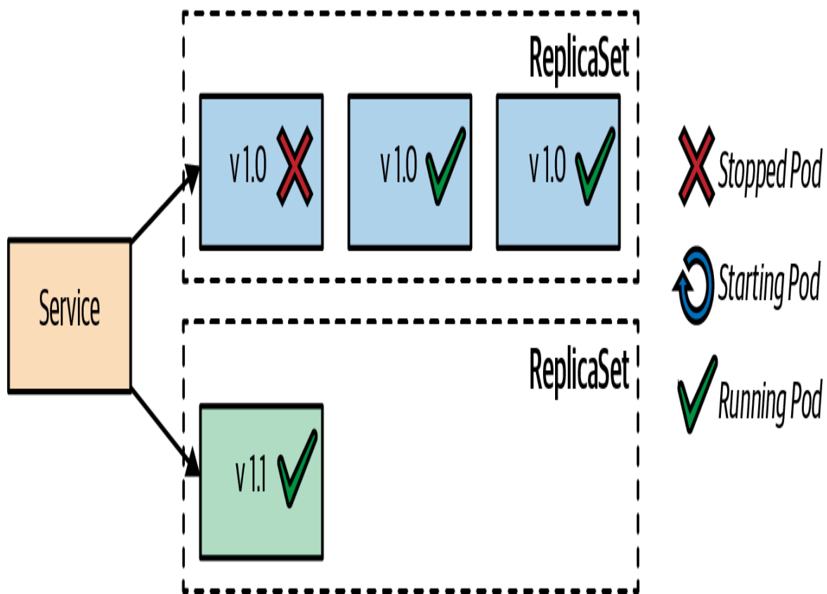
Figure 3-4. Canary release
