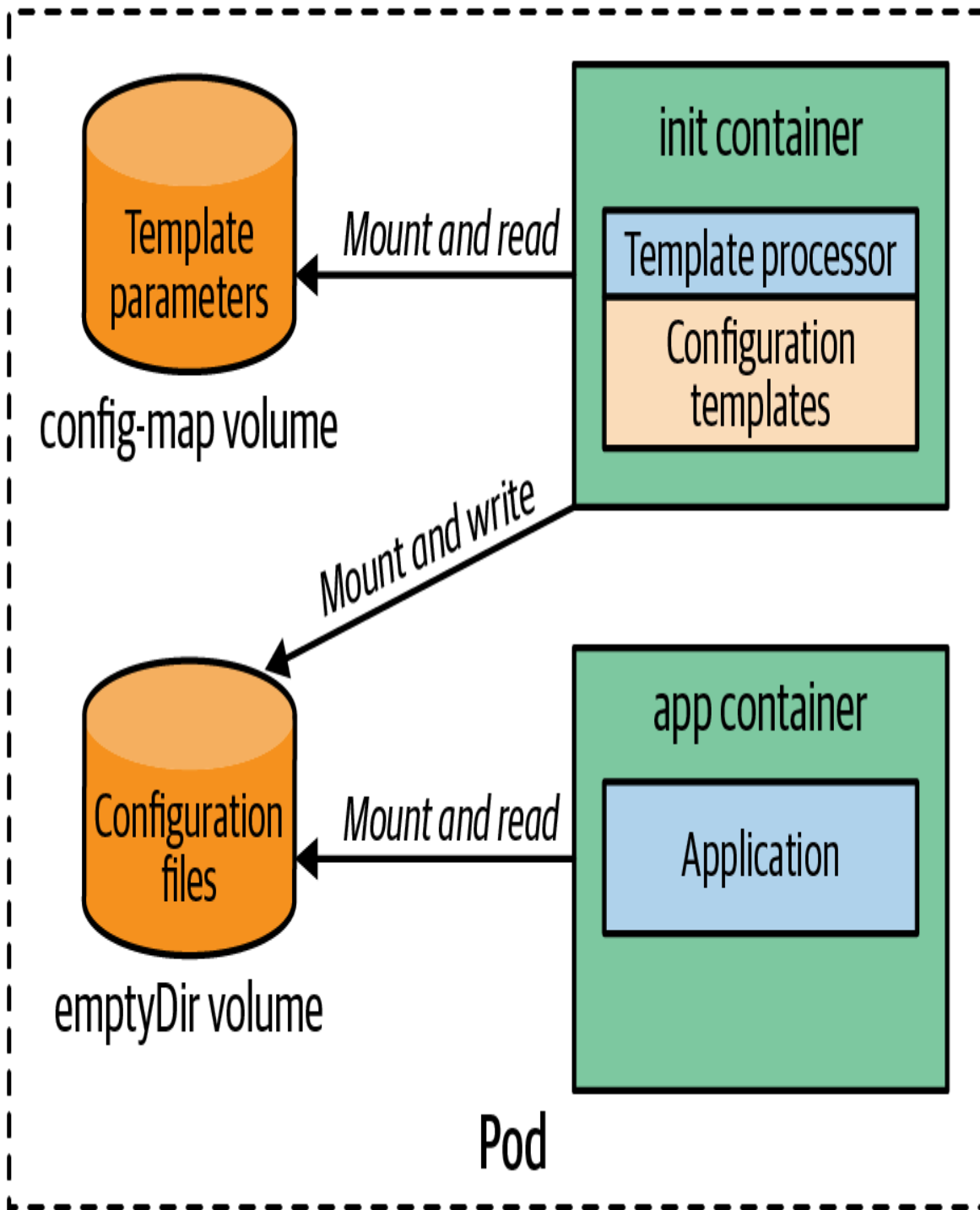
Figure 22-1. Configuration template
