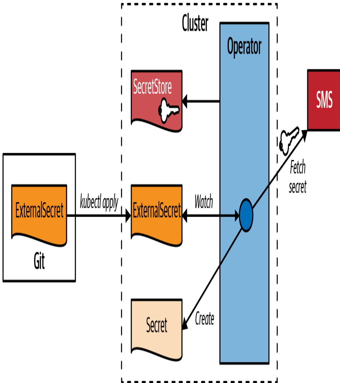
Figure 25-2. External Secrets
