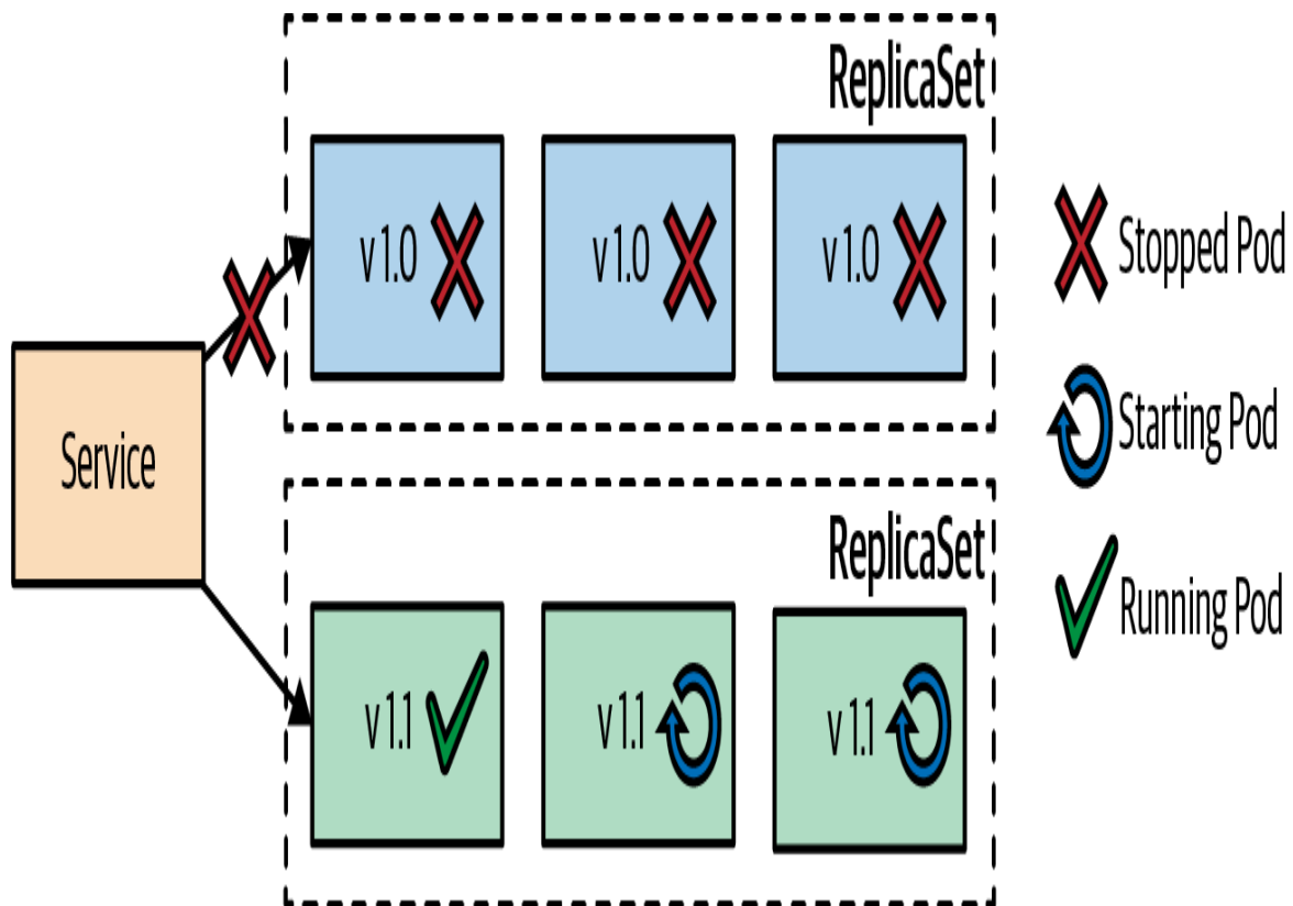
Figure 3-2. Fixed deployment using a Recreate strategy
