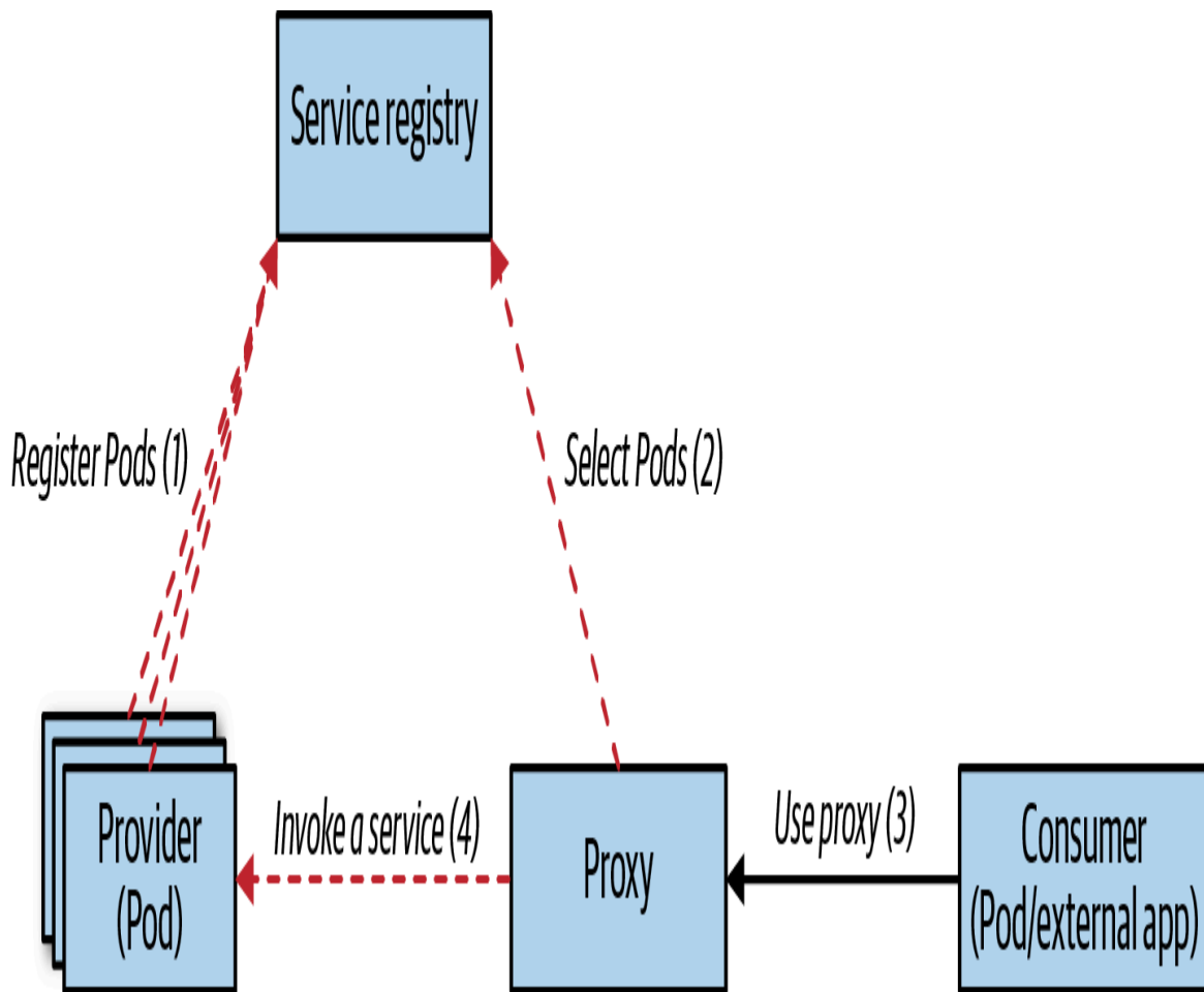
Figure 13-2. Server-side service discovery
