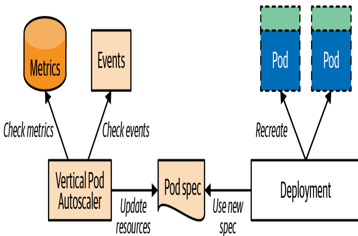
Figure 29-4. Vertical Pod autoscaling mechanism
