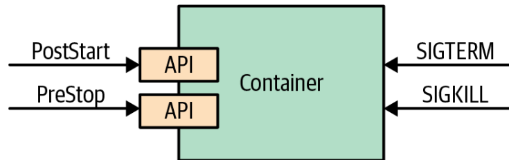
Figure 5-1. Managed container lifecycle
