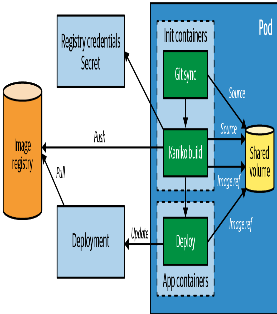
Figure 30-2. In-cluster container image build with a build Pod
