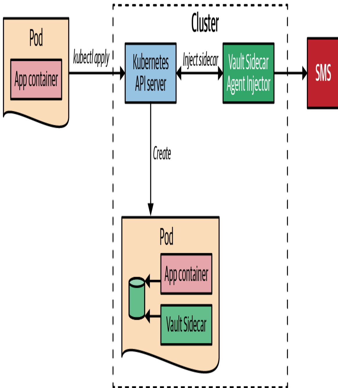
Figure 25-5. Vault Injector
