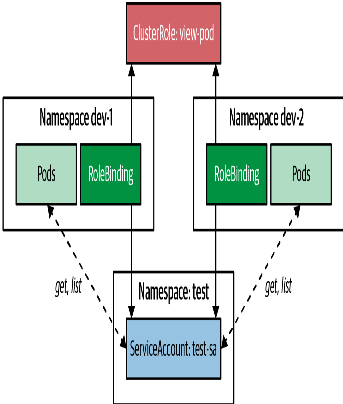
Figure 26-4. Sharing a ClusterRole in multiple namespaces
