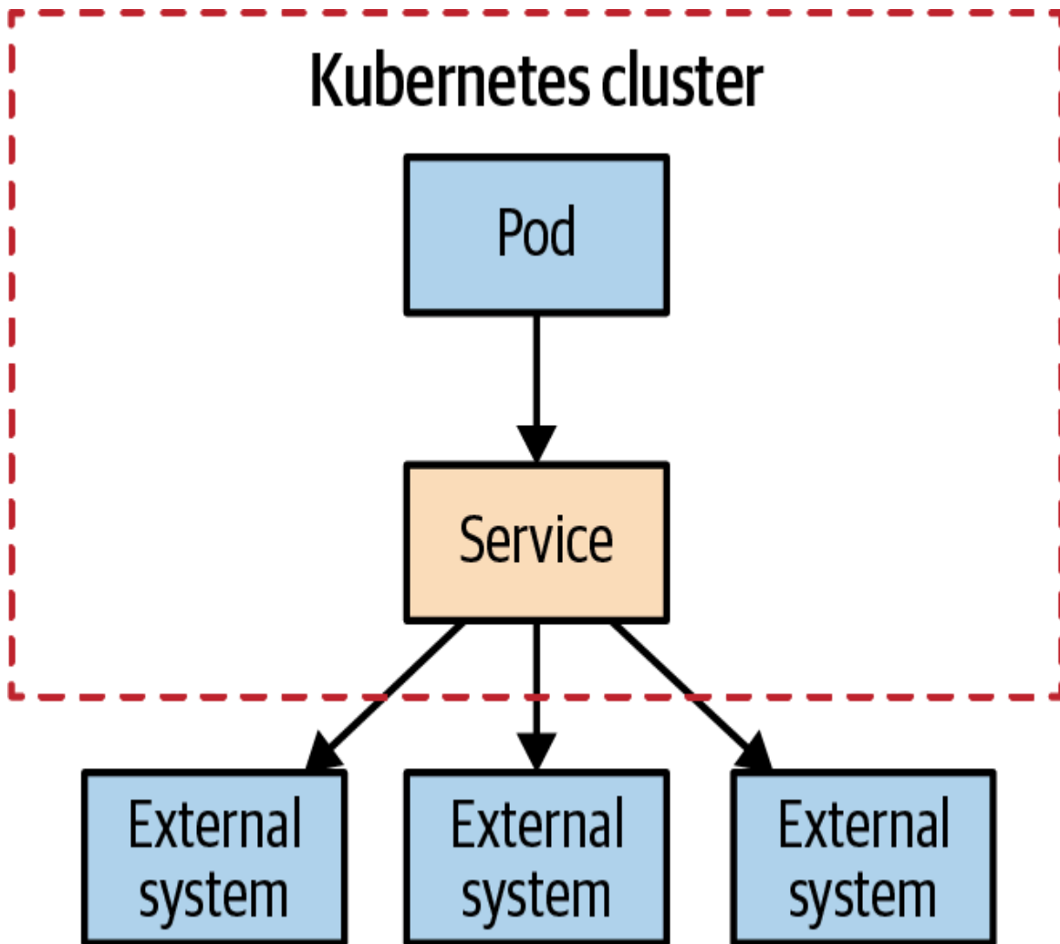
Figure 13-4. Manual service discovery
