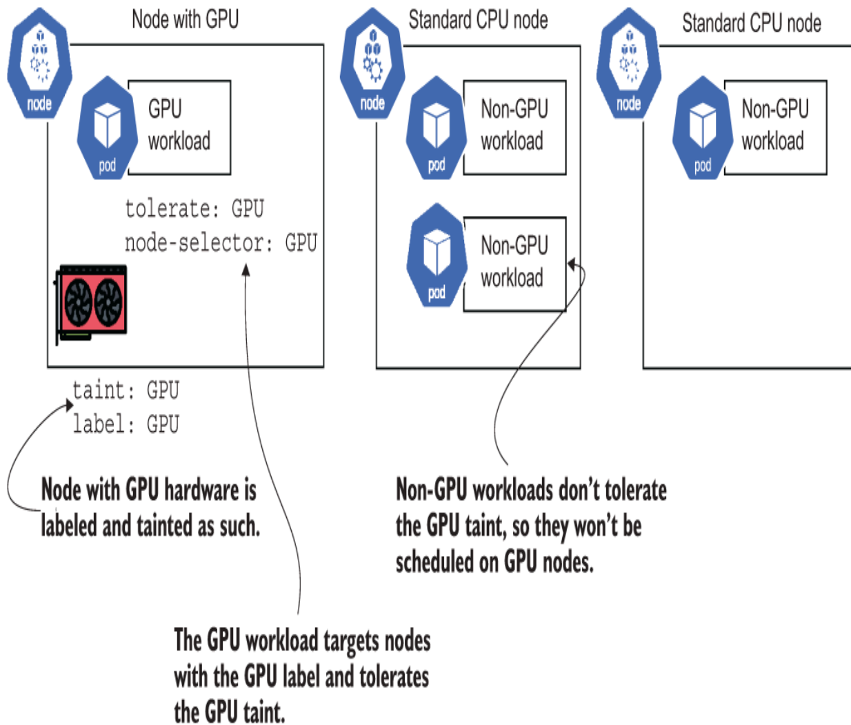
Figure 8.2 This cluster has a special node with a GPU and two standard nodes. The GPU node is tainted to prevent standard workloads from being scheduled on it. The GPU workload tolerates the taint so it can be scheduled on the GPU node and uses a node selector to ensure it is only scheduled on this node.
