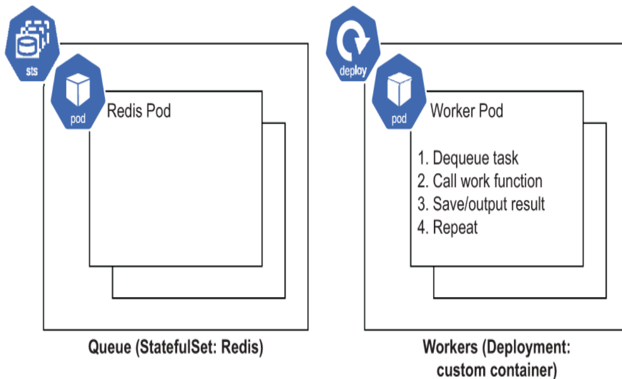
Figure 10.2 Kubernetes architecture of the background processing task queue
