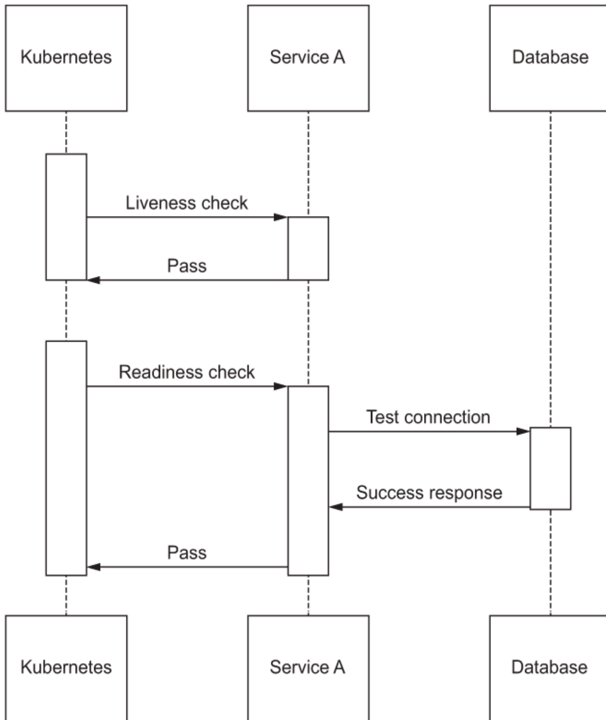
Figure 4.1 Liveness and readiness checks and external dependencies
