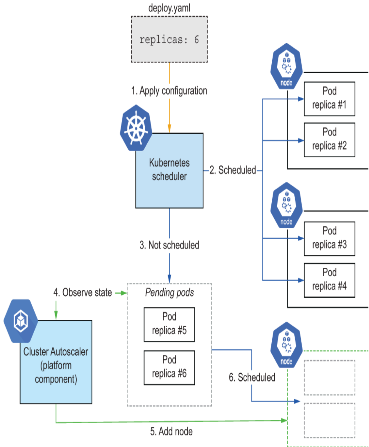
Figure 6.1 The Cluster Autoscaler watches for pending Pods and creates new nodes if needed.
