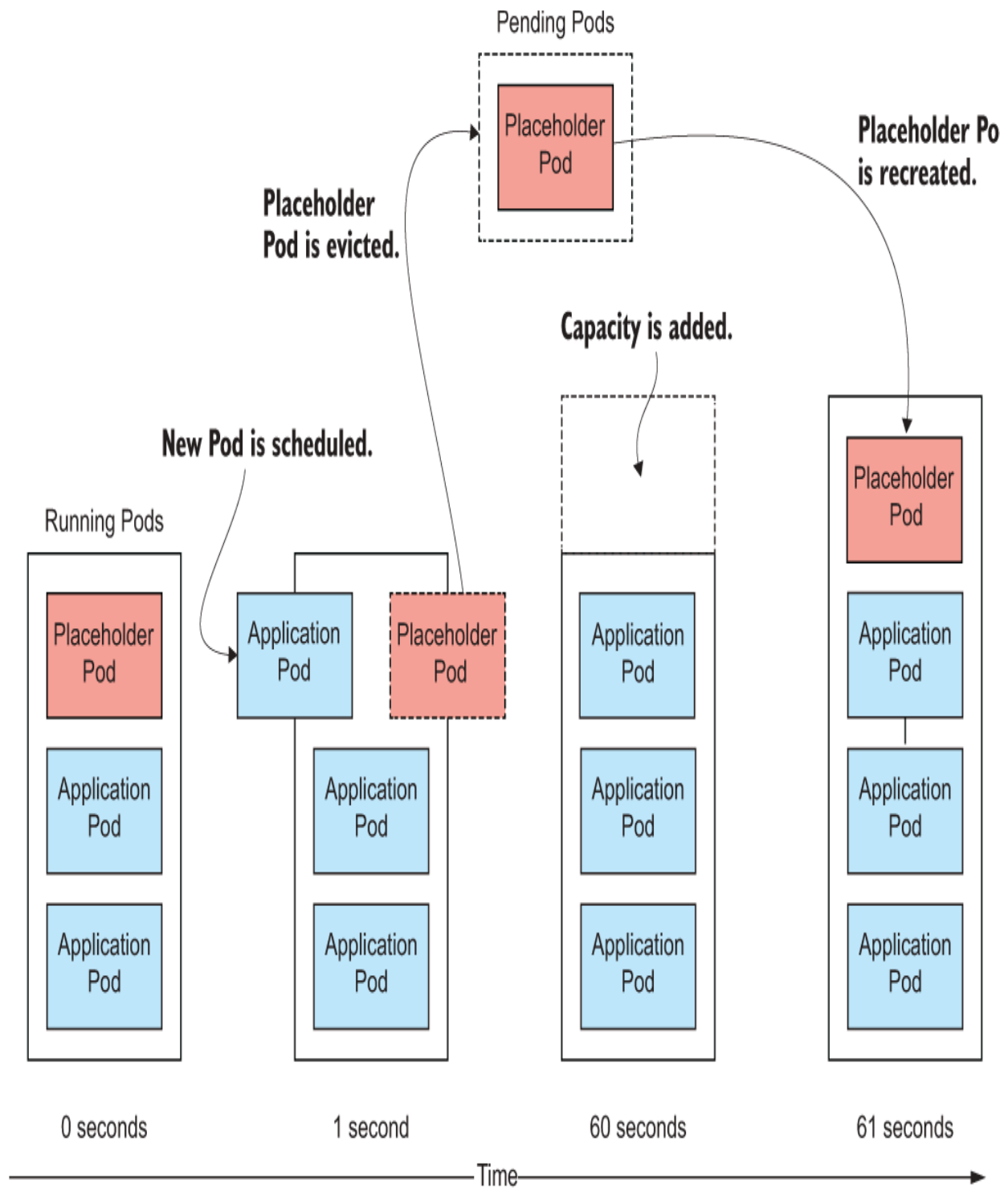
Figure 6.3 Autoscaling with a placeholder Pod, allowing for rapid booting of new Pods using spare capacity
