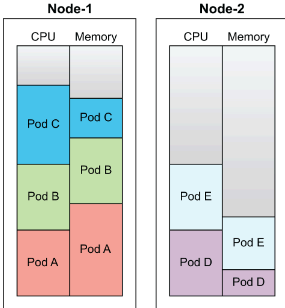
Figure 5.3 Five containers allocated on two nodes based on their resource needs
