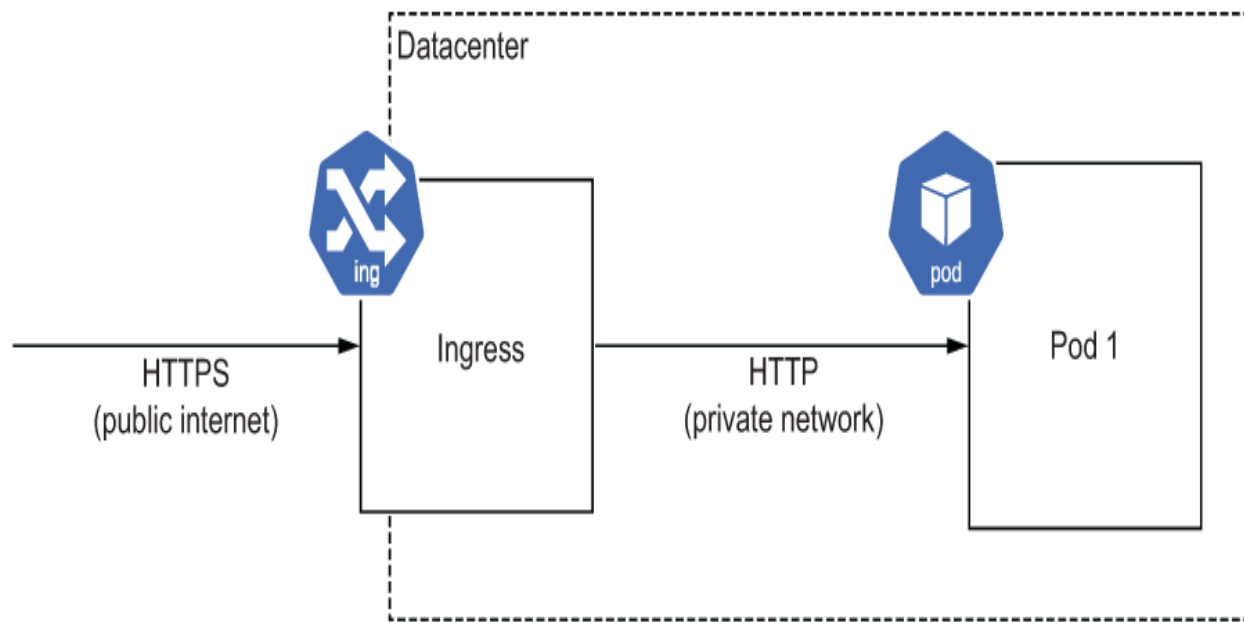
Figure 7.5 The Ingress terminates HTTPS (TLS) traffic and can forward it to the serving Pods over plain HTTP or HTTPS connections.
