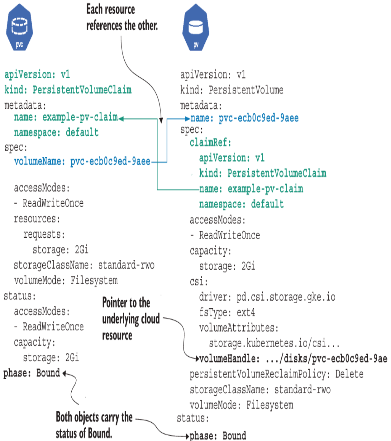
Figure 9.4 The PersistentVolumeClaim and PersistentVolume after the latter was provisioned, and they were bound together
