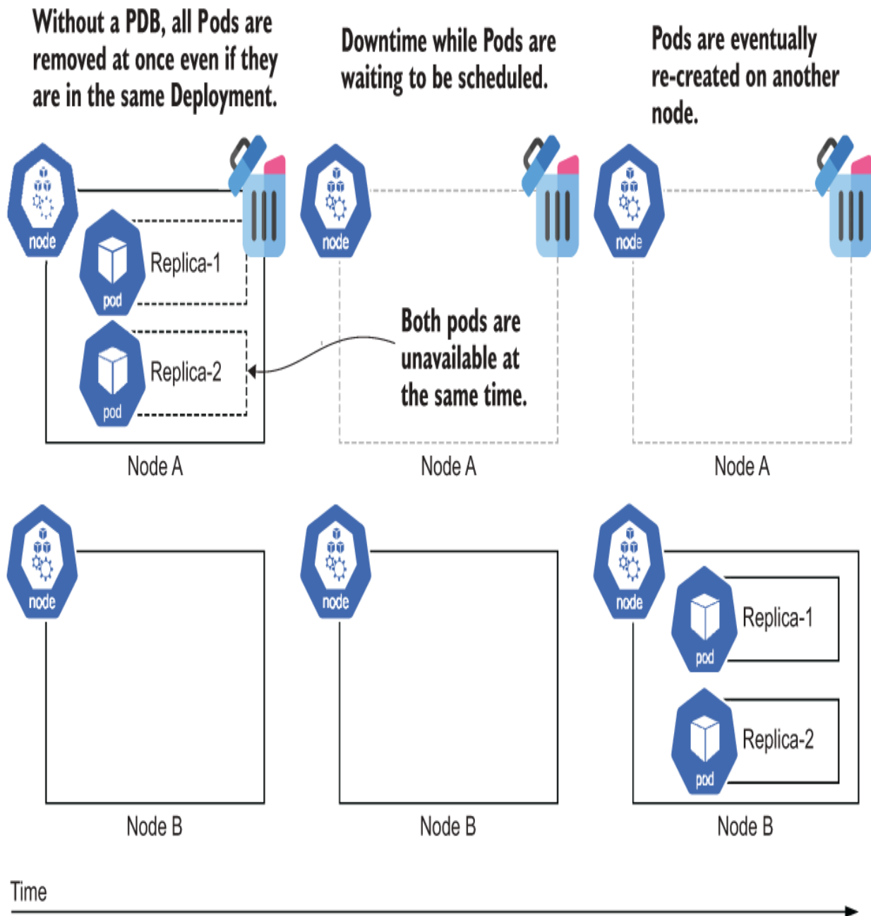
Figure 12.1 Node deletion without Pod disruption budgets. All the Pods on the node will become unavailable at once.
