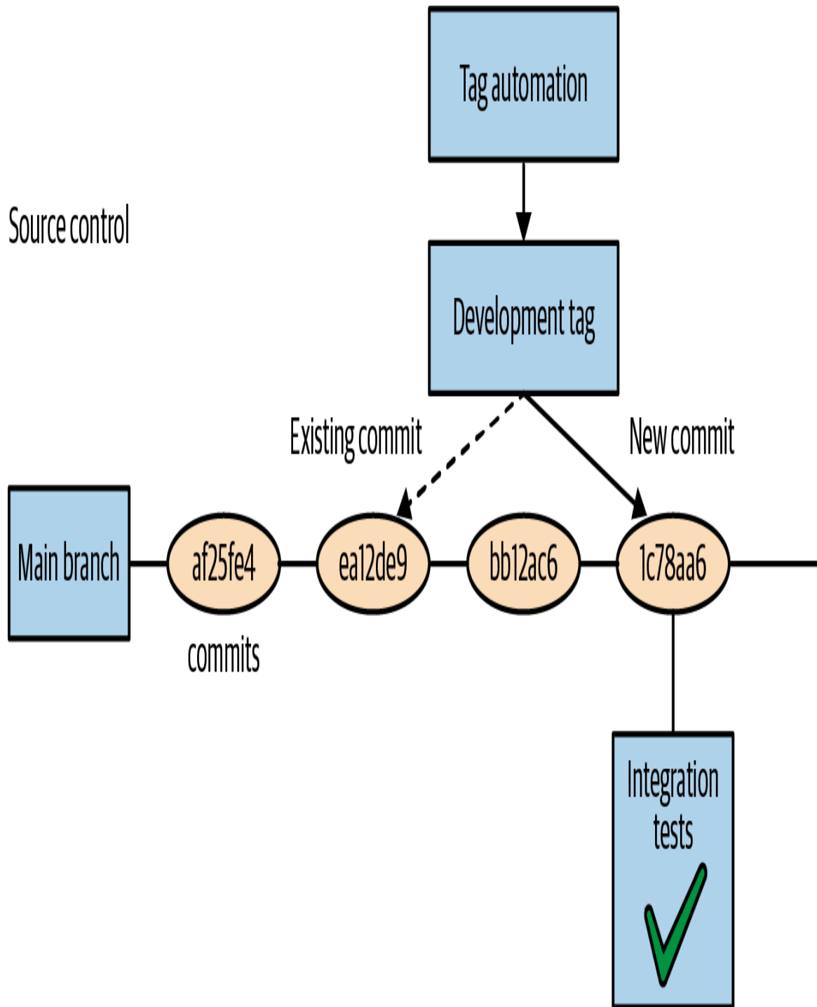
Figure 22-2. Development tag workflow
