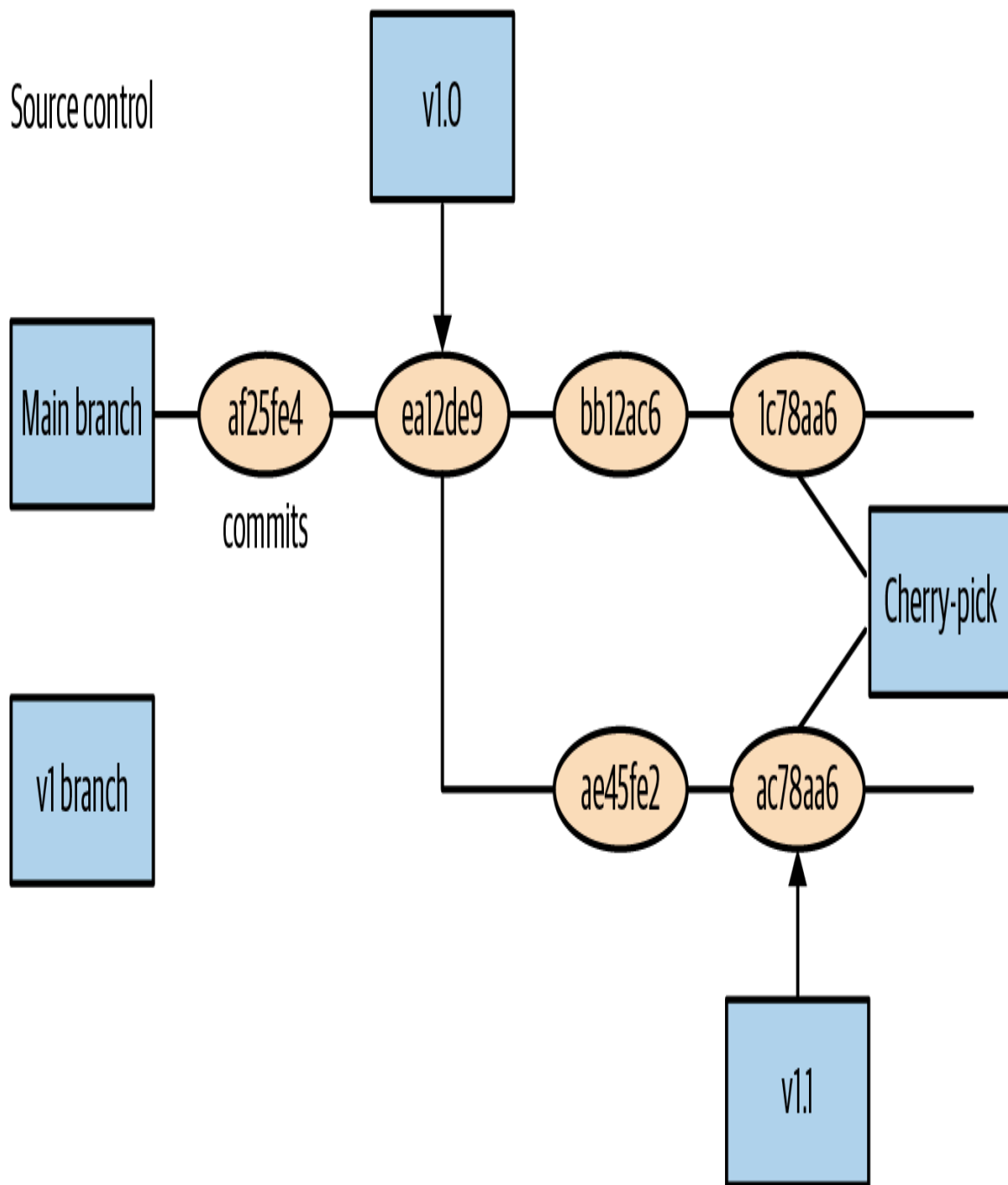
Figure 22-1. Cherry-pick workflow
