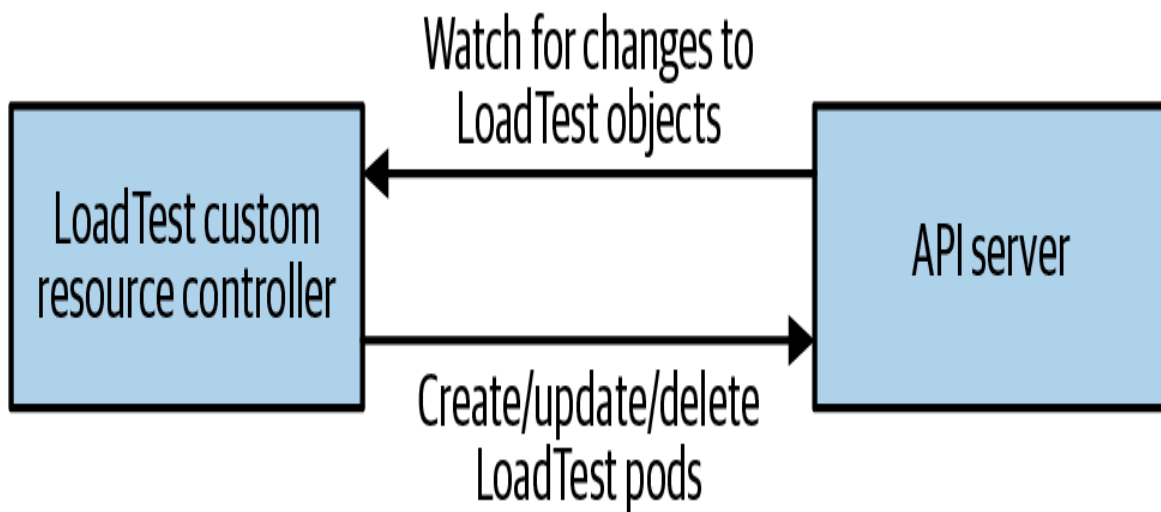
Figure 17-2. CustomResourceDefinition interactions
