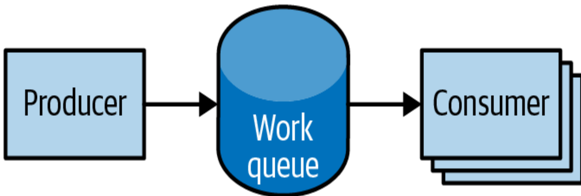
Figure 12-1. Parallel jobs
