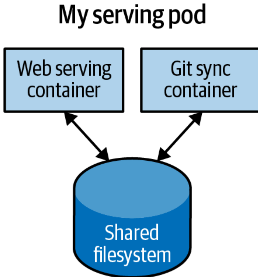
Figure 5-1. An example Pod with two containers and a shared filesystem
