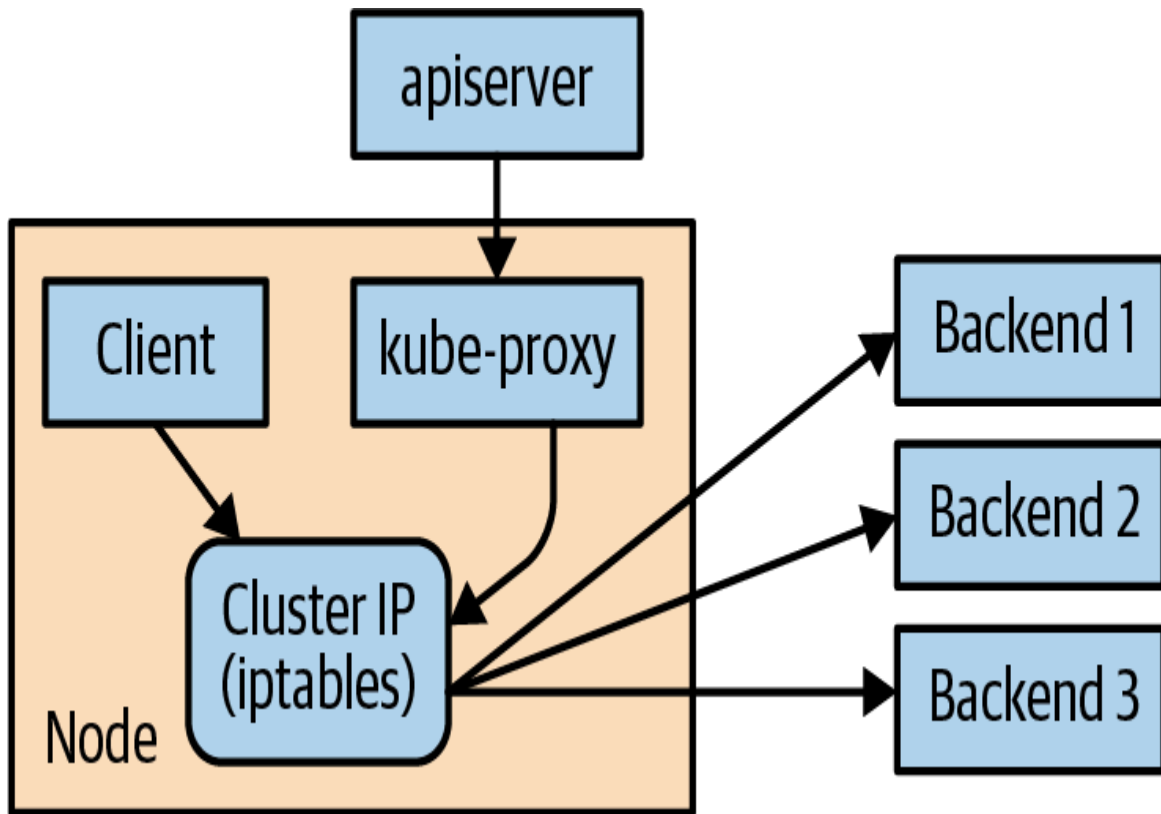
Figure 7-1. Configuring and using a cluster IP
