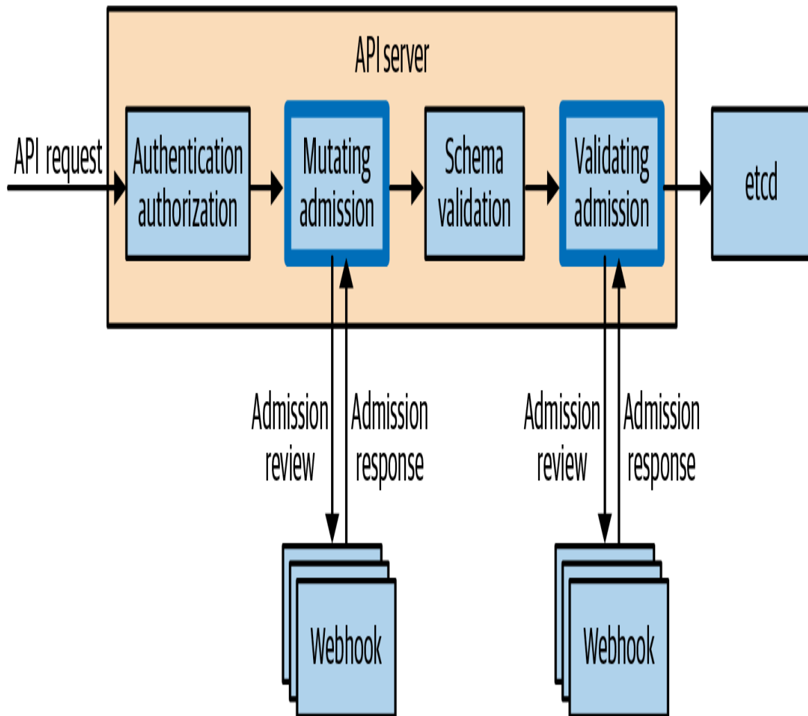
Figure 20-1. API request flow through the Kubernetes API server
