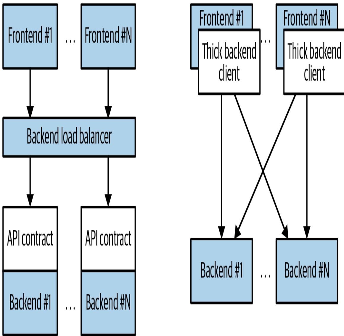
Figure 10-1. Diagrams of decoupled (left) and coupled (right) application architectures
