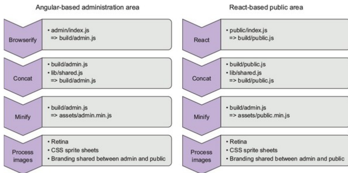
Figure 4.1. Two build processes that share functionality
