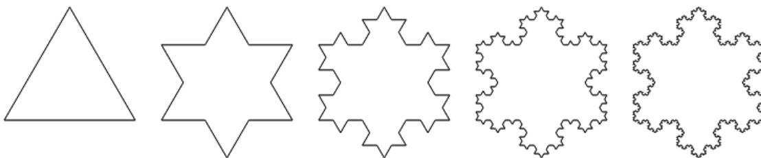
Figure 15-12. Koch snowflakes
