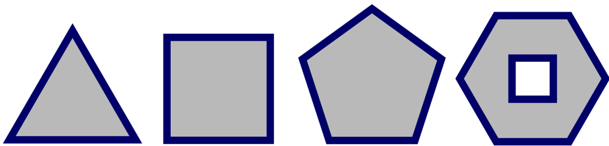
Figure 15-8. Regular polygons
