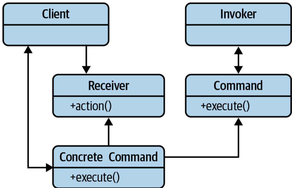
Figure 7-12. Command pattern
