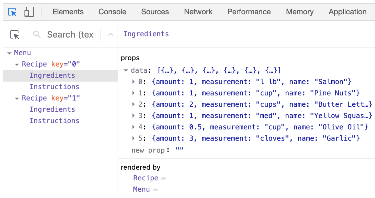
Figure 5-3. Resulting virtual DOM in React Developer Tools
