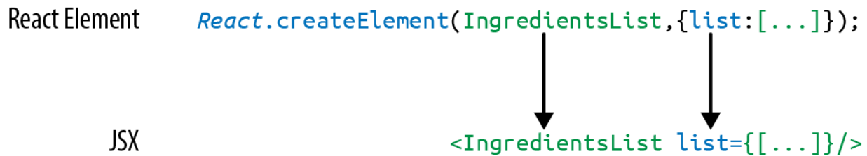
Figure 5-1. Creating the IngredientsList with JSX
