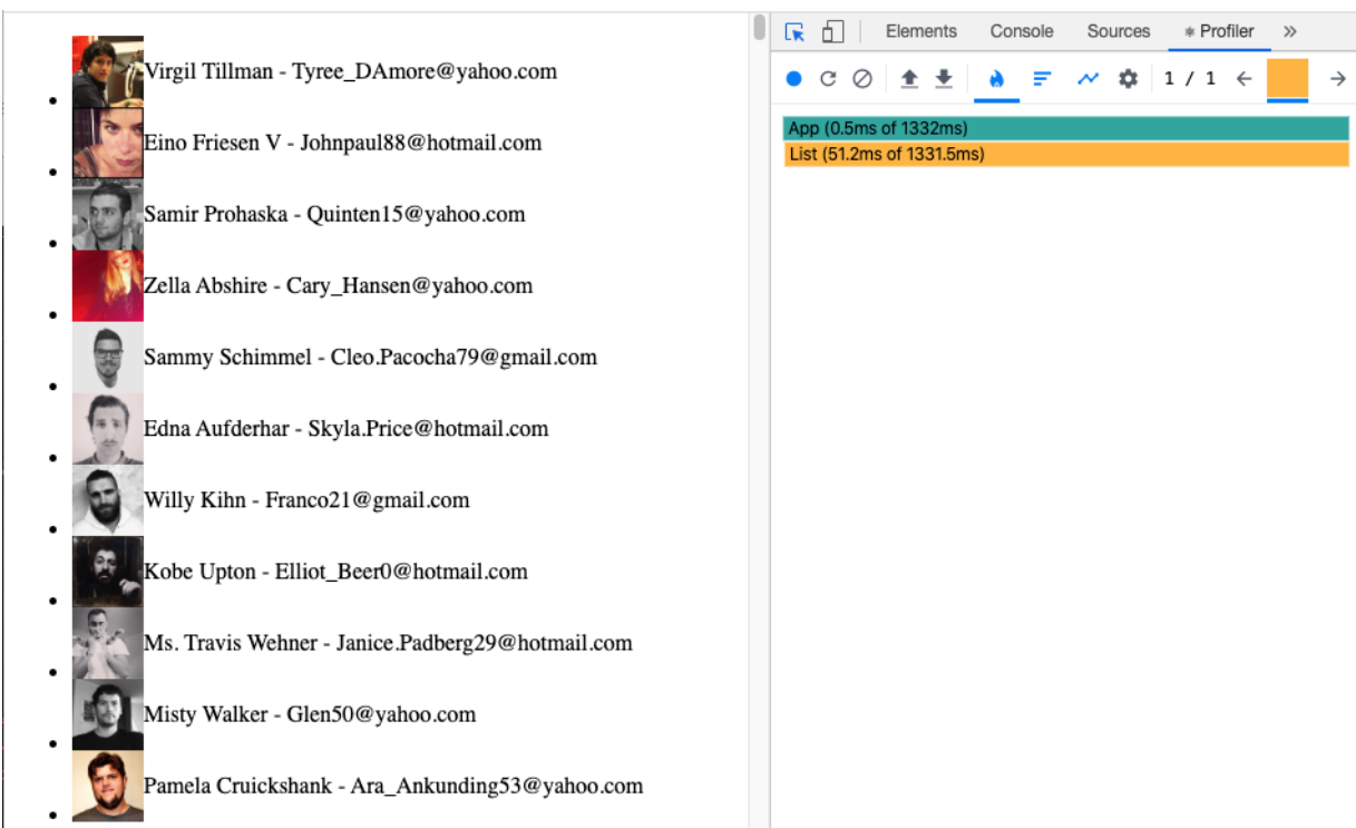
Figure 8-3. Performance results
