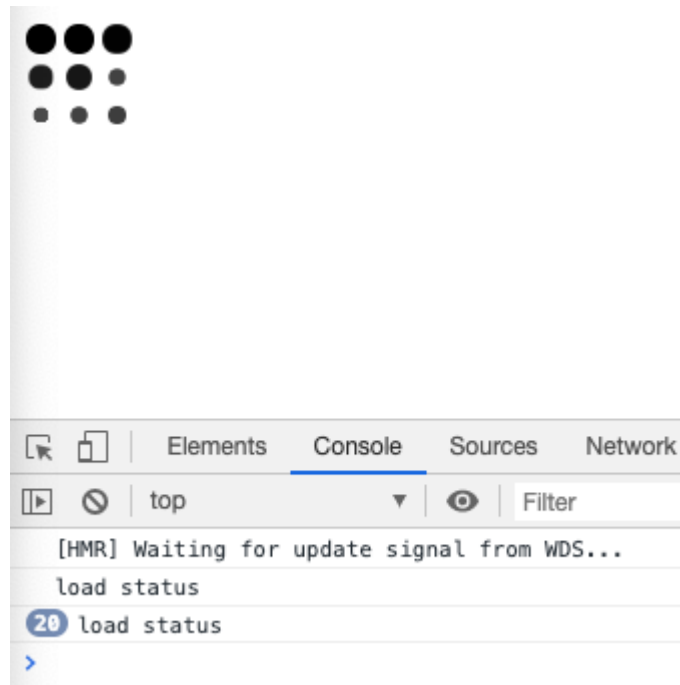
Figure 9-12. Suspense recursion
