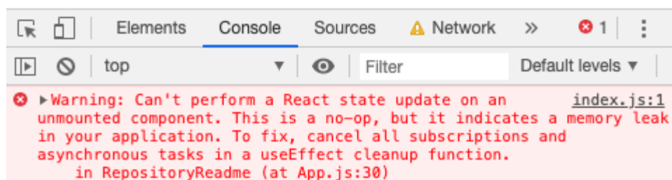
Figure 8-10. Mounted error
