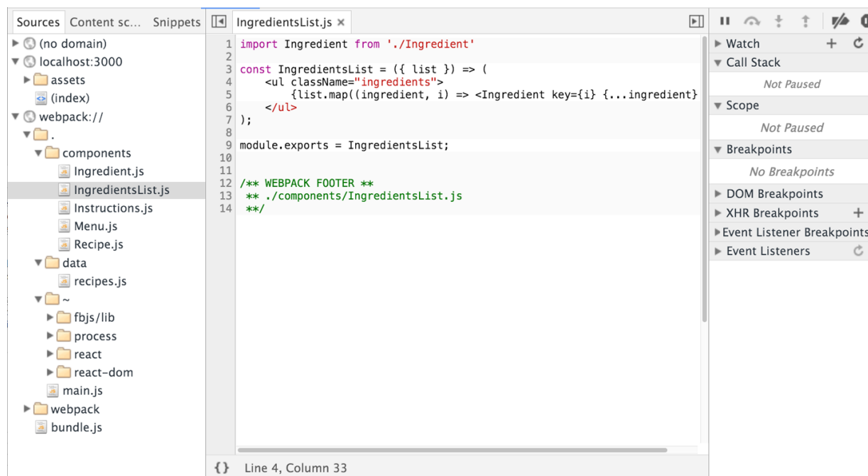
Figure 5-4. Sources panel of Chrome Developer Tools
