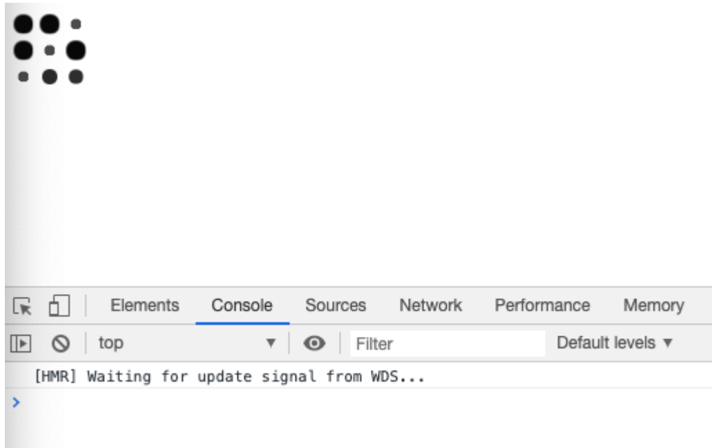
Figure 9-7. GridLoader
