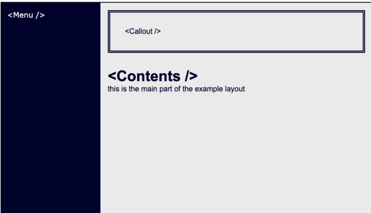
Figure 9-1. Sample layout
