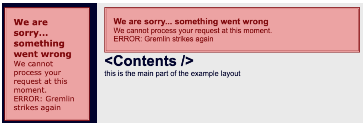
Figure 9-2. ErrorBoundaries
