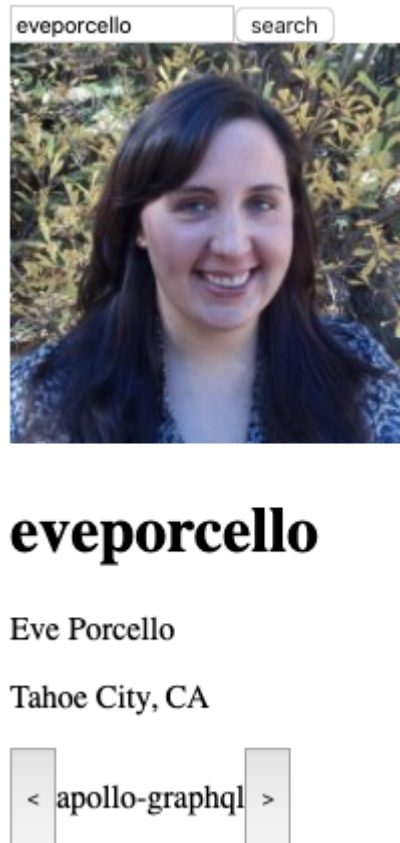
Figure 8-5. Repository output
