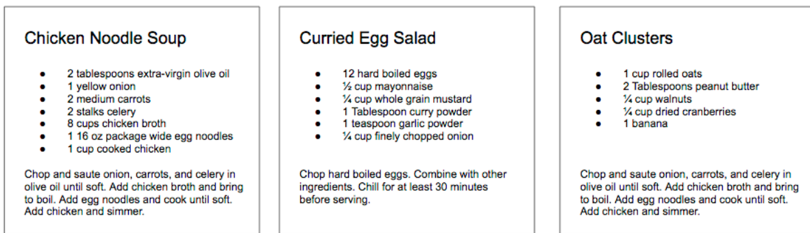
Figure 4-2. Recipes app
