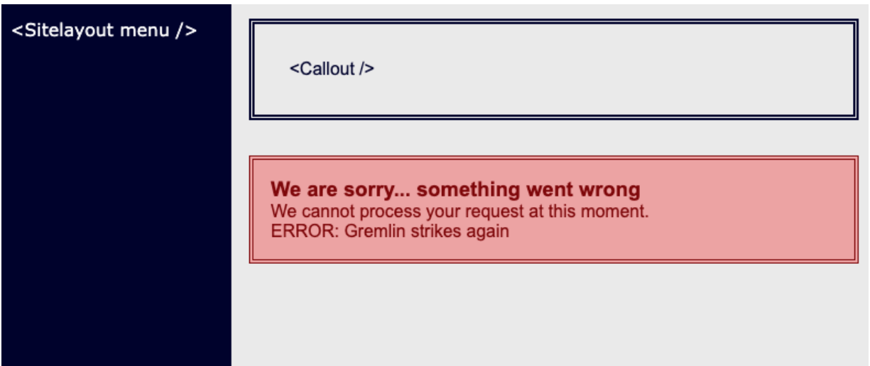
Figure 9-3. Error
