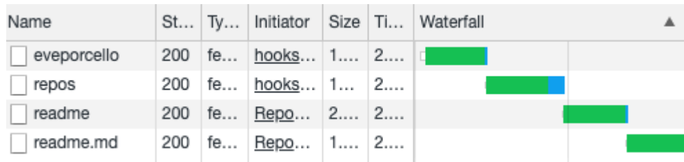
Figure 8-8. The waterfall of a request
