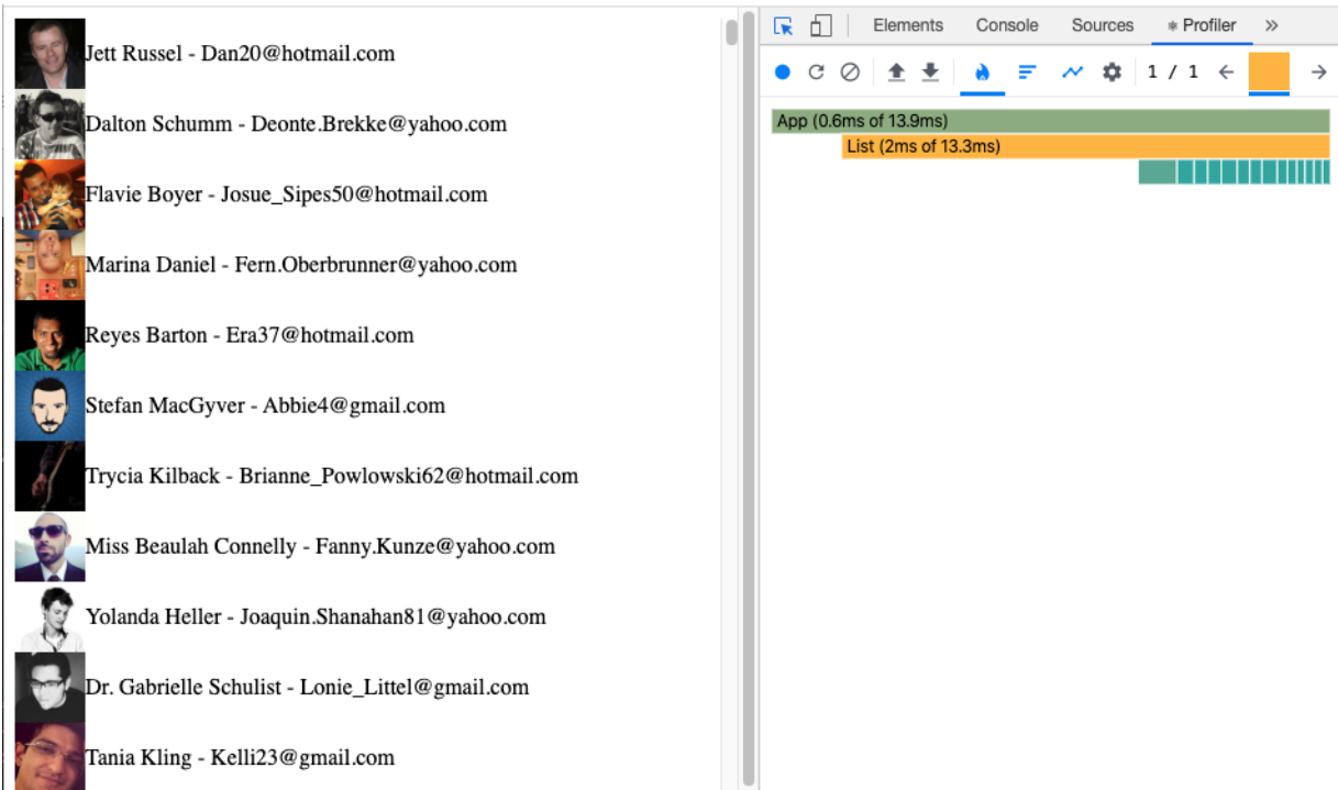
Figure 8-4. 2.6ms for this render
