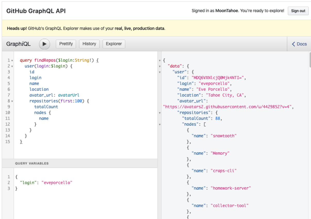
Figure 8-11. GitHub GraphQL Explorer
