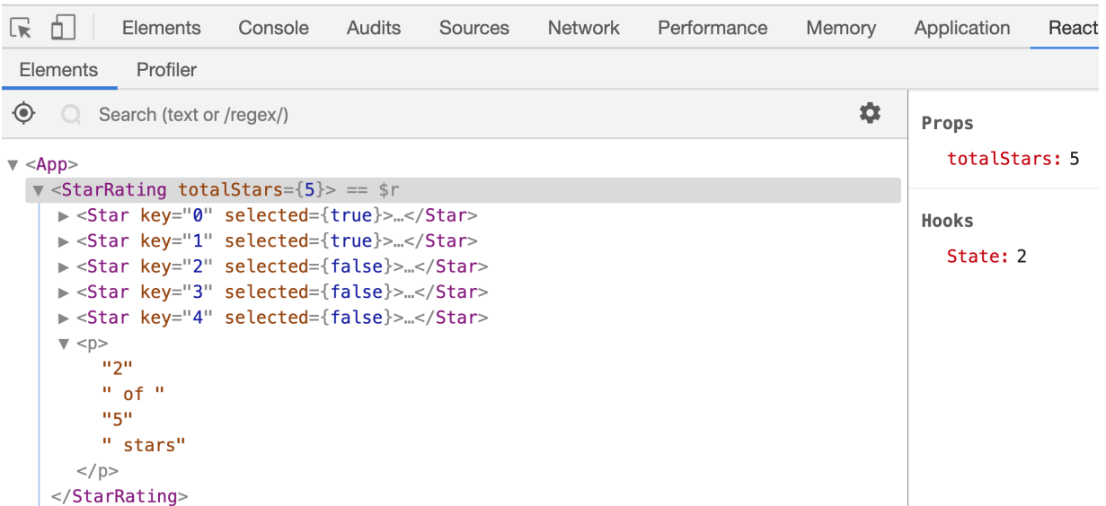
Figure 6-4. Hooks in React developer tools
