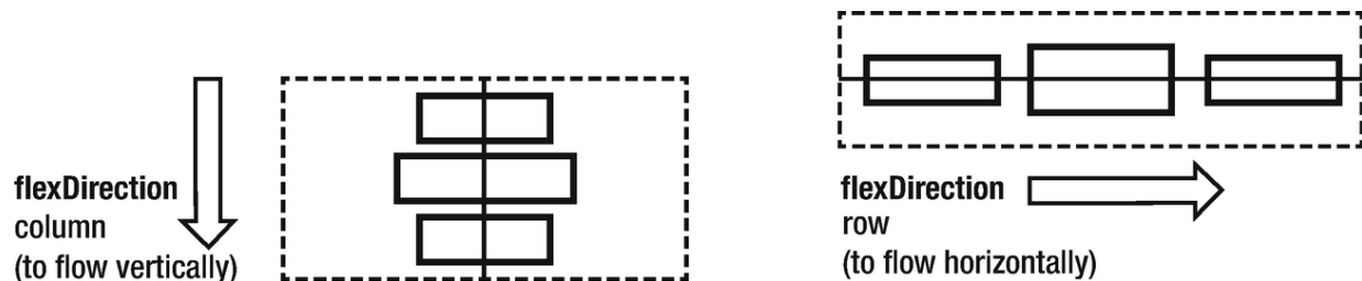
Figure 2-4 alignItem: 'center' on different flow directions
