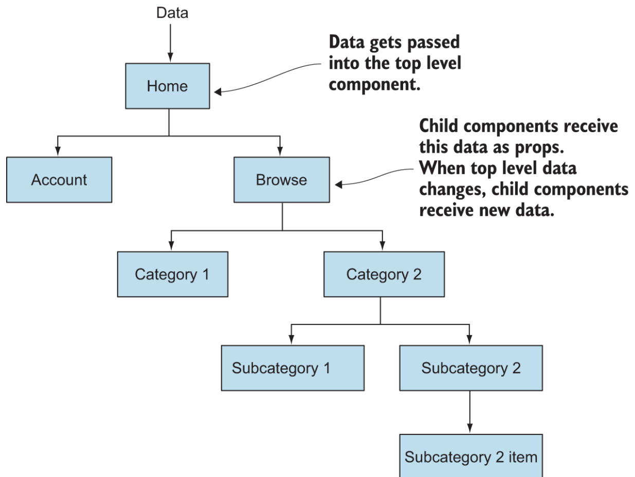
Figure 1.3 How one-way data flow works
