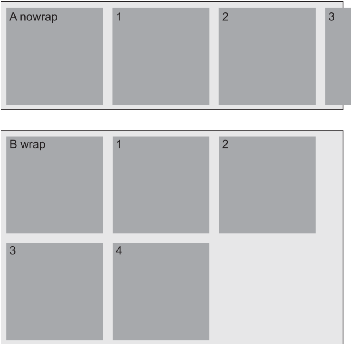
Figure 5.21 An example of two overflowing containers: one with flexWrap set to nowrap and the other with flexWrap set to wrap
