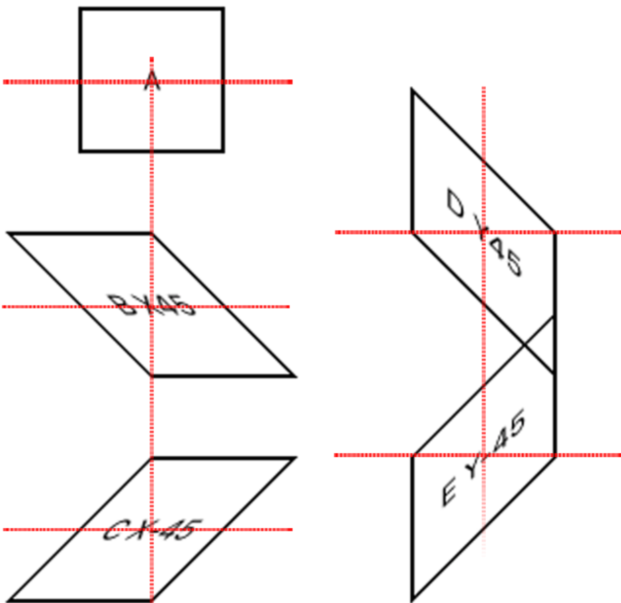
Figure 5.15 Examples of skewing a square along the x- and y-axes on iOS. Square A has no transformation applied. Square B is skewed along the x-axis by 45^\circ . Square C is skewed along the x-axis by -45^\circ . Square D is skewed along the y-axis by 45^\circ , and square E is skewed along the y-axis by -45^\circ .
