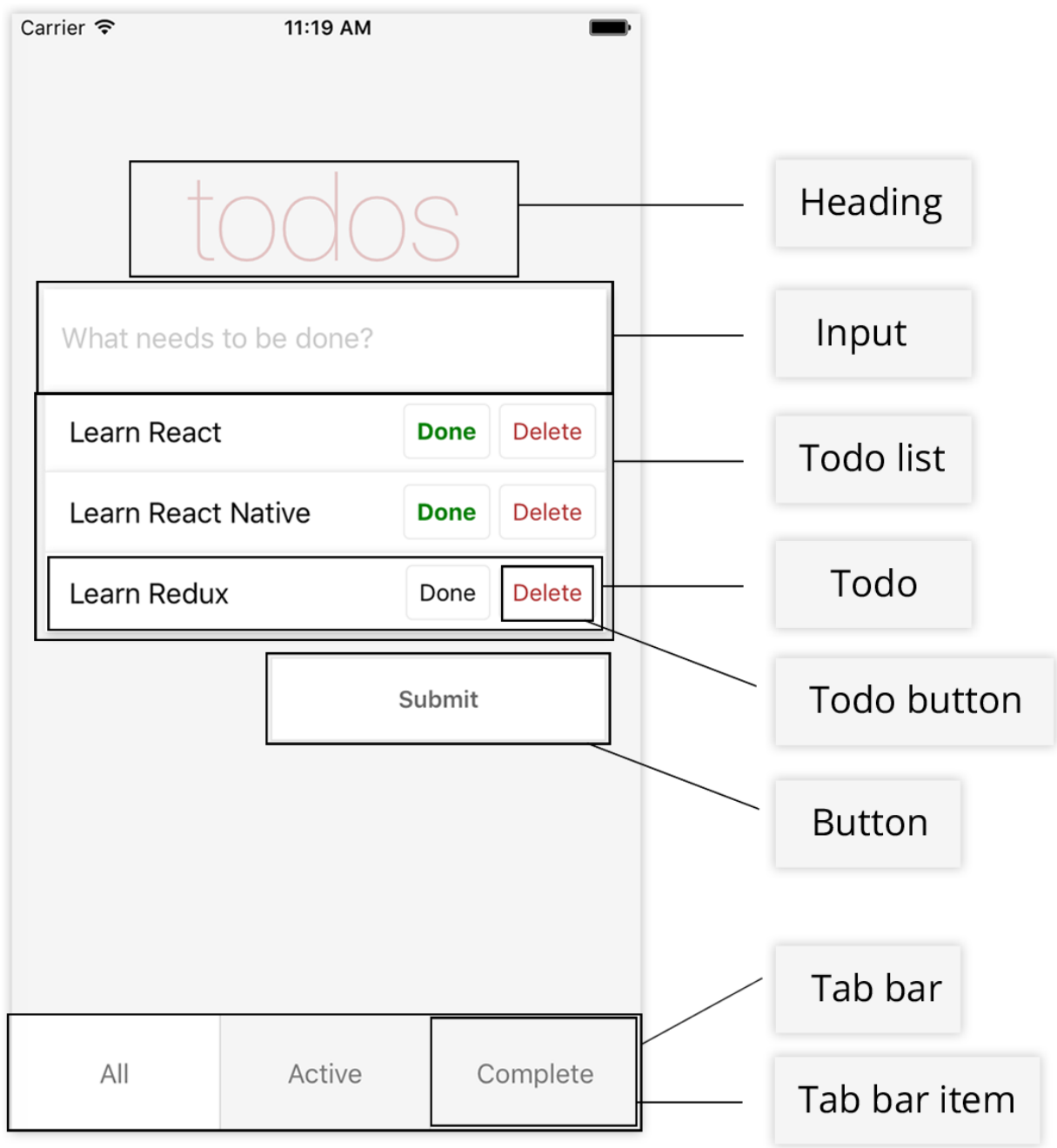
Figure 3.2 Todo app with descriptions
