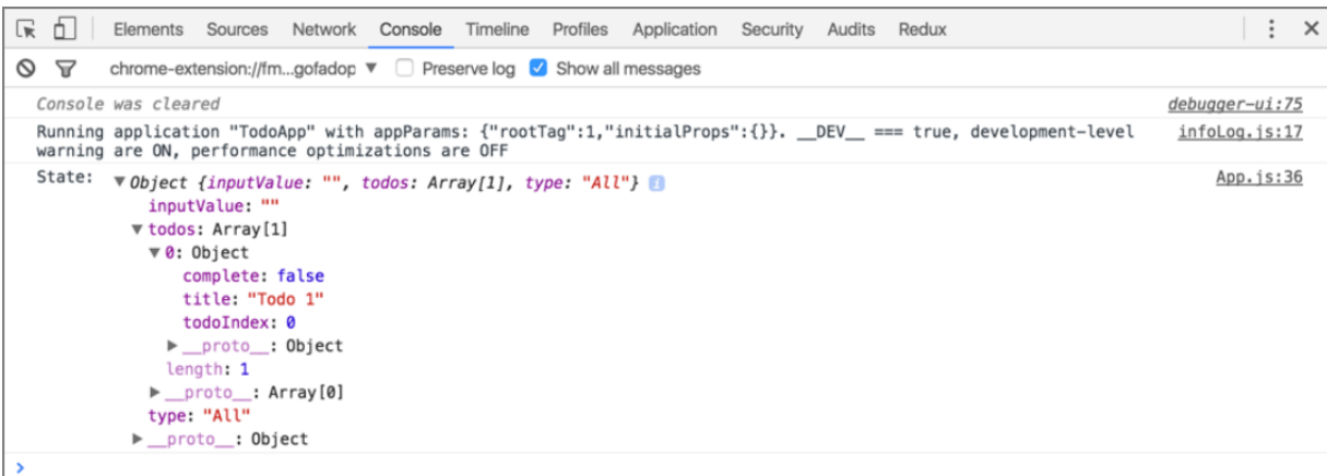
Figure 3.16 Logging the state
