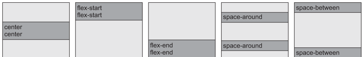
Figure 5.18 Examples of how justifyContent affects the distribution of space between flexible child elements for each of the supported options: center , flex-start , flex-end , space-around , and space-between .
