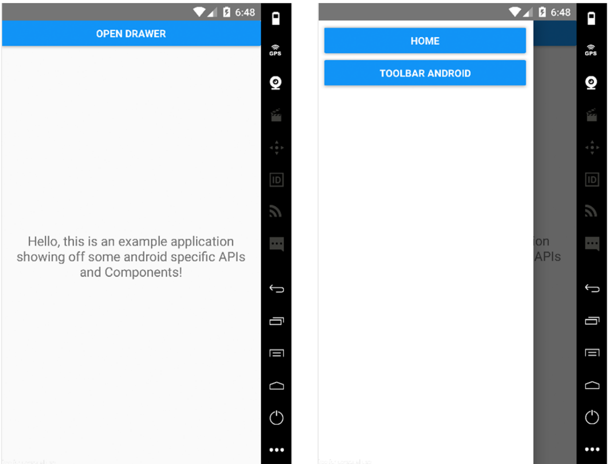
Figure 11.1 Initial layout of the application using DrawerLayoutAndroid . The button at the top in the first screen, Open Drawer, will call a method that opens the drawer. The second screen is the opened drawer.
