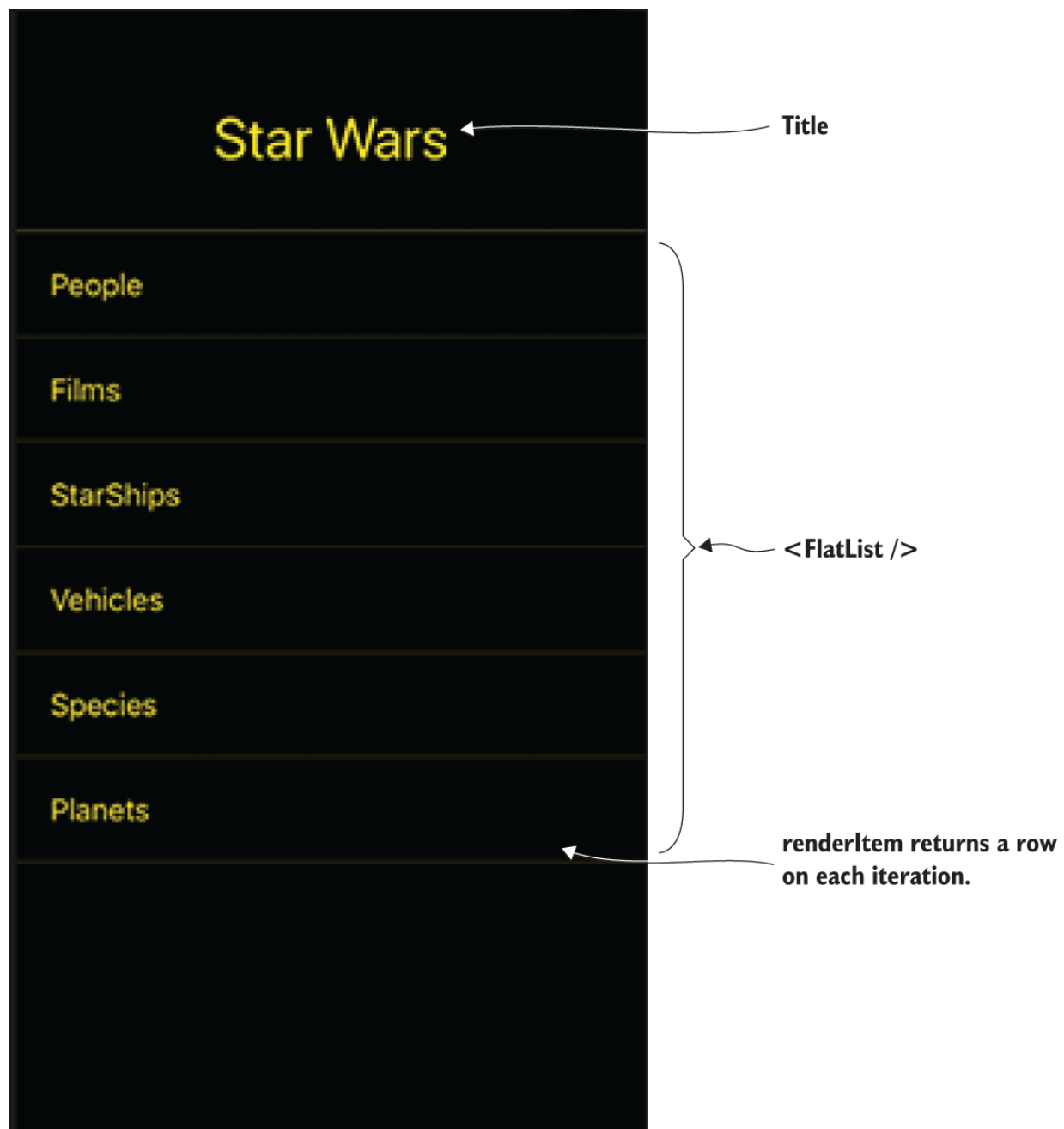
Figure 12.3 Components and title for the StarWars component
