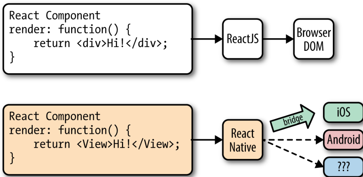
Figure 2-2. React can render to different targets
