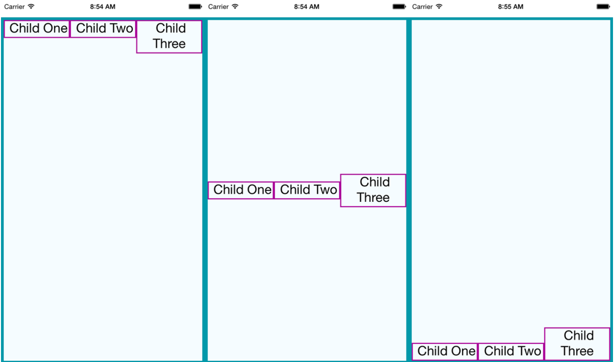
Figure 5-3. Setting alignItems positions children on the cross-axis, which is the axis orthogonal to the flexDirection ; here, we see flex-start , center , and flex-end
