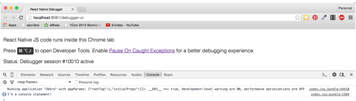
Figure 9-5. Console output as viewed in Chrome
