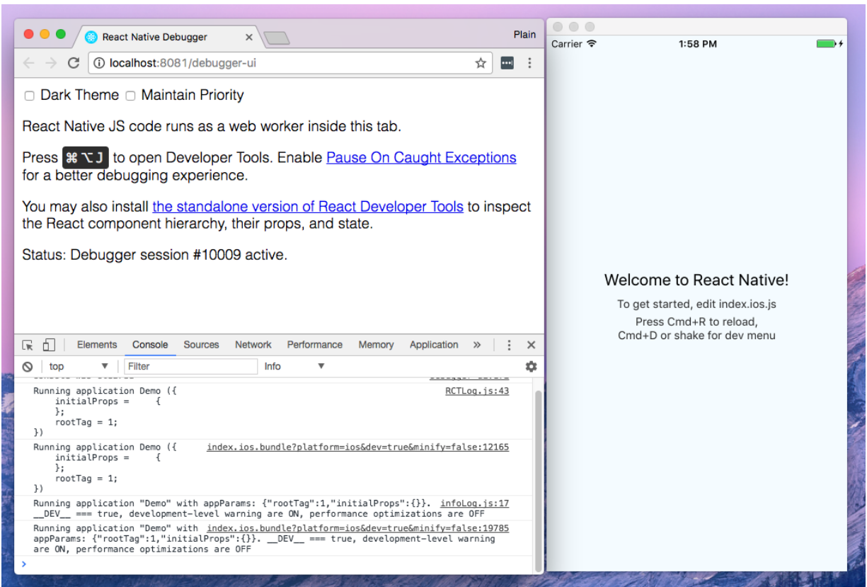
Figure 1-1. Using the Chrome Debugger with React Native
