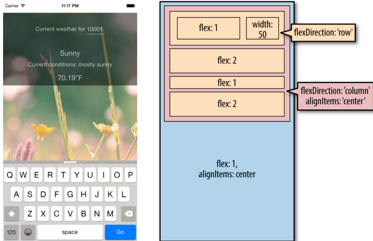
Figure 3-5. Layout of the finished weather application
