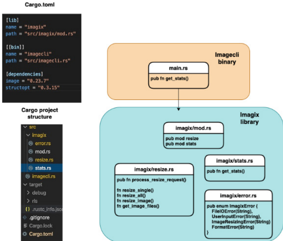
Figure 4.5 – Code organization
