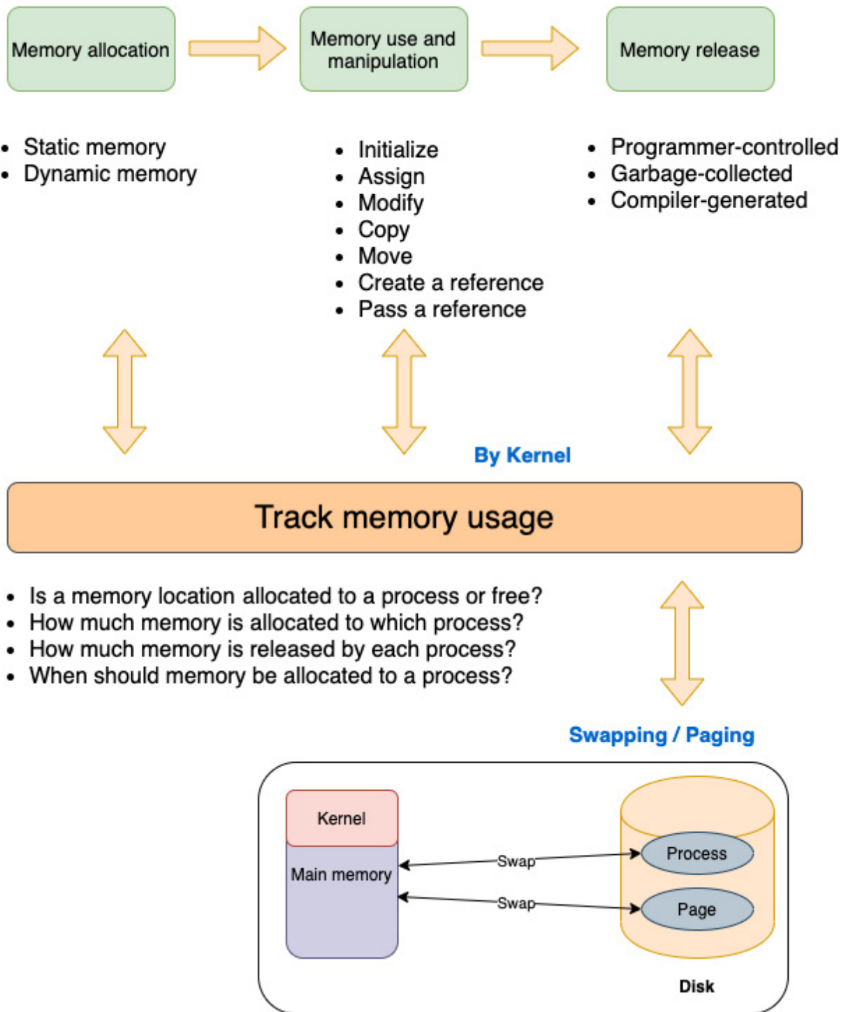
Figure 5.2 – Memory lifecycle
