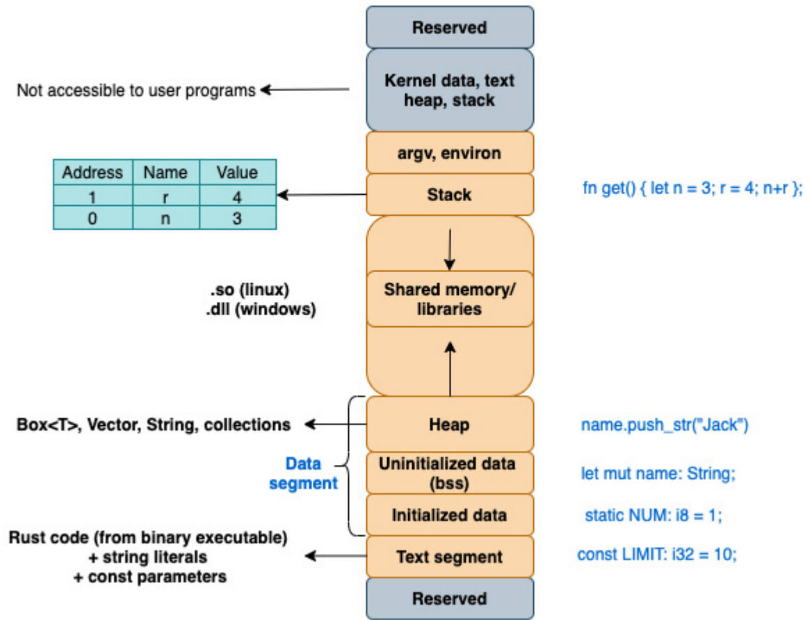
Figure 8.1 – Program memory layout
