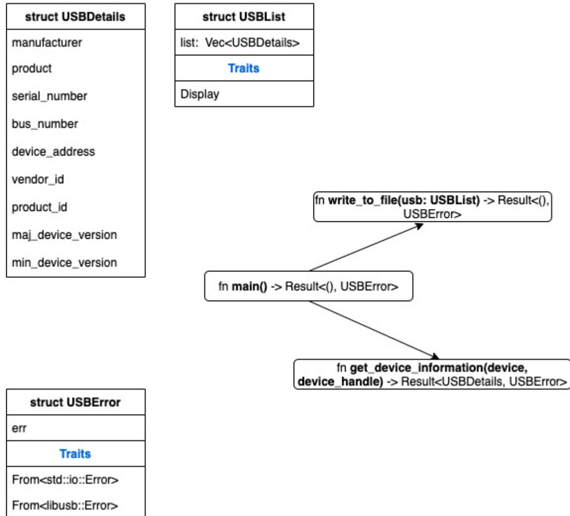
Figure 10.2 – Design of the USB detector project
