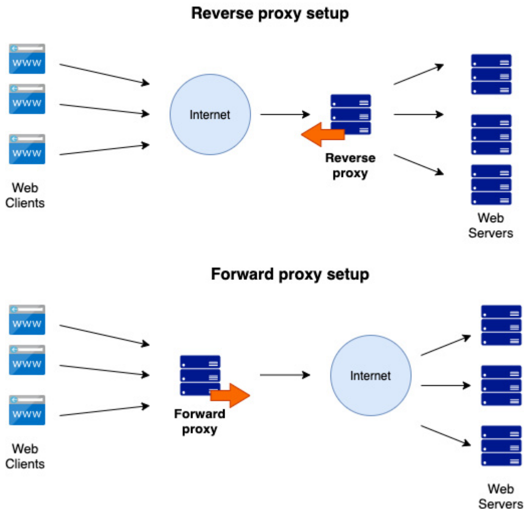
Figure 11.4 – Types of proxy servers
