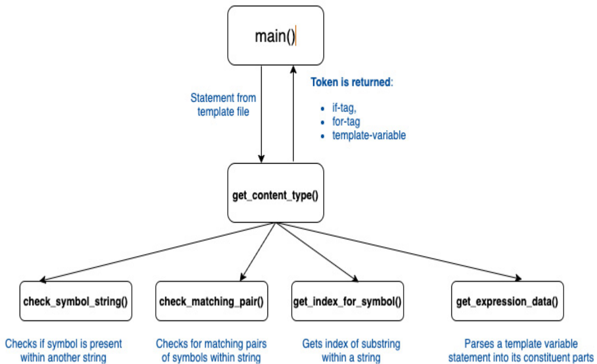
Figure 3.9: Parser design
