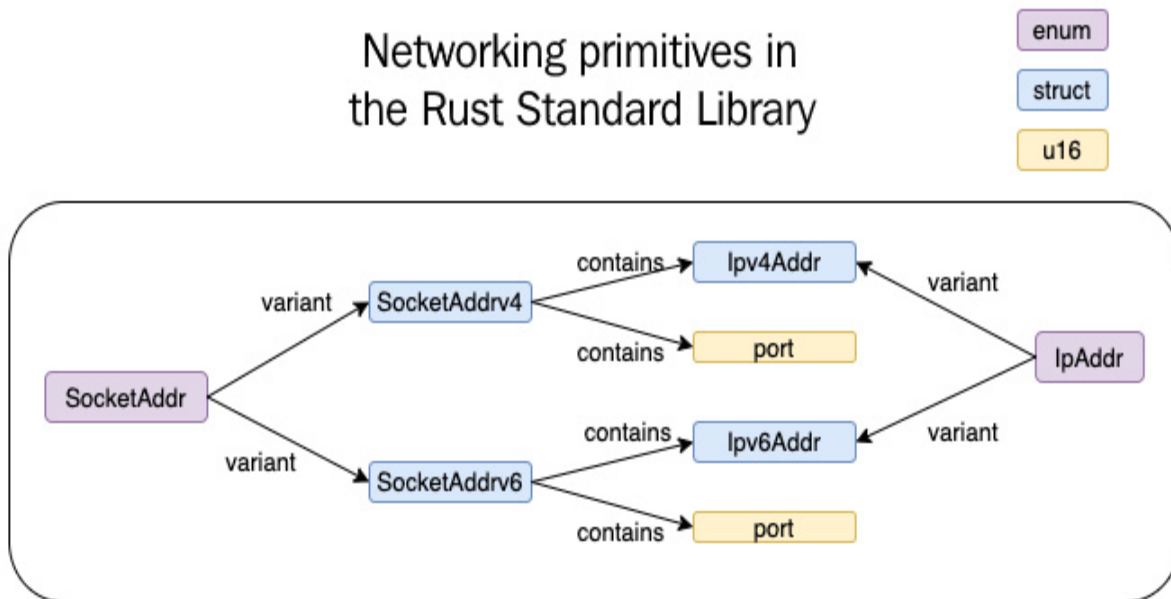
Figure 11.3 – Networking primitives in the Rust standard library
