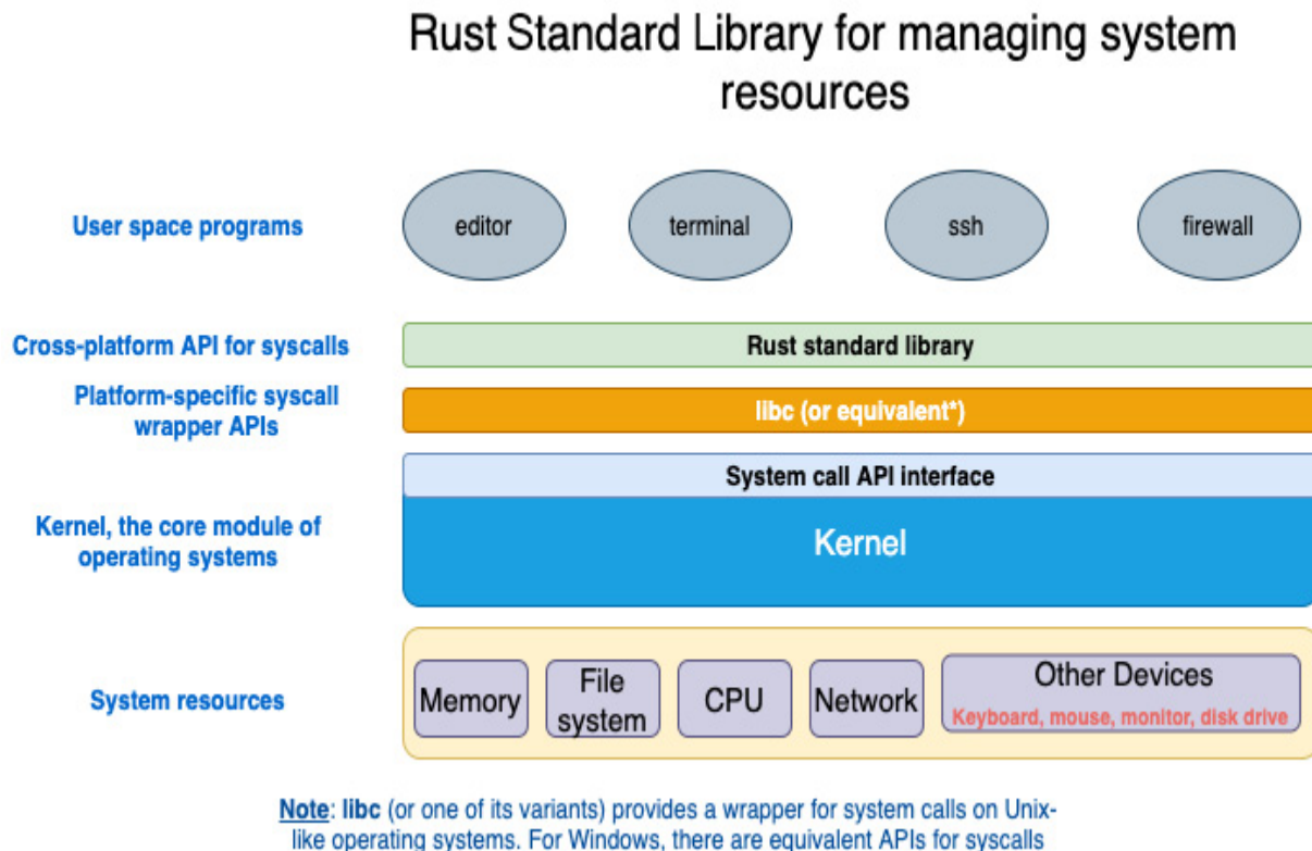
Figure 3.1 – Rust Standard Library
