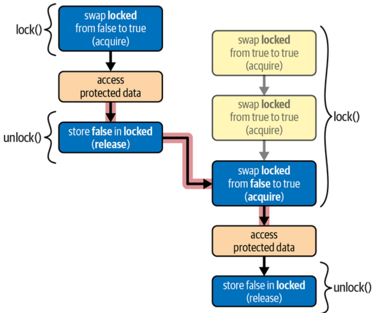
Figure 4-1. The happens-before relationships between two threads using our SpinLock to protect access to some shared data
