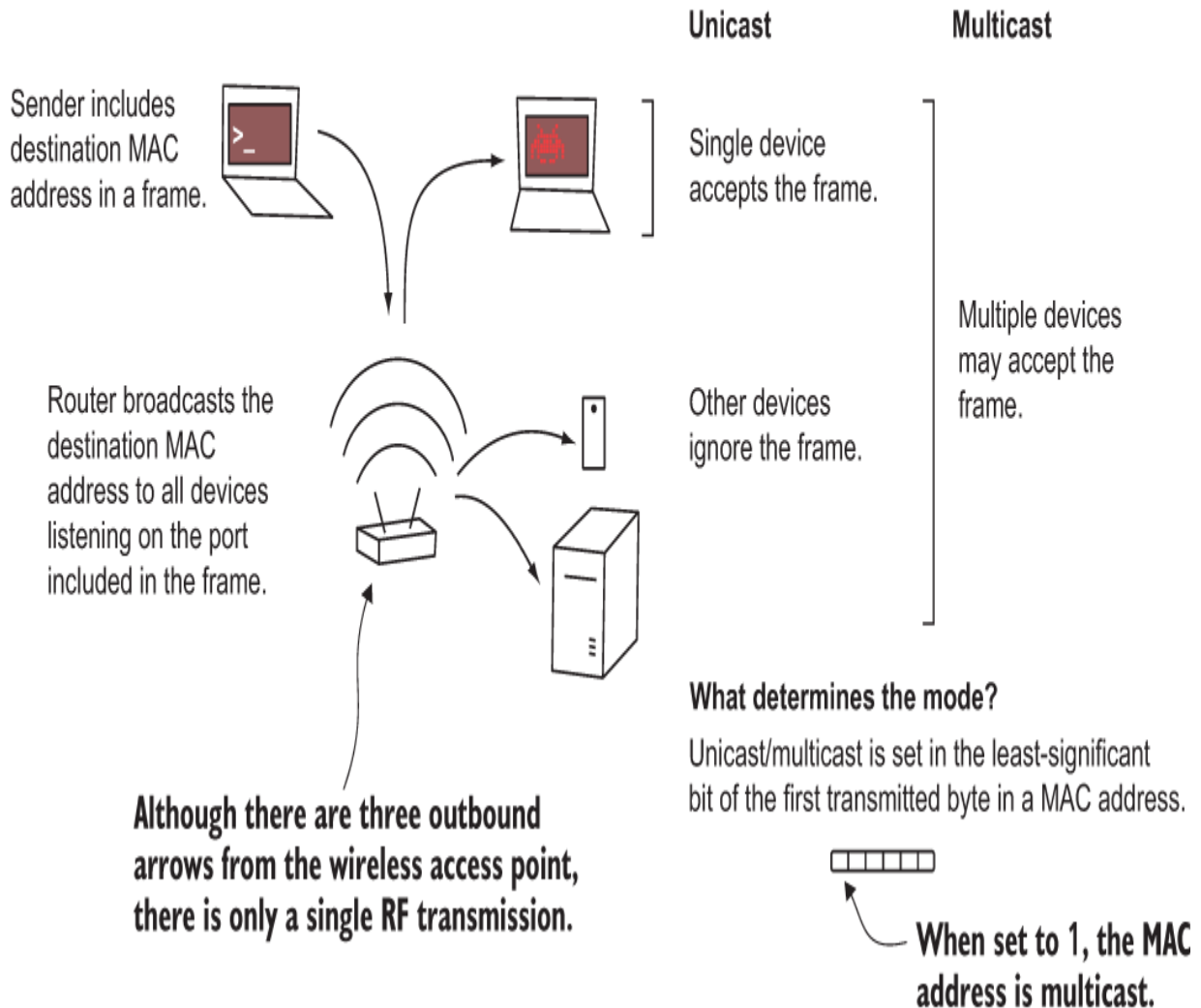
Figure 8.4 The differences between multicast and unicast MAC addresses
