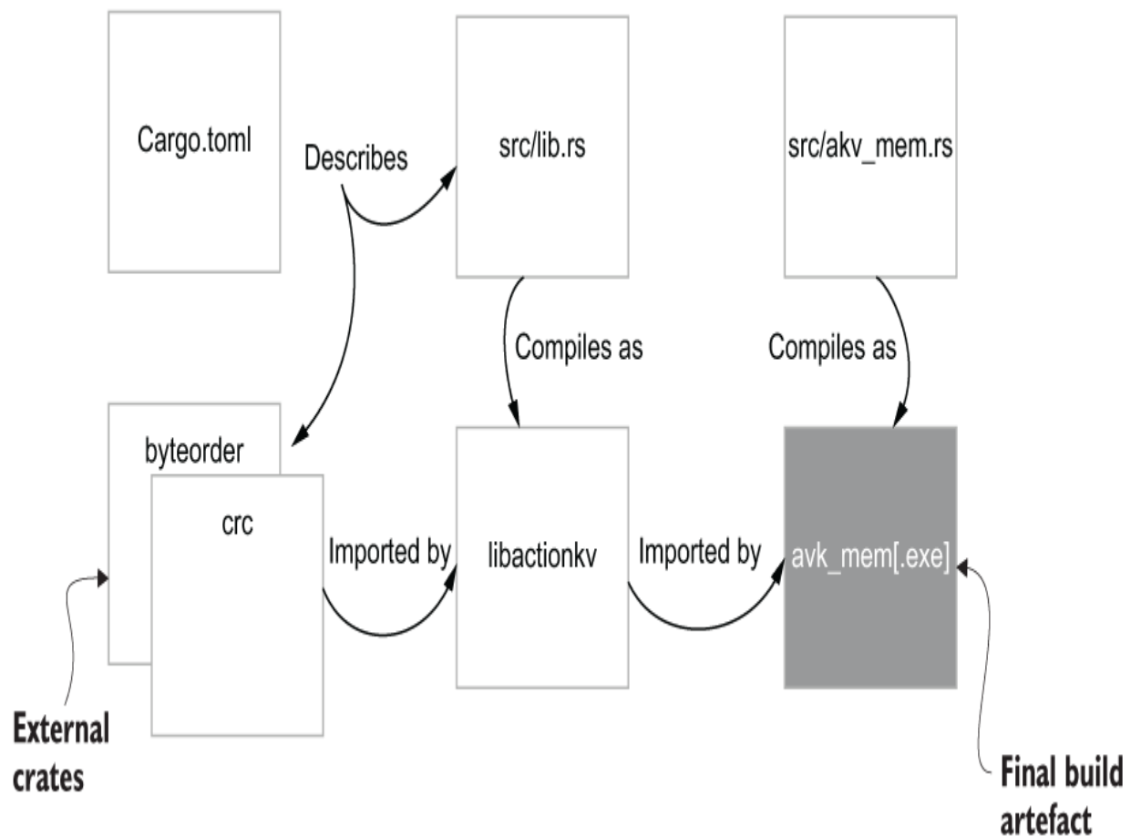
Figure 7.1 An outline of how the different files and their dependencies work together in the actionkv project. The project's Cargo.toml coordinates lots of activity that ultimately results in an executable.
