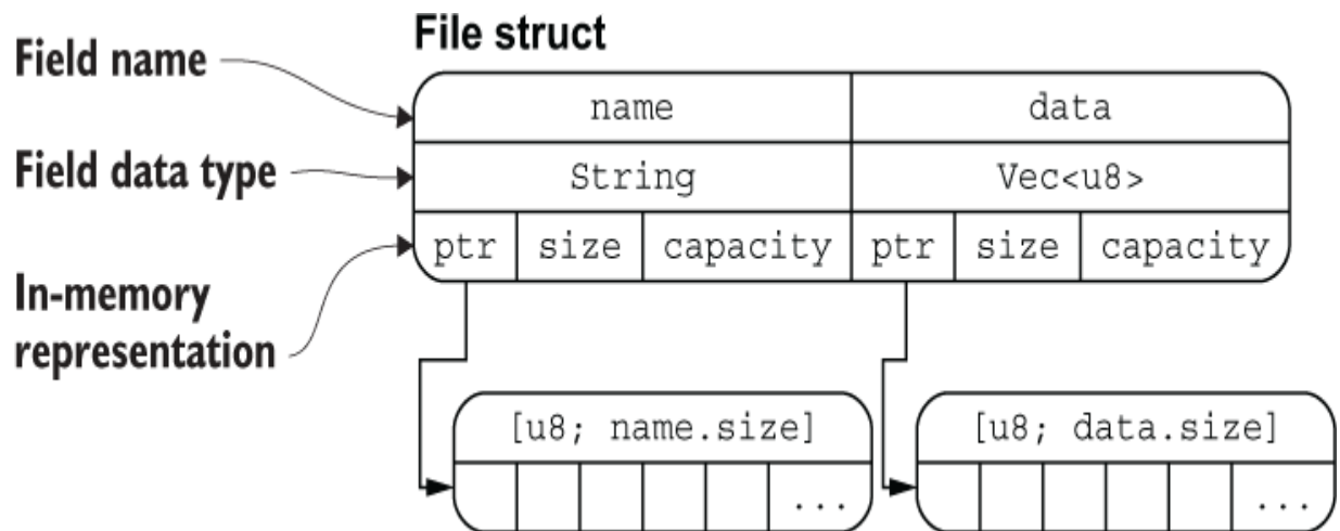
Figure 3.1 Inspecting the internals of the File struct
