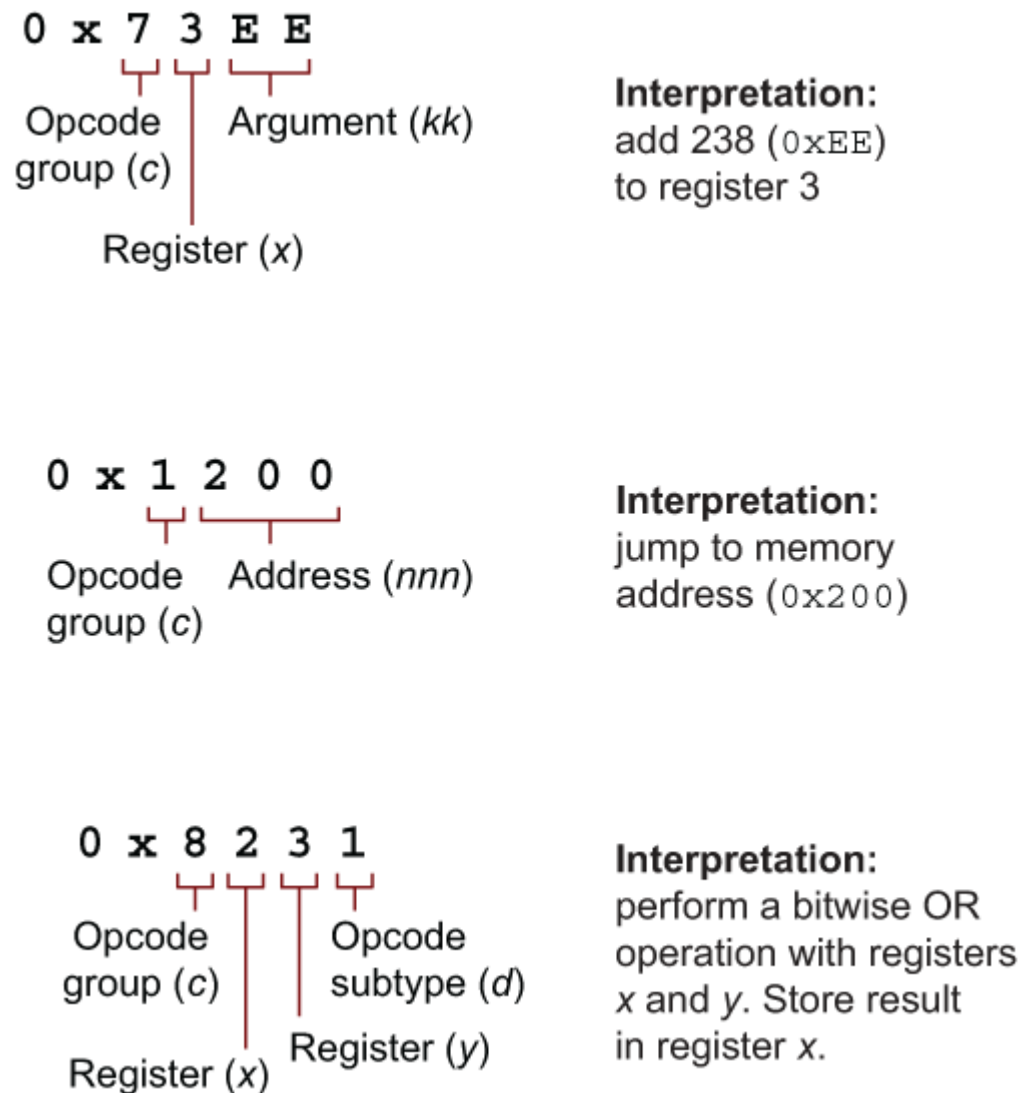
Figure 5.3 CHIP-8 opcodes are decoded in multiple ways. Which to use depends on the value of the leftmost nibble.
