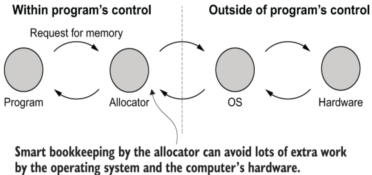
Figure 6.6 Conceptual view of dynamic memory allocation. Requests for memory originate and terminate at the program level but involve several other components. At each stage, the components may short-circuit the process and return quickly.
