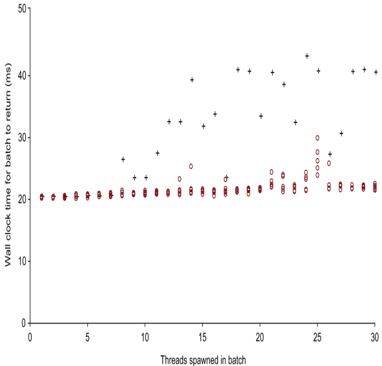
Figure 10.3 Comparing the time taken to wait for 20m using the sleep strategy (circles) versus the spin lock strategy (plus symbols). This chart shows the differences that occur as the number of threads exceeds the number of CPU cores (6).
