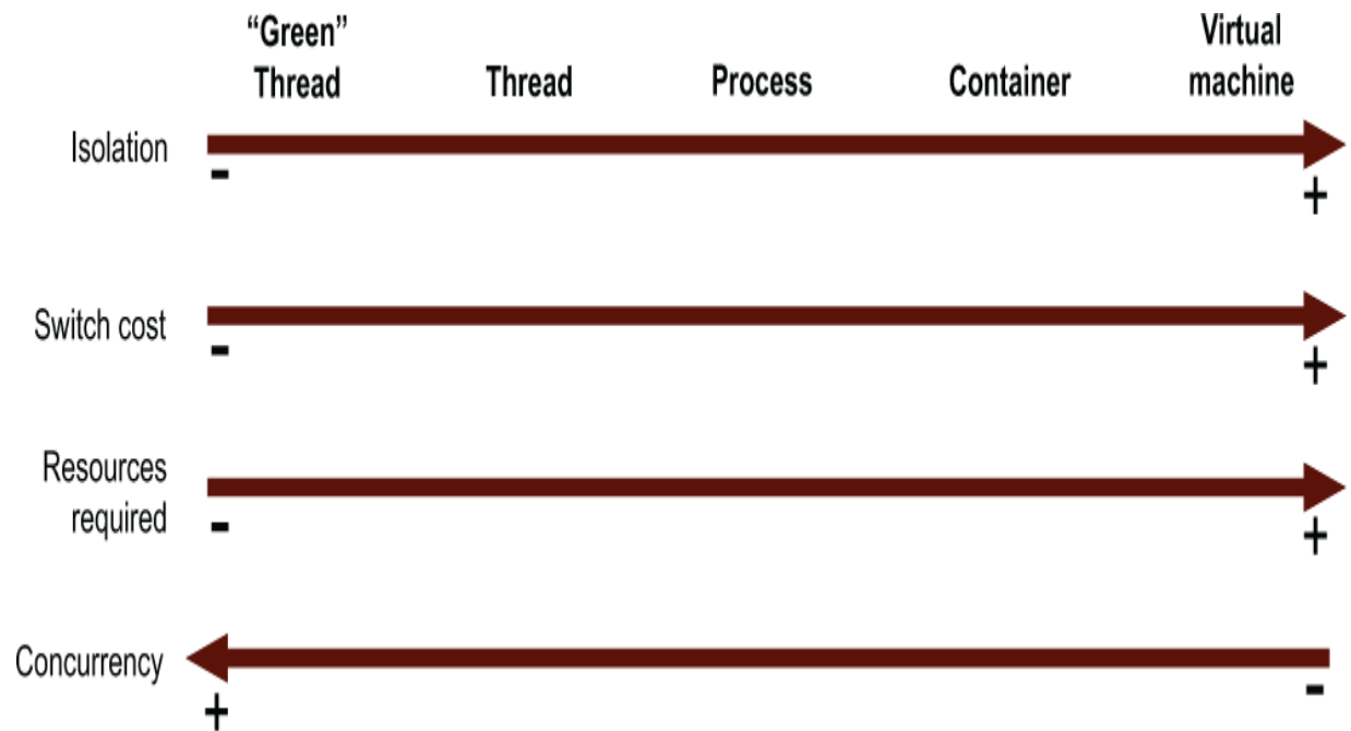
Figure 10.5 Trade-offs relating to different forms of task isolation in computing. In general terms, increasing the isolation level increases the overhead.
