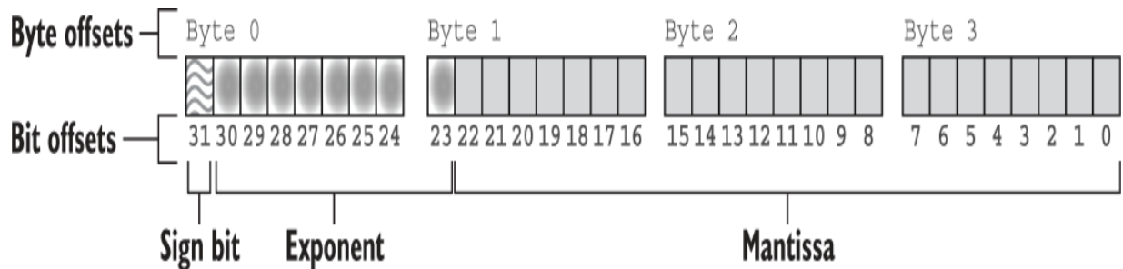
Figure 5.1 An overview of the three components encoded within the bits of a floating-point number for the f32 type in Rust
