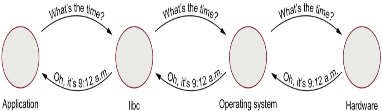
Figure 9.1 An application gets time information from the OS, usually functionally provided by the system's libc implementation.
