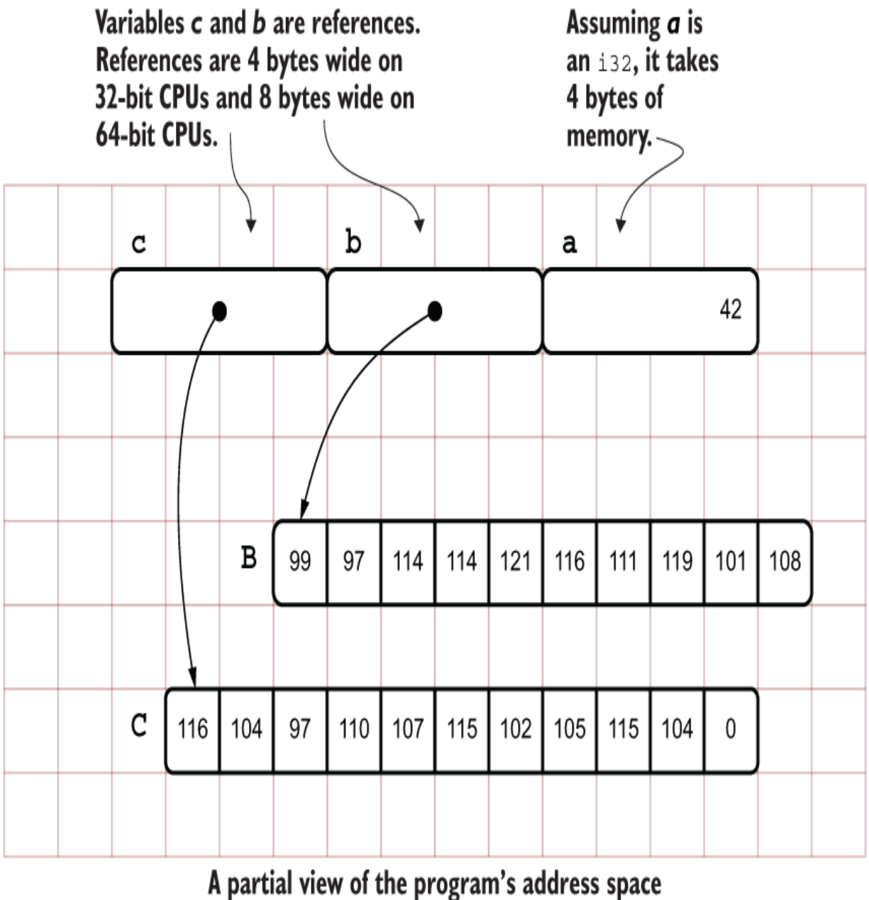
Figure 6.2 An abstract view of how two pointers operate alongside a standard integer. The important lesson here is that the programmer might not know the location of the referent data beforehand.
