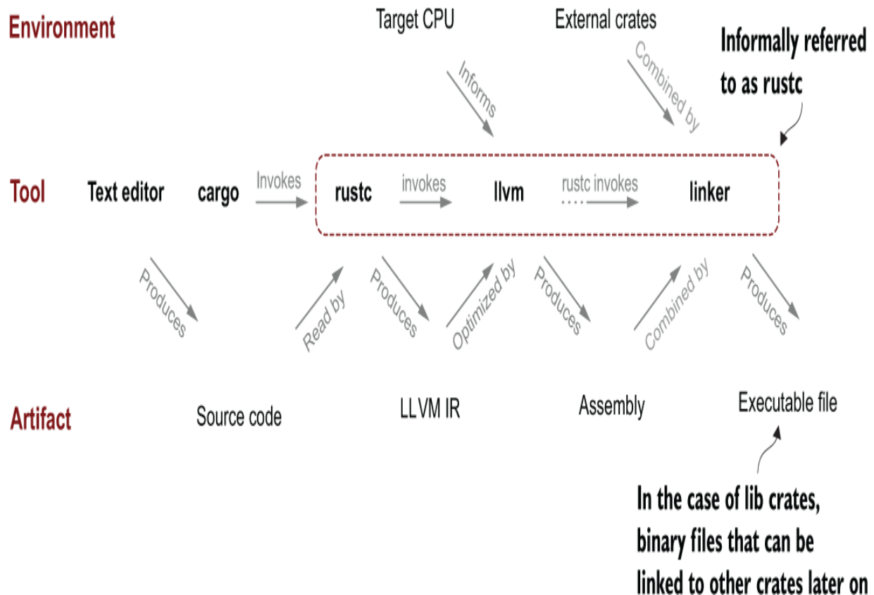
Figure 12.6 Some of the major steps required to generate an executable from Rust source code. LLVM is an essential part of the process but not one that is user-facing.
