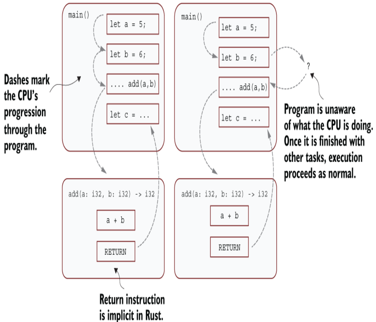
Figure 12.2 Using addition to demonstrate control flow for handling signals
