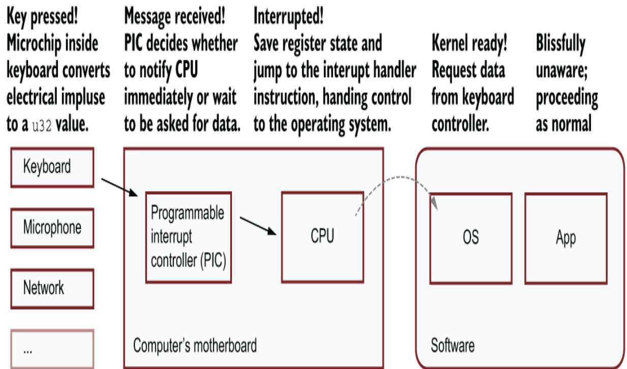
Figure 12.3 How applications are notified of an interrupt generated from a hardware device. Once the OS has been notified that data is ready, it then directly communicates with the device (in this case, the keyboard) to read the data into its own memory.
