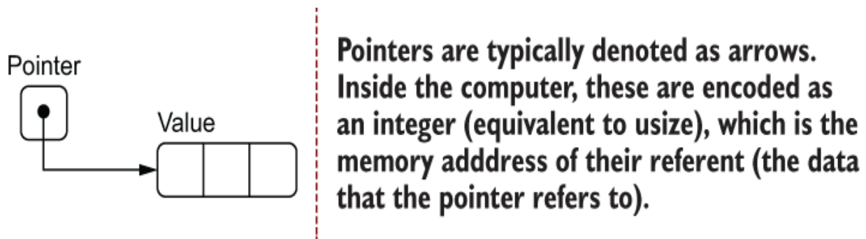
Figure 6.1 Depicting notation used in this chapter’s figures for illustrating a pointer. In Rust, pointers are most frequently encountered as &T and &mut T , where T is the type of the value.
