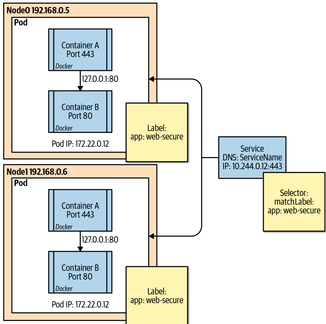
Figure 8-3. Service to pod communication
