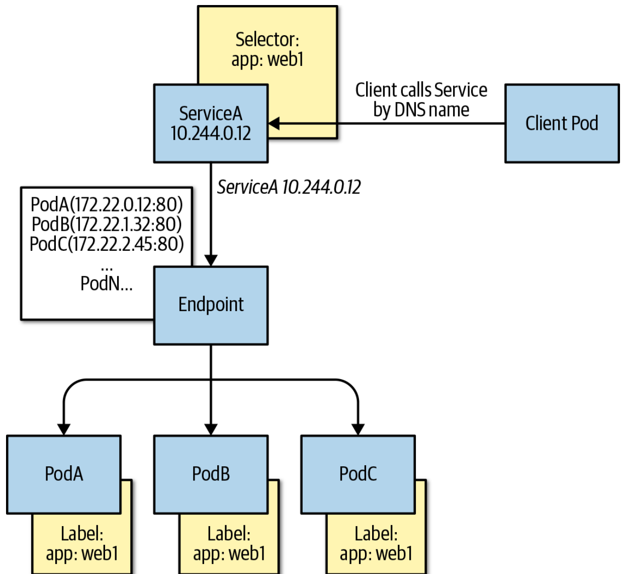
Figure 8-4. ClusterIP Pod and Service visualization
