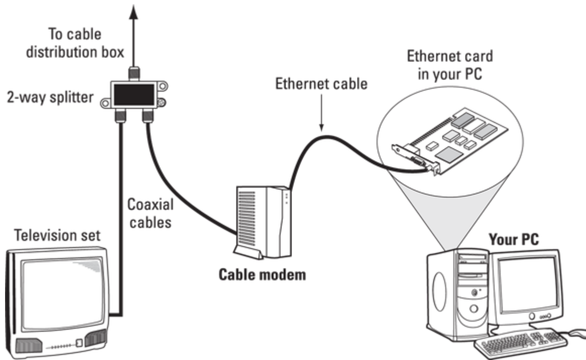
FIGURE 1-4: The cable TV signal is split between the TV and the cable modem.
