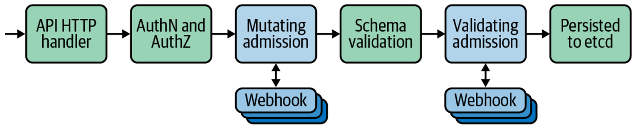
Figure 8-1. Admission chain.
