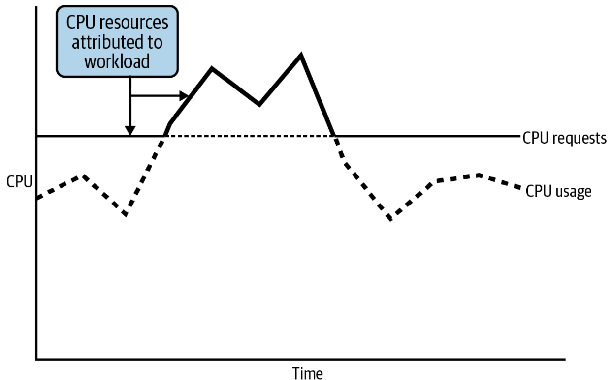
Figure 9-6. Showback based on CPU consumption when bursting above requests.
