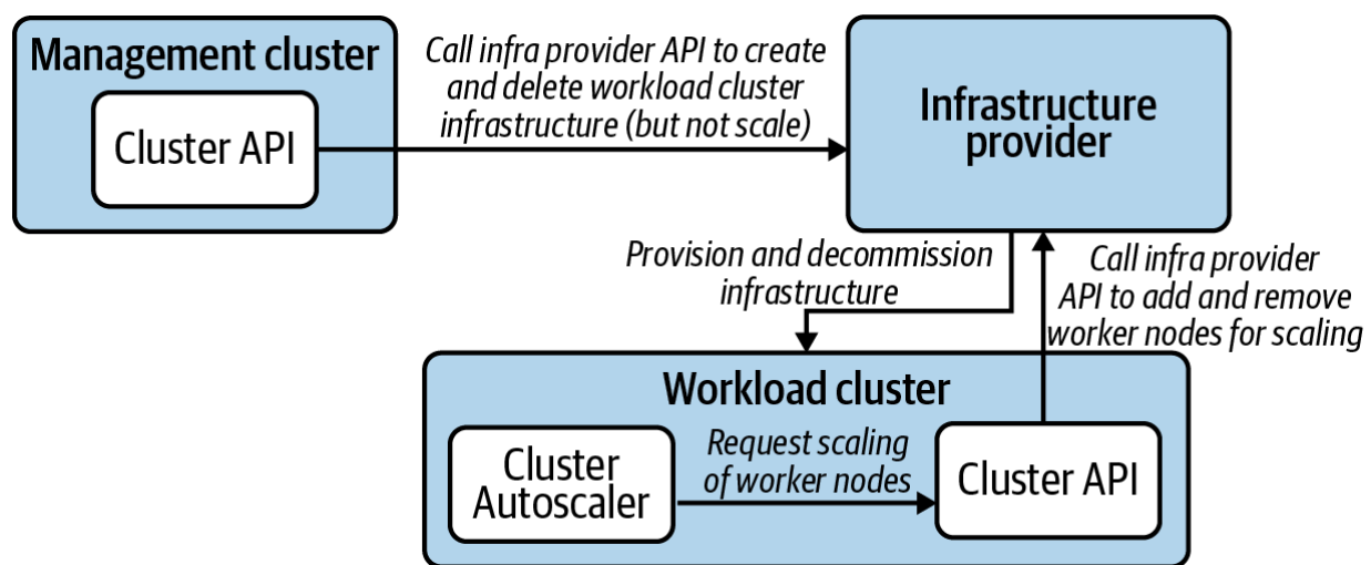
Figure 2-2. Cluster Autoscaler accessing a local Cluster API component to perform scaling events.
