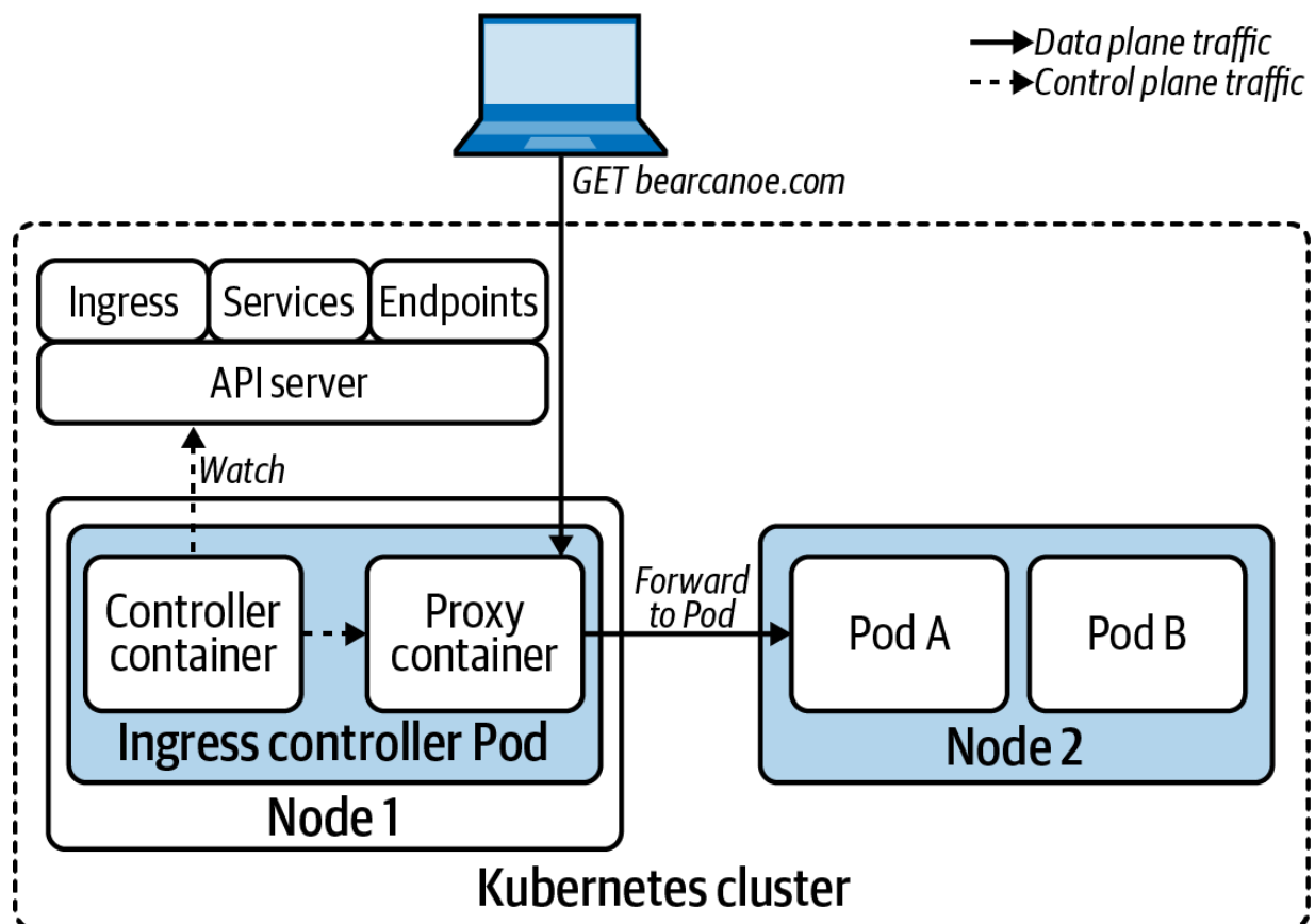
Figure 6-10. The Ingress controller watches various resources in the API server and configures the proxy accordingly. The proxy handles incoming traffic and forwards it to Pods, according to the Ingress configuration.
