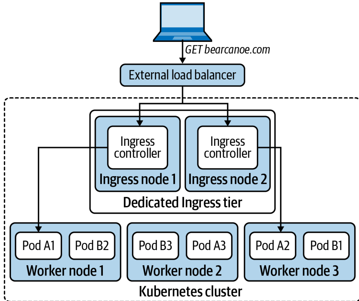
Figure 6-16. Dedicated ingress nodes are reserved for the Ingress controller. The ingress nodes serve as the “edge” of the cluster or the Ingress tier.
