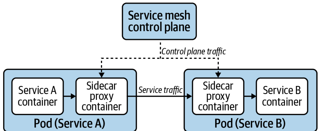
Figure 6-21. Pods participating in the mesh have a sidecar proxy that intercepts the Pod's network traffic.
