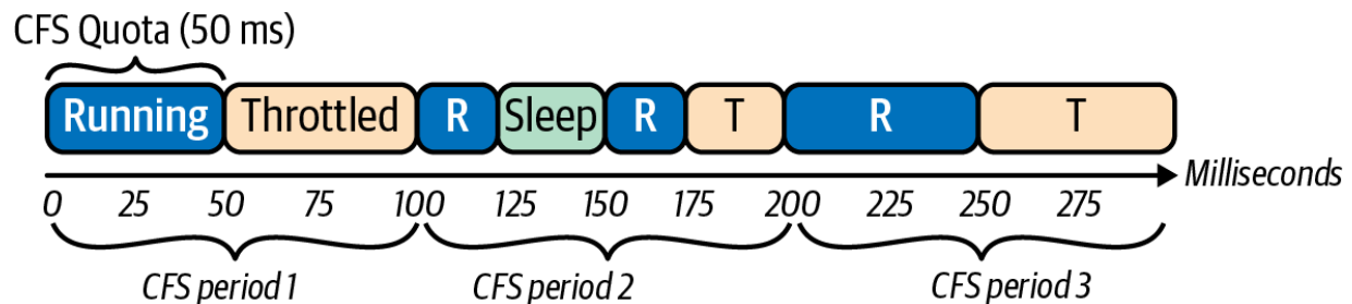
Figure 12-4. CPU consumption and throttling of a process running in a cgroup that has a CFS period of 100 milliseconds and a CPU quota of 50 milliseconds.
