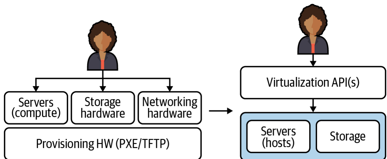
Figure 2-3. Comparison of administrator interactions when provisioning and managing bare metal compute infrastructure versus virtual machines.
