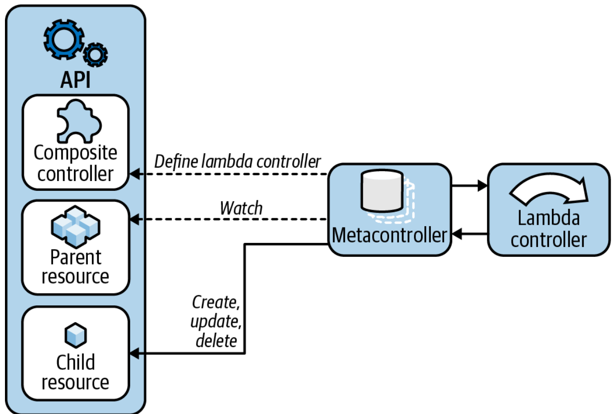
Figure 11-3. Metacontroller abstracts the Kubernetes API for your lambda controller.
