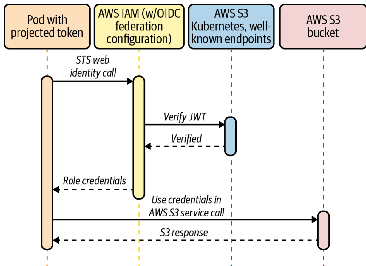
Figure 10-11. IAM roles for Service Accounts.
