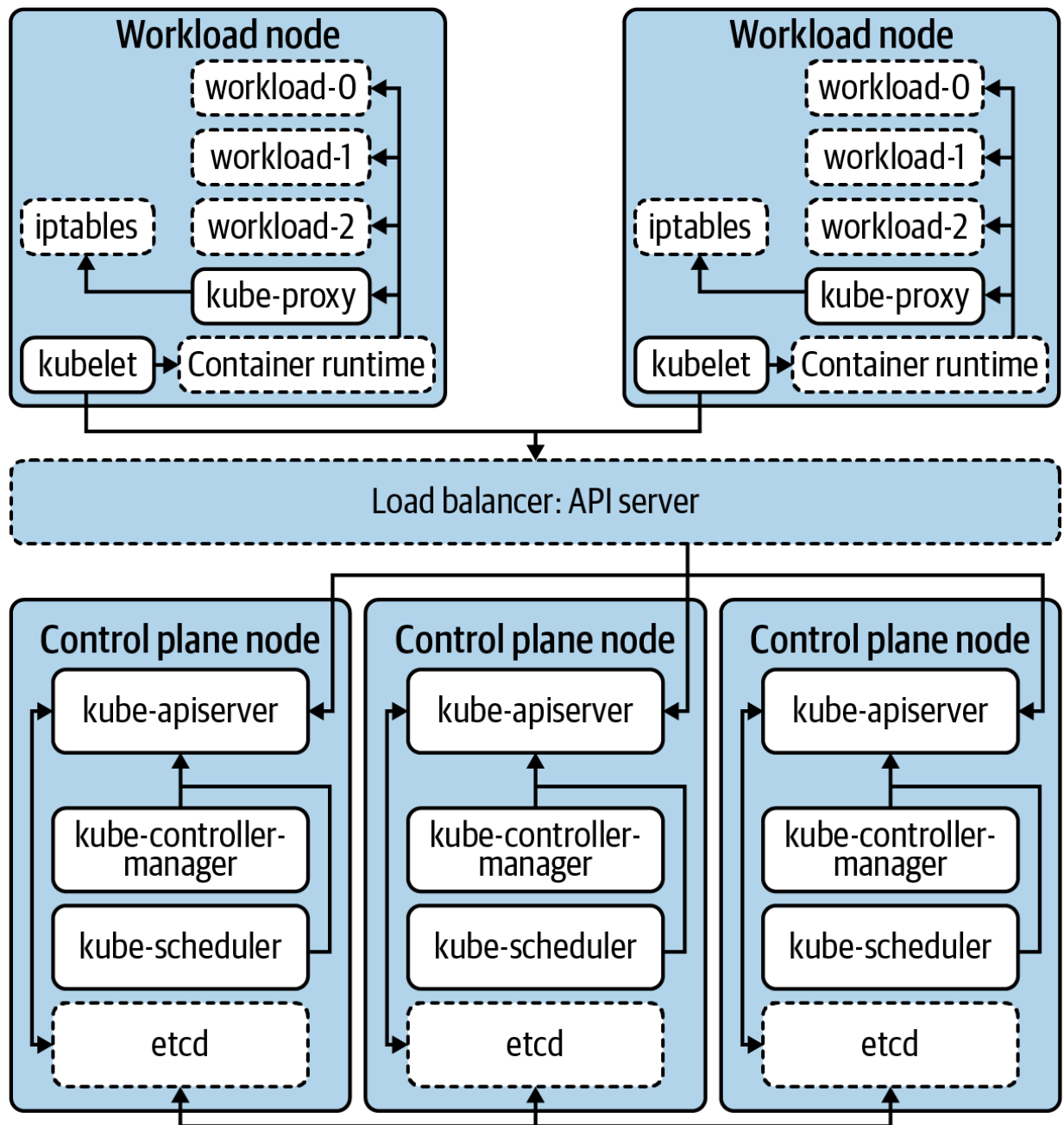
Figure 1-1. The primary components that make up the Kubernetes cluster. Dashed borders represent components that are not part of core Kubernetes.
