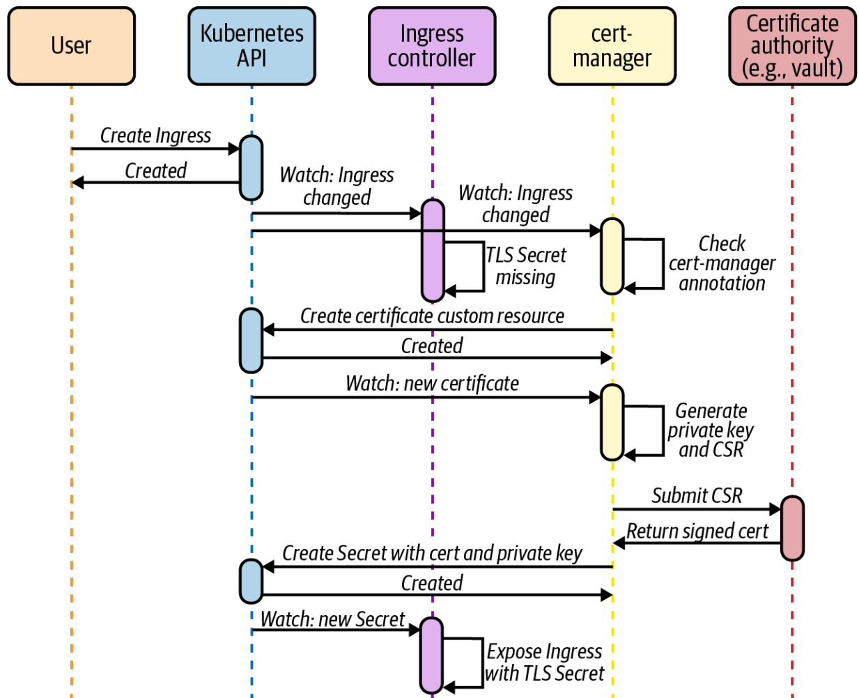
Figure 6-17. Cert-manager watches the Ingress API and requests a certificate from a Certificate Authority when the Ingress resource has the cert-manager.io/cluster-issuer annotation.
