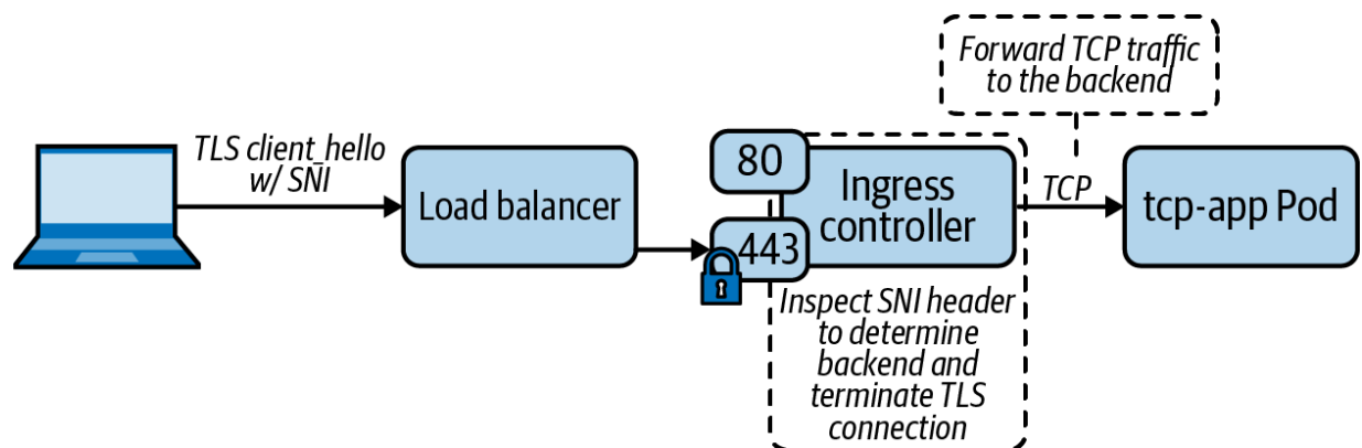
Figure 6-14. The Ingress controller inspects the SNI header to determine the backend, terminates the TLS connection, and forwards the TCP traffic to the Pod.
