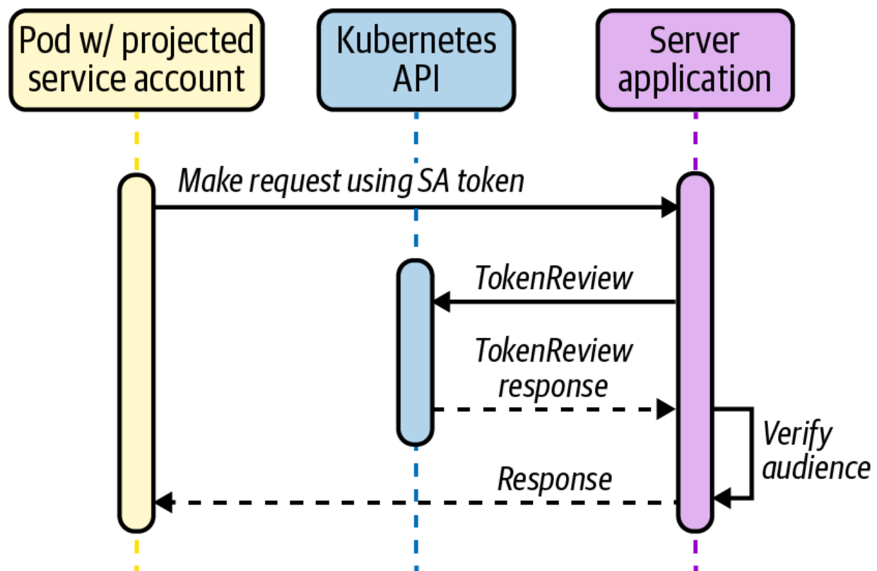
Figure 10-6. Projected Service Account tokens.
