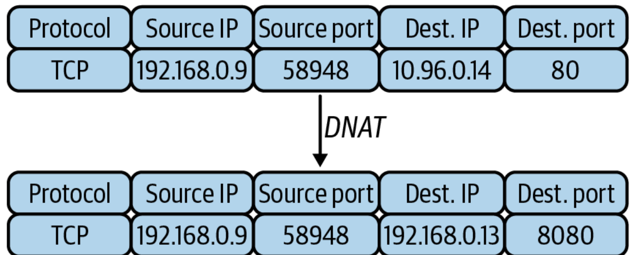
Figure 6-8. Connection tracking (conntrack) table entry that tracks the connection from a Pod ( 192.168.0.9 ) to a Service ( 10.96.0.14 ).
