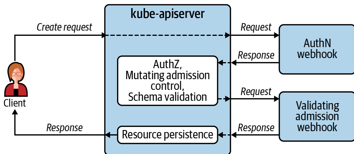
Figure 11-1. Webhook extensions are backend servers leveraged by the Kubernetes API server.
