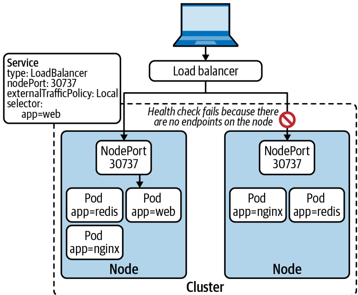
Figure 6-6. LoadBalancer Service with Local external traffic policy. The external load balancer runs health checks against the nodes. Any node that does not have a Service endpoint is removed from the load balancer's backend pool.
