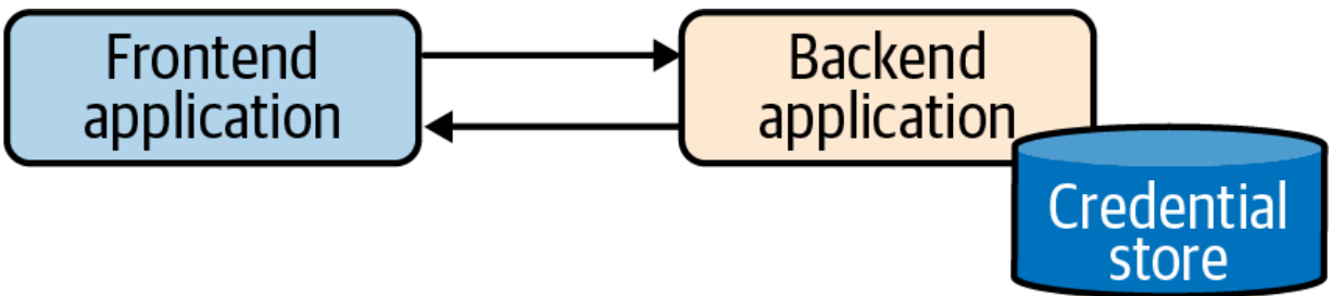
Figure 10-1. Shared secrets flow.
