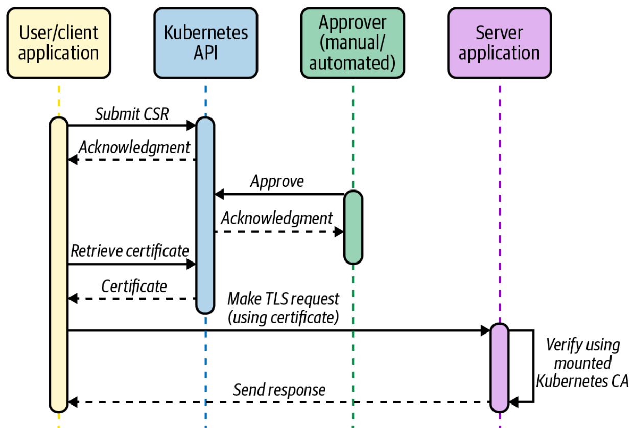
Figure 10-2. CSR flow.
