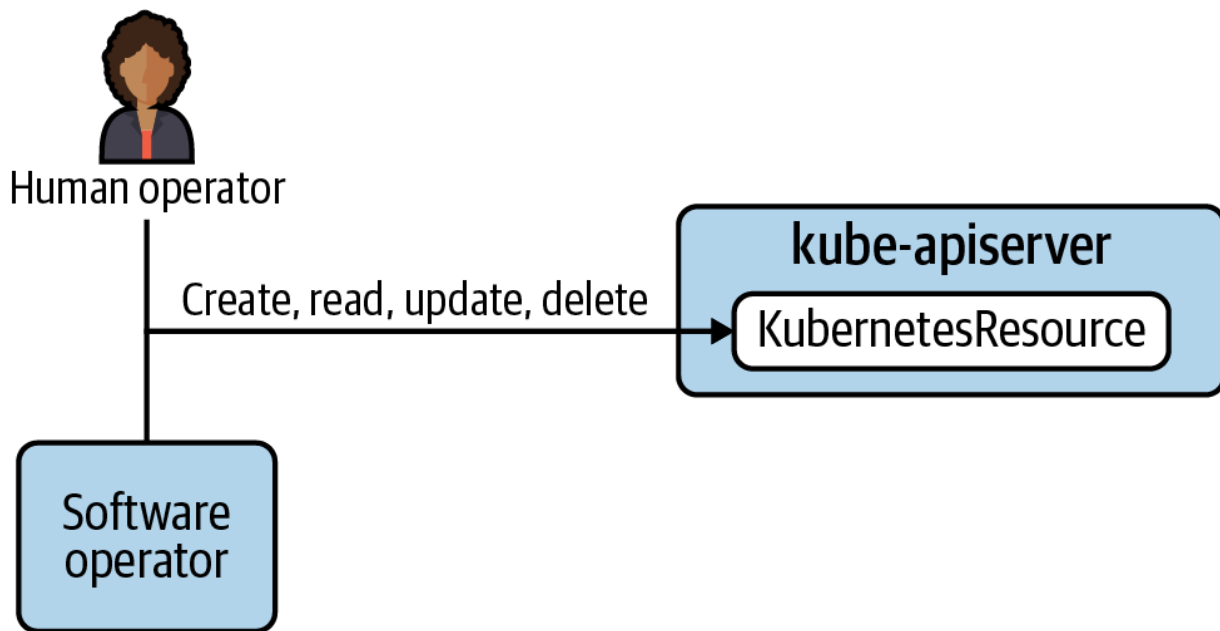
Figure 11-2. Operator extensions are clients of the Kubernetes API server.
