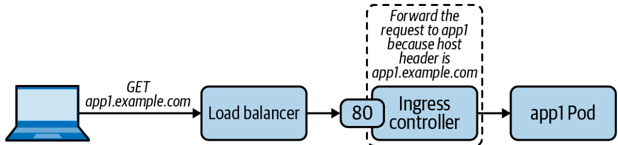
Figure 6-11. Path of an HTTP request from the client to the target Pod through the Ingress controller.
