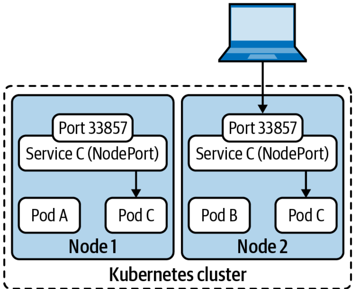
Figure 6-3. The NodePort Service opens a random port on all cluster nodes. Clients outside of the cluster can reach the Service through this port.
