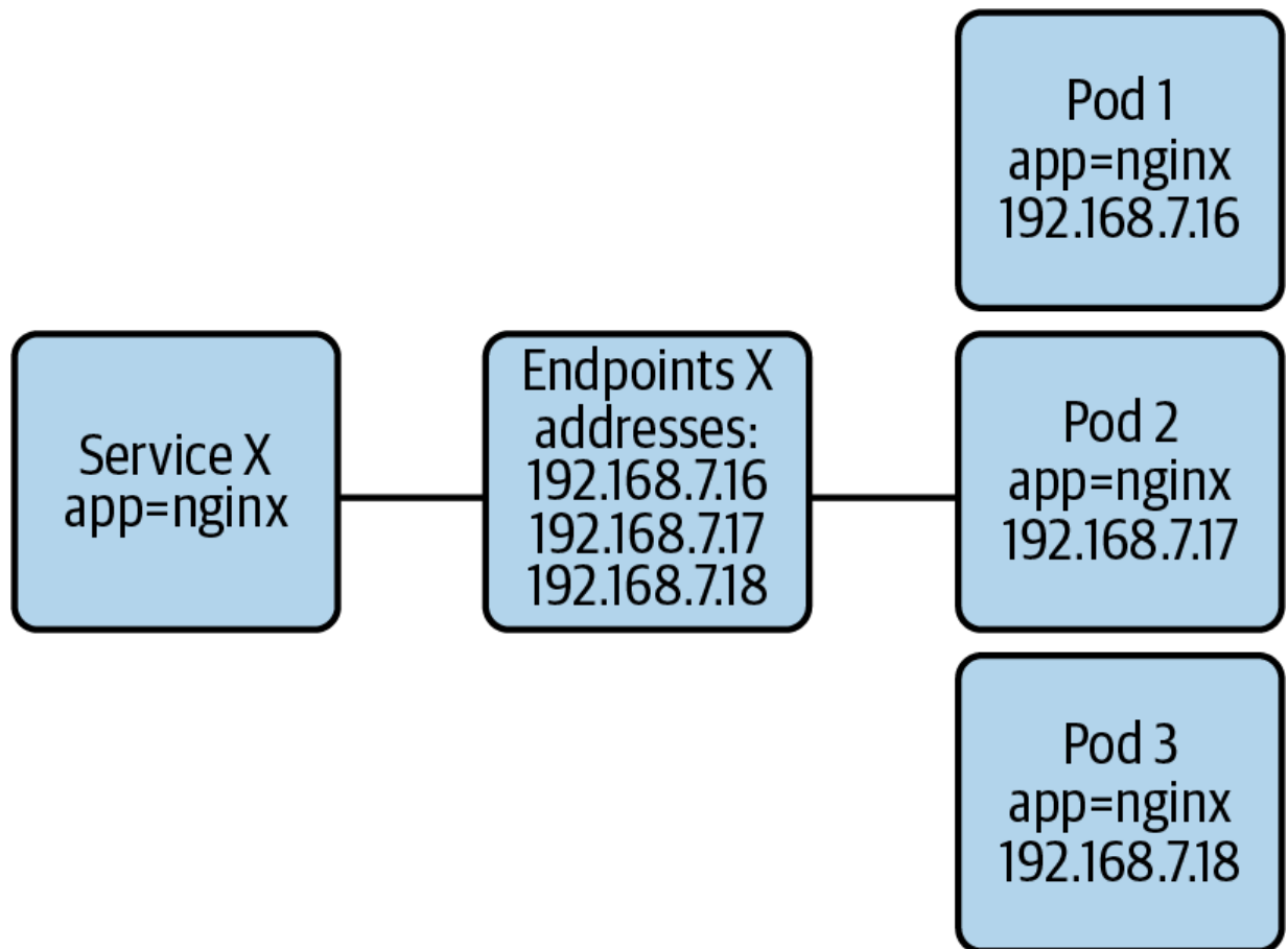
Figure 6-5. Relationship between the Service and the Endpoints resources.
