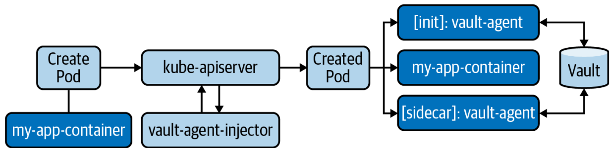
Figure 7-6. Sidecar injection architecture. Along with my-app-container, all Vault Pods are run as sidecars.
