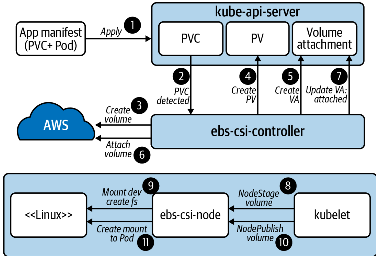
Figure 4-4. End-to-end flow of the driver and Kubernetes working together to satisfy the storage request.
