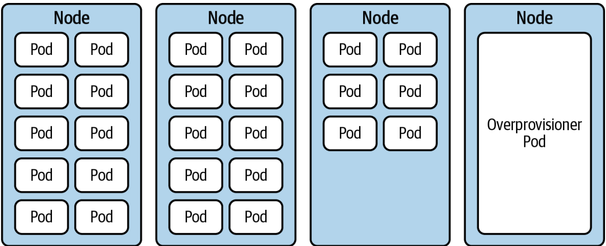
Figure 13-6. Cluster overprovisioning.
