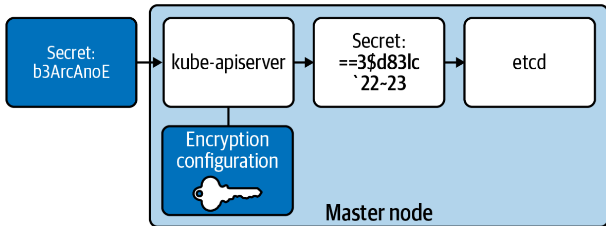
Figure 7-4. The relationship between an encryption key, on the API server, being used to encrypt secrets before storing them in etcd.
