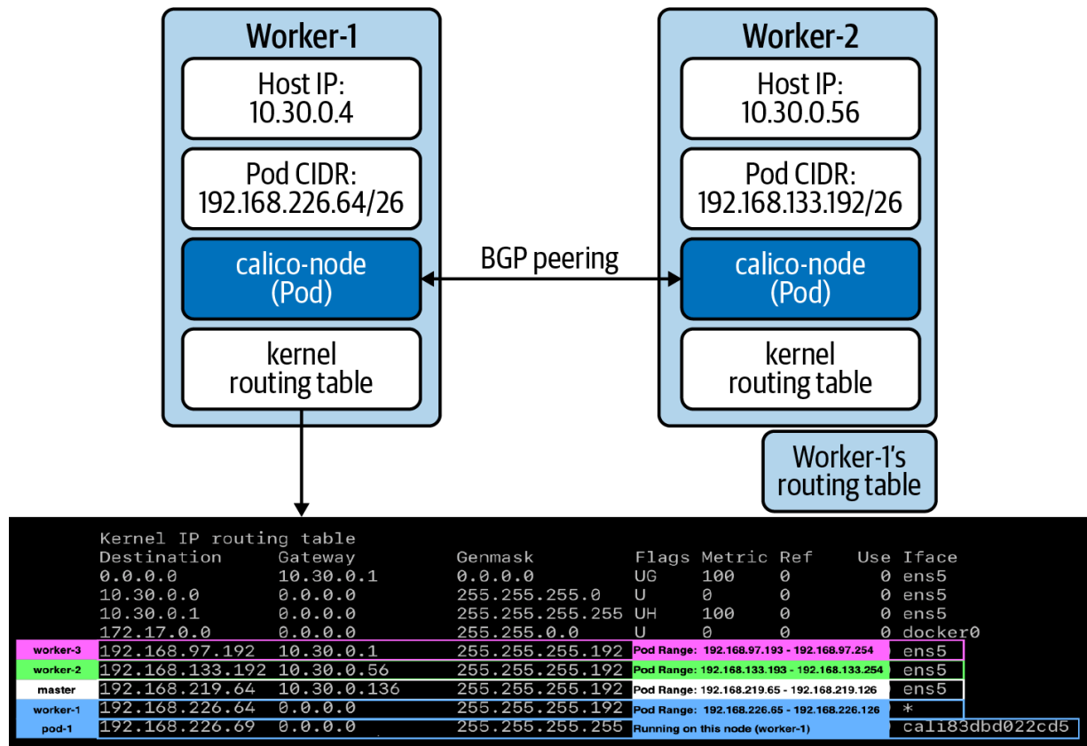
Figure 5-2. The calico-pod sharing routes via its BGP peer. The kernel routing table is then programmed accordingly.
