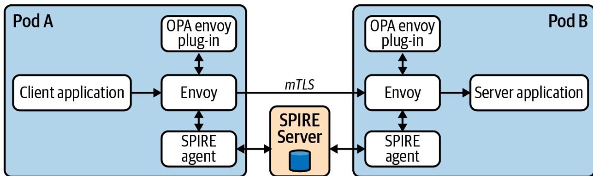
Figure 10-15. SPIRE with Envoy.
