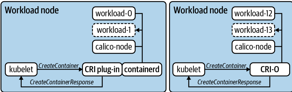
Figure 1-2. Two workload nodes running two different container runtimes. The kubelet sends commands defined in the CRI such as CreateContainer and expects the runtime to satisfy the request and respond.
