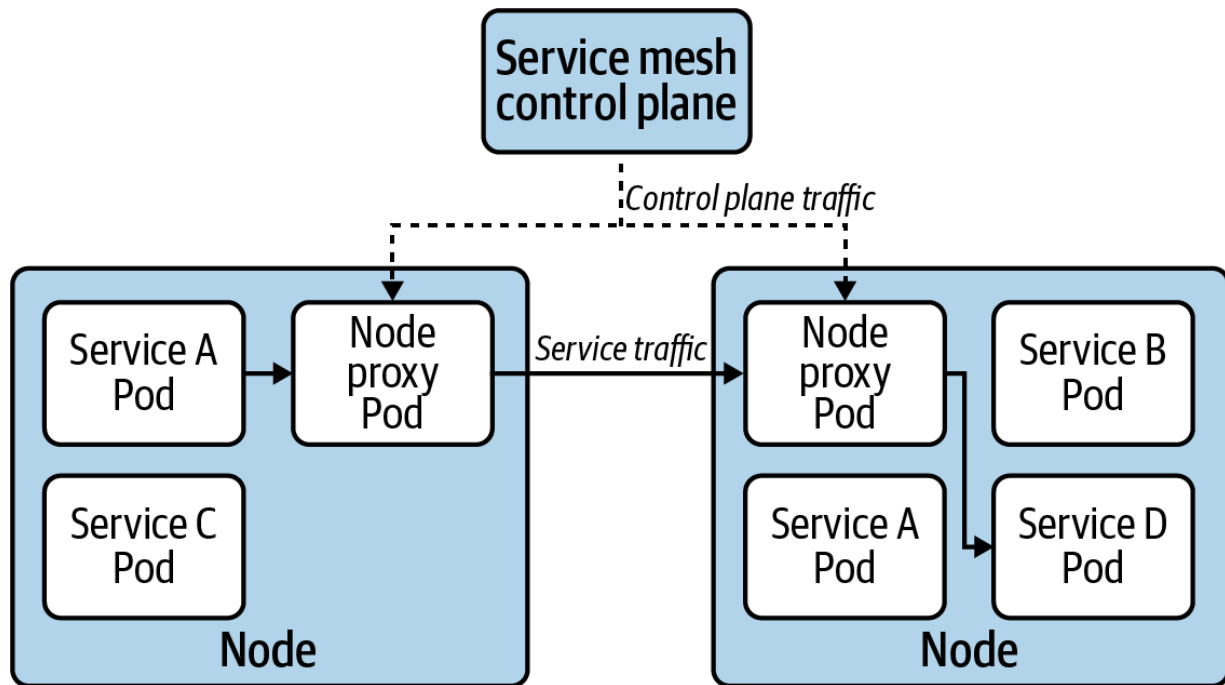
Figure 6-22. The node proxy model involves a single service mesh proxy that handles the traffic for all services on the node.
