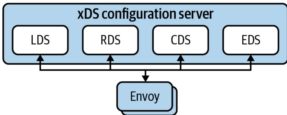
Figure 6-18. Envoy supports dynamic configuration via the XDS APIs. Envoy connects to a configuration server and requests its configuration using LDS, RDS, EDS, CDS, and other xDS APIs.
