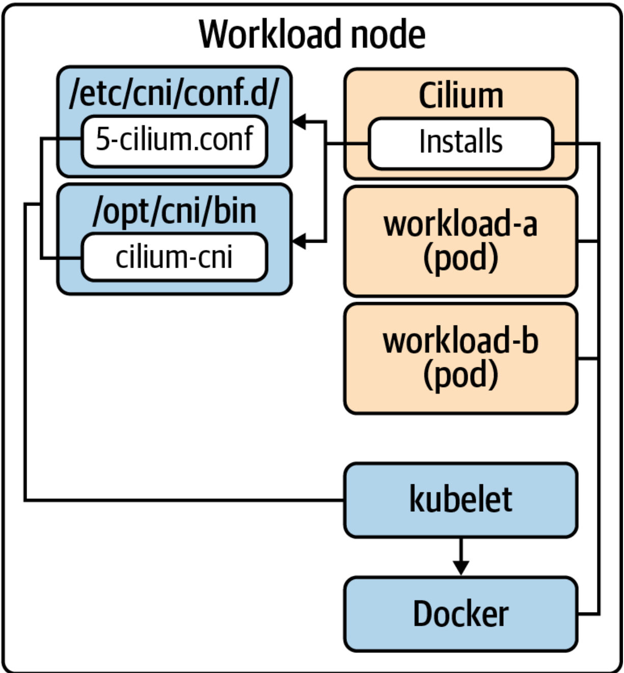
Figure 5-4. Docker is used to run containers. The kubelet interacts with the CNI to attach network interfaces and configure the Pod's network.
