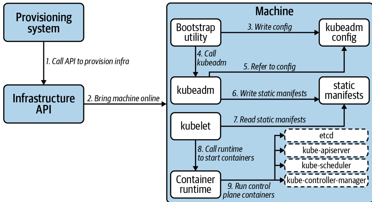
Figure 2-5. Bootstrapping a machine to initialize Kubernetes.
