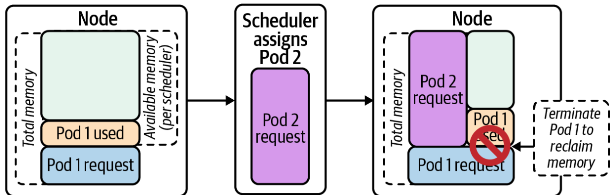
Figure 12-3. Pod consuming memory above its request is terminated to reclaim memory for the new Pod.
