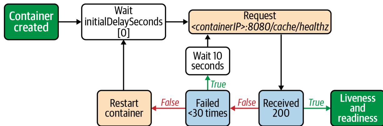
Figure 14-4. Flowchart that shows an HTTP-based startup probe with a period of 10 seconds. If the probe returns a successful response, the startup probe is disabled and the liveness/readiness probes are enabled. Otherwise, if the probe fails 30 times consecutively, the kubelet restarts the Pod.
