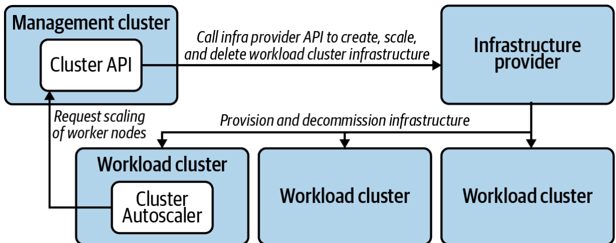
Figure 2-1. Cluster Autoscaler accessing a management cluster to trigger scaling events.
