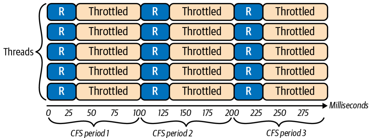
Figure 12-5. Multithreaded application consumes the entire CPU quota in the first 20 milliseconds of the 100-millisecond period.
