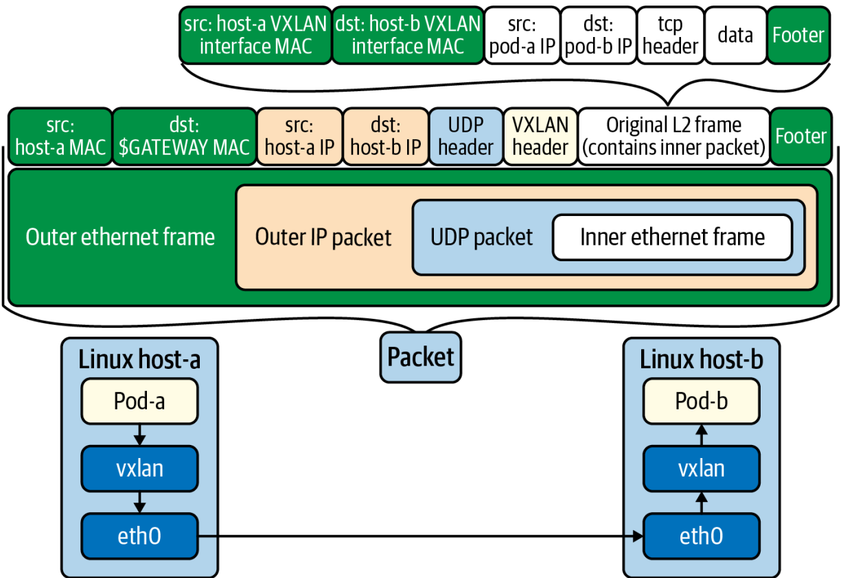
Figure 5-3. VXLAN encapsulation used to move an inner packet, for workloads, across hosts. The network cares only about the outer packet, so it needs to have zero awareness of workload IPs and their routes.
