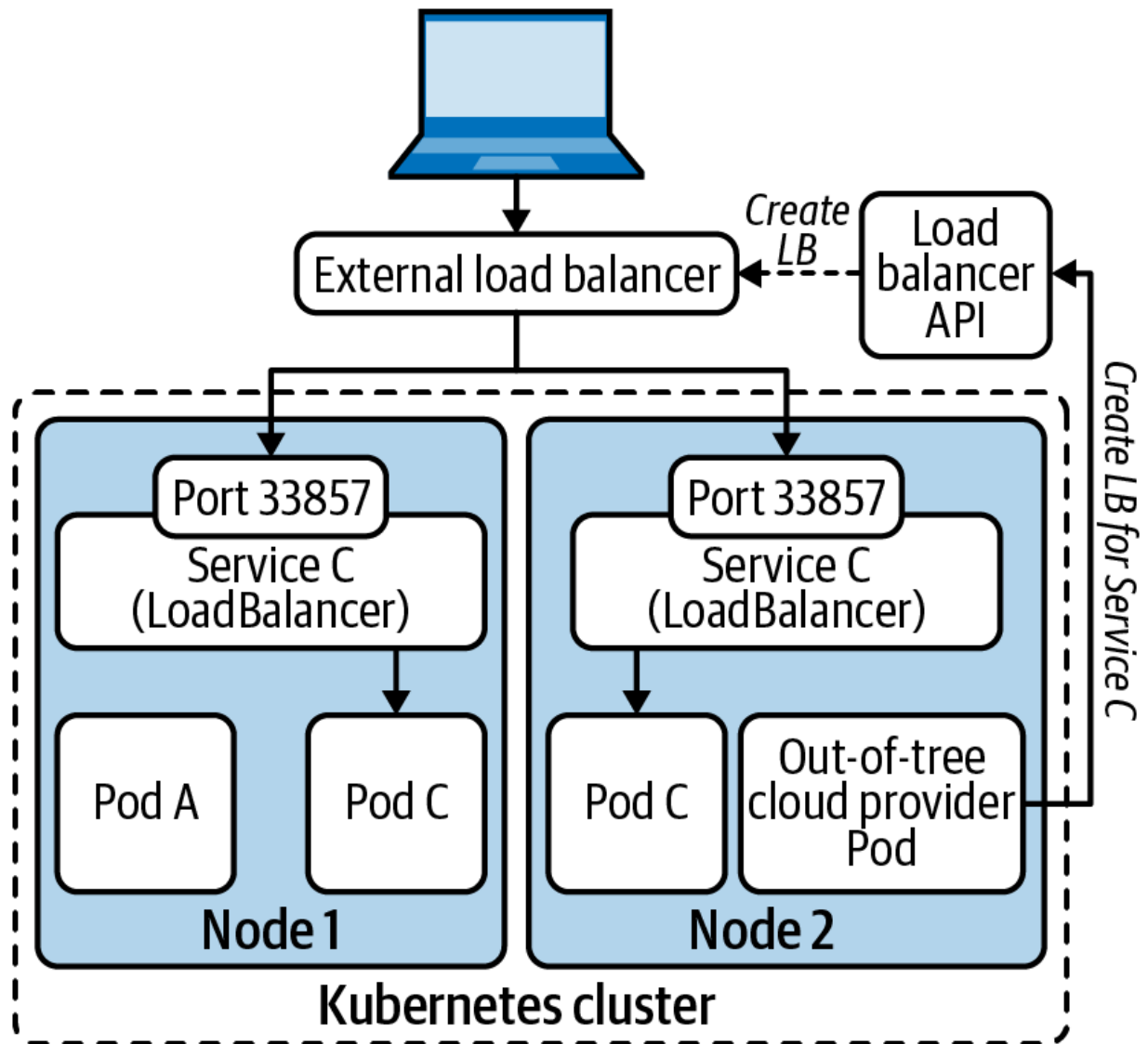
Figure 6-4. The LoadBalancer Service leverages a cloud provider integration to create an external load balancer, which forwards traffic to the node ports. At the node level, the Service is the same as a NodePort.
