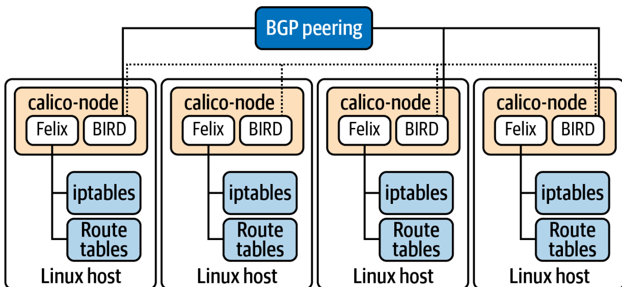
Figure 5-5. Calico component relationship showing the BGP peering to communicate routes and the programming of iptables and kernel routing tables accordingly.
