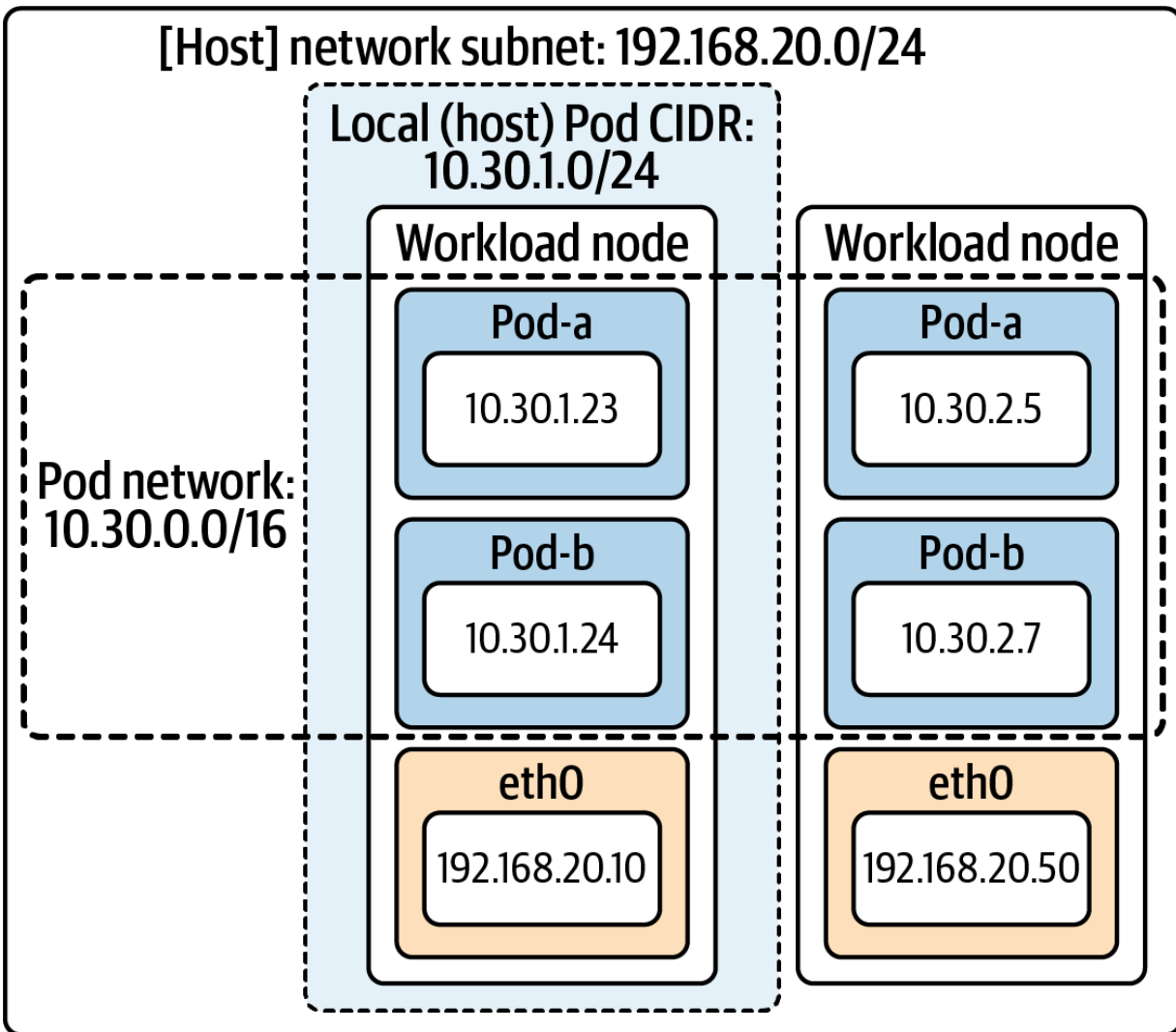
Figure 5-1. The IP spaces and IP allocations of the host network, Pod network, and each [host] local CIDR.
