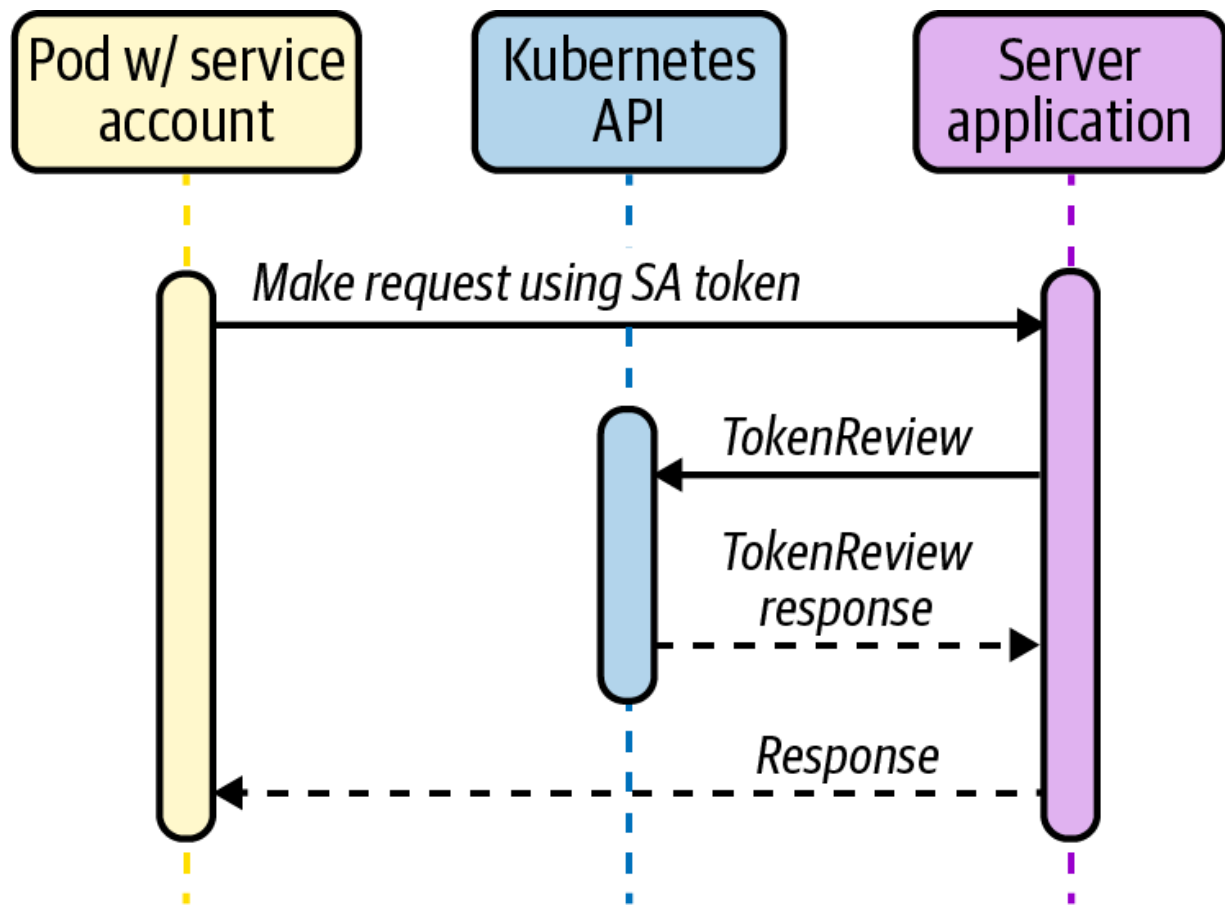
Figure 10-5. Service Account tokens.
