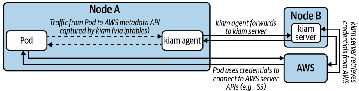
Figure 10-9. kiam architecture and data flow.
