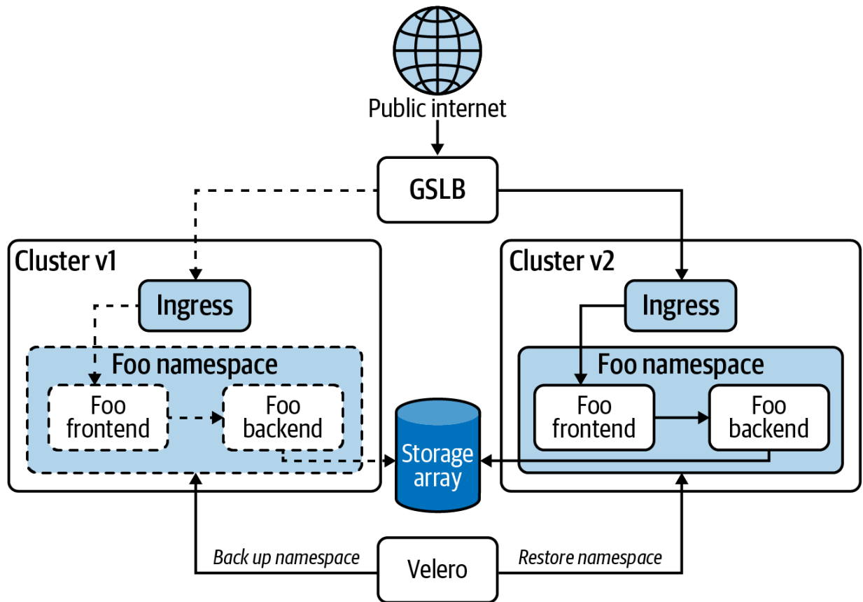
Figure 2-6. Migrating workloads between clusters with a backup and restore using Velero.
