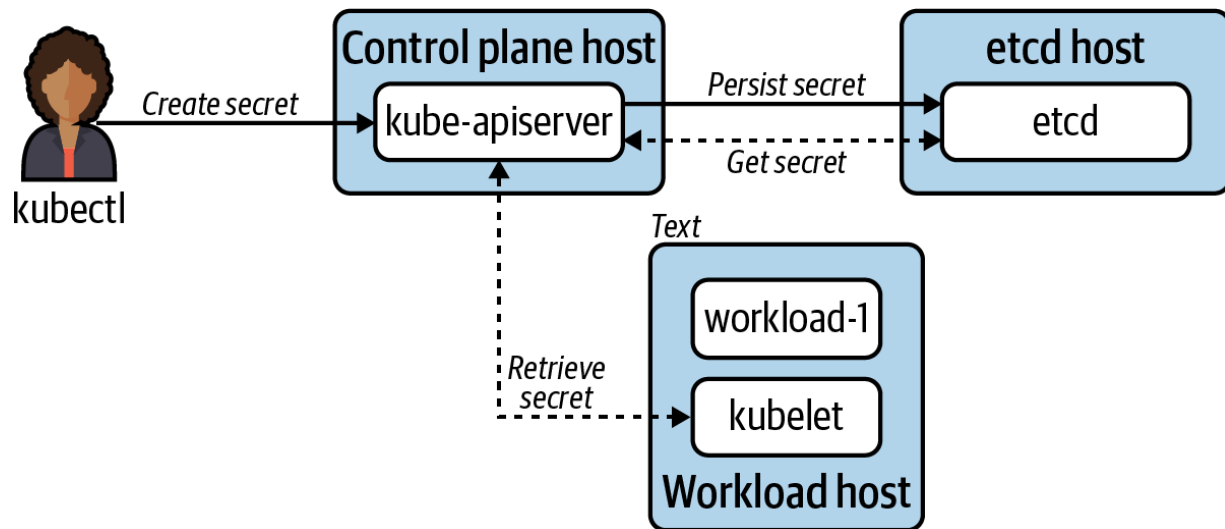
Figure 7-2. Diagram demonstrating points where a secret may pass over the wire.
