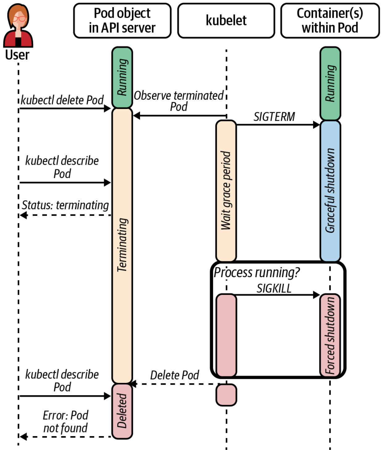
Figure 14-1. Application termination in Kubernetes. The kubelet first sends a SIGTERM signal to the workload and waits up to the configured graceful termination period. If the process is still running after the period expires, the kubelet sends a SIGKILL to terminate the process.
