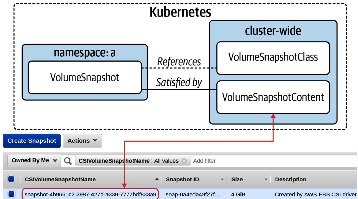
Figure 4-5. The various objects and their relations that make up the snapshot flow.
