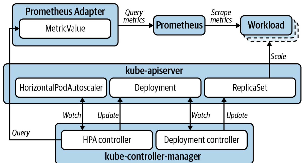
Figure 13-3. Horizontal Pod autoscaling with custom metrics.
