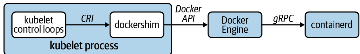
Figure 3-2. Interaction between the kubelet and Docker Engine via the dockershim.
