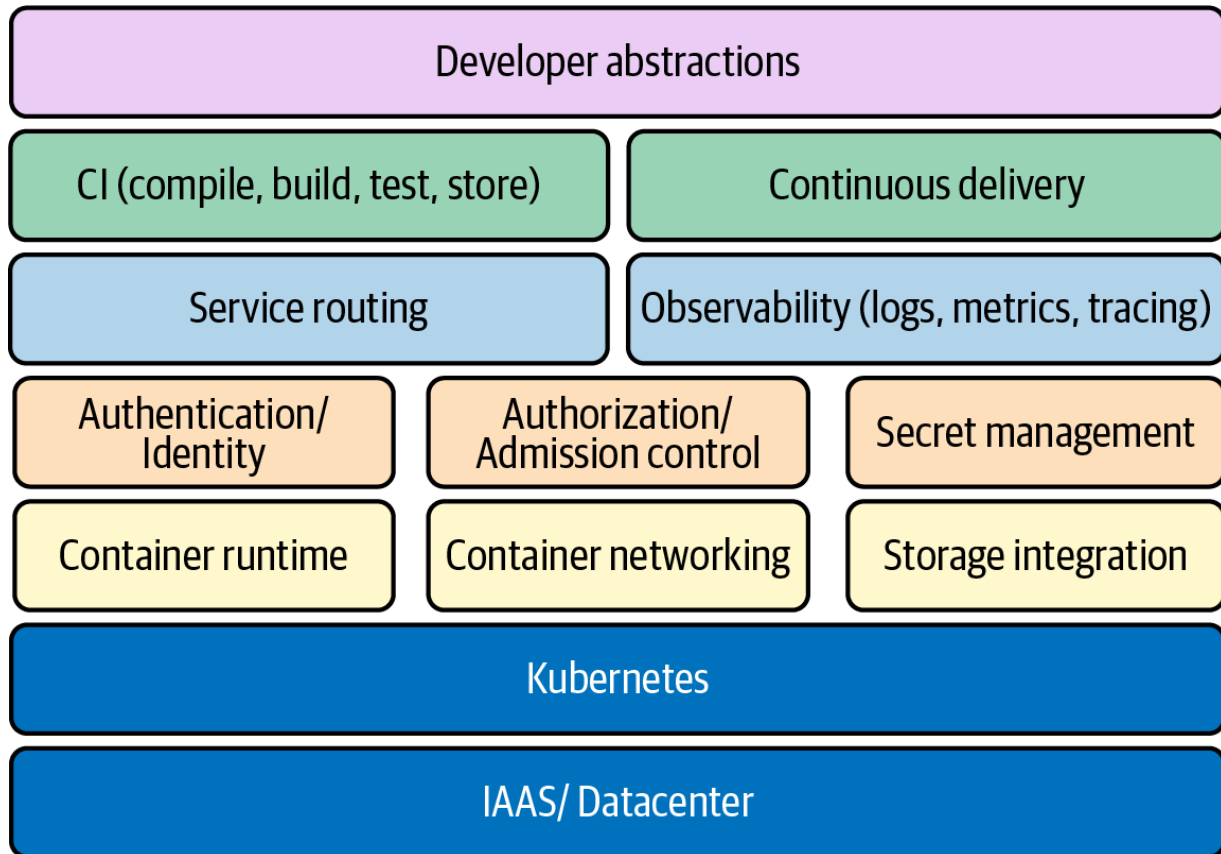
Figure 1-10. Many of the key building blocks involved in establishing an application platform.
