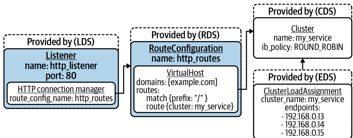
Figure 6-19. Envoy configuration with a Listener that binds to port 80. The Listener has an HTTP connection manager filter that references a routing configuration. The routing config matches requests with / prefix and forwards requests to the my_service cluster, which has three endpoints.
