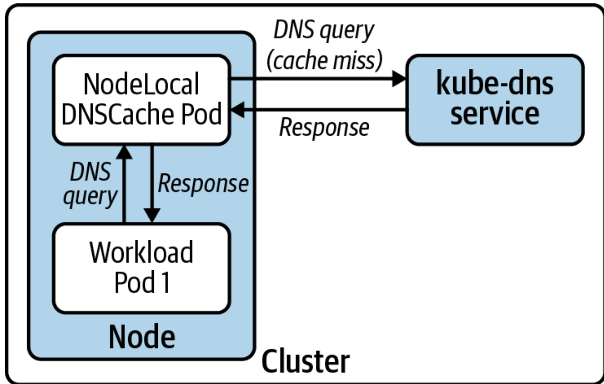
Figure 6-9. Node-level architecture of the NodeLocal DNSCache add-on. The DNS cache intercepts DNS queries and responds immediately if there's a cache hit. In the case of a cache miss, the DNS cache forwards the query to the cluster DNS service.
