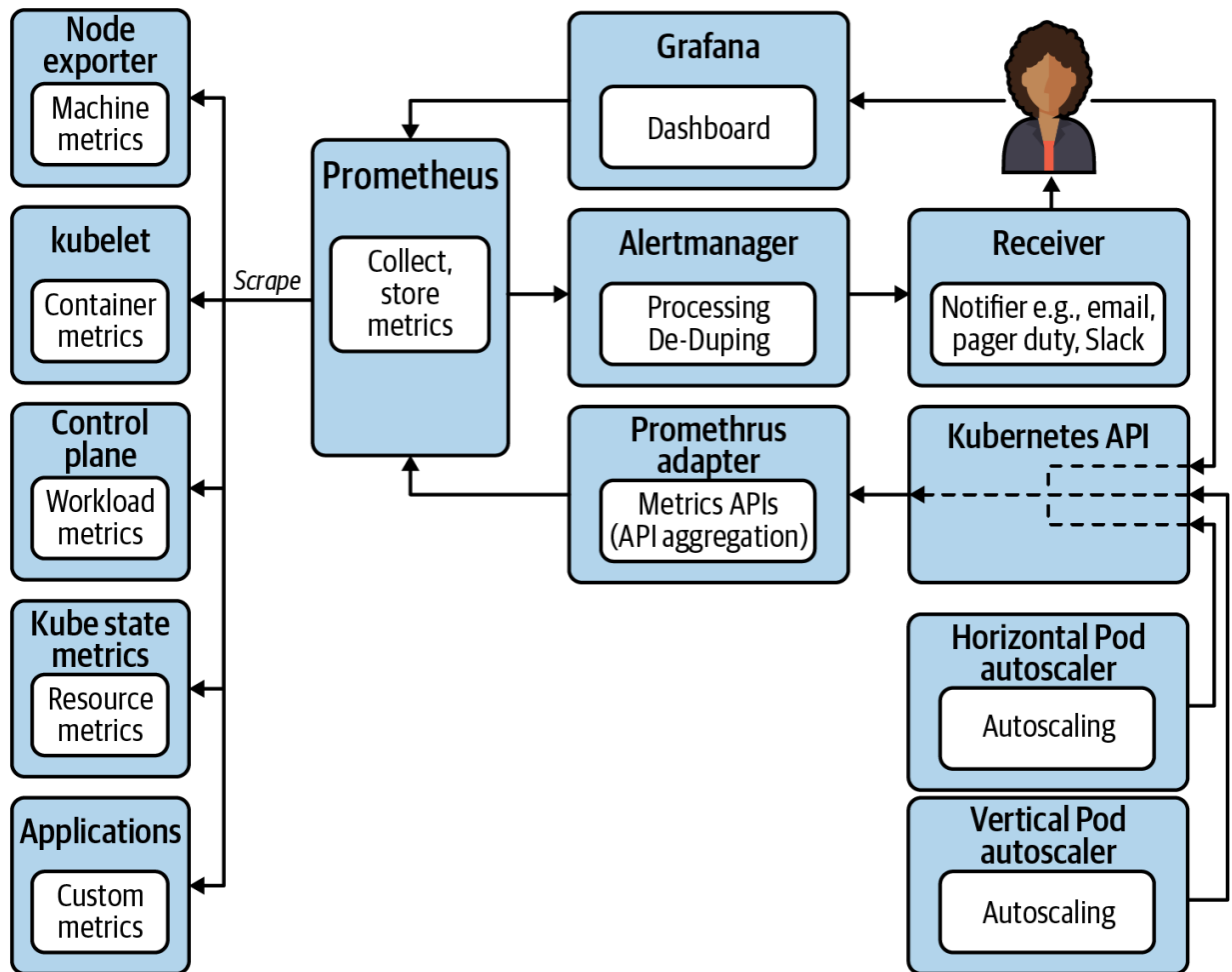
Figure 9-7. Common components in a Prometheus metrics stack.
