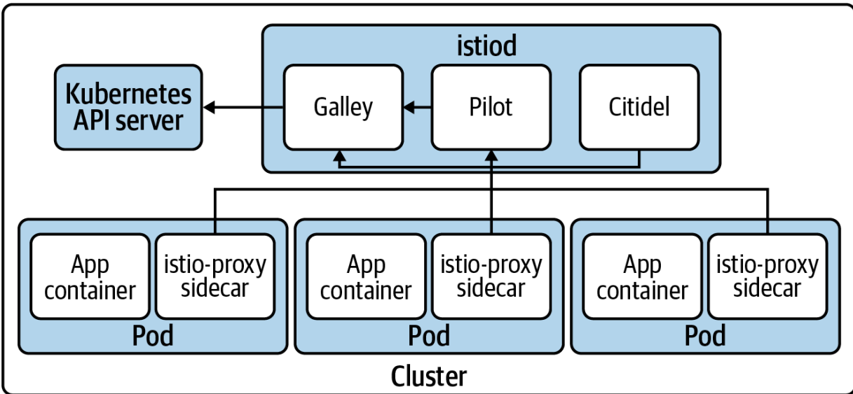
Figure 6-20. Istio control plane interactions.
