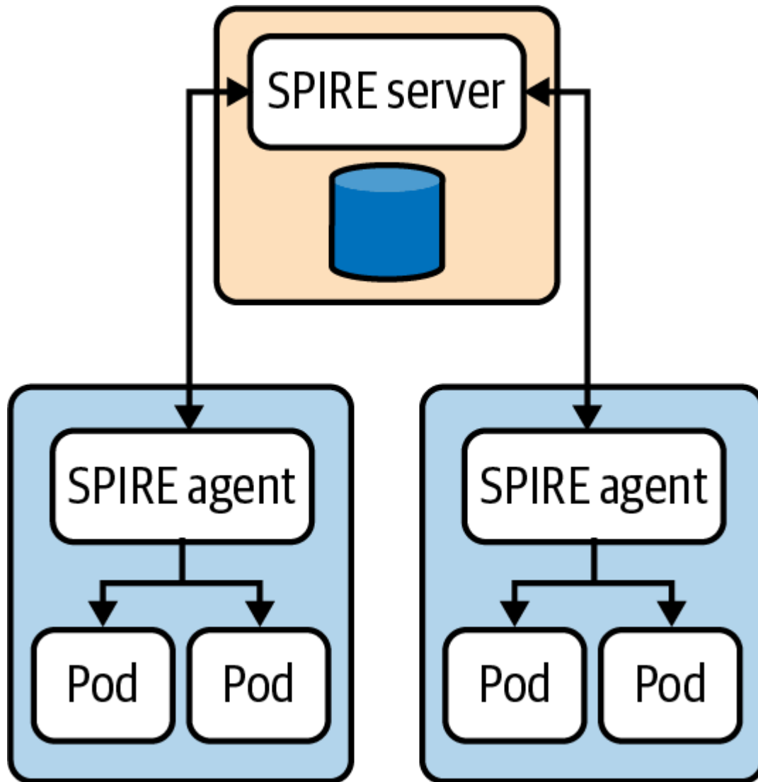
Figure 10-12. SPIRE Architecture. Reproduced from the official SPIRE documentation .
