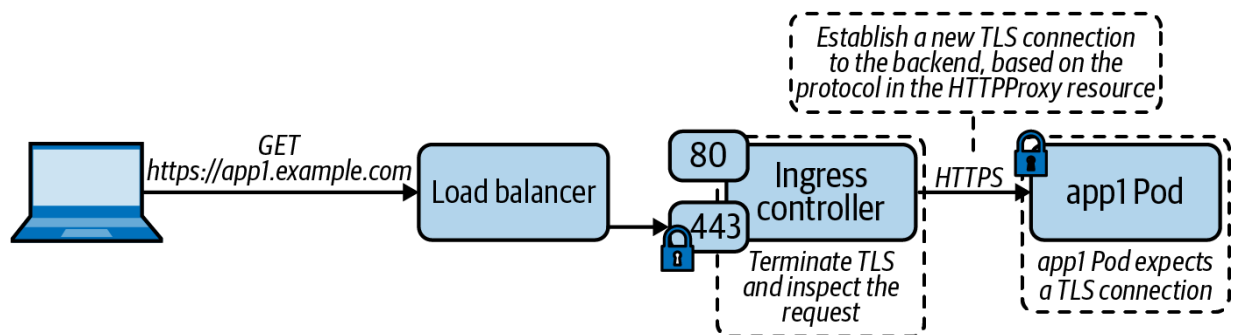
Figure 6-13. Ingress controller terminating TLS and establishing a new TLS connection with the backend Pod when handling HTTPS requests.
