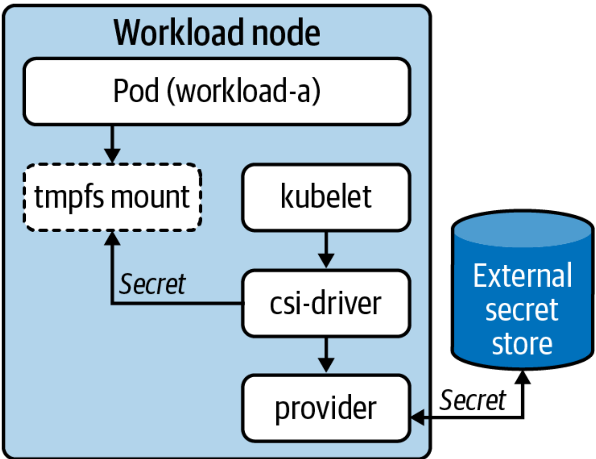
Figure 7-7. CSI driver interaction flow.
