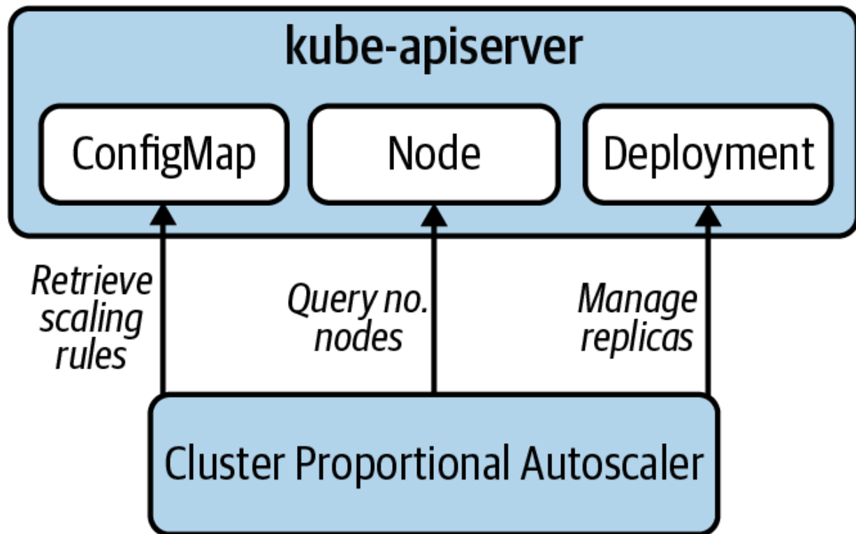
Figure 13-4. Cluster proportional autoscaling.
