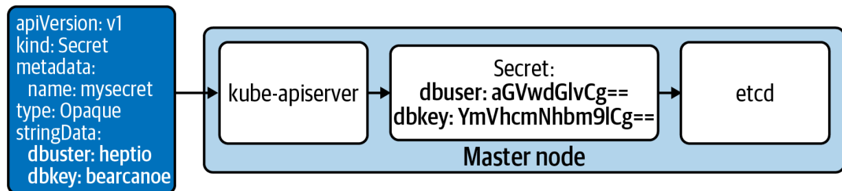
Figure 7-3. Default secret data flow in Kubernetes (the colocated etcd is sometimes run on a separate host).
