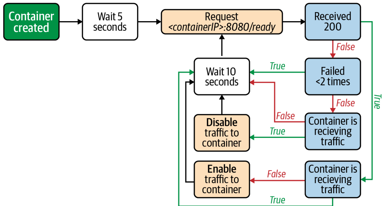
Figure 14-3. Flowchart that shows an HTTP-based readiness probe with a period of 10 seconds. If the probe fails twice consecutively, the Pod is deemed not ready and it is taken out of the set of ready endpoints.
