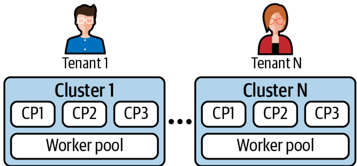
Figure 12-1. Each tenant runs in a separate cluster (CP represents a control plane node).
