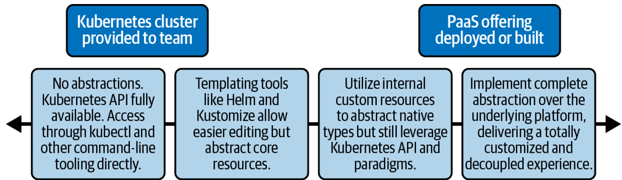
Figure 16-1. Spectrum of abstraction.
