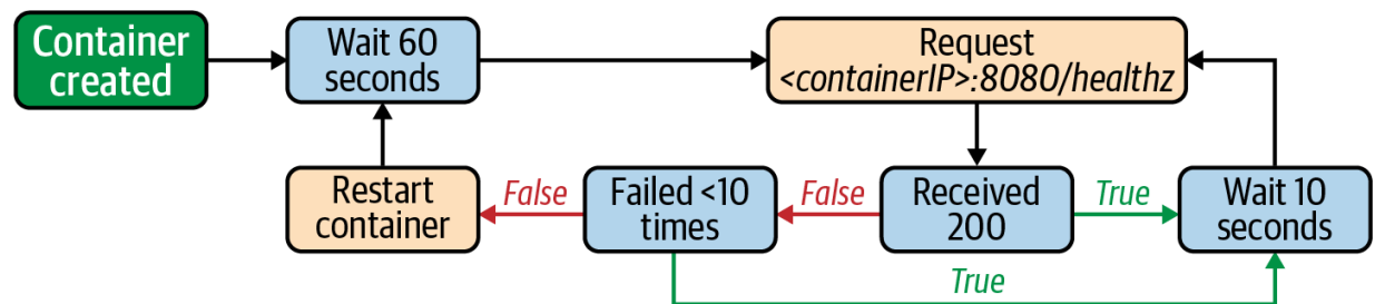
Figure 14-2. Flowchart that shows an HTTP-based liveness probe with a period of 10 seconds. If the probe fails 10 times consecutively, the Pod is deemed unhealthy and the kubelet restarts it.
