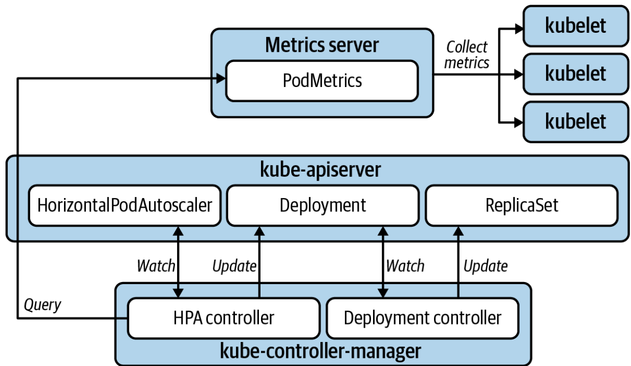
Figure 13-1. Horizontal Pod autoscaling.
