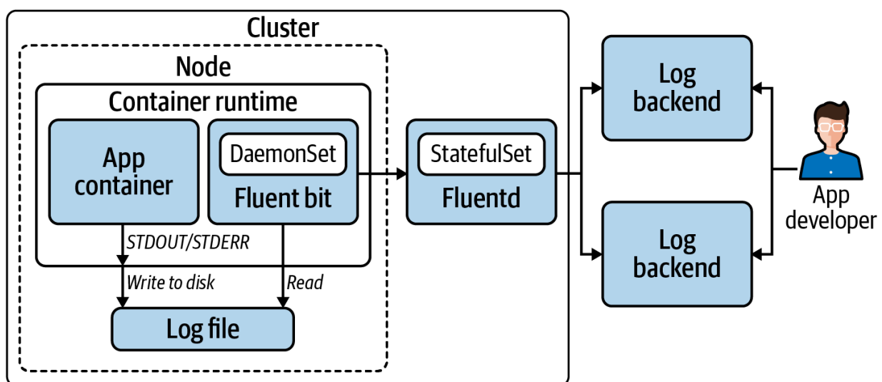
Figure 9-1. Aggregation of logs from containerized apps to backend.
