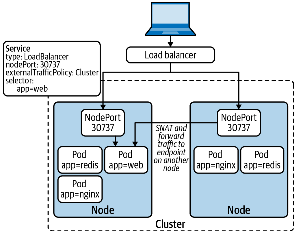
Figure 6-7. LoadBalancer Service with Cluster external traffic policy. Nodes that do not have node-local endpoints forward the traffic to an endpoint on another node.
