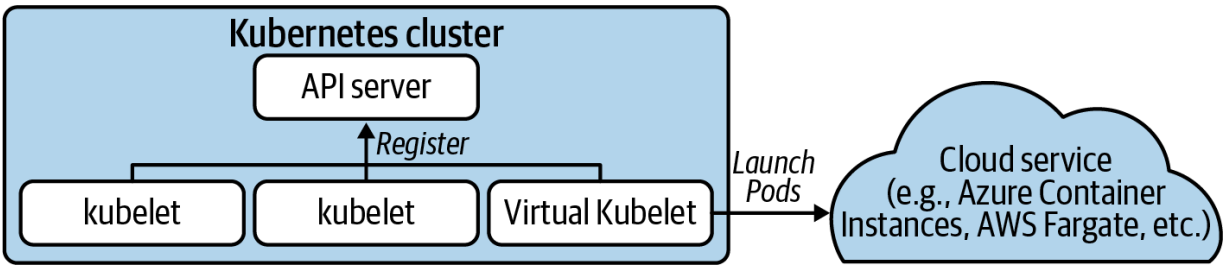
Figure 3-6. Virtual Kubelet running Pods on a cloud service, such as Azure Container Instances, AWS Fargate, etc.
