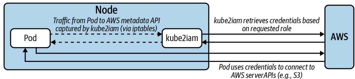
Figure 10-8. kube2iam architecture and data flow.
