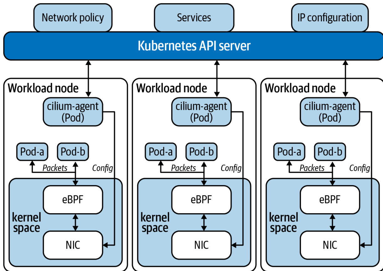
Figure 5-7. Cilium interacts with eBPF maps and programs at the kernel level.
