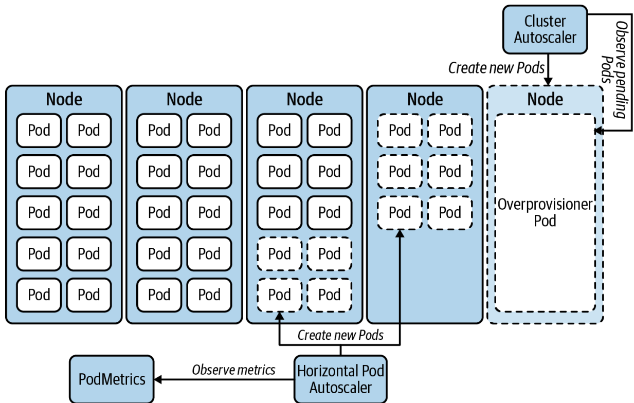
Figure 13-7. Scaling out with cluster-overprovisioner.
