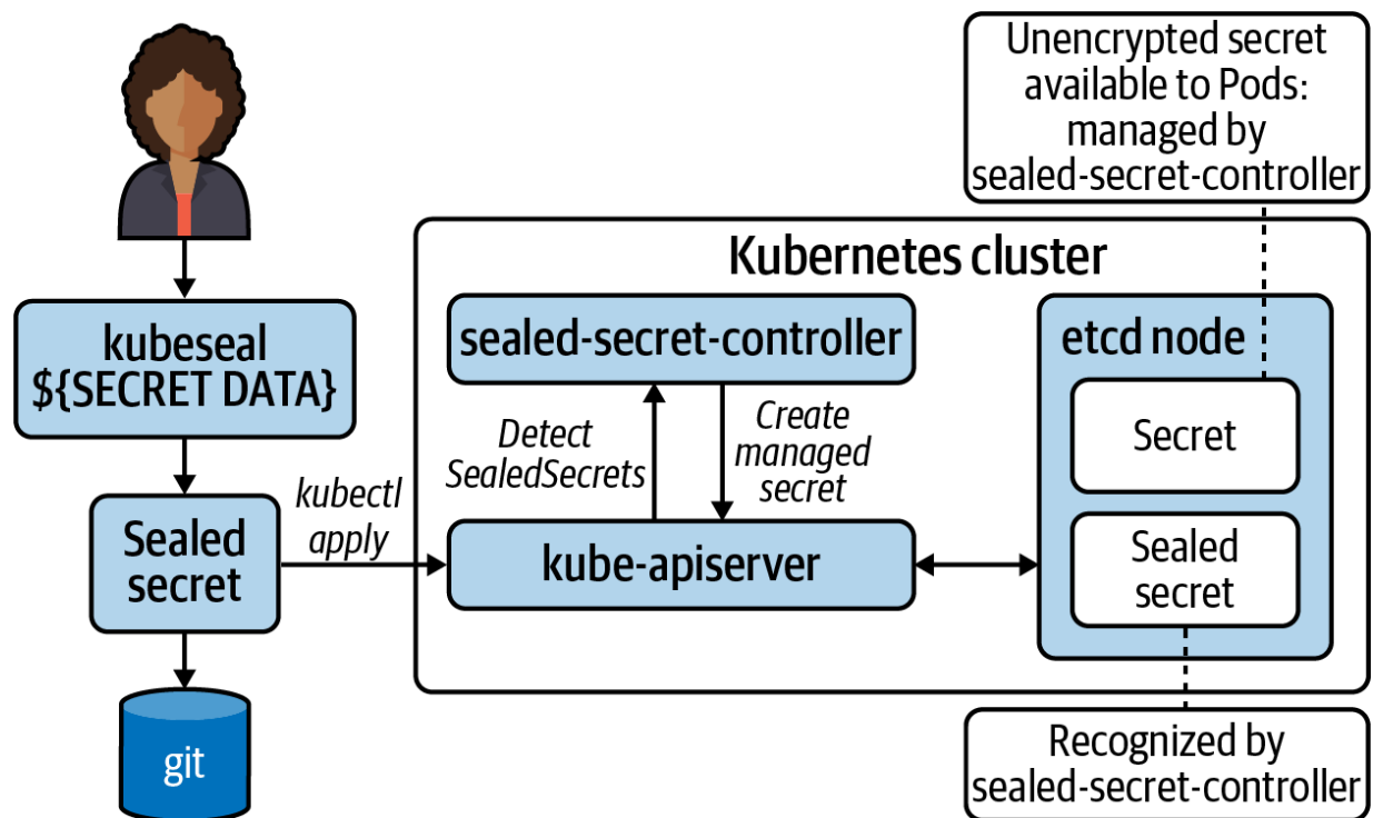
Figure 7-9. Sealed-secret-controller interaction around managing sealed and unsealed secrets.
