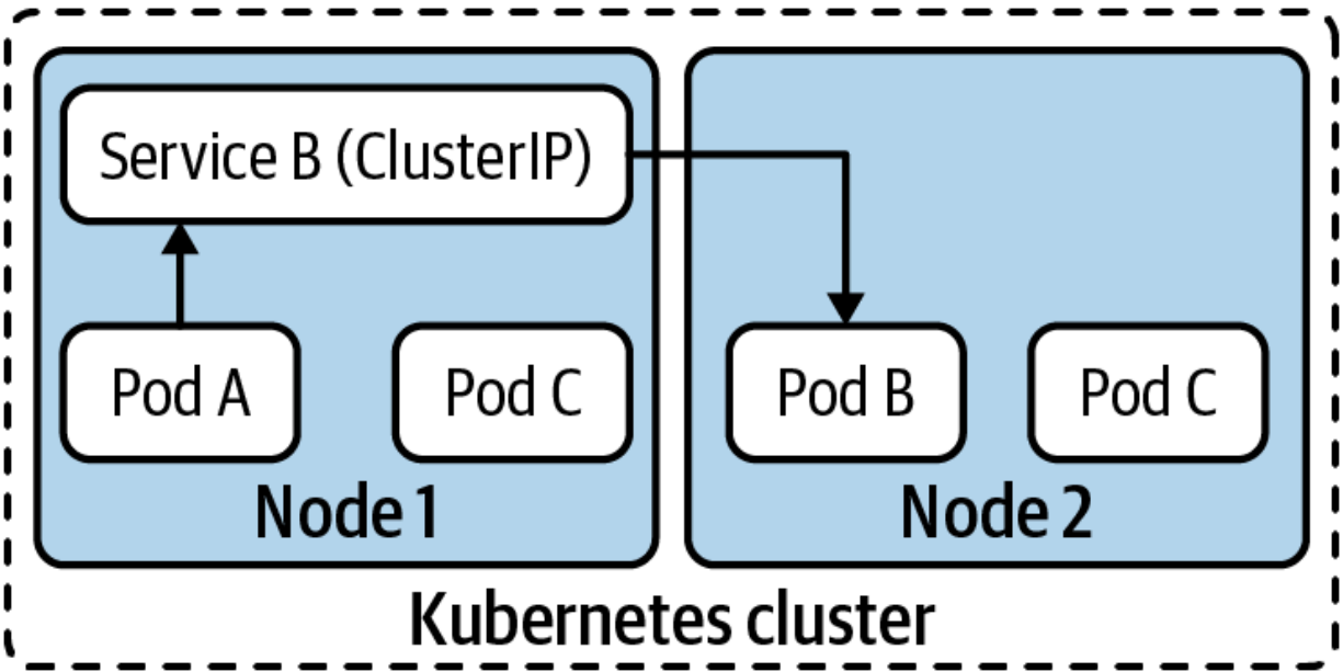
Figure 6-2. The ClusterIP Service is a VIP that is accessible to workloads running within the cluster.
