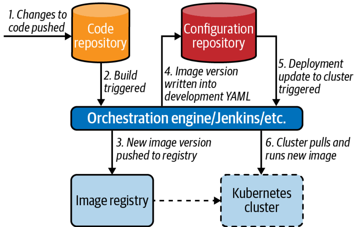
Figure 15-4. Push-based deployments.
