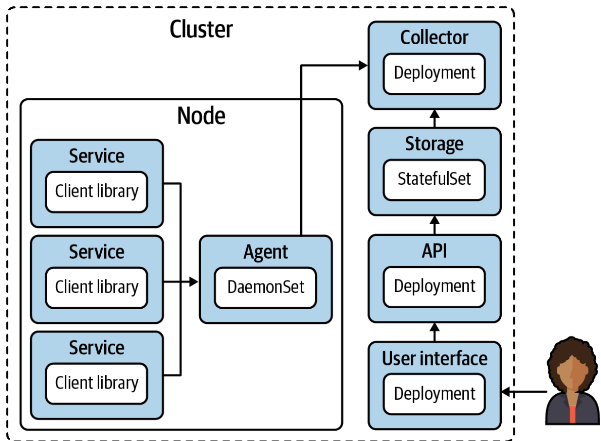
Figure 9-8. Components of a tracing platform service.
