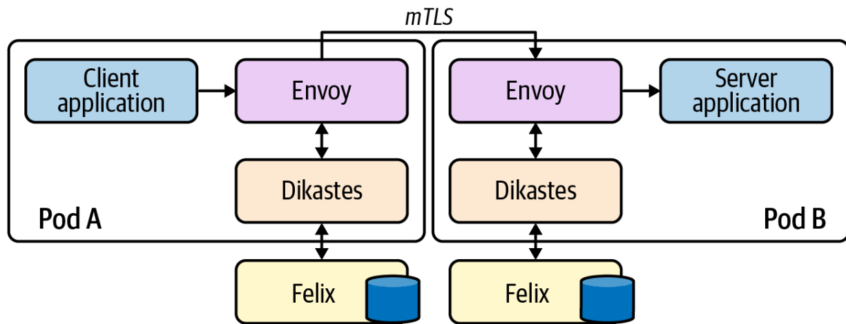
Figure 10-4. Architecture diagram using Dikastes with Envoy.
