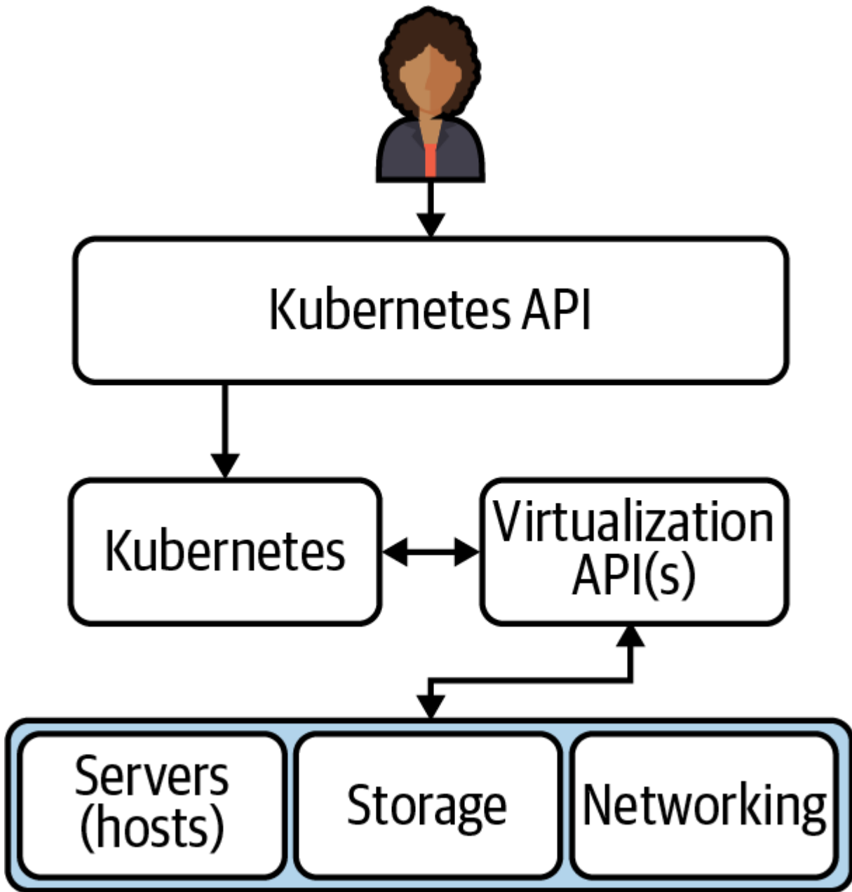
Figure 2-4. Operator interactions when using Kubernetes.
