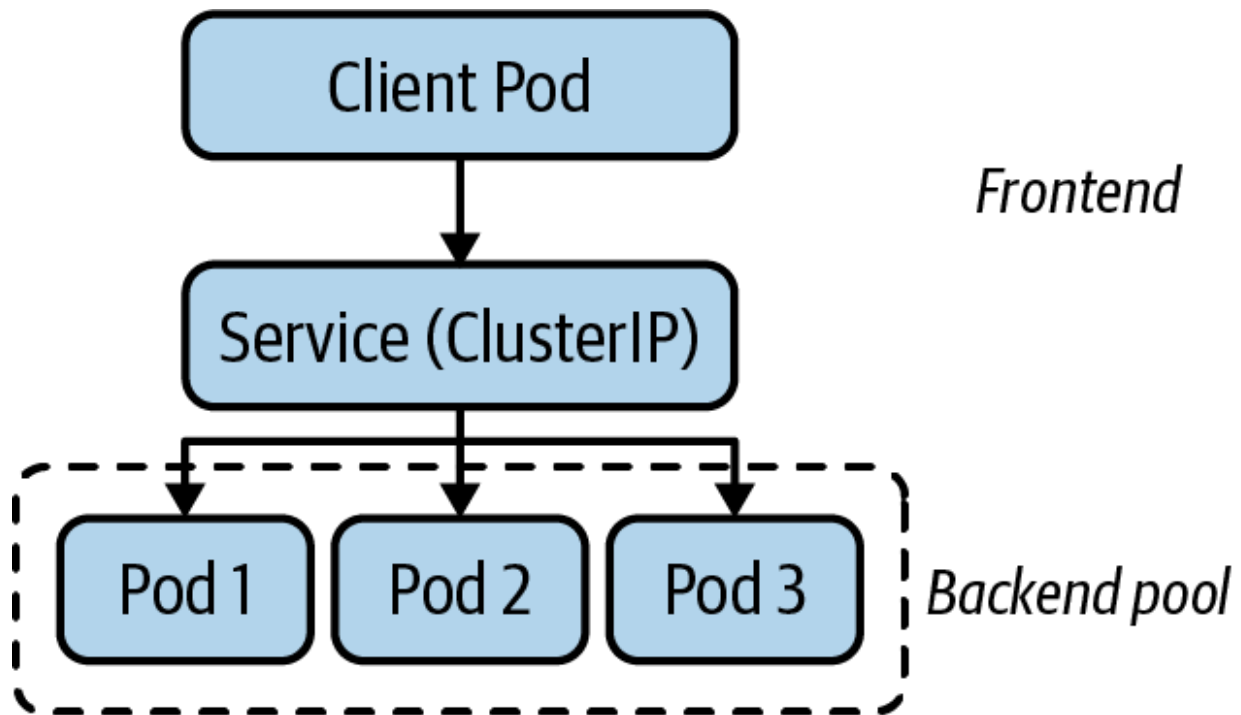
Figure 6-1. The Service has a frontend and a backend pool. The frontend is the ClusterIP, while the backend is a set of Pods.
