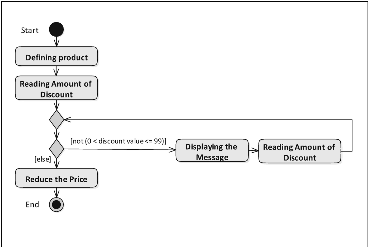
Figure 4-5 Simple while statement
