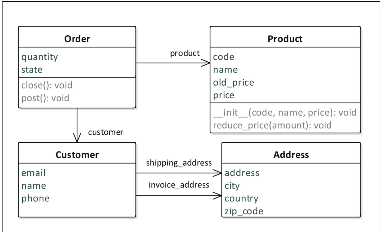
Figure 3-7 The order and the associated classes
