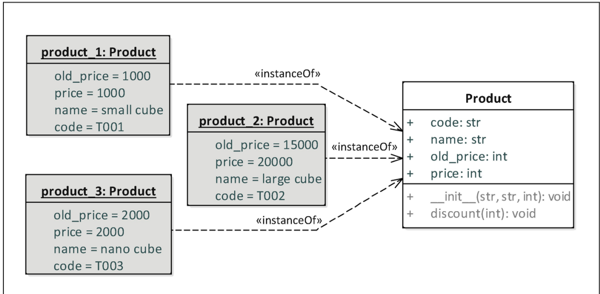
Figure 3-2 Product objects and class
