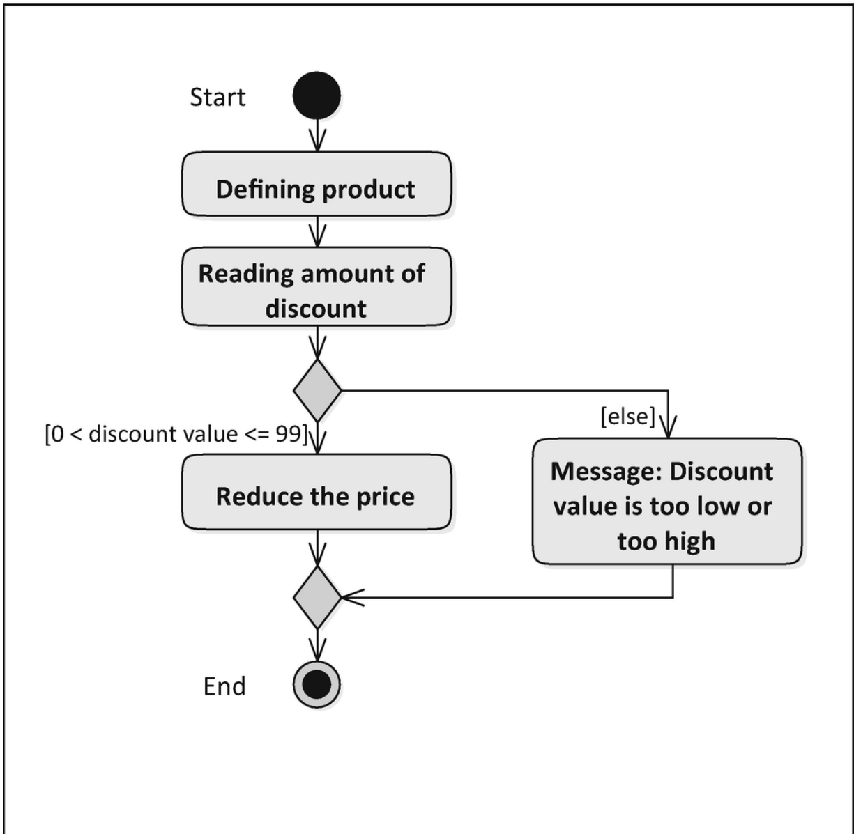
Figure 4-1 Simple if statement
