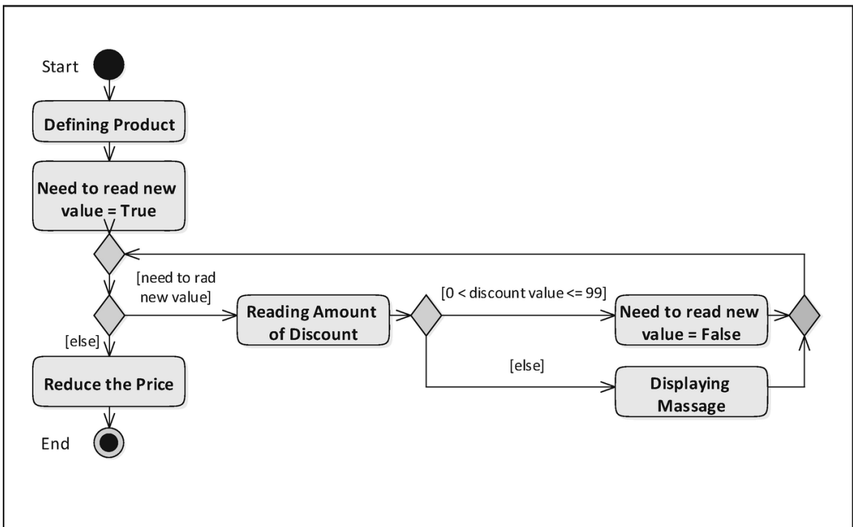
Figure 4-6 while statement with a status variable
