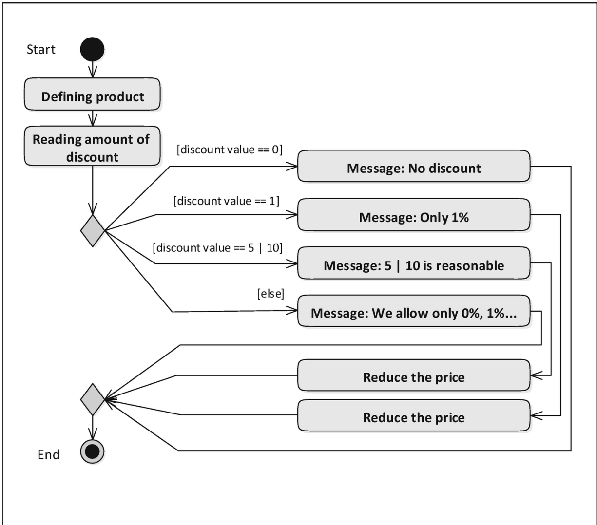
Figure 4-3 match statement with literals
