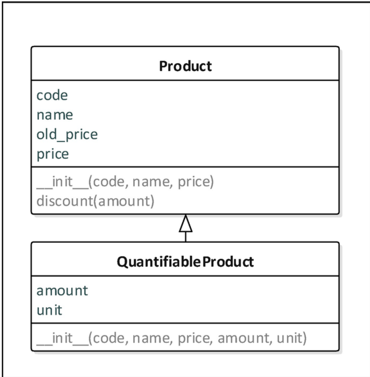
Figure 3-8 Inheritance among classes
