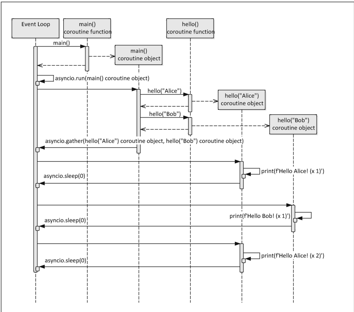
Figure C-2 Execution of multiple native coroutines
