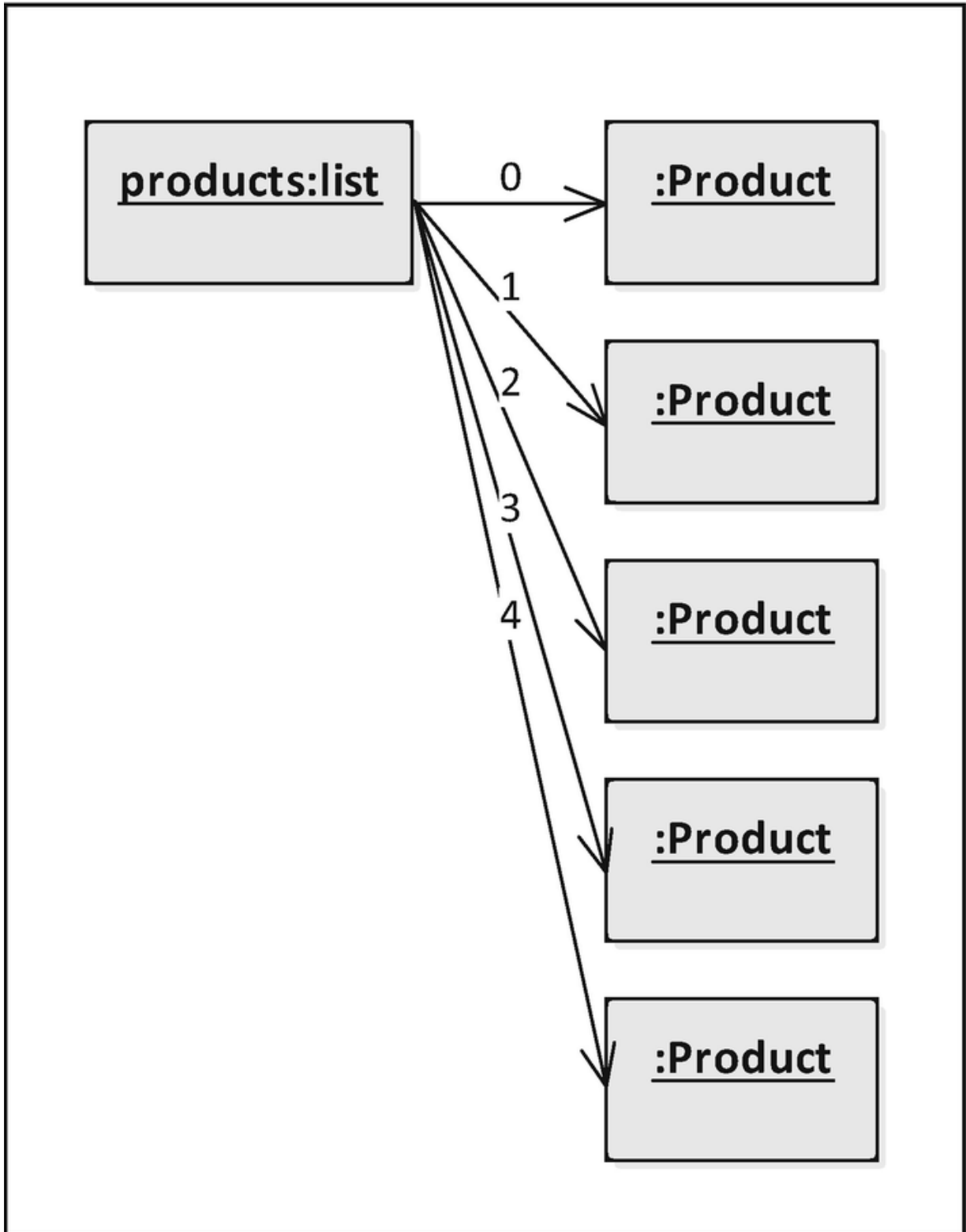
Figure 5-2 List of products
