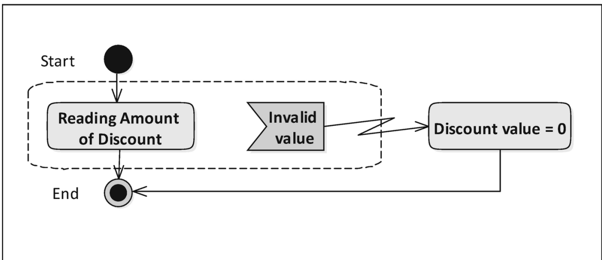
Figure 4-10 Exception handling
