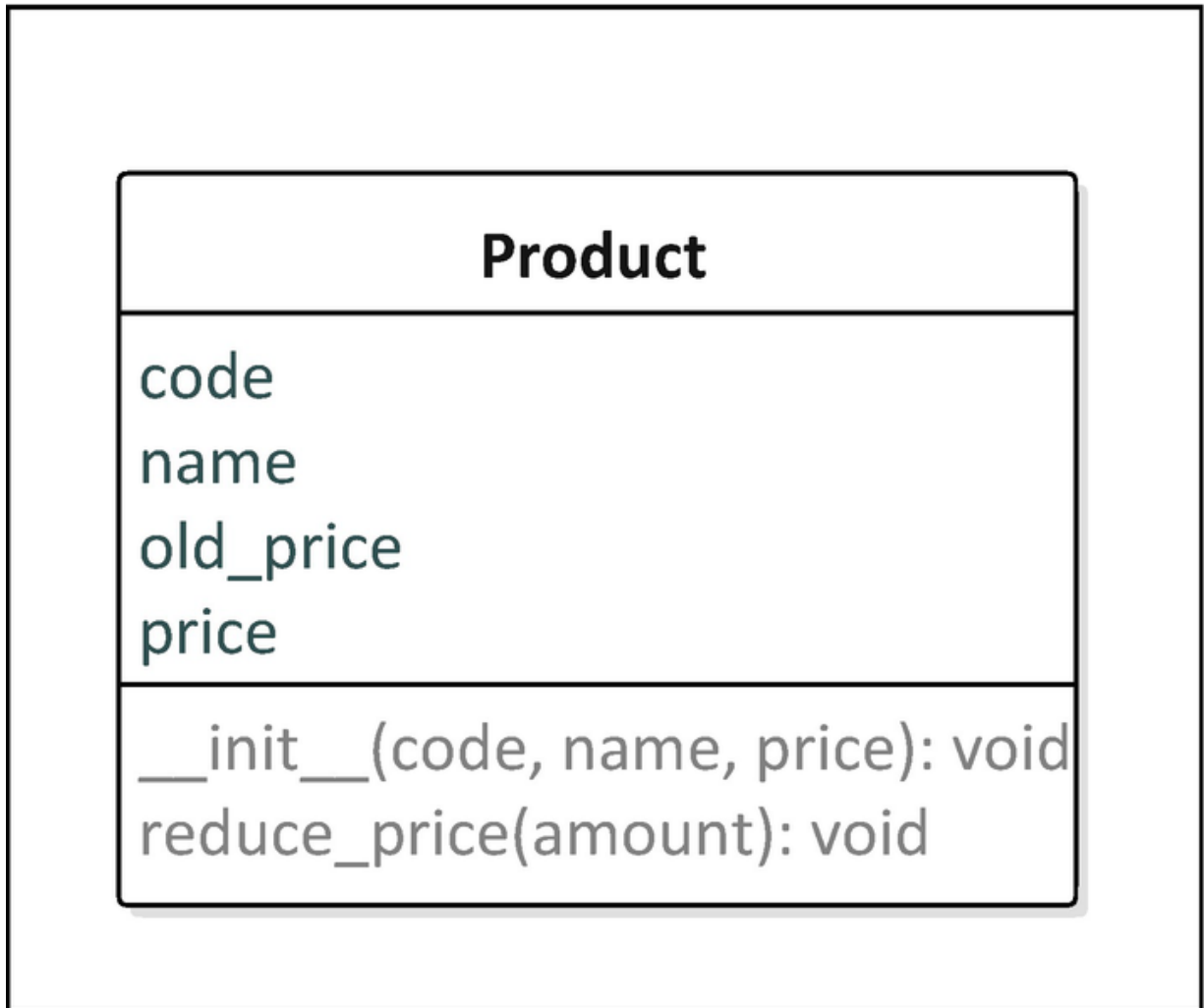
Figure 3-4 Product class
