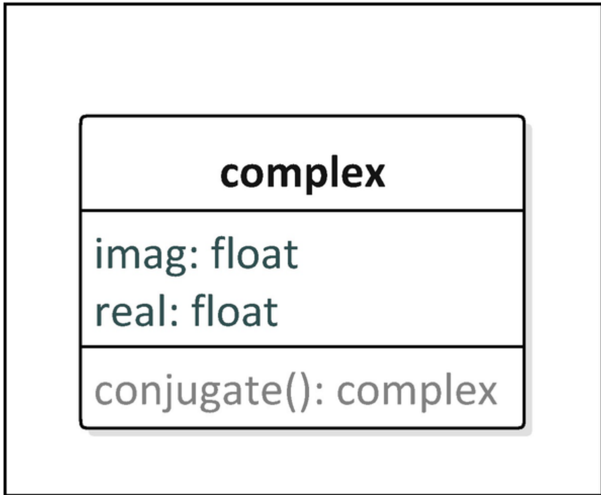
Figure 3-3 Complex class
