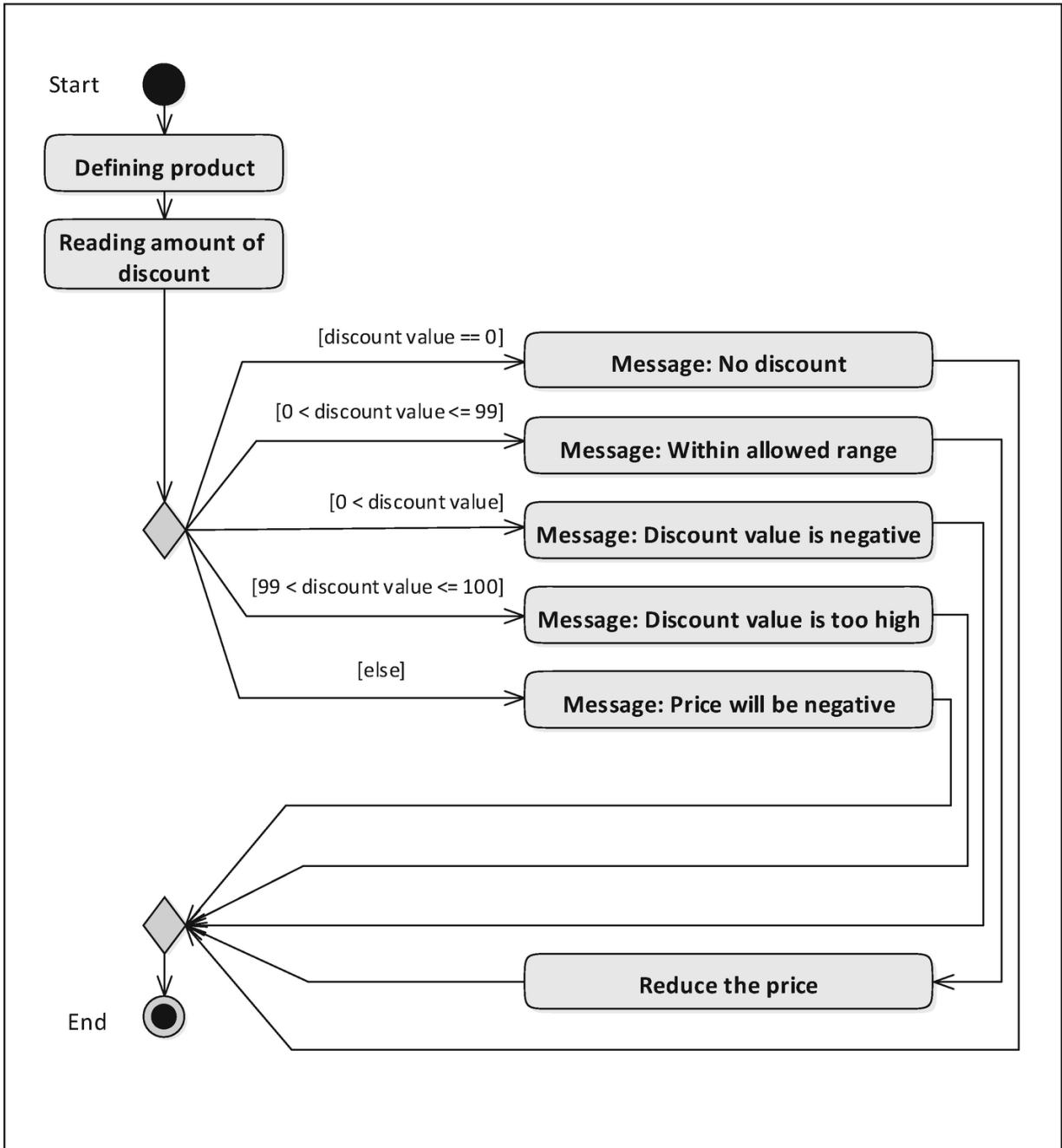
Figure 4-4 match statement with guard conditions
