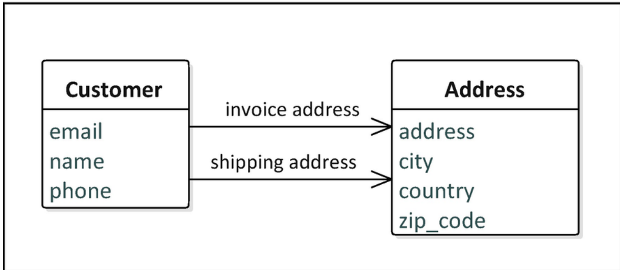
Figure 3-6 Customer class
