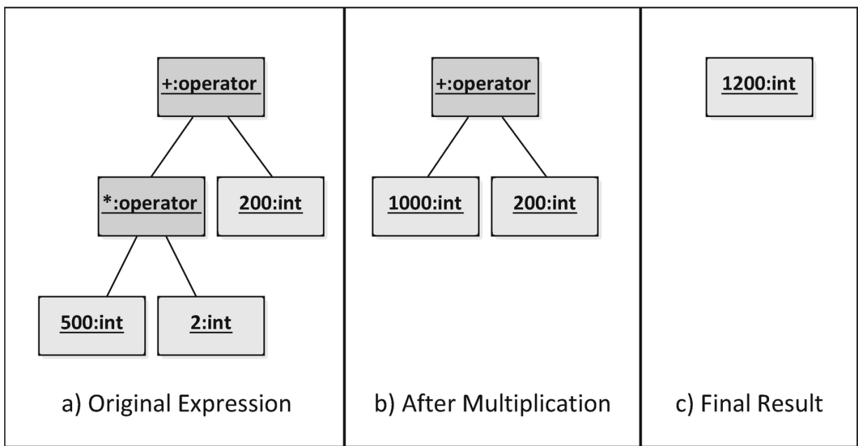
Figures 1-1a, 1-1b, and 1-1c Simple expression
