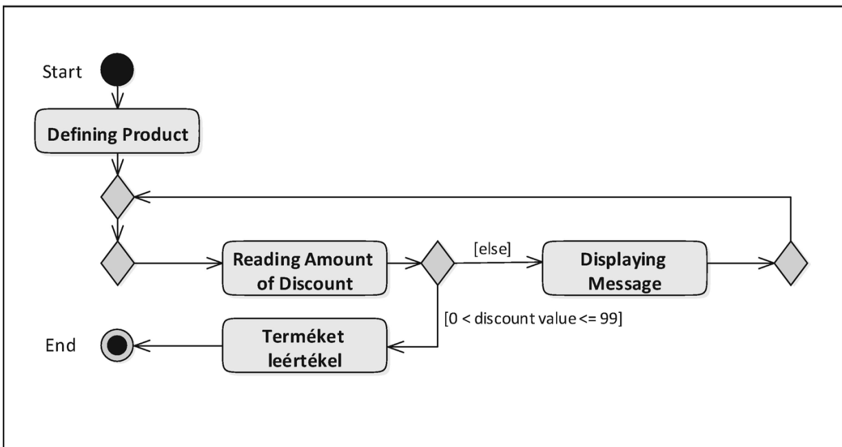
Figure 4-7 while statement as an infinite loop
