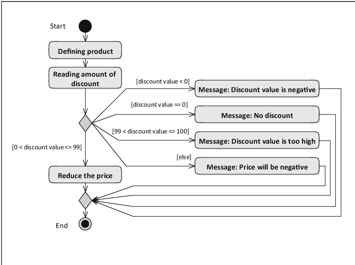
Figure 4-2 if statement with multiple branches
